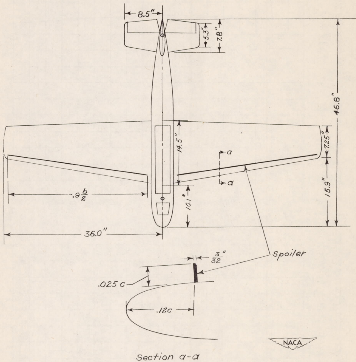
Figure 3.- Test model with spoiler detail.
