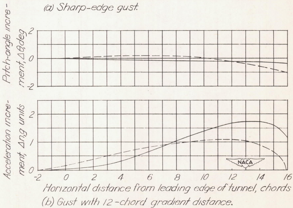
Figure 4.- History of events in test gusts.
