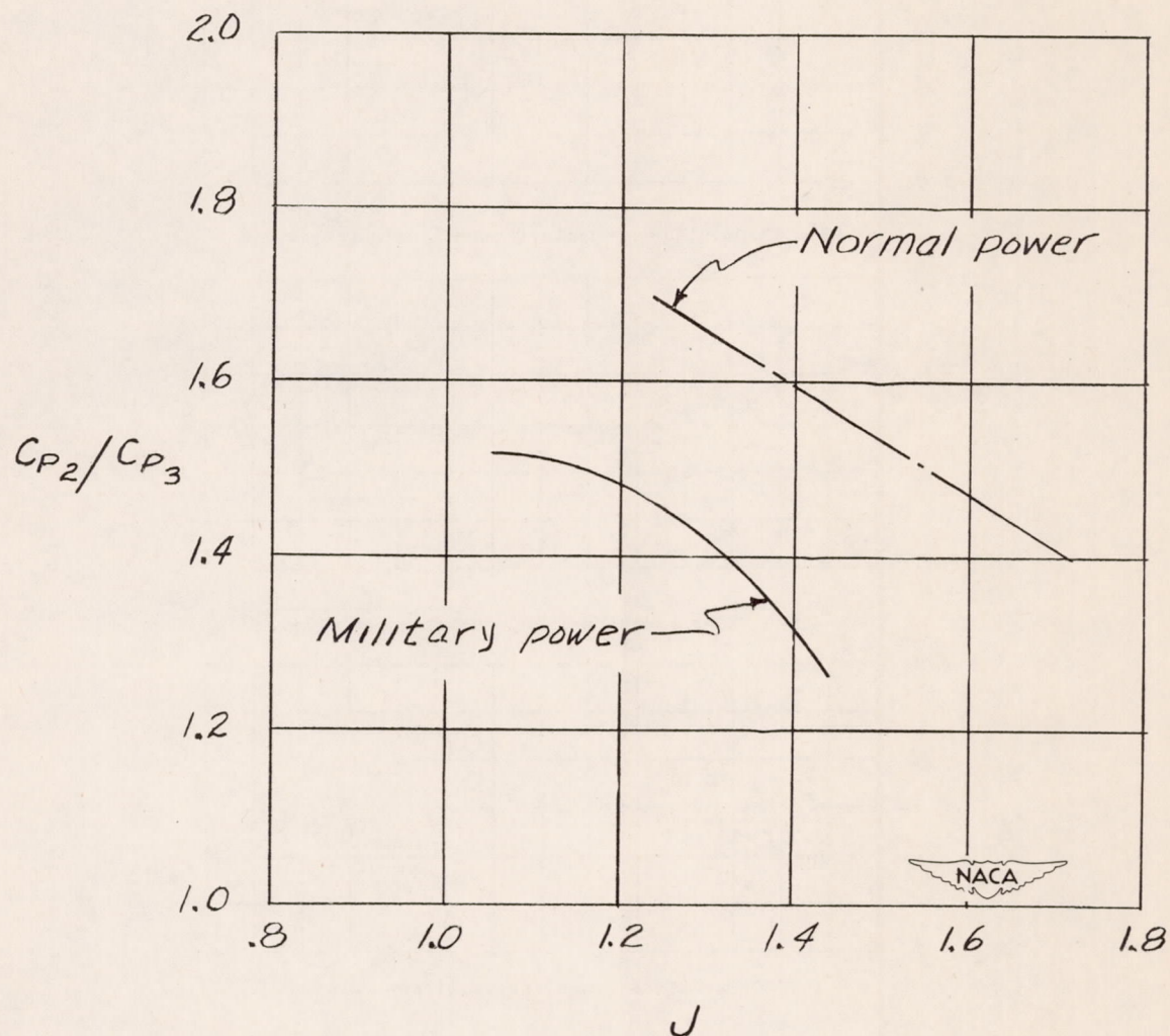
Figure 8.- Ratio of power coefficient per blade for two-blade operation to three-blade operation for various advance ratios in climbs.
