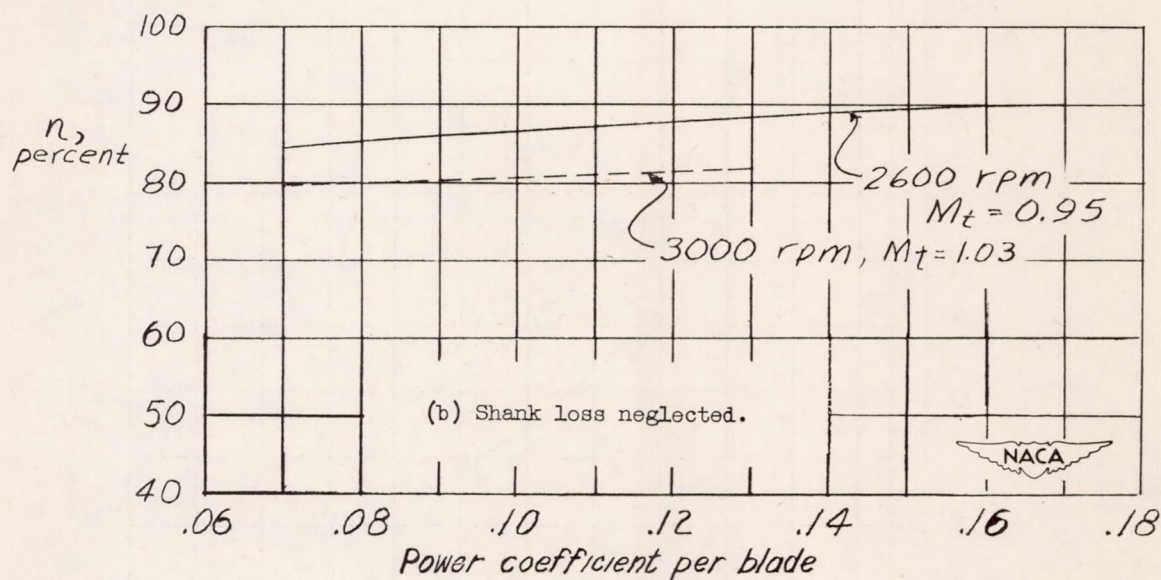
Figure 15.- Effect of power loading on efficiency of tested propeller at airplane Mach number of 0.7.
