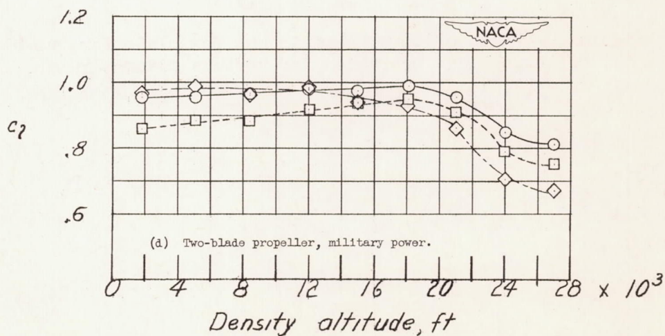
Figure 9.- Variation of c_l of tested propeller with altitude in climbs.
