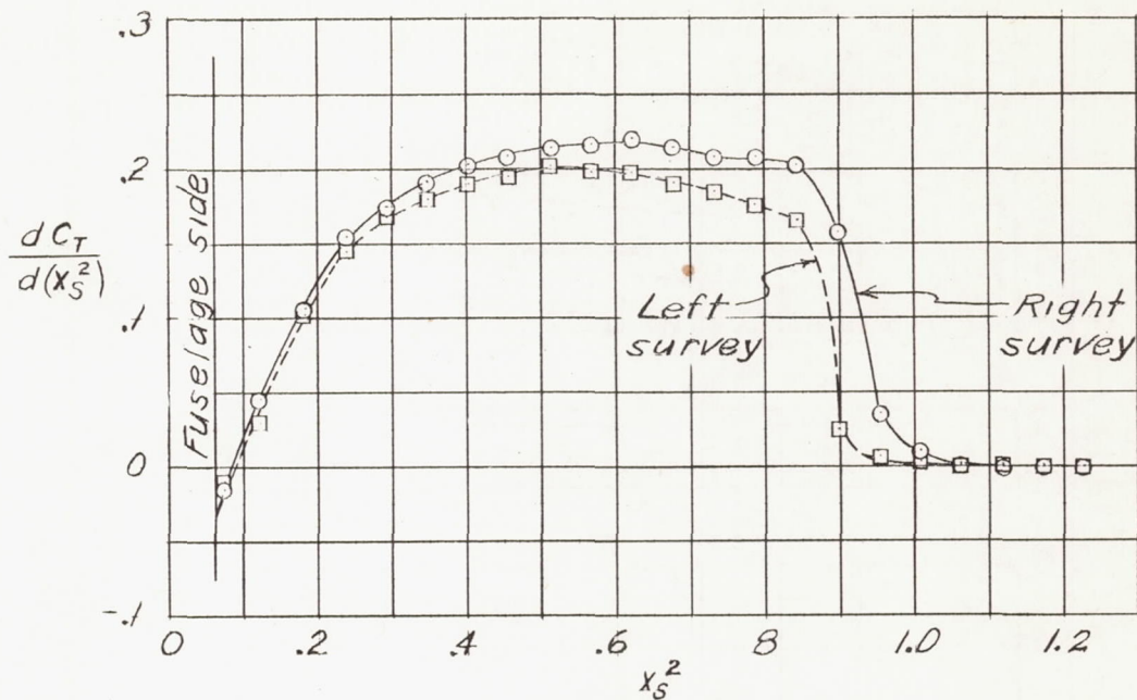
(a) Test conditions: \eta = 82.8 percent; J = 1.09 ; C_P = 0.183 ; C_T = 0.139 ; M = 0.242 ; M_t = 0.739 .
