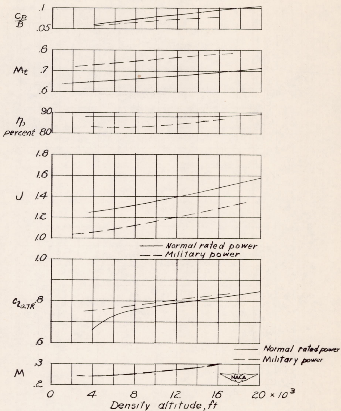
Figure 10.- Comparison of results for normal rated and military power in climb with three-blade propeller.
