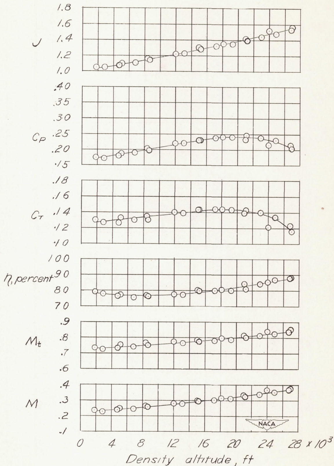
Figure 7.- Military-power climb at an indicated airspeed of 165 miles per hour with two-blade propeller on a fighter-type airplane.
