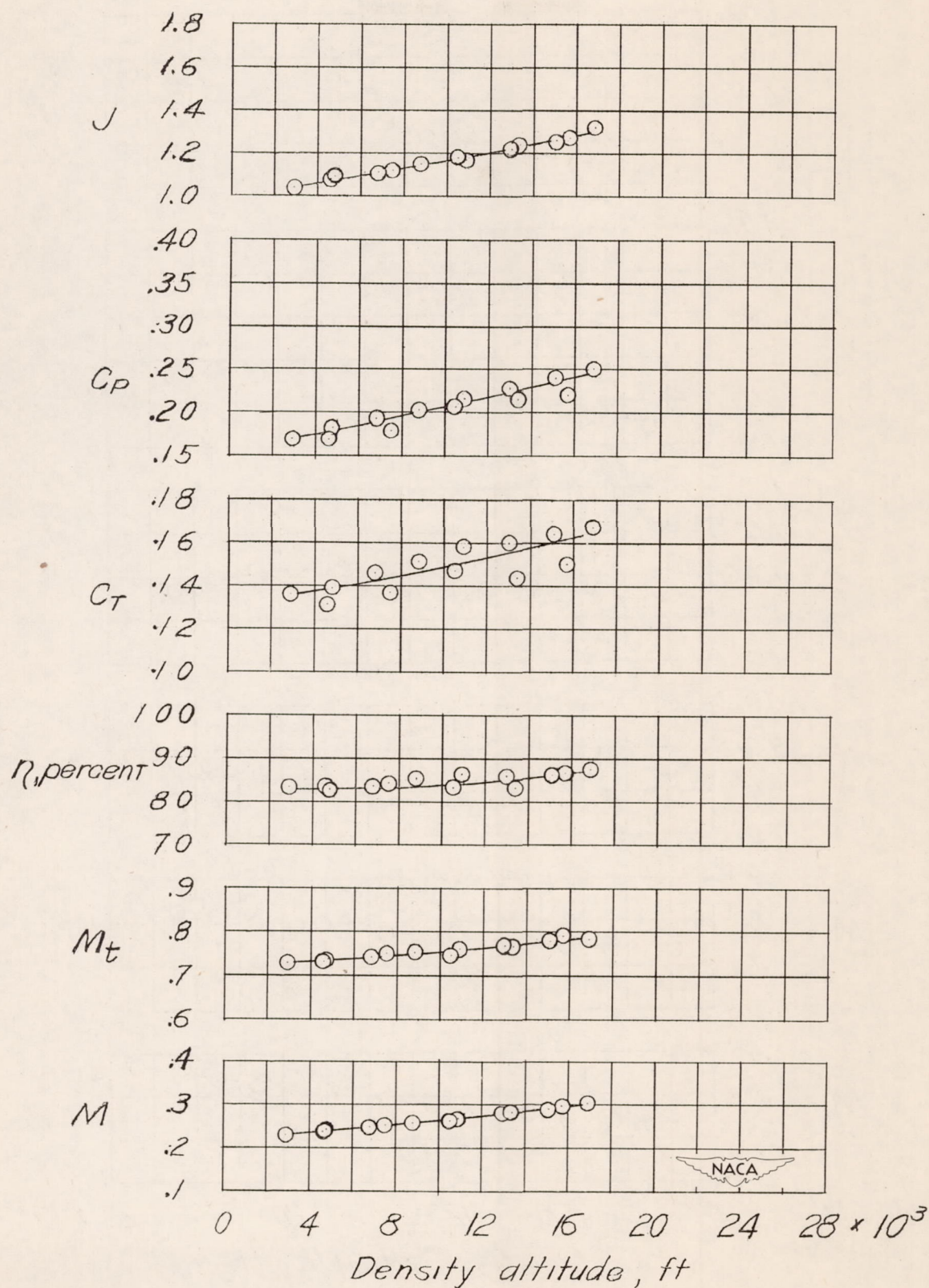
Figure 6.- Military-power climb at an indicated airspeed of 165 miles per hour with three-blade propeller on a fighter-type airplane.
