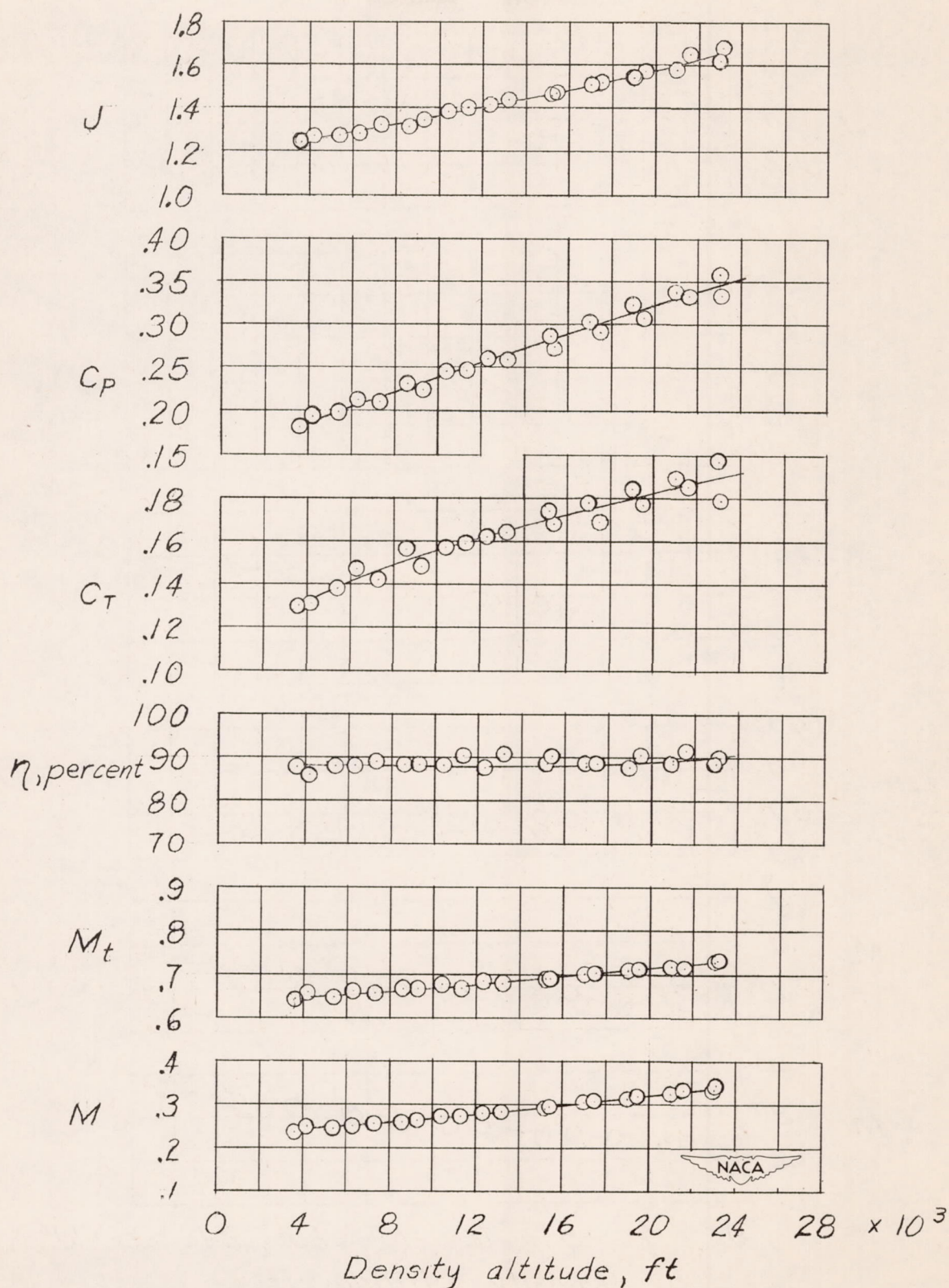
Figure 4.- Normal-rated-power climb at an indicated airspeed of 165 miles per hour with three-blade propeller on a fighter-type airplane.
