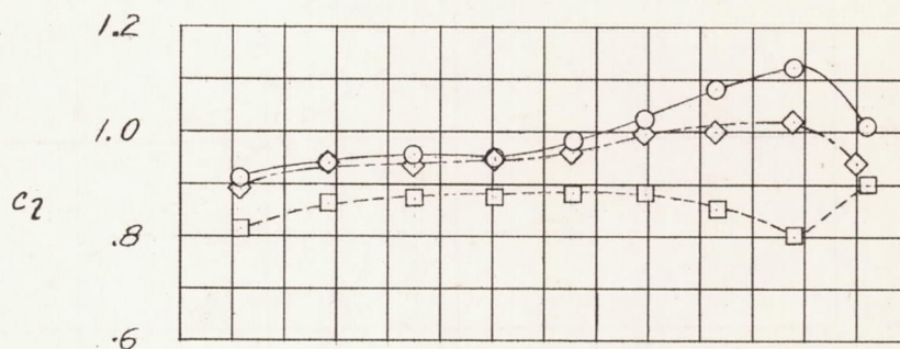
(b) Two-blade propeller, normal rated power.
