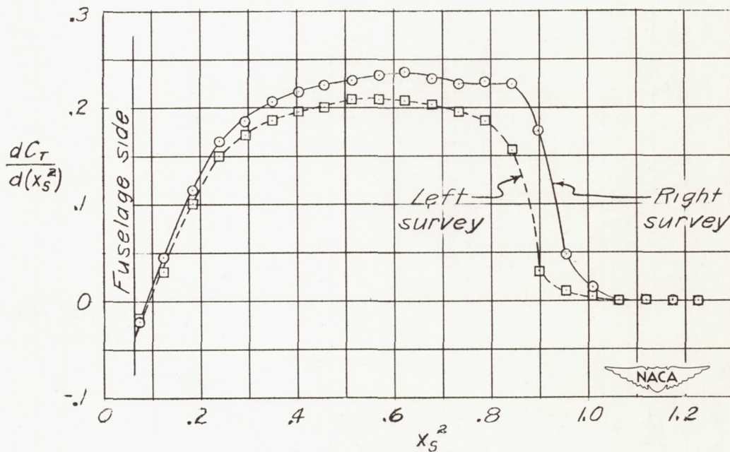
(b) Test conditions: \eta = 85.3 percent; J = 1.15 ; C_P = 0.202 ; C_T = 0.151 ; M = 0.259 ; M_t = 0.754 .
