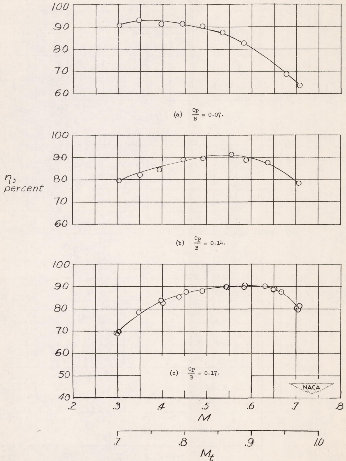
Figure 13.- Variation of efficiency of tested propeller with Mach number at engine speed of 2600 rpm.
