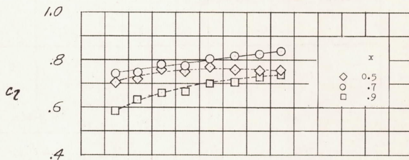
(c) Three-blade propeller, military power.
