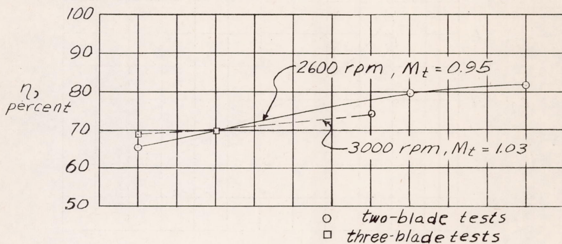
(a) Propeller as tested, with shank loss.
