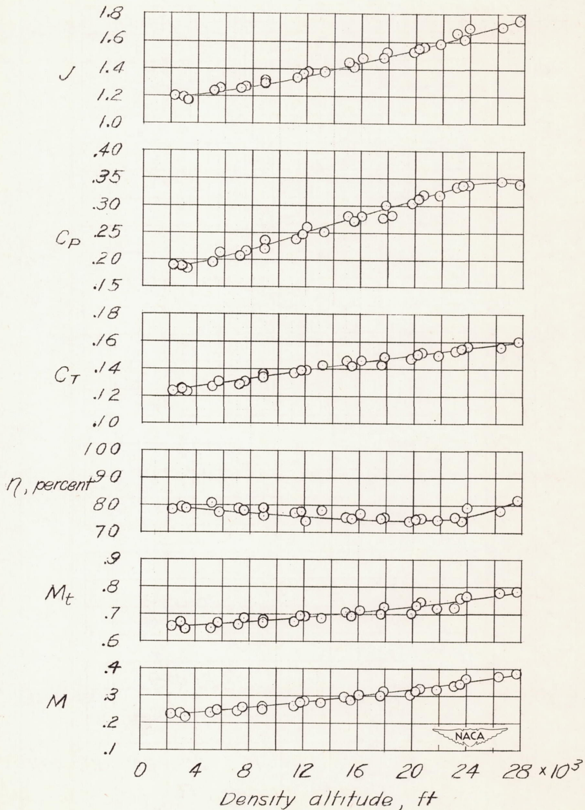
Figure 5.- Normal-rated-power climb at an indicated airspeed of 165 miles per hour with two-blade propeller on a fighter-type airplane.
