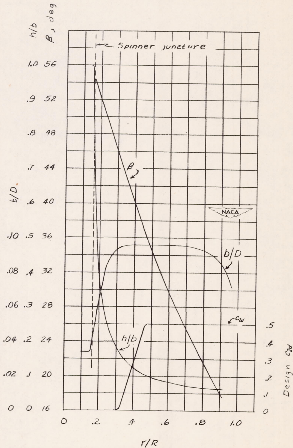
Figure 1.- Blade-form curves of propeller tested.
