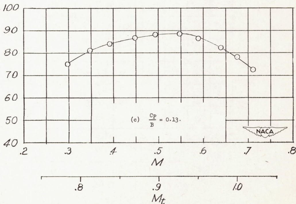
Figure 14.- Variation of efficiency of tested propeller with Mach number at engine speed of 3000 rpm.
