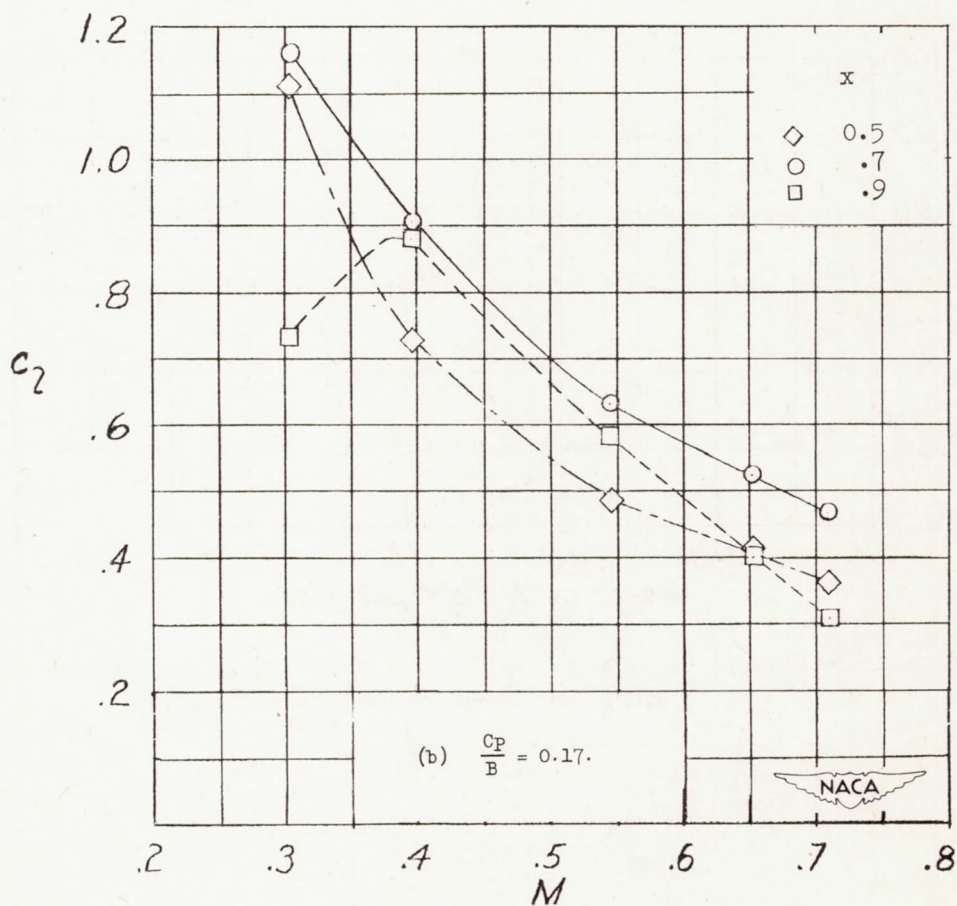
Figure 16.- Variation of c_l of propeller tested with Mach number at high speeds. Engine speed, 2600 rpm.
