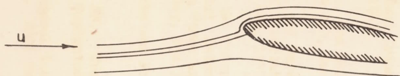
BOUNDARY-LAYER FLOW FROM THE STAGNATION POINT AROUND THE NOSE OF AN AIRFOIL AT A SMALL ANGLE OF ATTACK.
