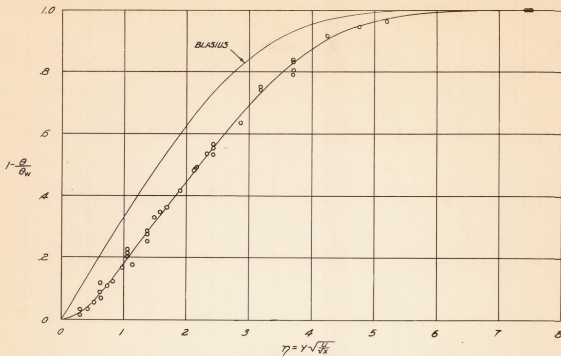
FIGURE 11.~ TEMPERATURE DISTRIBUTION IN THE BOUNDARY LAYER OF THE HEATED PLATE. REGULAR PROFILE CONFIRMING ANALYTICAL CONSIDERATIONS.
