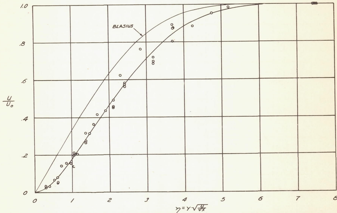
FIGURE 10.- VELOCITY DISTRIBUTION IN THE BOUNDARY LAYER OF THE HEATED PLATE. REGULAR PROFILE CONFIRMING ANALYTICAL CONSIDERATIONS.
