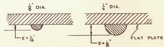
FIGURE 2c.- MOUNTING OF ROUGHNESS ELEMENTS.
