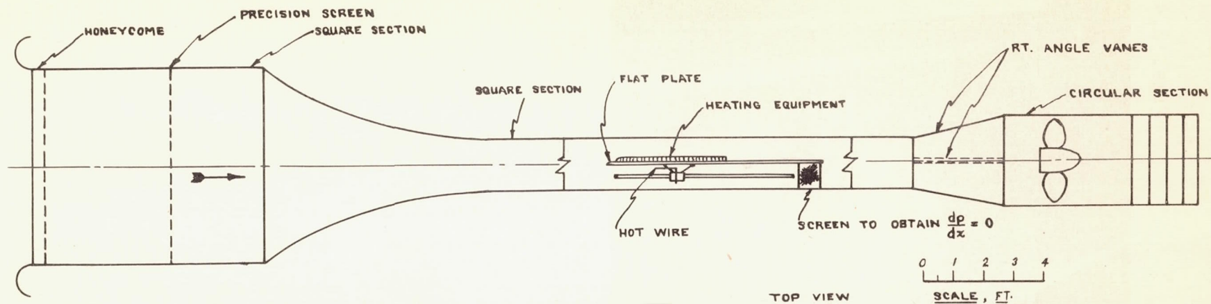
FIGURE 2a.- SCHEMATIC DIAGRAM OF THE WIND TUNNEL.
