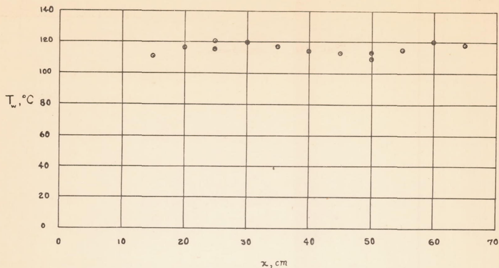
FIGURE 6. - TEMPERATURE DISTRIBUTION ALONG THE HEATED PLATE.
