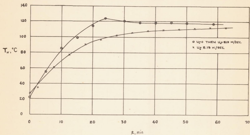
FIGURE 7. - TWO METHODS OF HEATING THE FLAT PLATE.
