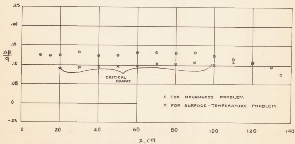
FIGURE 8. - PRESSURE DISTRIBUTION ALONG THE TEST PLATE.
