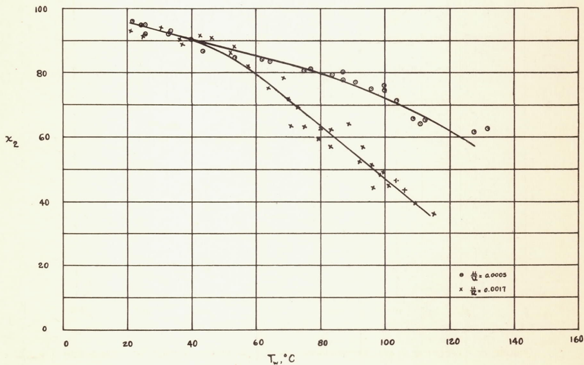
FIGURE 13. — EFFECT OF PLATE TEMPERATURE ON TRANSITION.
