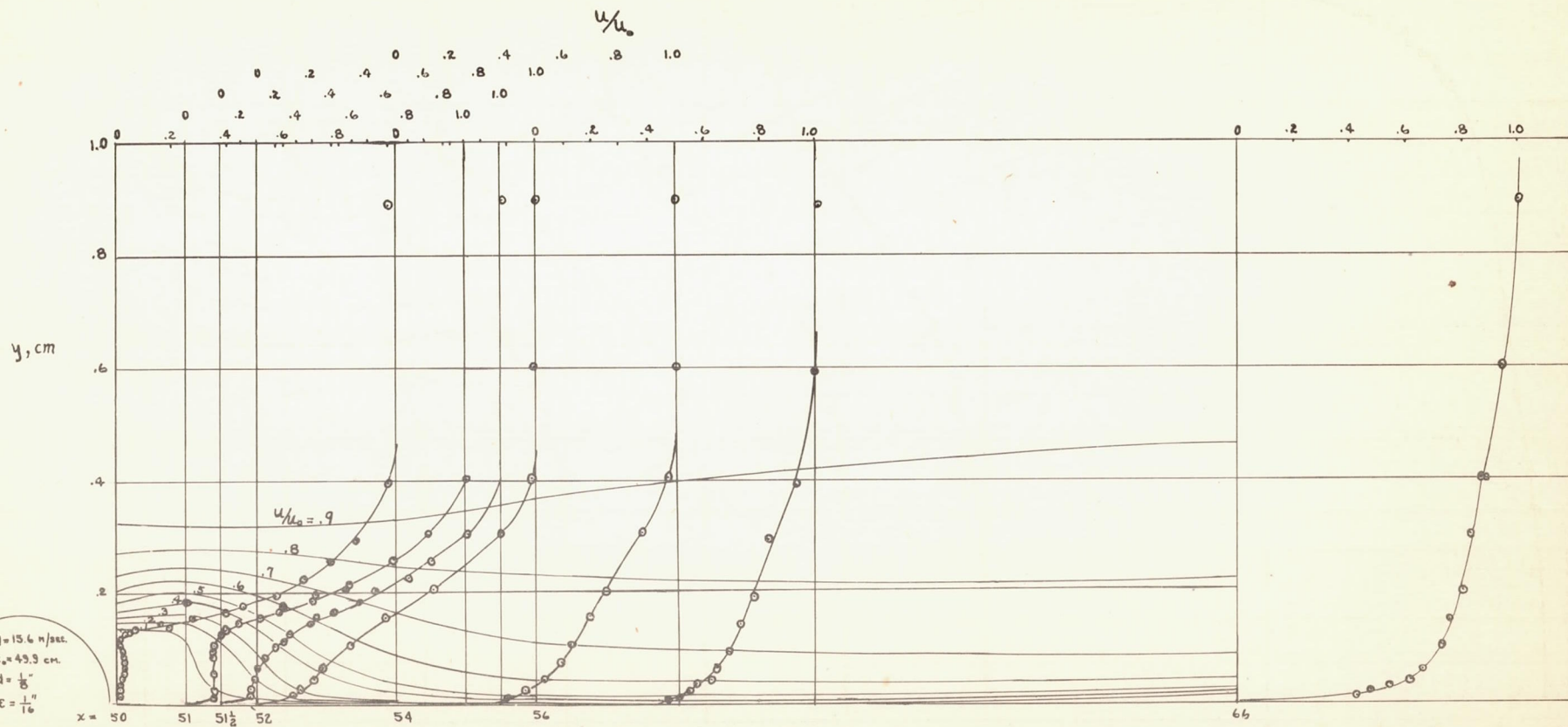
FIGURE 16c.—VELOCITY PROFILES DOWNSTREAM FROM A SMALL ROUGHNESS ELEMENT.
