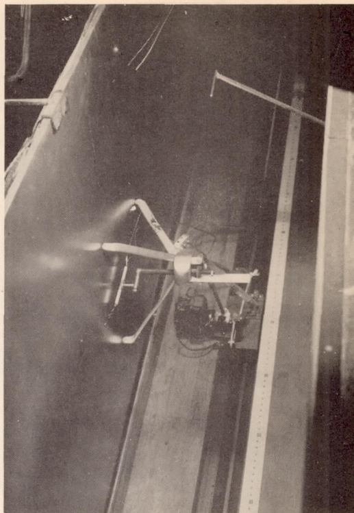
Figure 4.- Traversing mechanism.
