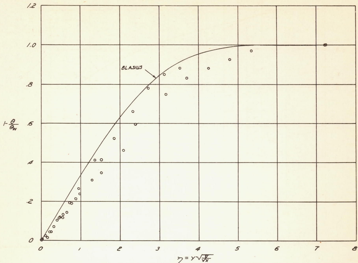
FIGURE 12b. — TEMPERATURE DISTRIBUTION IN THE BOUNDARY LAYER OF THE HEATED PLATE. UNPREDICTED PROFILE DUE PROBABLY TO SECONDARY FLOW.
