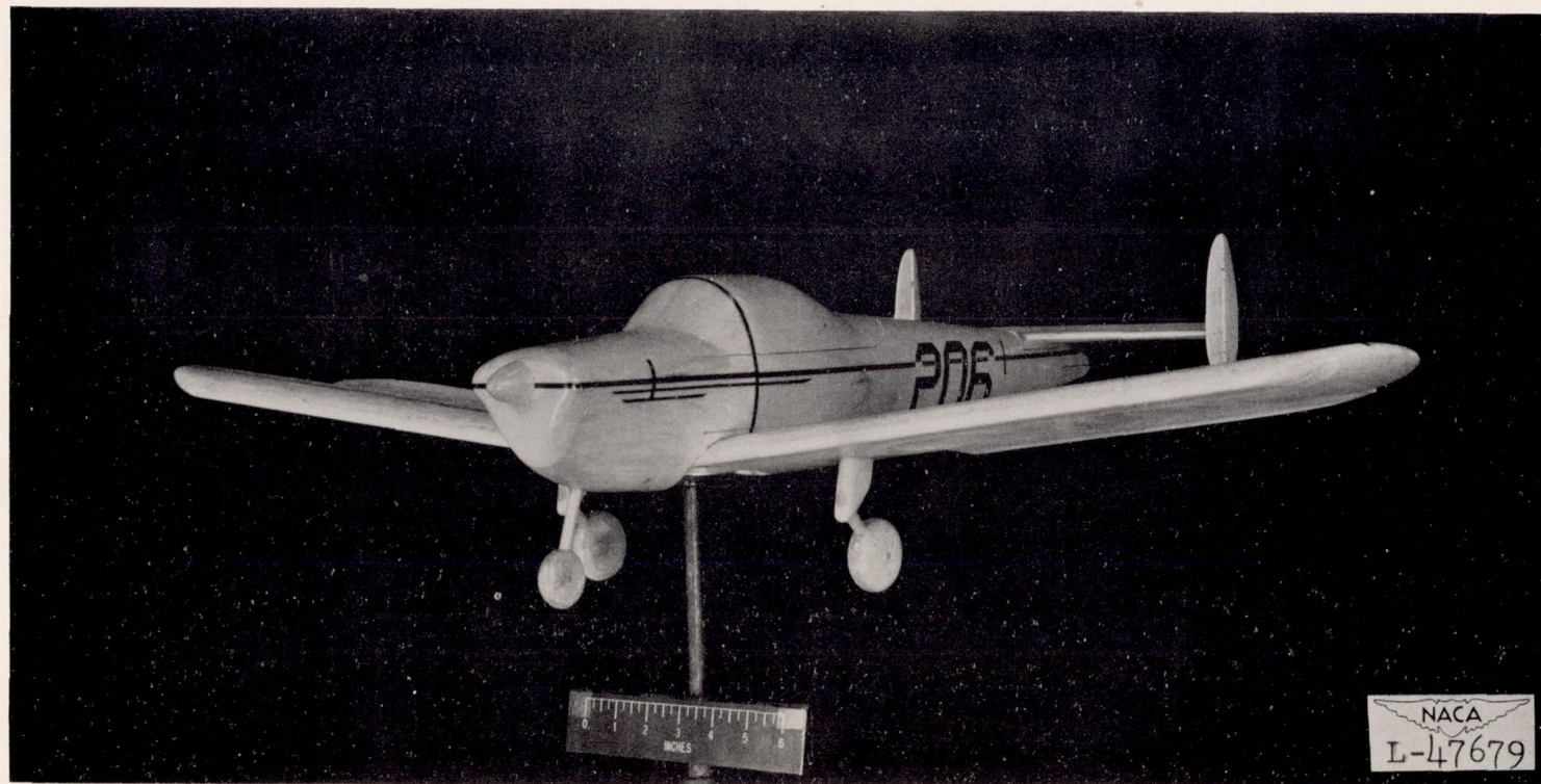
Figure 2.- Photograph of the model as tested in the Langley 20-foot free-spinning tunnel.
