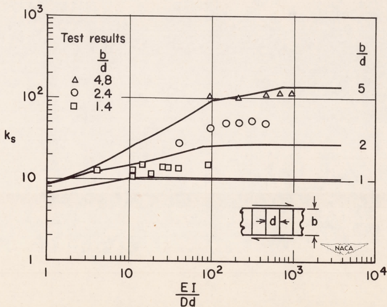
Figure 2.- Theoretical critical shear-stress coefficient \left(k_s = \frac{\pi^2 b^2}{\pi^2 D}\right) compared with experimental results for infinitely long, transversely stiffened plates with various panel aspect ratios \frac{b}{d} and stiffness ratios \frac{EI}{Dd} .
