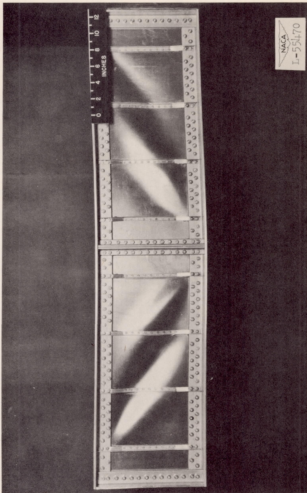
Figure 3.- Thick web beam (with uprights connected to flanges) after failure.
