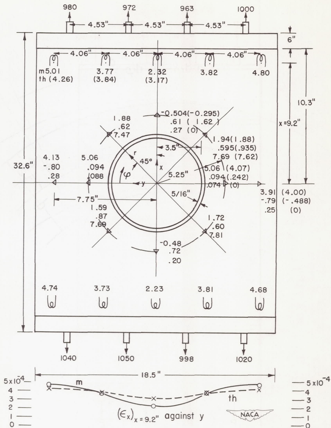
Figure 7.- Strain measurements on plane sheet with reinforced cutout.
