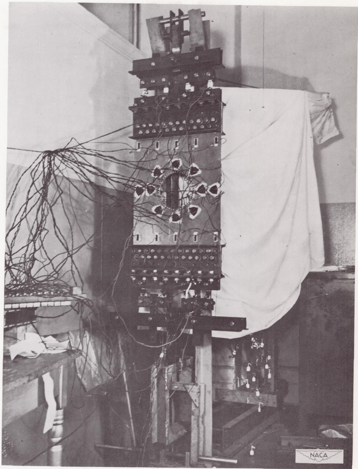
Figure 4.- Test specimen.
