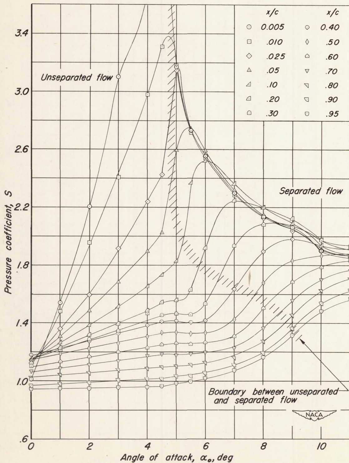
Figure 5.—Variation of pressure coefficient with angle of attack for various chordwise stations.
