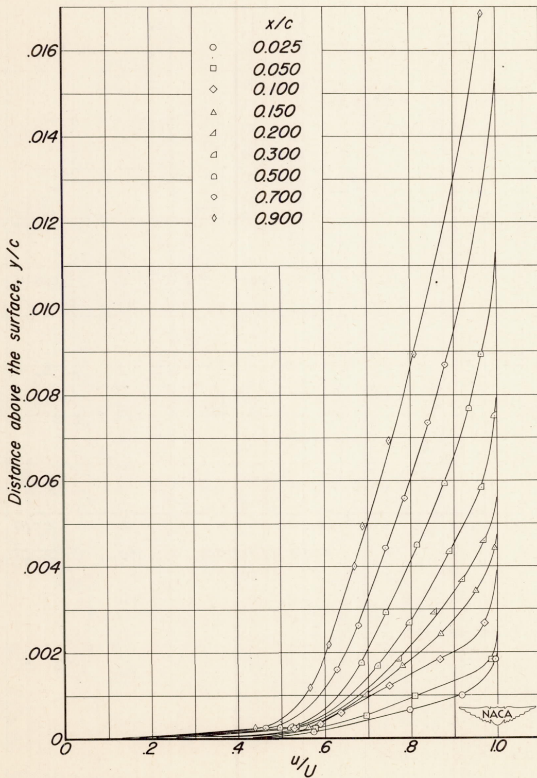
Figure 6.—Boundary-layer velocity profiles.
