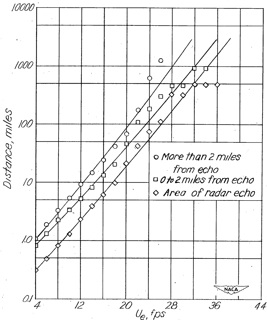
Figure 1.— Average number of miles required to exceed a given gust velocity.
