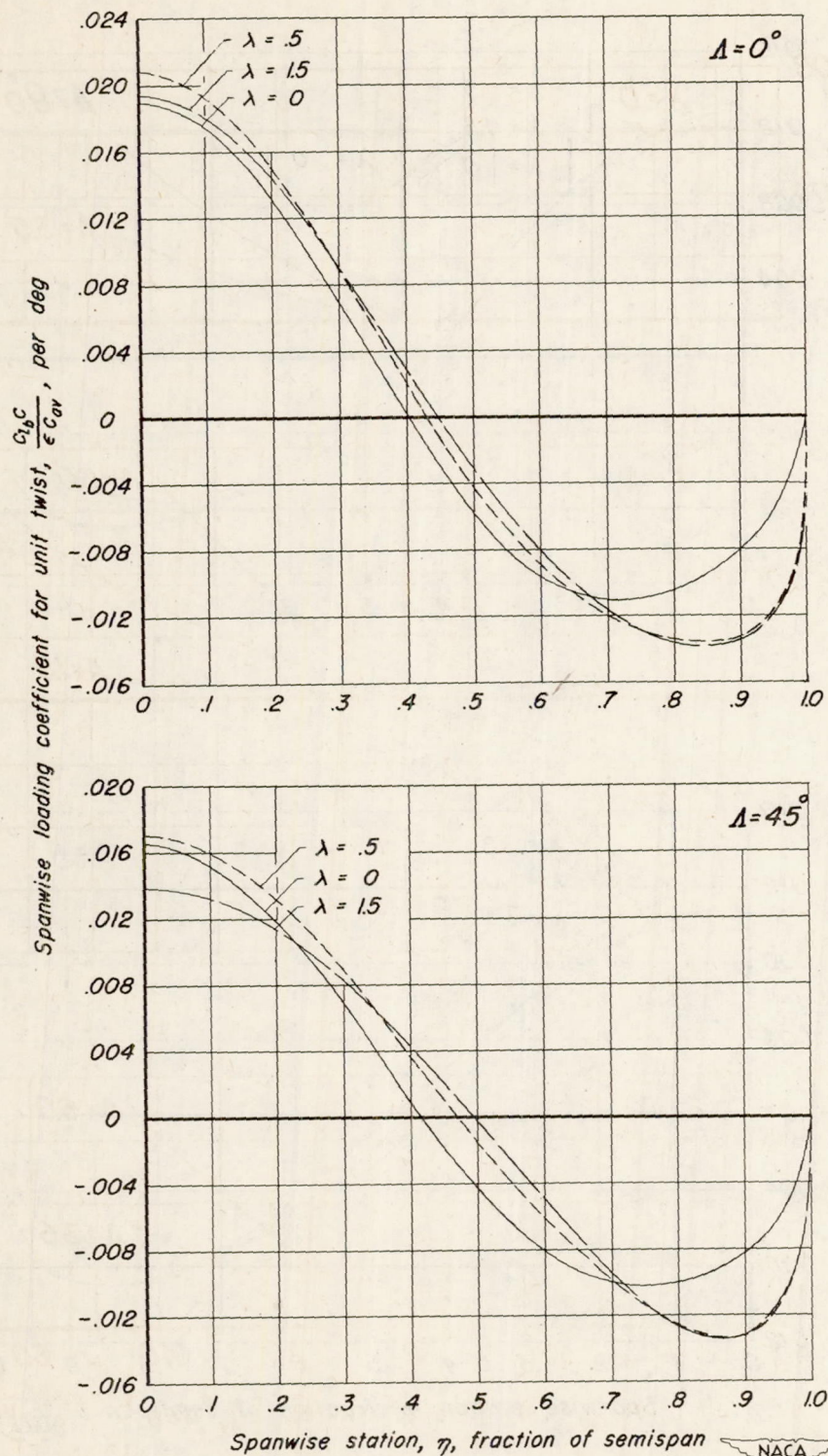
Figure 7.—The effect of taper ratio on the basic loading of wings having an aspect ratio of 6.0.
