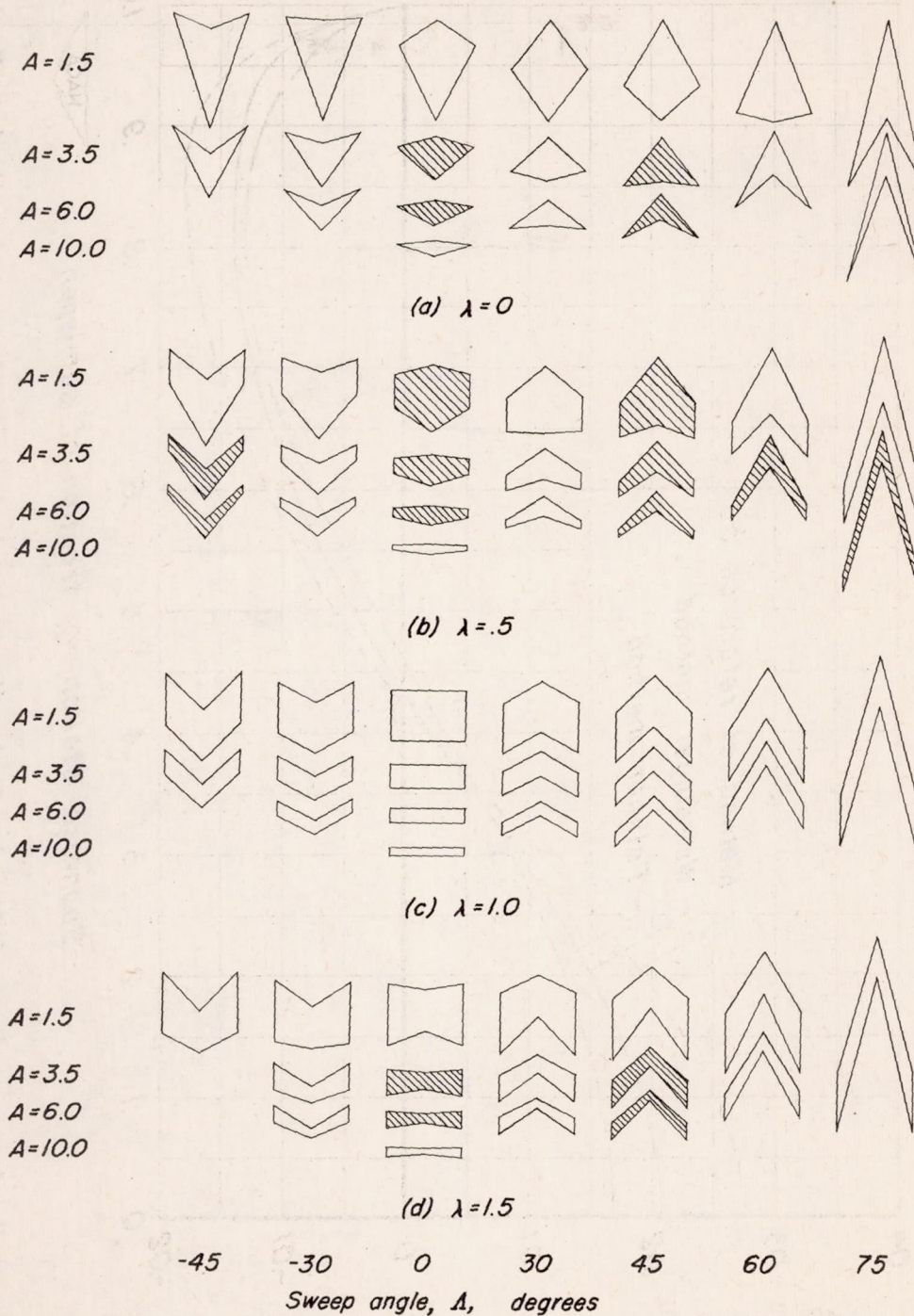
Figure 2.— Approximate range of planforms for which values of coefficients a_{\eta n} are presented in table I.
