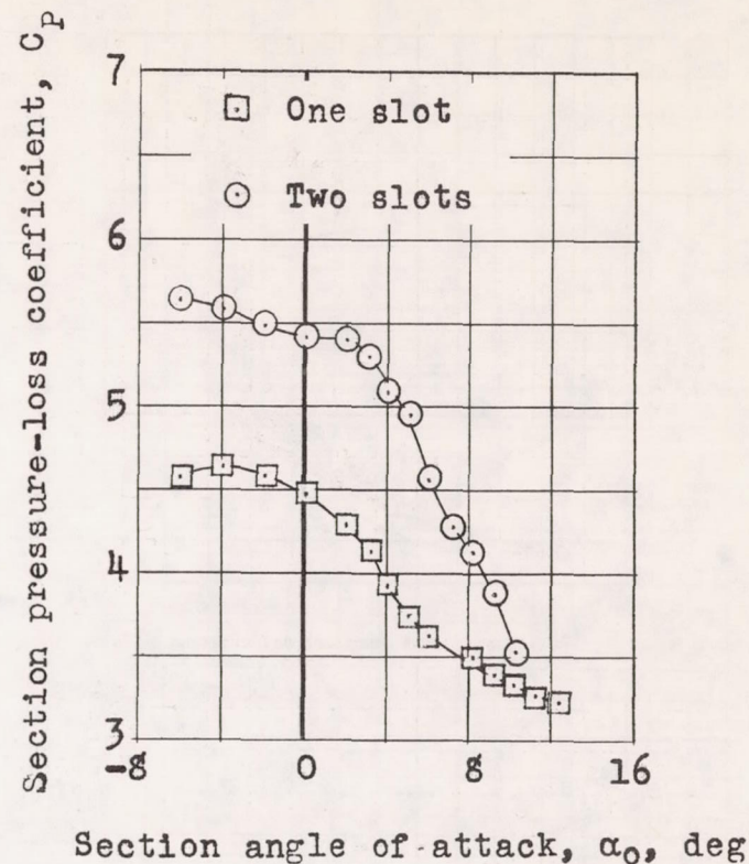
Figure 10.- Effect on maximum section lift coefficient and section pressure-loss coefficient of sealing the rear slot of the NACA 65 2 -415 airfoil section in the smooth condition with two boundary-layer control slots on a 0.25c plain flap. \delta_f = 50^\circ ; C_Q = 0.020 ; R = 2.2 \times 10^6 .
