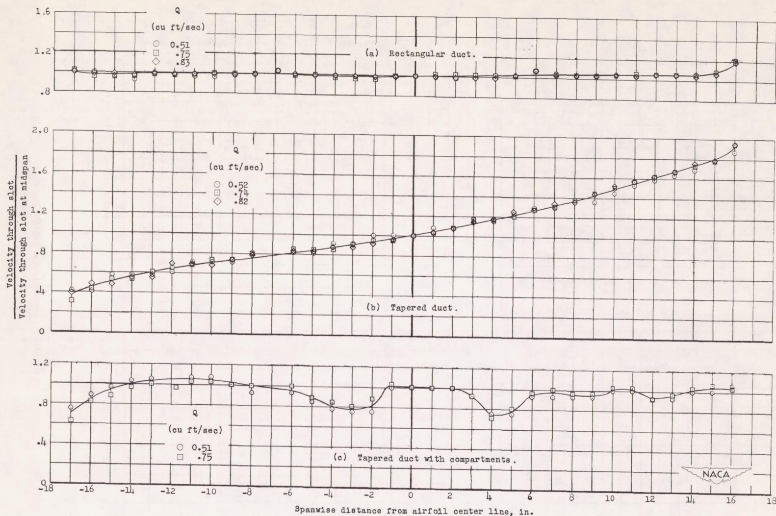
Figure 15.- Spanwise distribution of flow along a rectangular slot connected to three different types of ducts.
