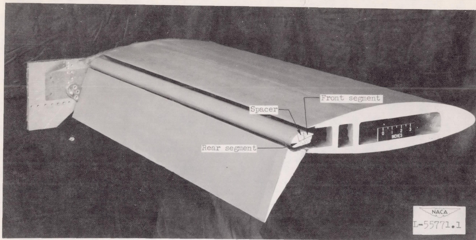
Figure 4.- Three-quarter rear view of the model of the NACA 65 2 -415 airfoil section with two boundary-layer control slots on a 0.25c plain flap.
