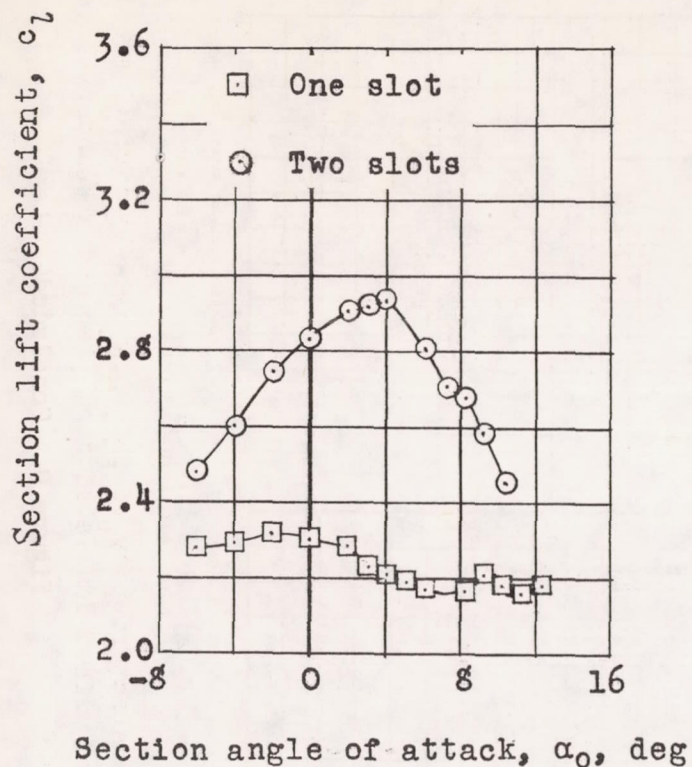
Figure 10.- Effect on maximum section lift coefficient and section pressure-loss coefficient of sealing the rear slot of the NACA 65 2 -415 airfoil section in the smooth condition with two boundary-layer control slots on a 0.25c plain flap. \delta_f = 50^\circ ; C_Q = 0.020 ; R = 2.2 \times 10^6 .
