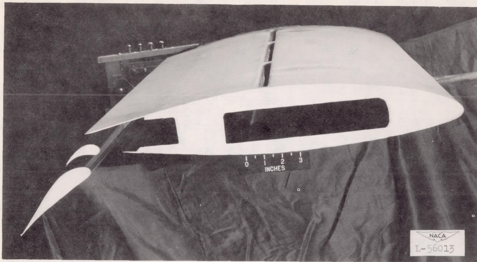
Figure 2.- End view of the model of the NACA 65 2 -415 airfoil section with a double slotted flap and a boundary-layer control slot on the upper surface at 0.45c.
