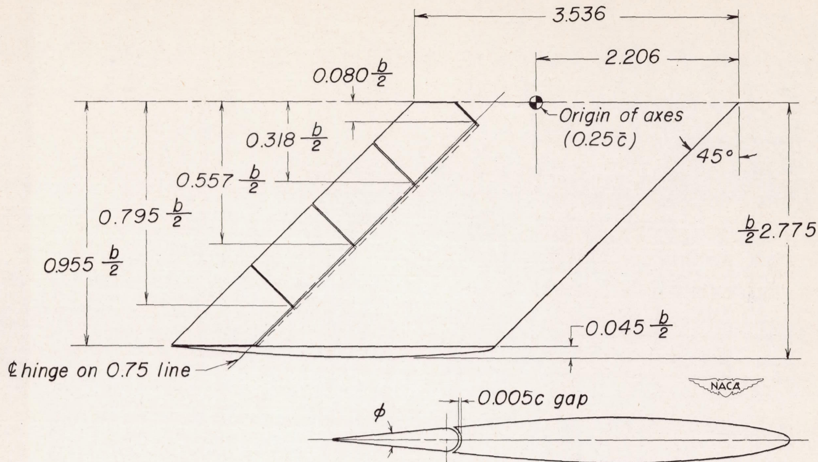
Figure 1.- Drawing of the 45° sweptback-semispan-wing model having an aspect ratio of 1.59. NACA 64A010 airfoil section normal to leading edge. Trailing-edge angle \phi measured perpendicular to hinge axis is 12.0^\circ and measured parallel to free stream is 8.5^\circ . (All dimensions are in feet.)
