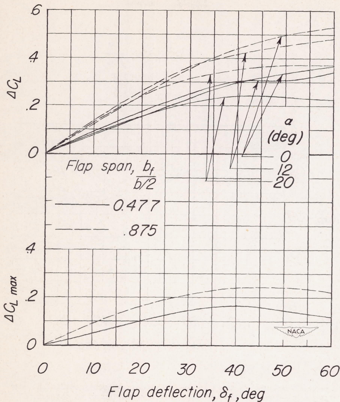
Figure 7.- Variation of the incremental lift coefficient with flap deflection for the 45^\circ sweptback wing having an aspect ratio of 1.59 and equipped with inboard half-span ( b_f = 0.477\frac{b}{2} ; y_{f_0} = 0.557\frac{b}{2} ) and full-span ( b_f = 0.875\frac{b}{2} ; y_{f_0} = 0.955\frac{b}{2} ) flaps. y_{f_1} = 0.080\frac{b}{2} .
