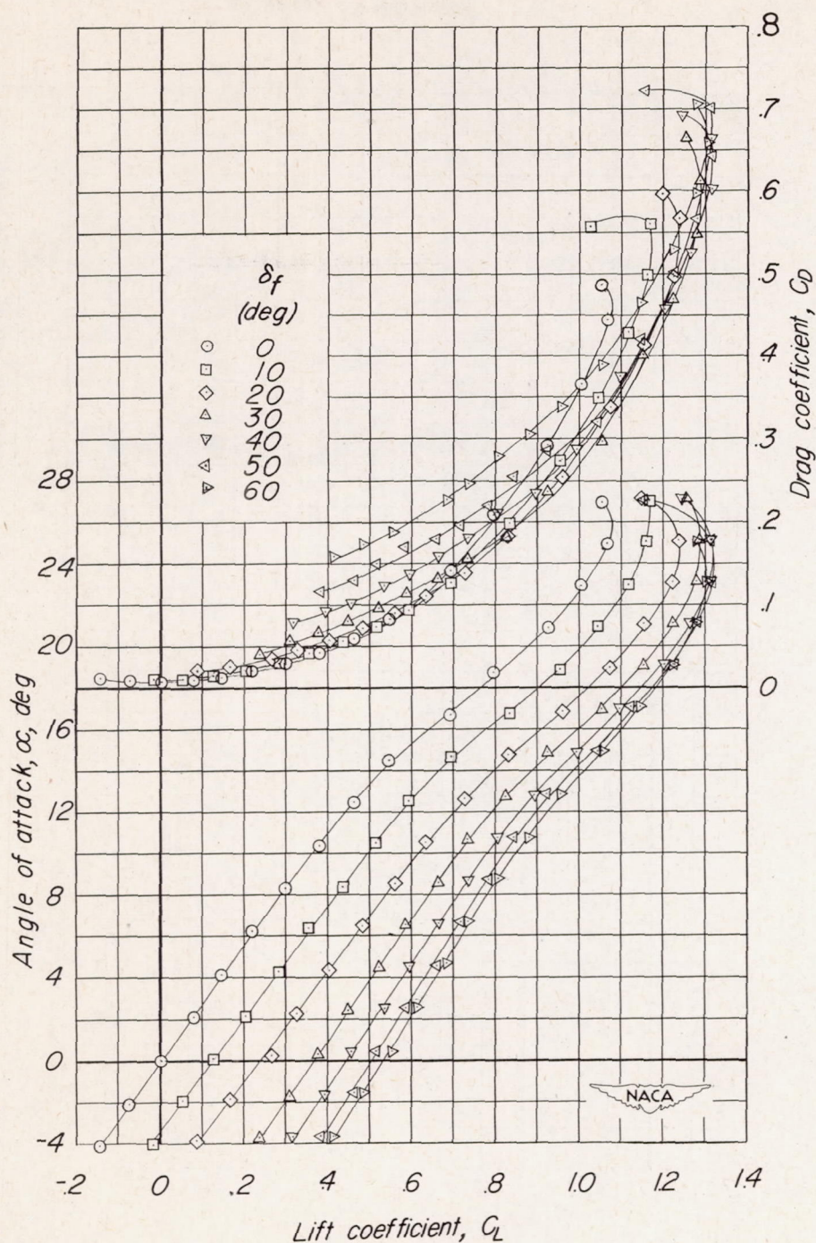
Figure 4.- Effect of flap deflection on the aerodynamic characteristics in pitch of the 45^\circ sweptback wing having an aspect ratio of 1.59 and equipped with full-span flaps ( b_f = 0.875 \frac{b}{2} ). y_{f1} = 0.080 \frac{b}{2} ; y_{f0} = 0.955 \frac{b}{2} .
