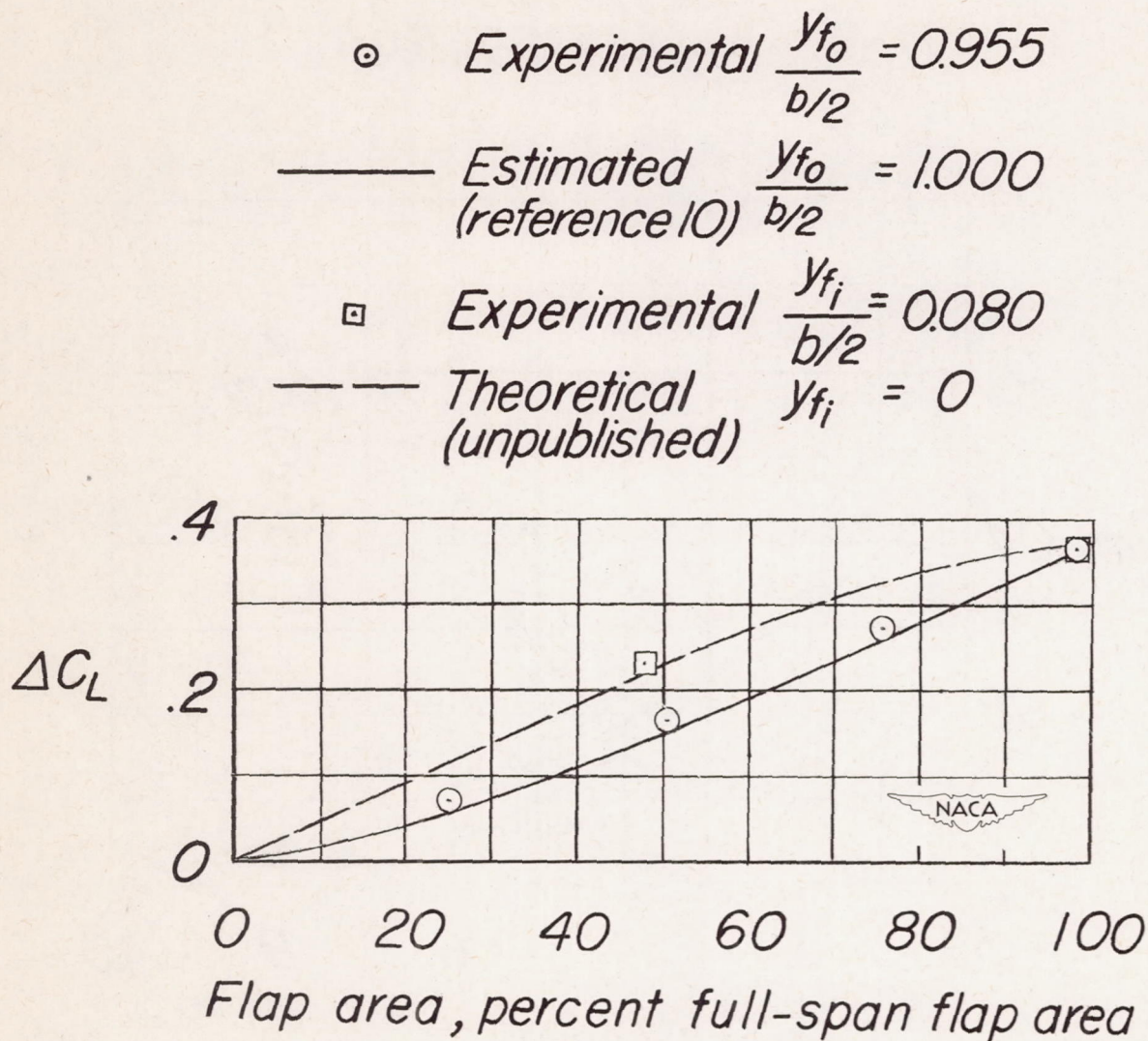
Figure 9.- Effect of flap span (expressed as percent of full-span flap area) and spanwise location on the incremental lift coefficient produced by a flap deflection of 30^\circ of the 45^\circ sweptback wing having an aspect ratio of 1.59. \alpha = 0^\circ .
