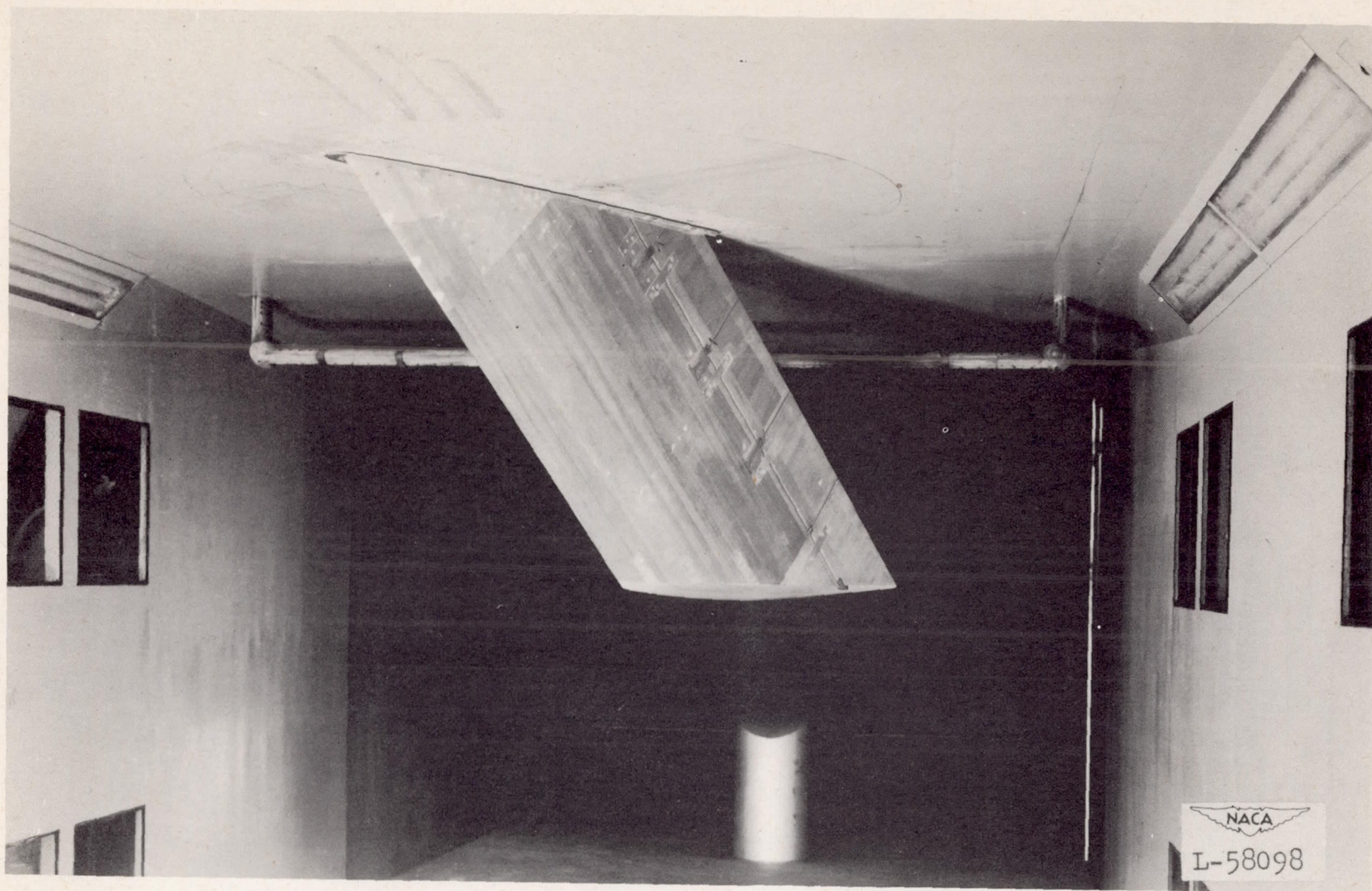
Figure 2.- The 45^\circ sweptback-semispan-wing model having an aspect ratio of 1.59 mounted in the Langley 300 MPH 7- by 10-foot tunnel.
