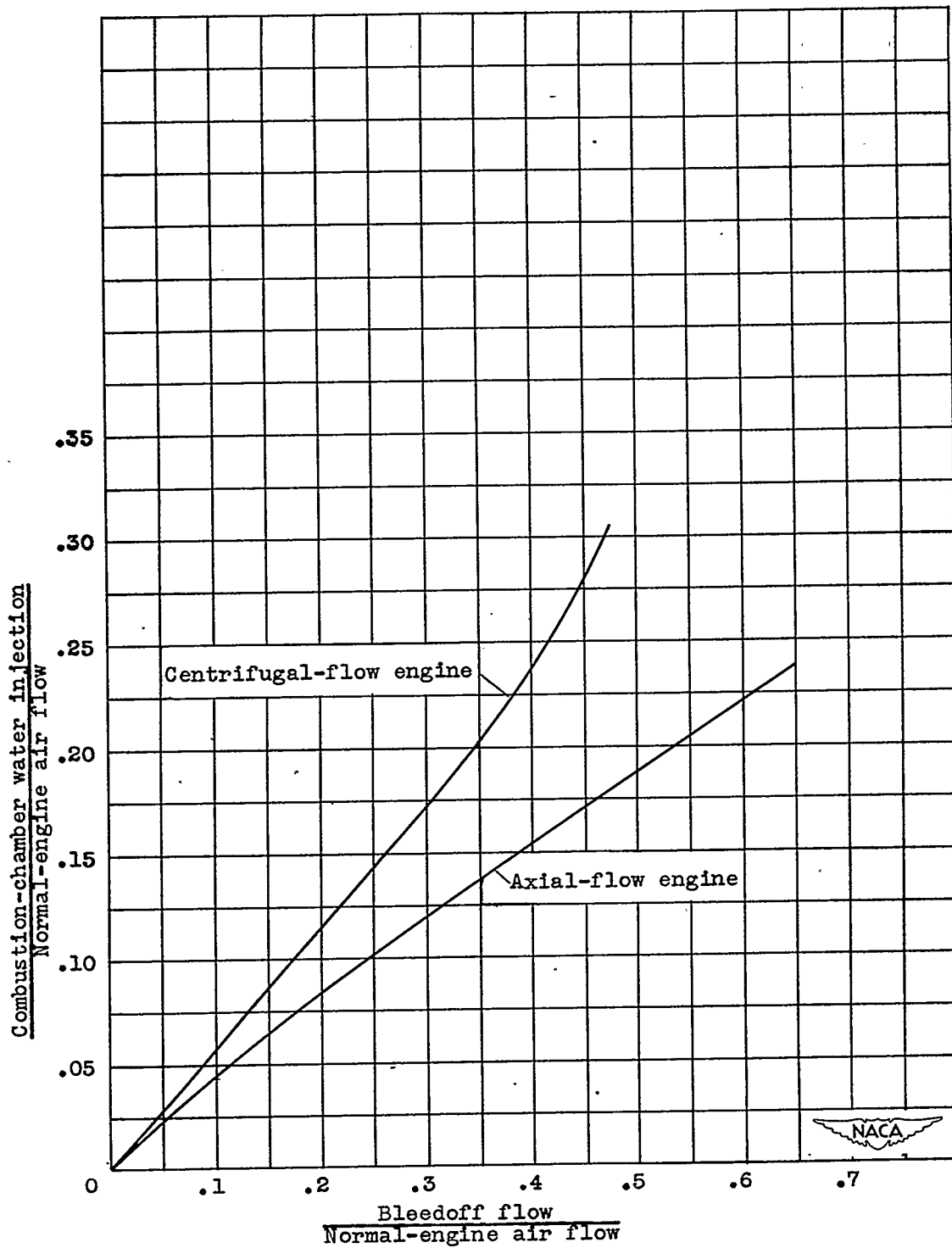
Figure 17. - Variation of water-injection rate into primary-engine combustion chambers with bleedoff flow. Flight Mach number, 0; altitude, sea level.
