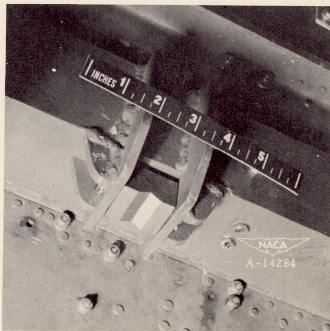
(c) Front V-block.
