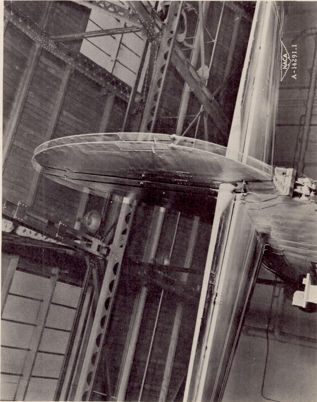
Figure 10.-- Double exposure showing oscillation in yaw.
