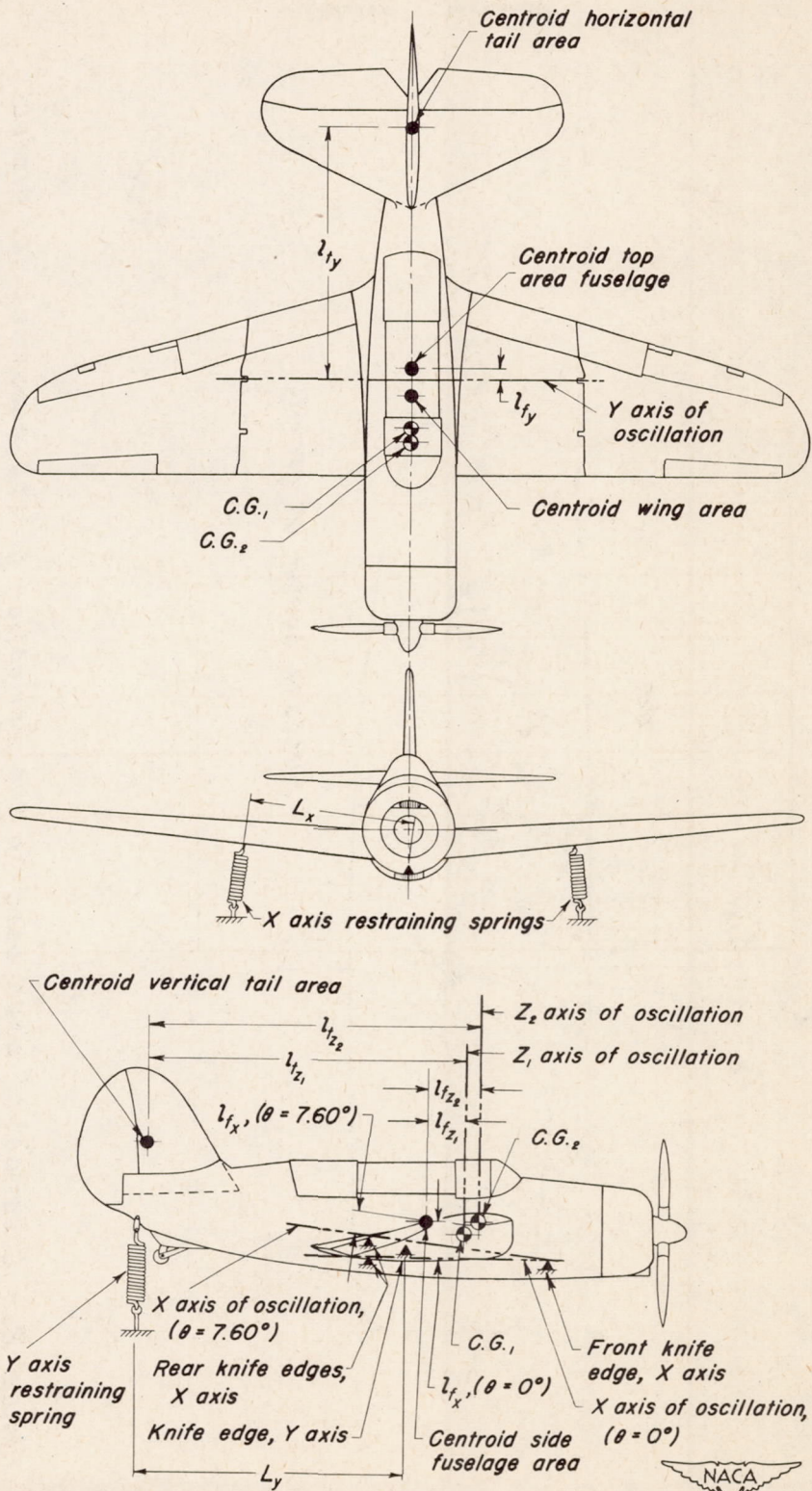
Figure 1.- Sketch of test airplane showing pertinent symbols for moment-of-inertia measurements.
