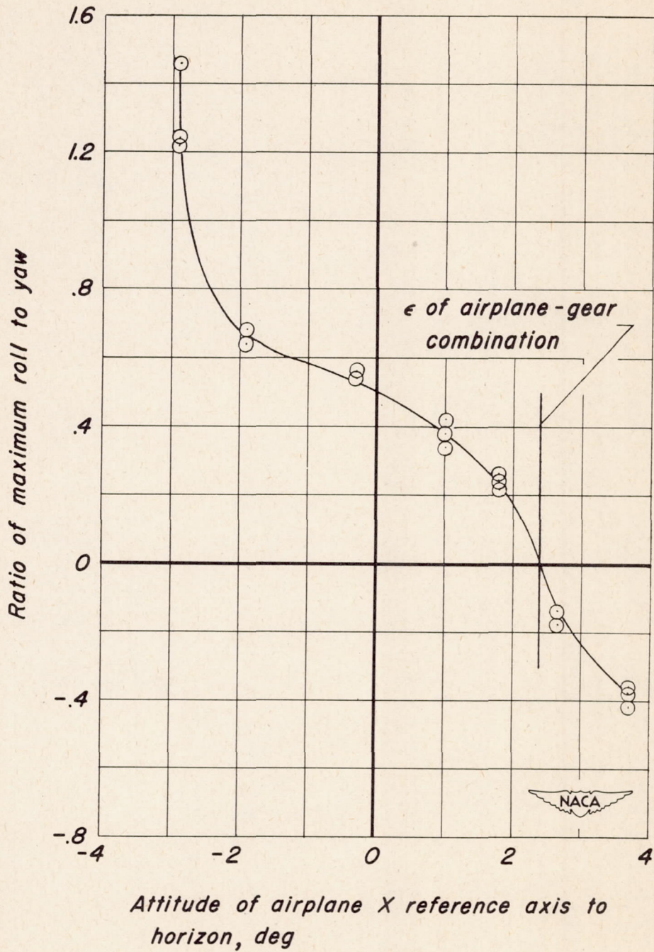
Figure 11.— Ratio of maximum roll to yaw as a function of airplane attitude as measured with the torsional pendulum. Load condition 1.
