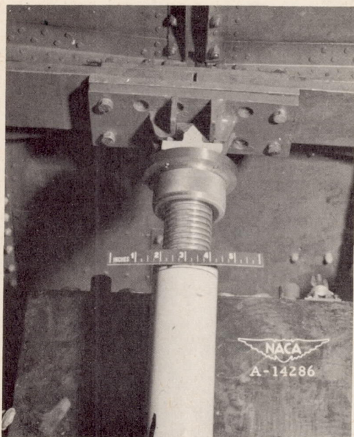
(a) Rear fitting, \theta=7.60^\circ .
