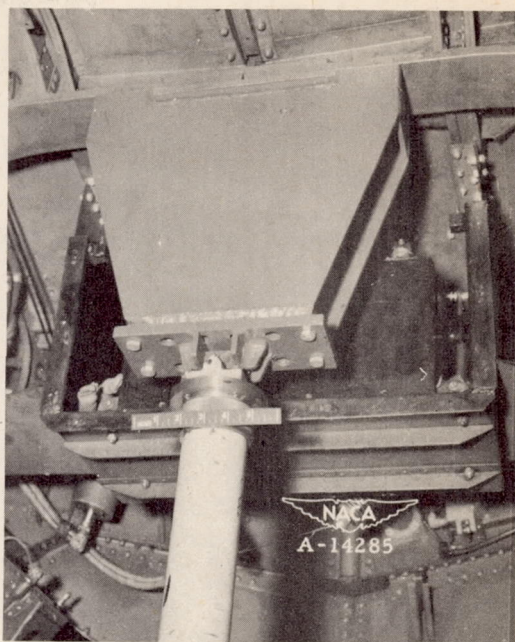
(b) Rear fitting, \theta=0^\circ .
