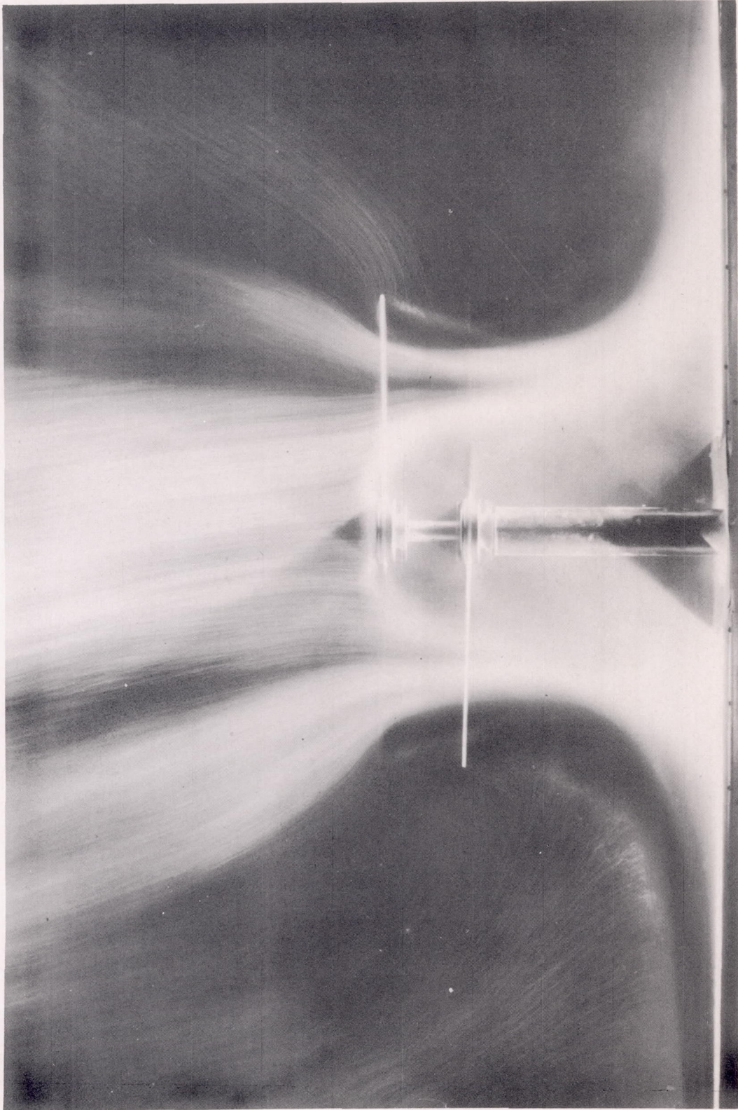
(b) Ground plane at 0.50 diameter.
