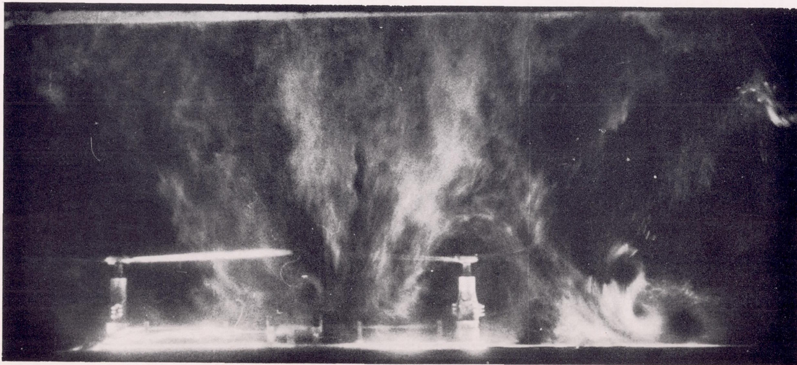
(b) Ground plane at 0.25 diameter.
