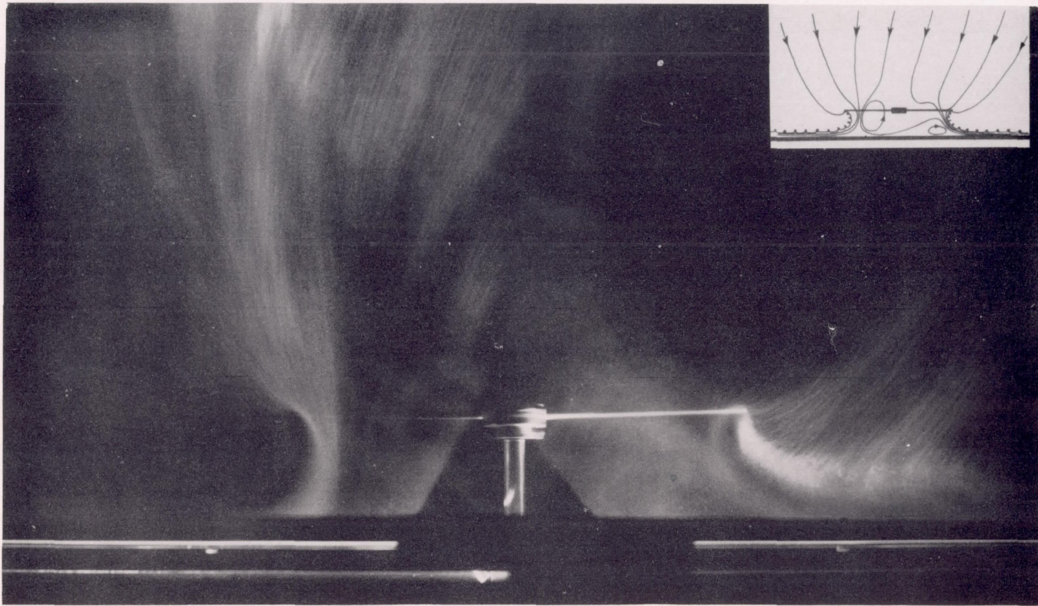
(c) Ground plane at 0.25 diameter.
