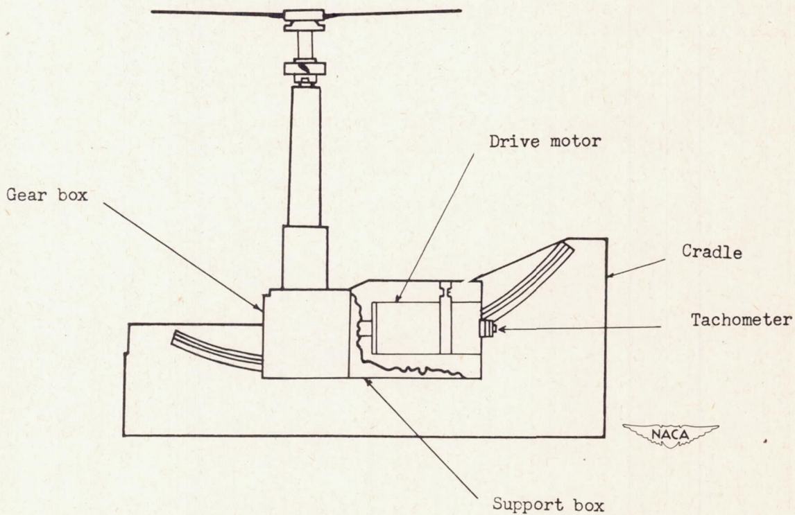
Figure 1.- Schematic diagram of the coaxial rotor model.
