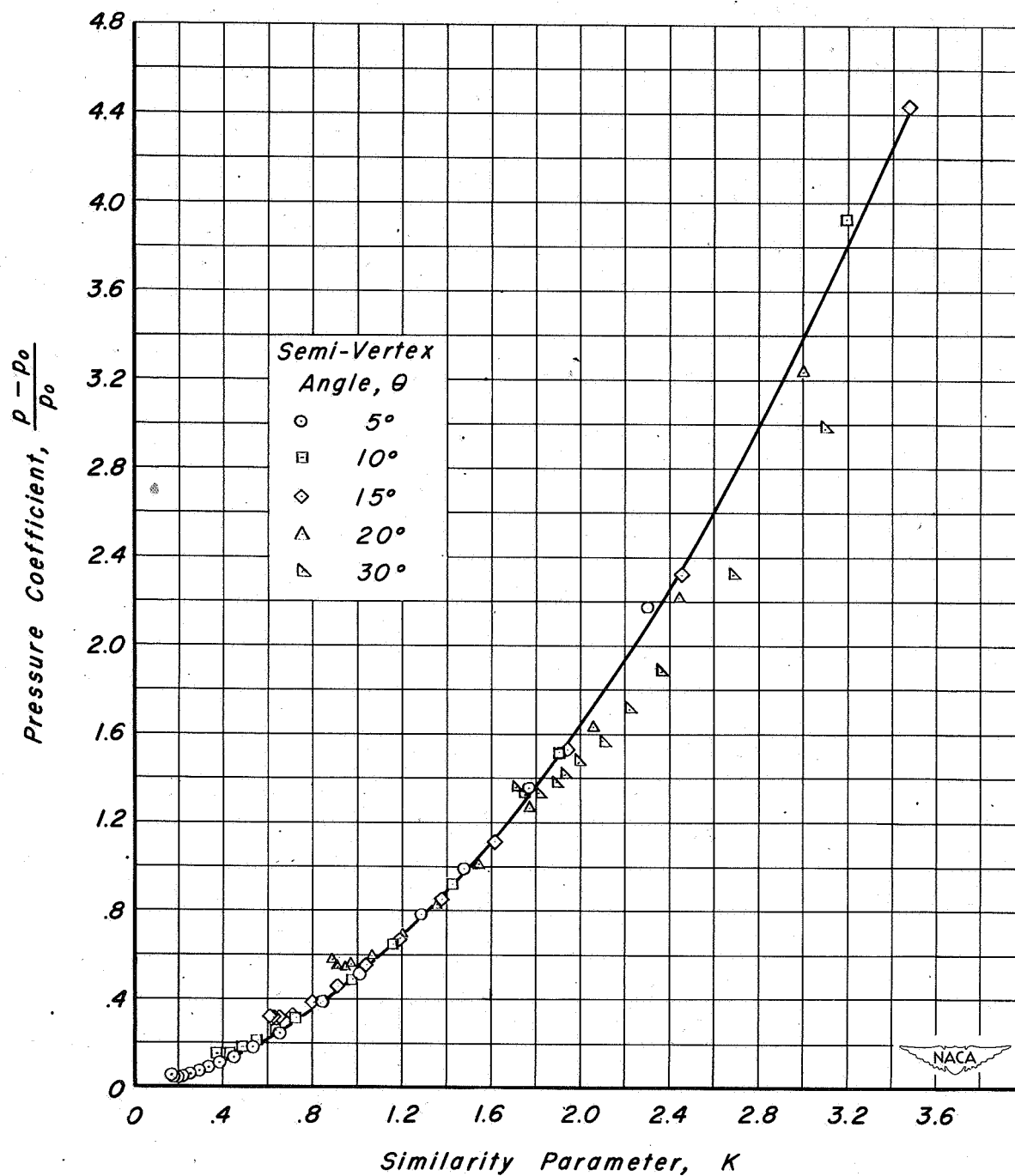
Figure 3.—Variation of pressure coefficient at vertex of body with similarity parameter.
