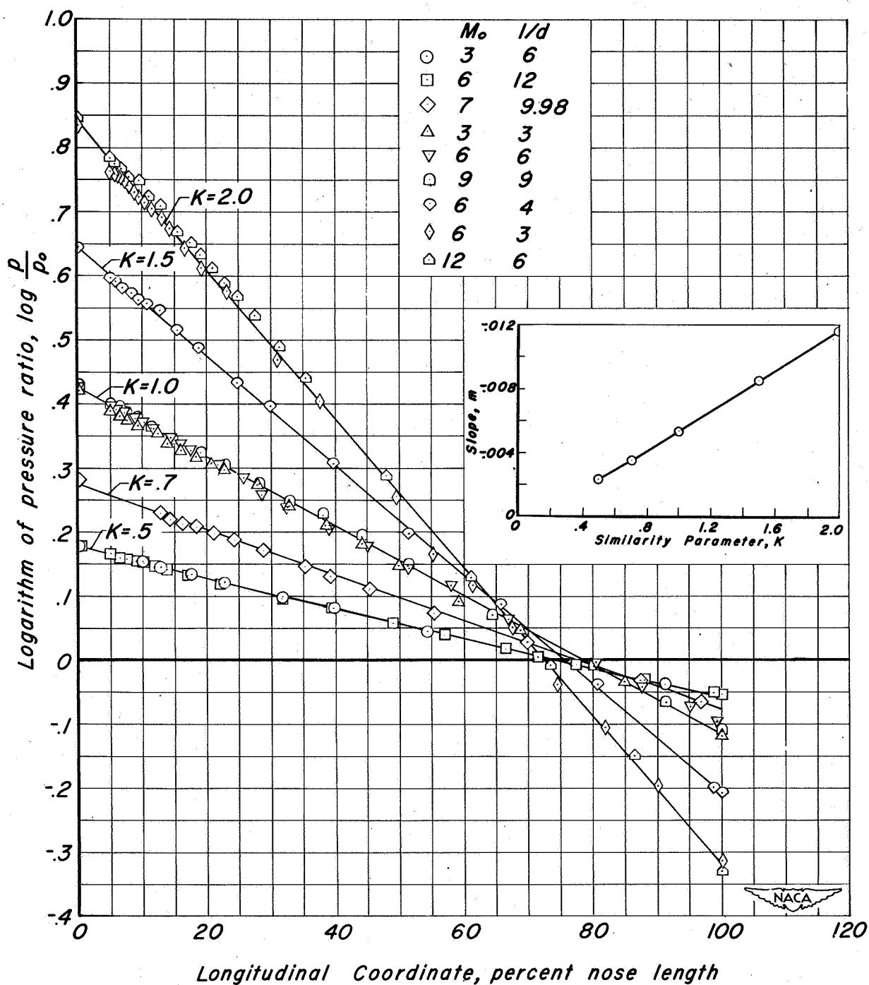
Figure 10.-Variation of the logarithm of the pressure ratio along ogives for various values of the similarity parameter.
