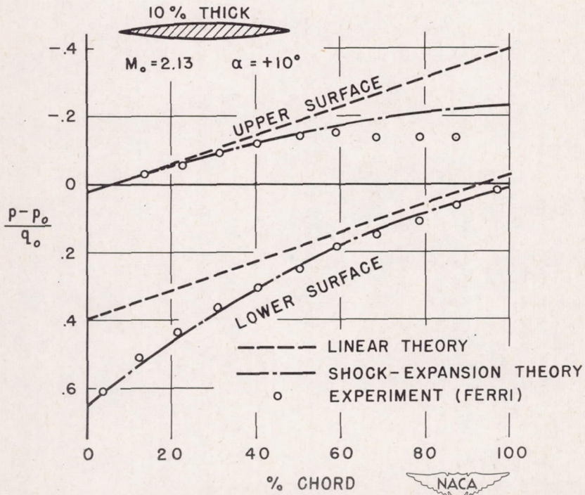
FIGURE 2. - PRESSURE DISTRIBUTION FOR SYMMETRICAL BICONVEX SECTION.
