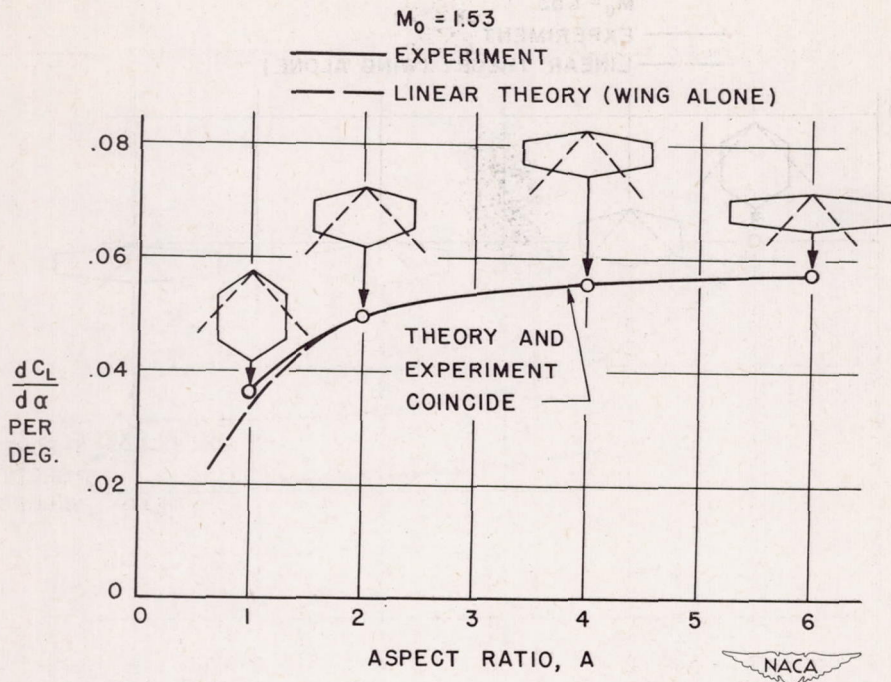
FIGURE 4.— EFFECT OF ASPECT RATIO ON LIFT-CURVE SLOPE.
