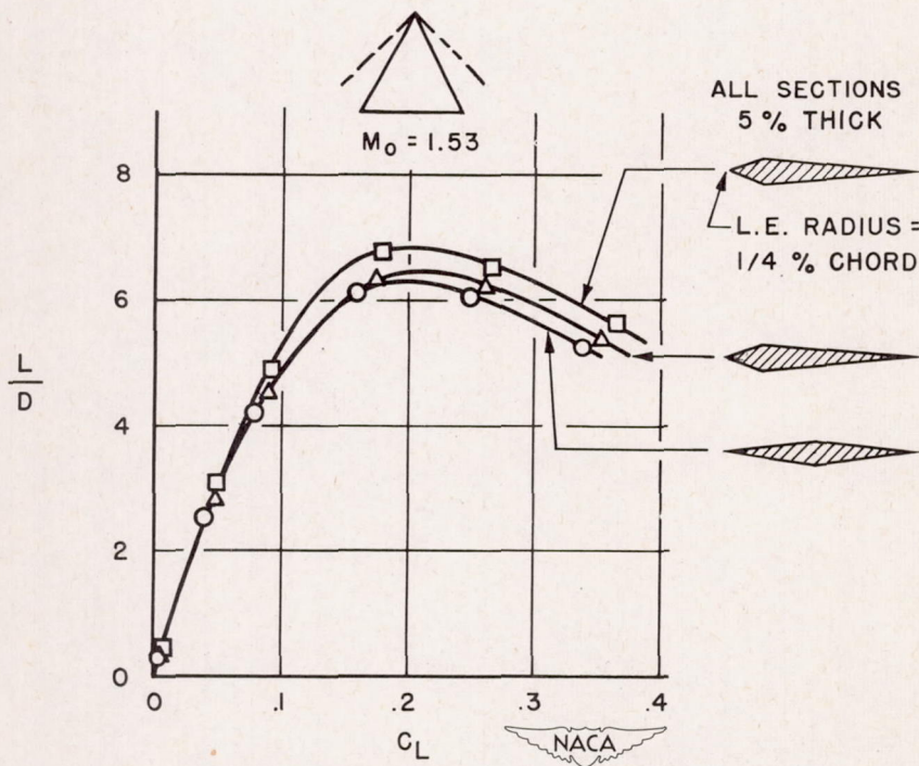
FIGURE 12.- EFFECT OF WING SECTION ON LIFT-DRAG RATIO OF TRIANGULAR WINGS.
