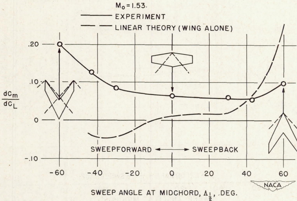
FIGURE 7.— EFFECT OF SWEEP ON MOMENT-CURVE SLOPE.
