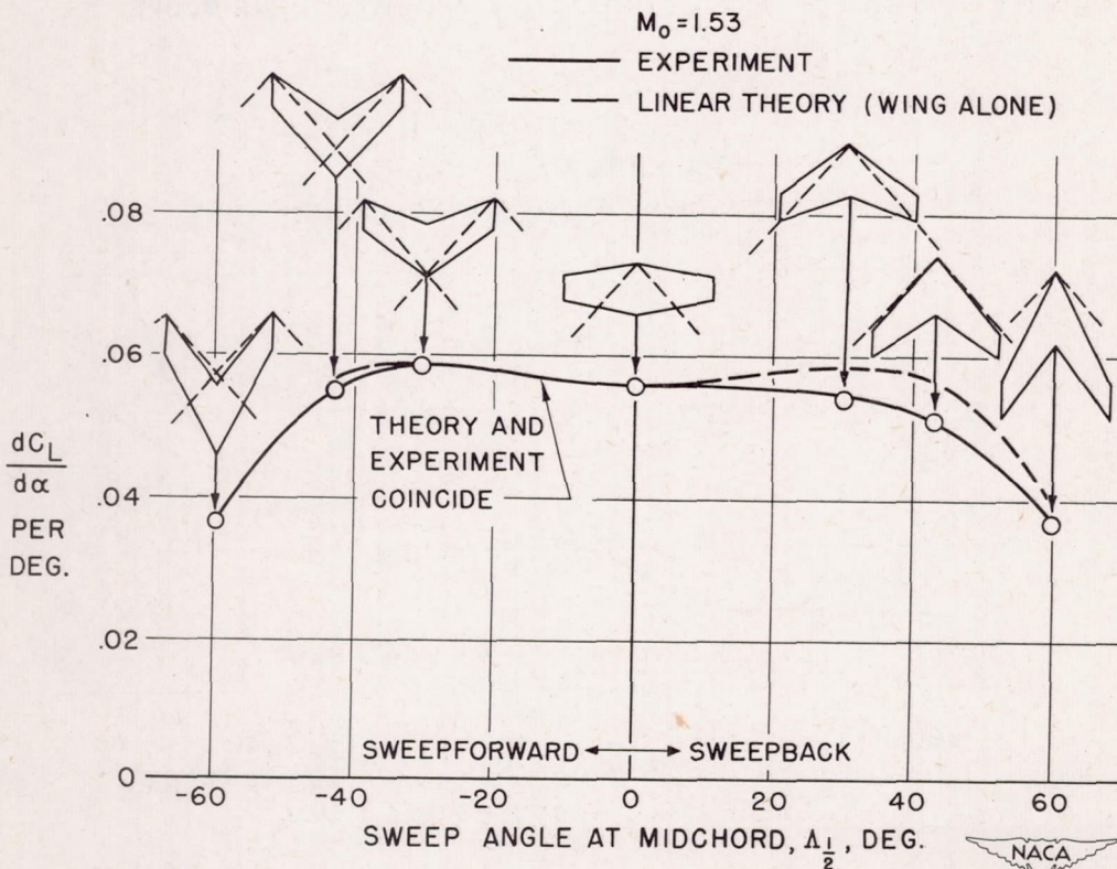
FIGURE 5.— EFFECT OF SWEEP ON LIFT-CURVE SLOPE.
