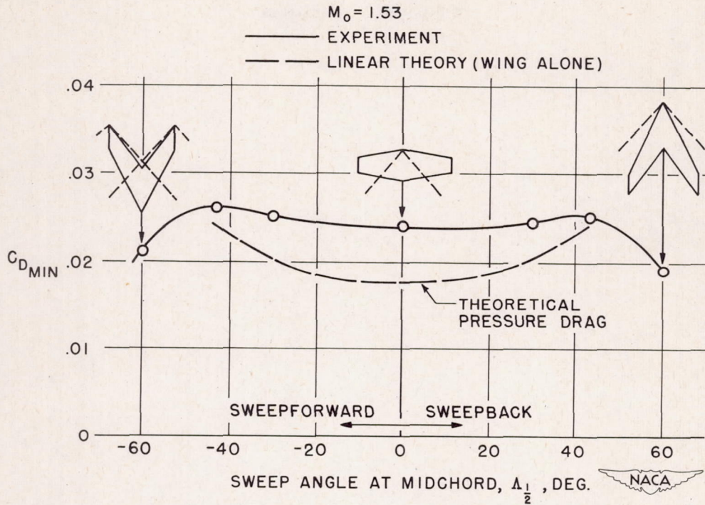
FIGURE 8.- EFFECT OF SWEEP ON MINIMUM DRAG.
