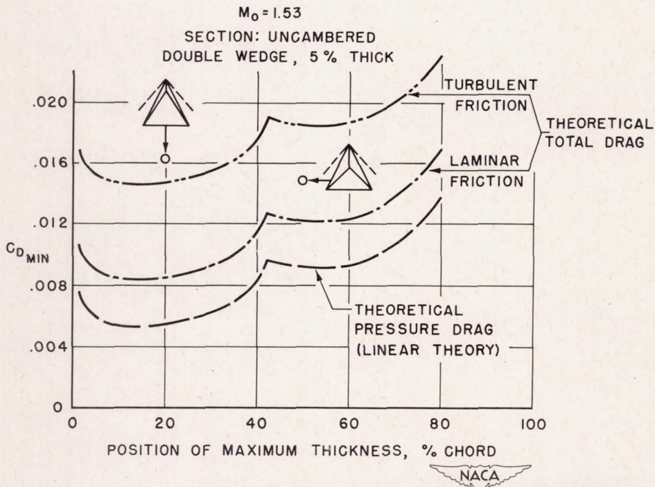
FIGURE 9.- EFFECT OF POSITION OF MAXIMUM THICKNESS ON MINIMUM DRAG OF TRIANGULAR WINGS.
