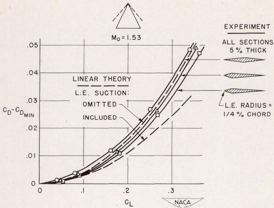
FIGURE 11.- EFFECT OF WING SECTION ON DRAG RISE OF TRIANGULAR WINGS.
