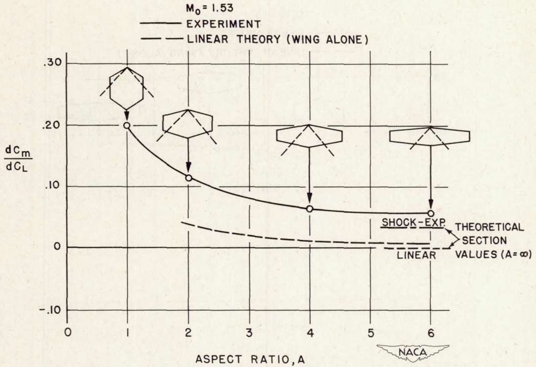
FIGURE 6.— EFFECT OF ASPECT RATIO ON MOMENT-CURVE SLOPE.
