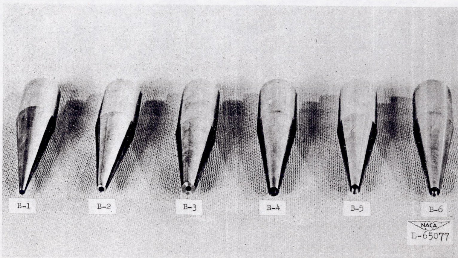
Figure 2.- Total-pressure tubes having 15^\circ conical-nose sections. Series B.
