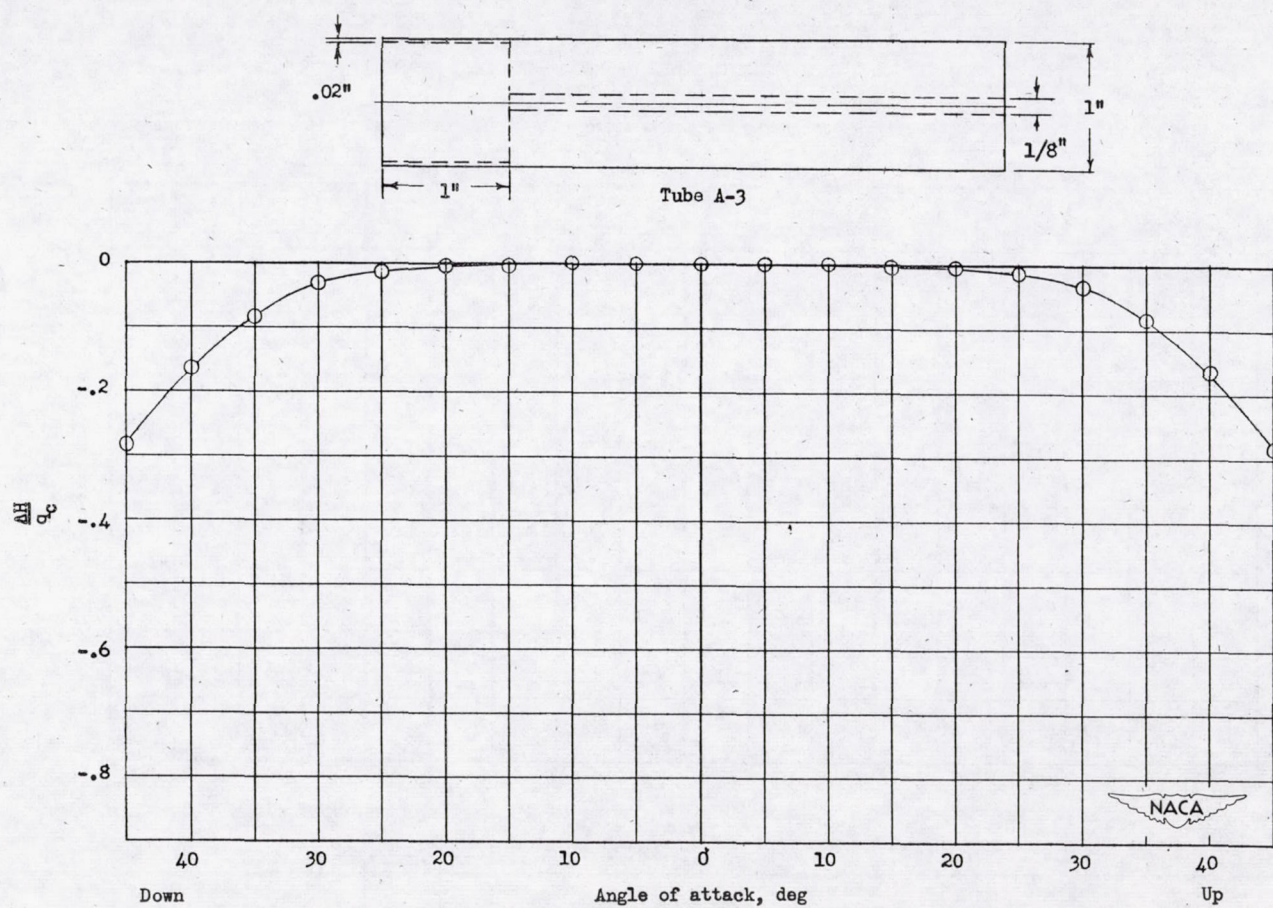
Figure 11.- Variation of total-pressure error with angle of attack. Tube A-3.
