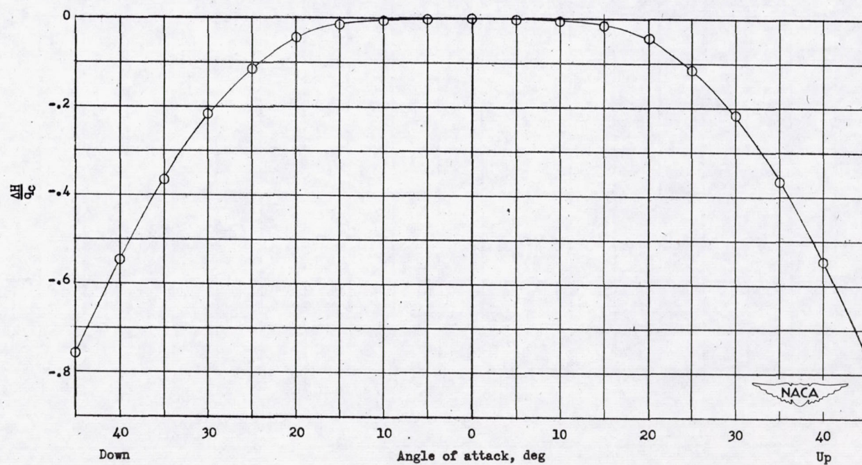
Figure 41.- Variation of total-pressure error with angle of attack. Tube D-6.
