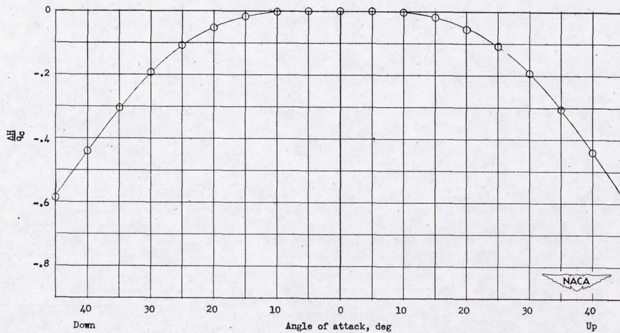
Figure 23.- Variation of total-pressure error with angle of attack. Tube B-2.
