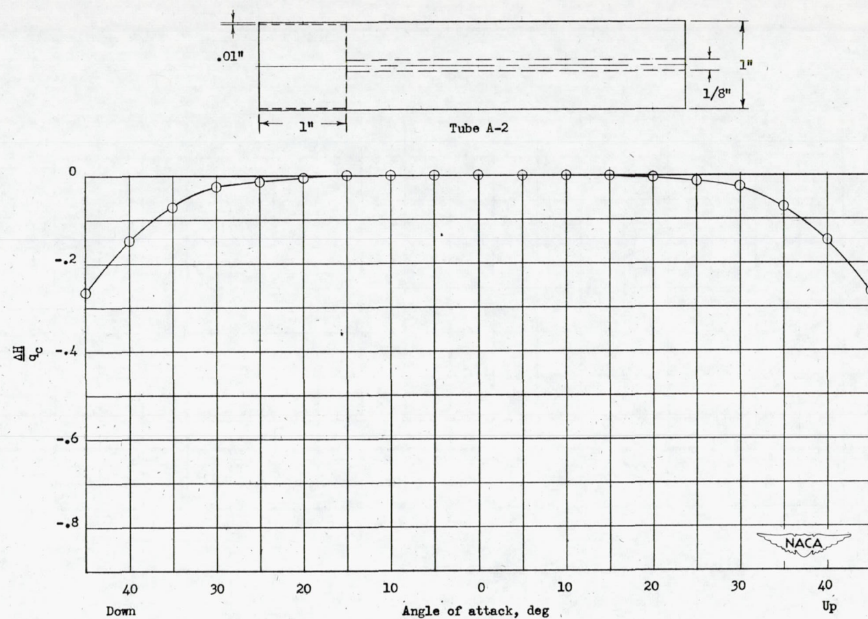
Figure 10.- Variation of total-pressure error with angle of attack. Tube A-2.
