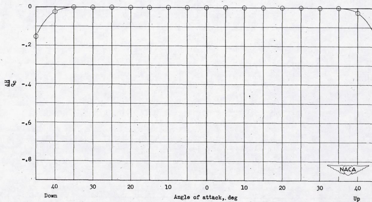
Figure 19.- Variation of total-pressure error with angle of attack. Tube A-11.
