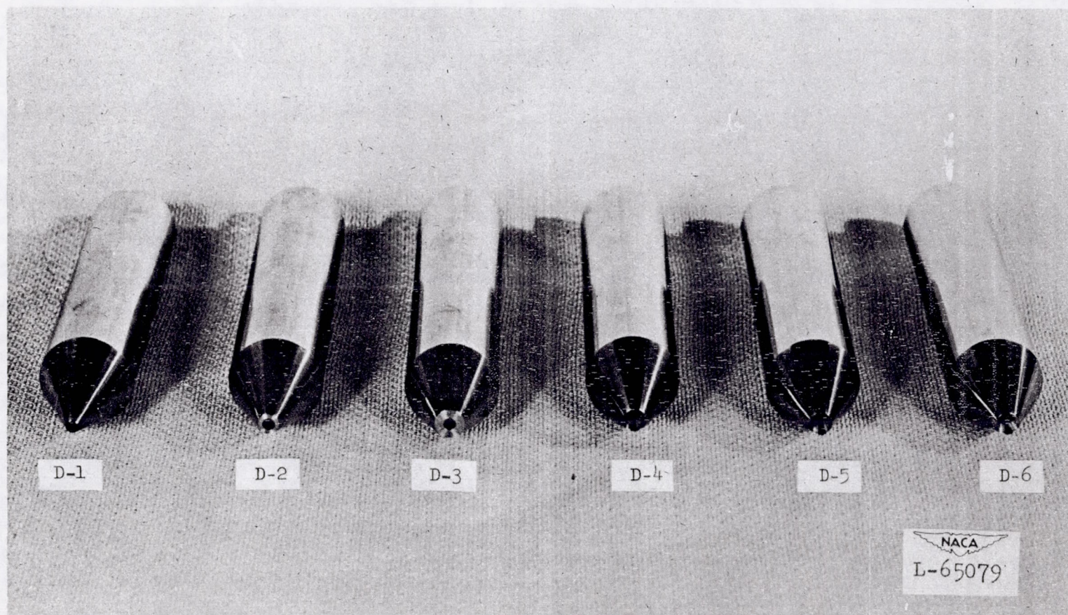
Figure 4.- Total-pressure tubes having 45^{\circ} conical-nose sections. Series D.
