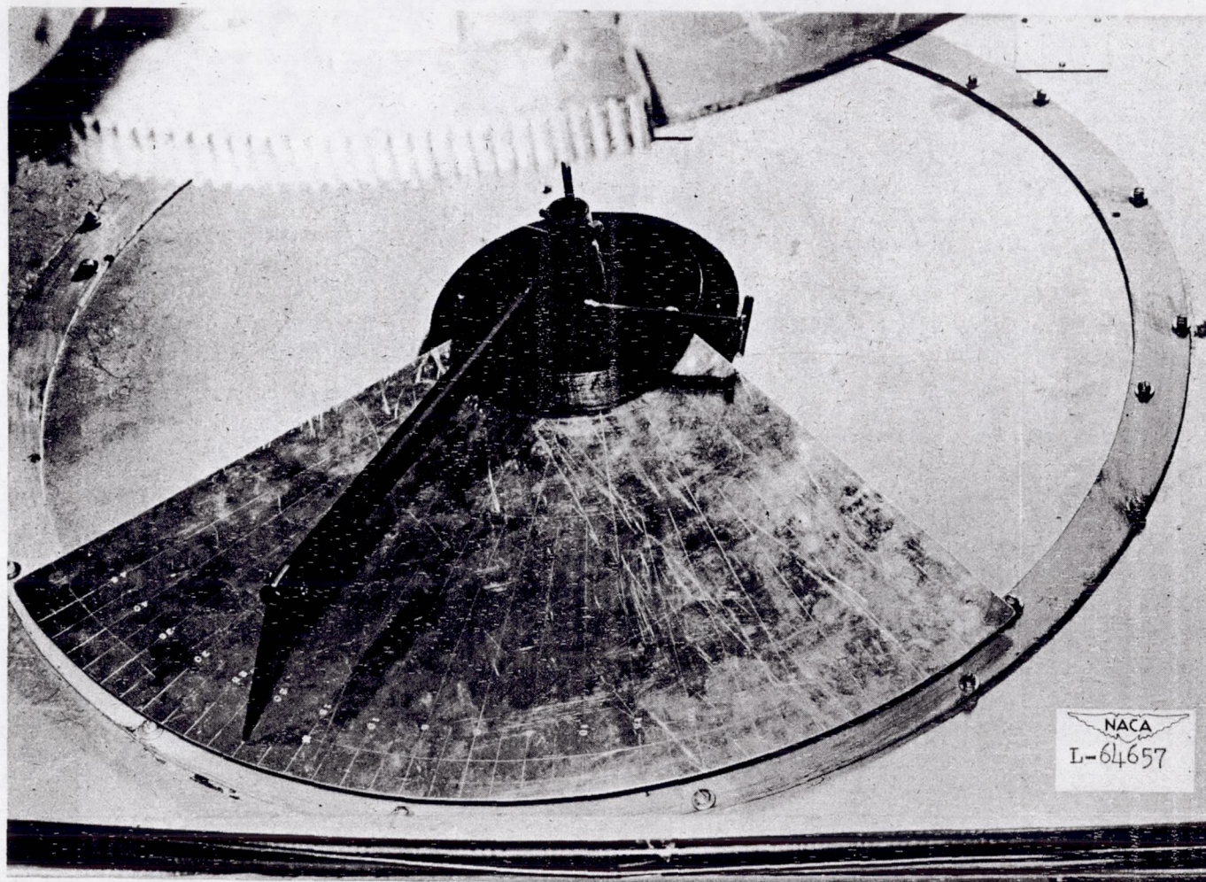
Figure 8.- View outside of tunnel wall showing control arm, pointer, and angle-of-attack scale.
