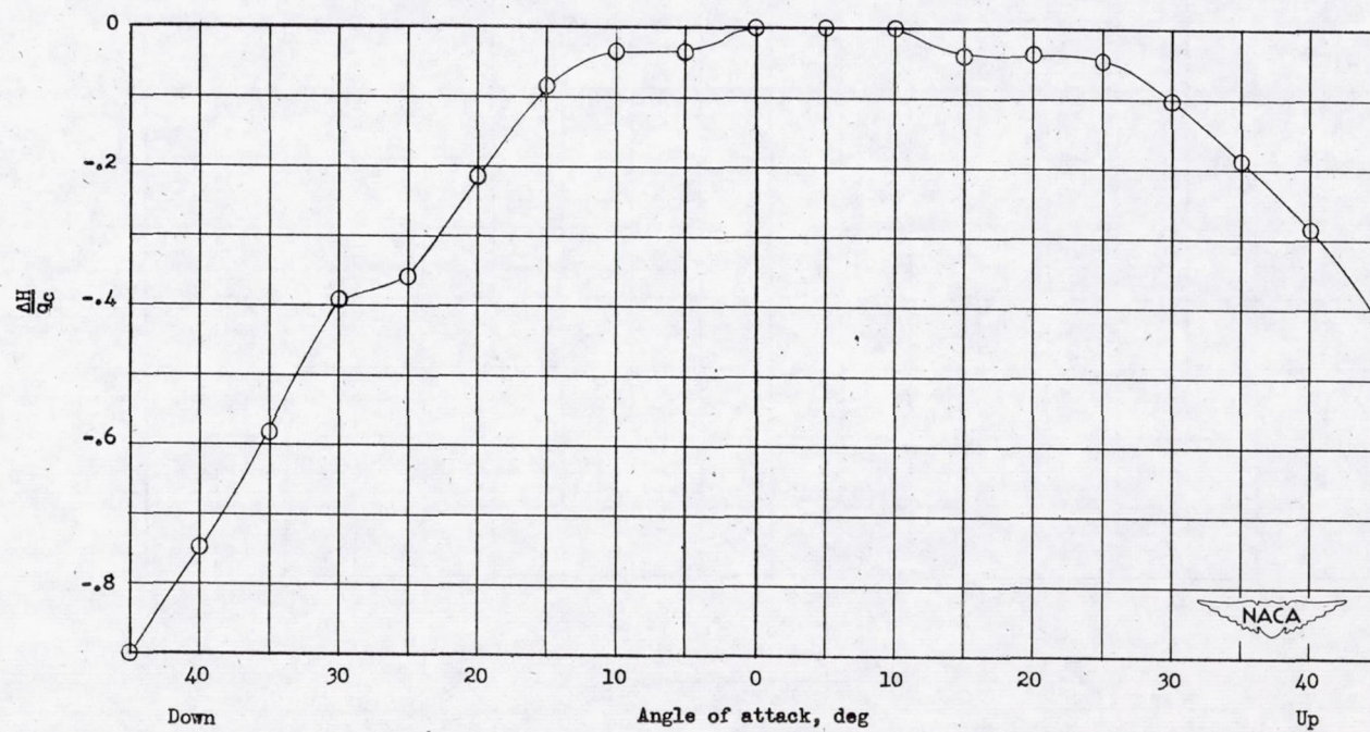
Figure 43.- Variation of total-pressure error with angle of attack. Tube E-2.
