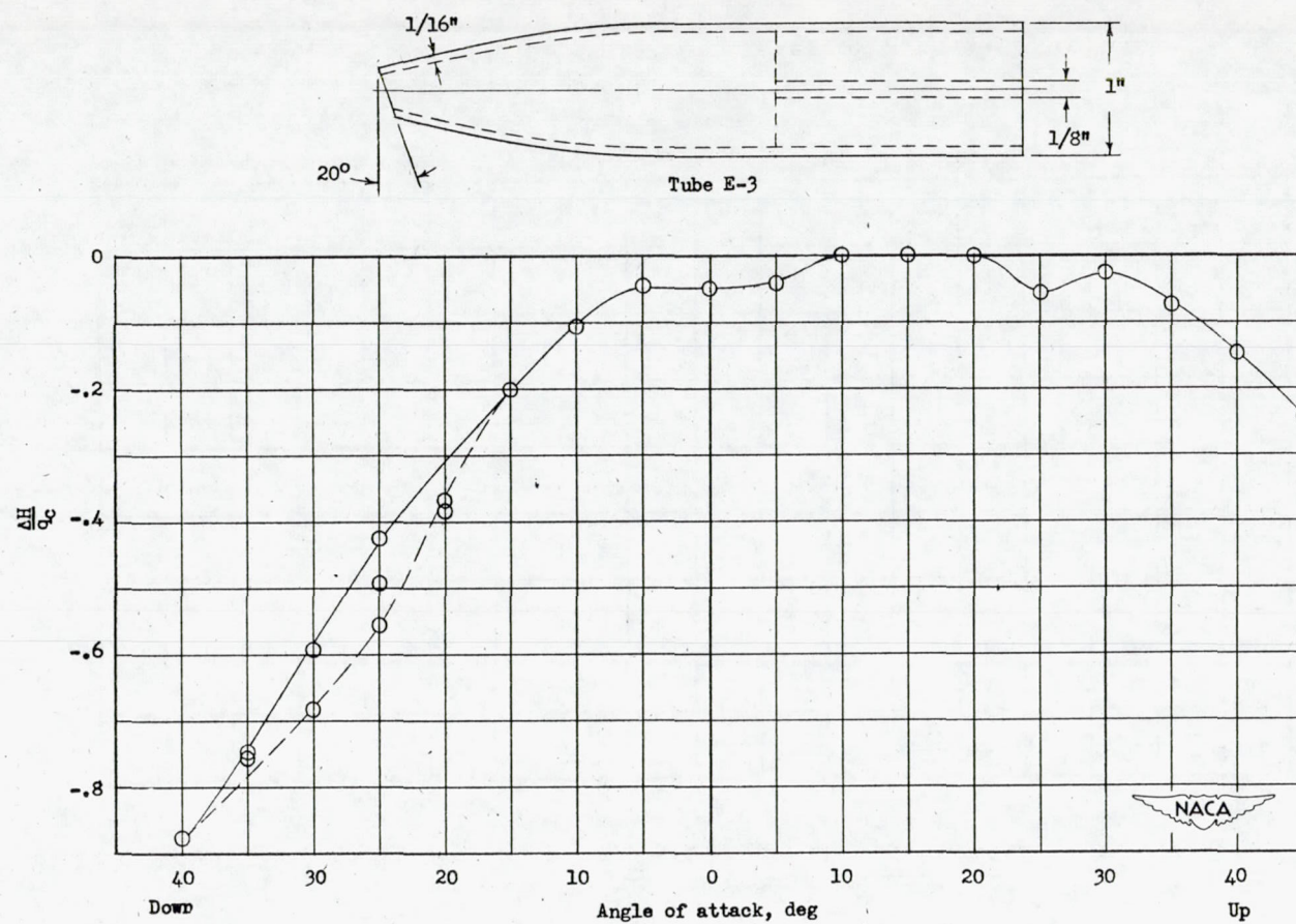
Figure 44.- Variation of total-pressure error with angle of attack. Tube E-3.
