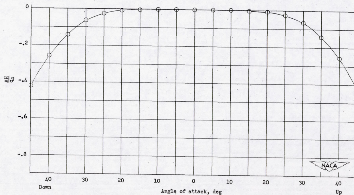
Figure 25.- Variation of total-pressure error with angle of attack. Tube B-4.
