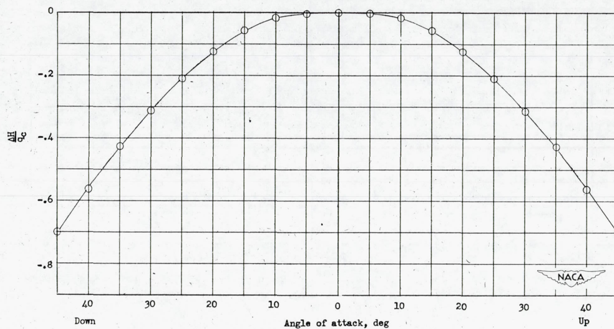
Figure 38.- Variation of total-pressure error with angle of attack. Tube D-3.
