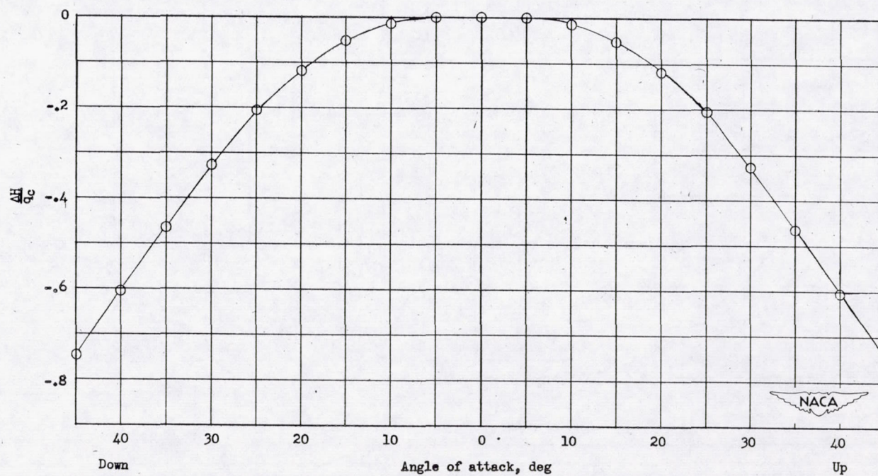
Figure 37.- Variation of total-pressure error with angle of attack. Tube D-2.
