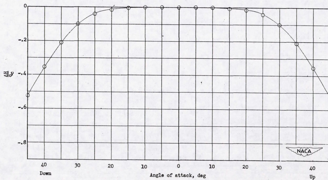
Figure 45.- Variation of total-pressure error with angle of attack. Tube E-4.
