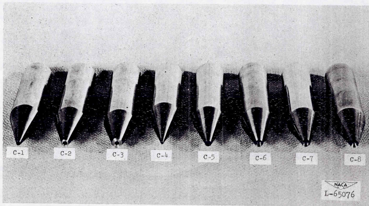
Figure 3.- Total-pressure tubes having 30^\circ conical-nose sections. Series C.
