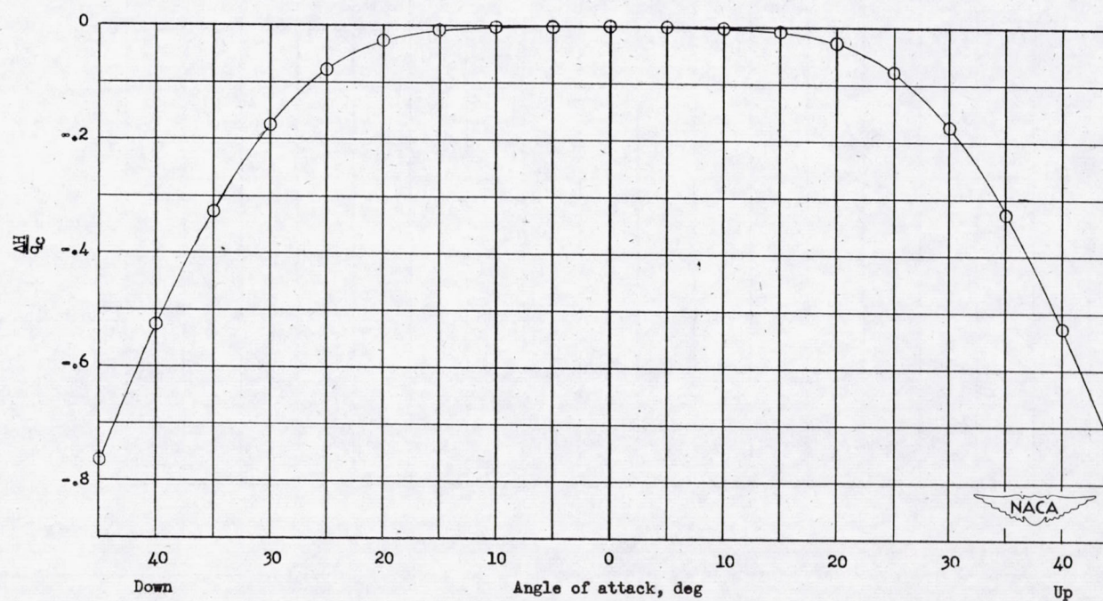
Figure 31.- Variation of total-pressure error with angle of attack. Tube C-4.
