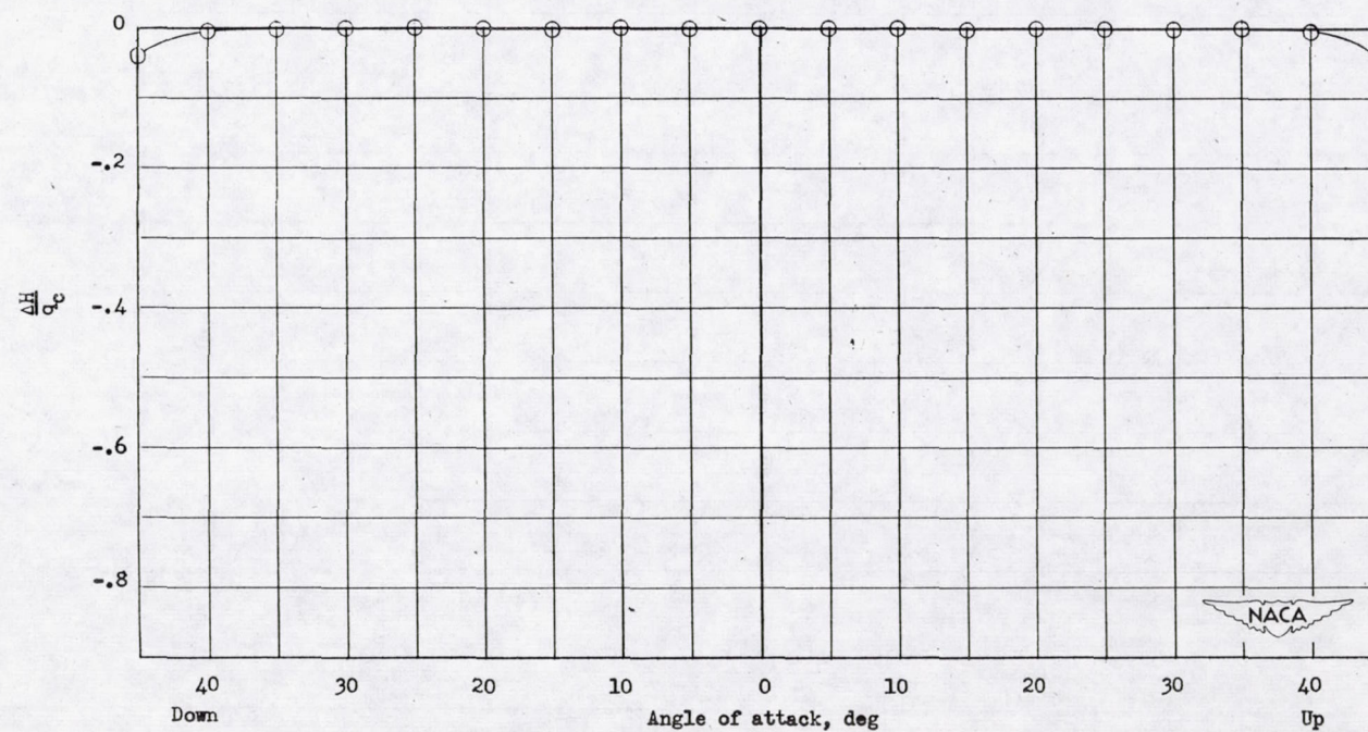
Figure 21.- Variation of total-pressure error with angle of attack. Tube A-13.
