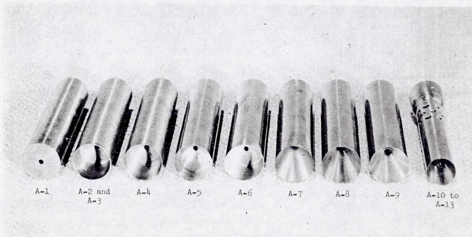
Figure 1.- Total-pressure tubes having straight external walls. Series A.
