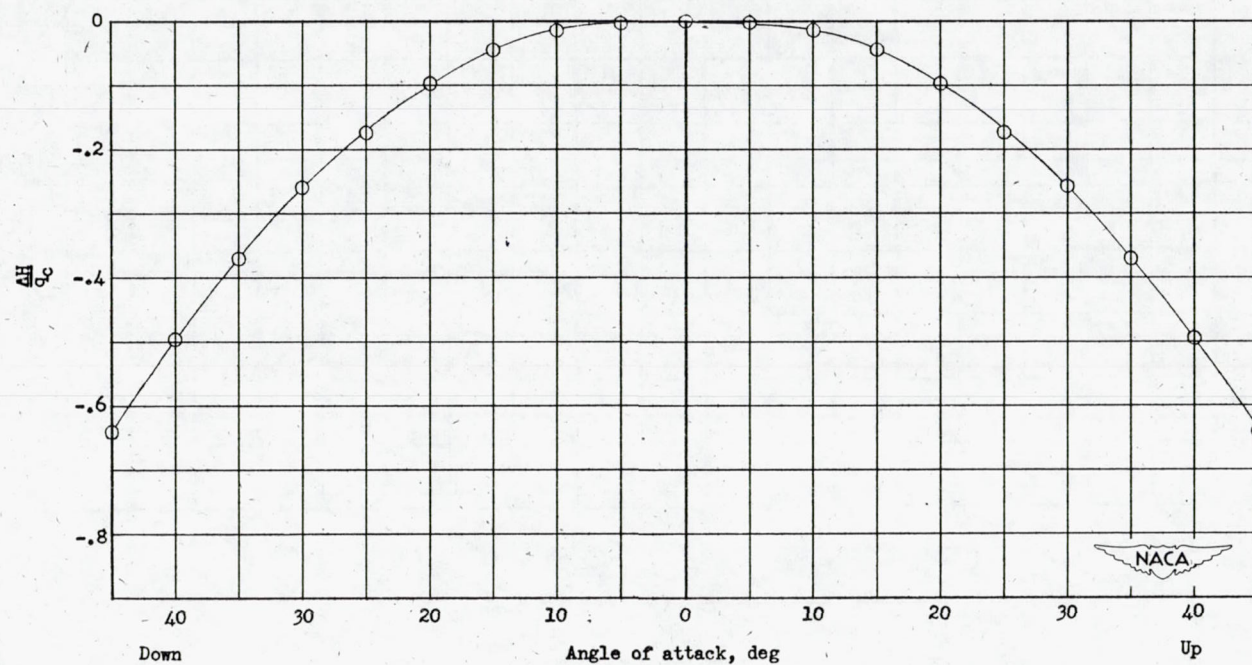
Figure 30.- Variation of total-pressure error with angle of attack. Tube C-3.
