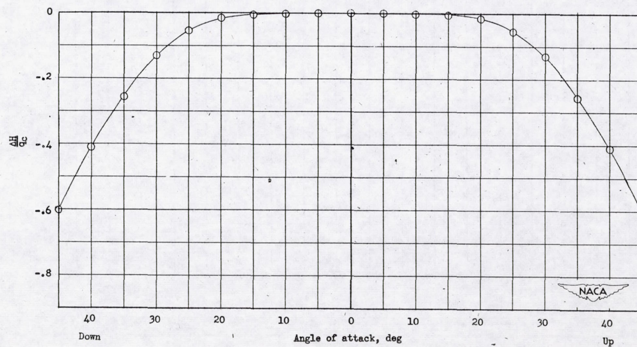
Figure 27.- Variation of total-pressure error with angle of attack. Tube B-6.
