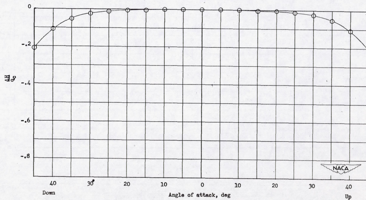
Figure 17.- Variation of total-pressure error with angle of attack. Tube A-9.
