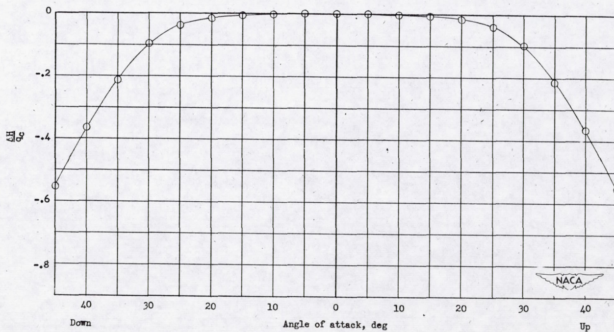
Figure 47.- Variation of total-pressure error with angle of attack. Tube E-6.
