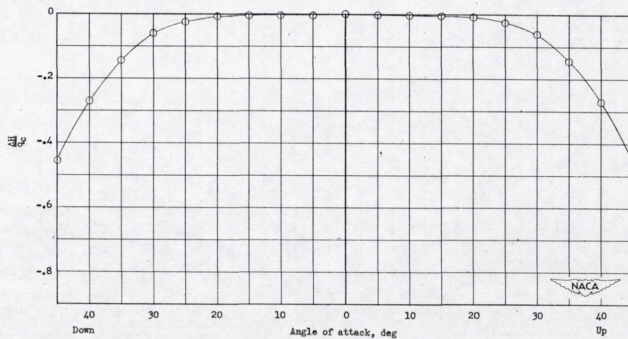
Figure 33.- Variation of total-pressure error with angle of attack. Tube C-6.
