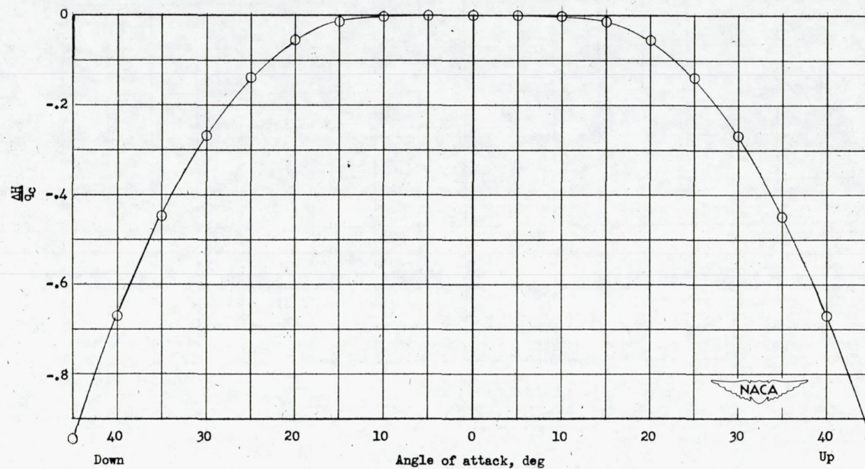
Figure 36.- Variation of total-pressure error with angle of attack. Tube D-1.
