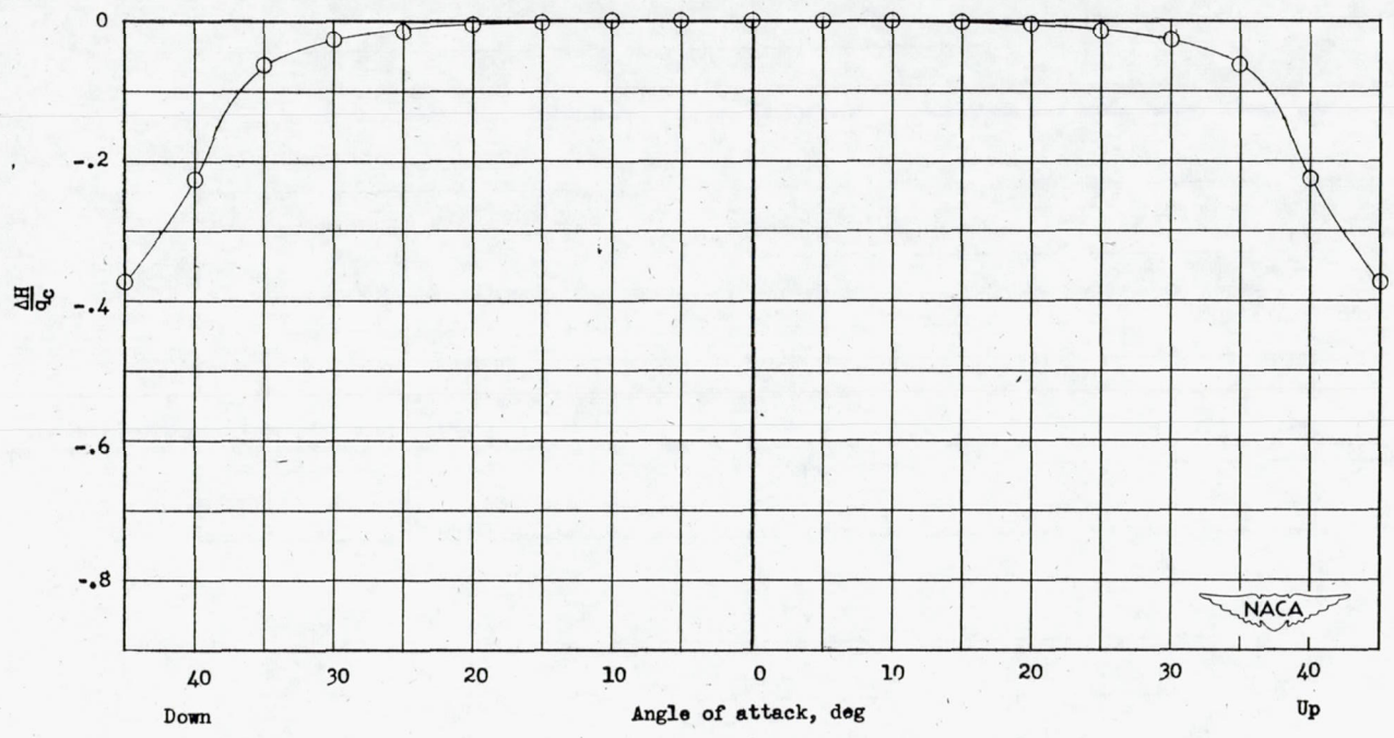
Figure 18.- Variation of total-pressure error with angle of attack. Tube A-10.
