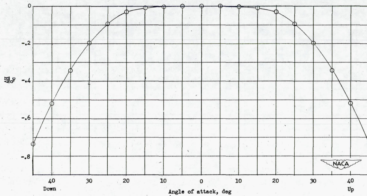
Figure 40.- Variation of total-pressure error with angle of attack. Tube D-5.
