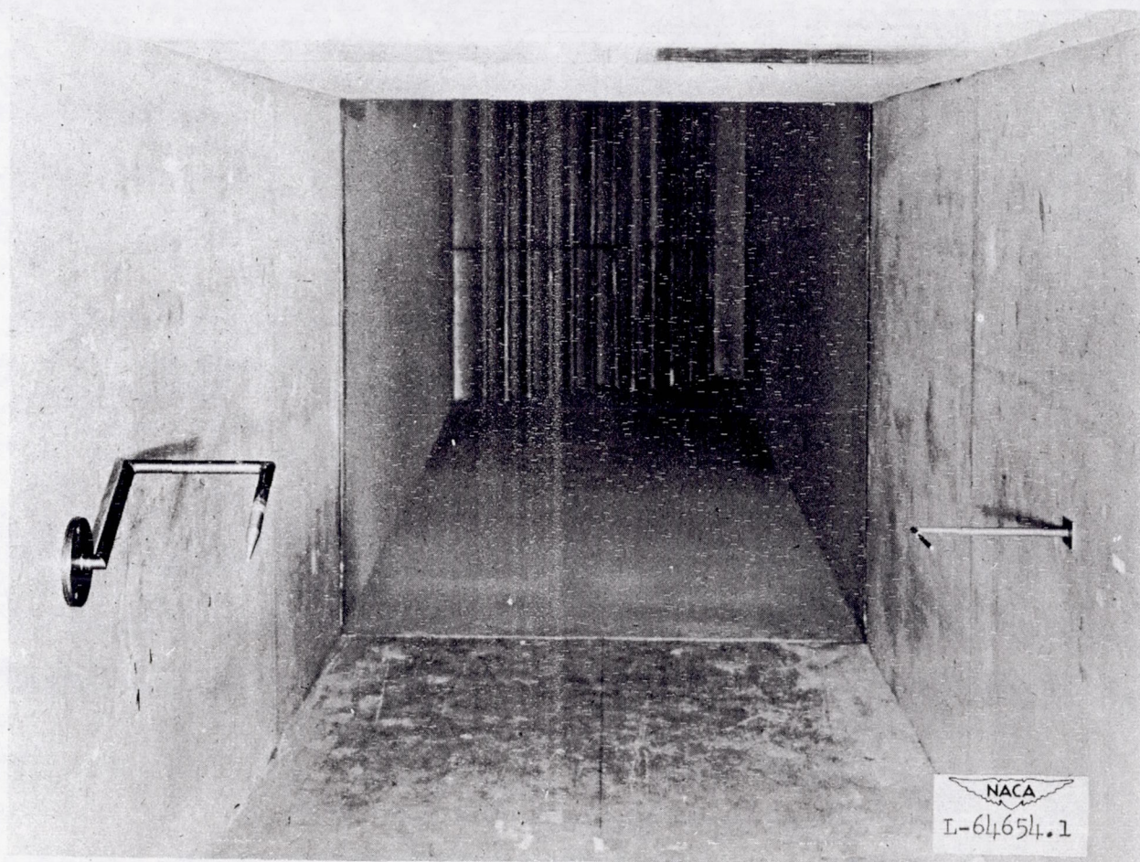
Figure 6.- View of Langley stability tunnel showing swivel arm with sample total-pressure tube on left wall and reference pitot-static tube on right wall.
