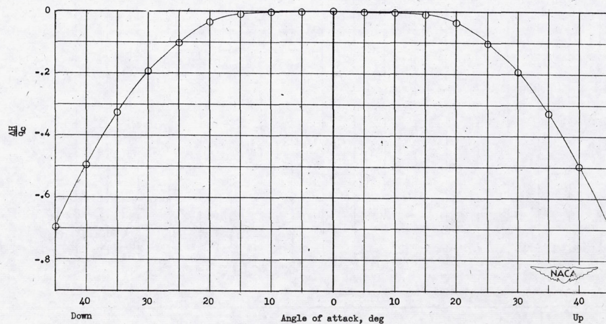
Figure 39.- Variation of total-pressure error with angle of attack. Tube D-4.
