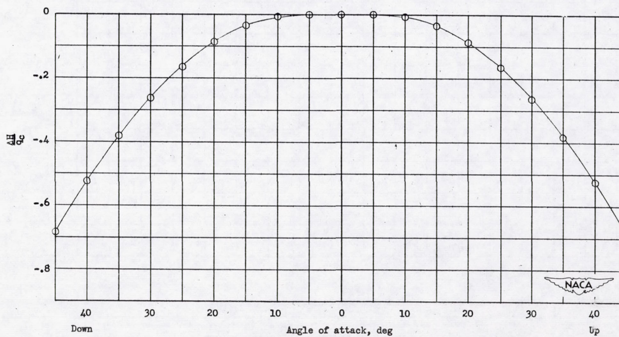
Figure 29.- Variation of total-pressure error with angle of attack. Tube C-2.
