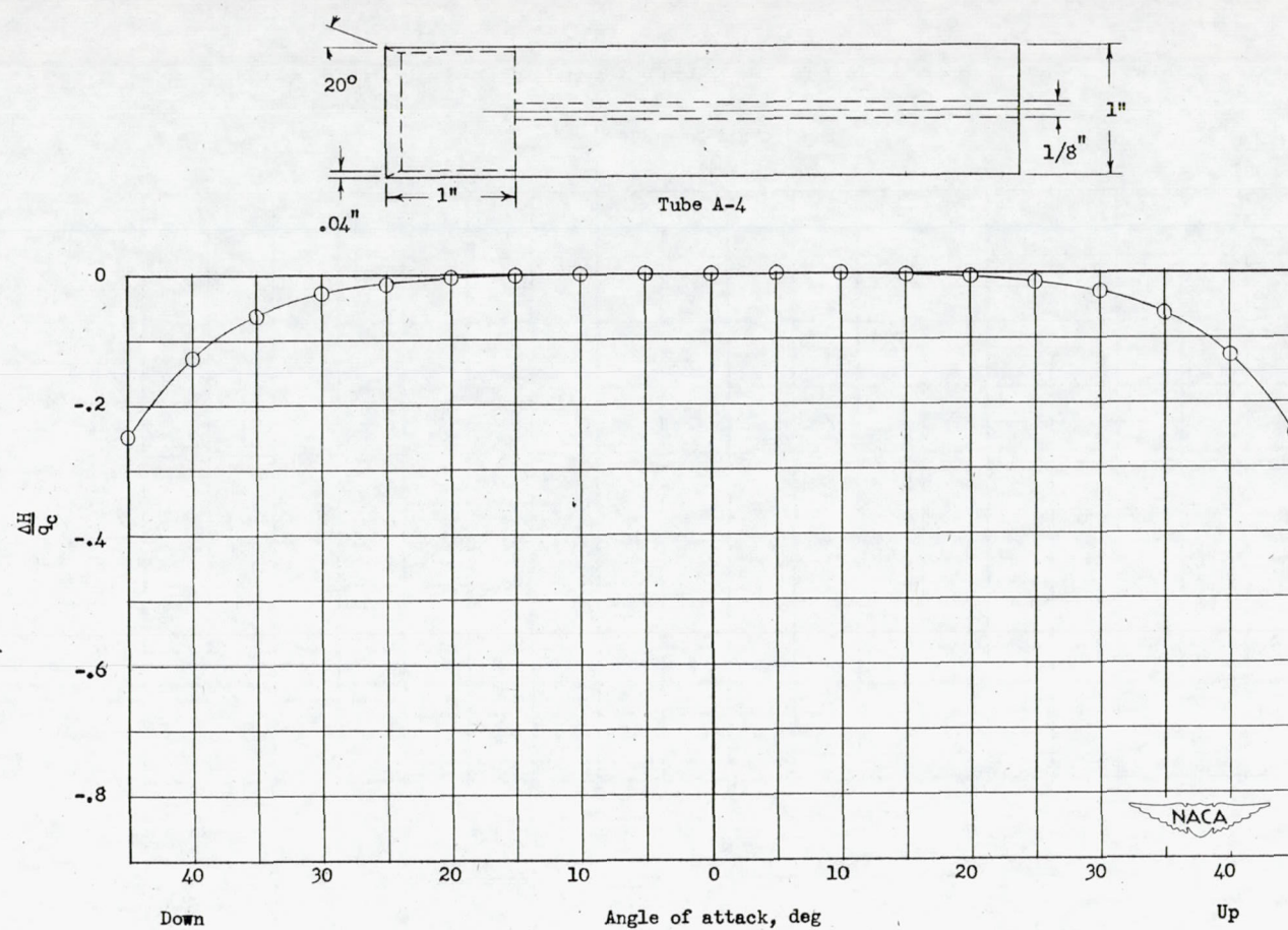
Figure 12.- Variation of total-pressure error with angle of attack. Tube A-4.
