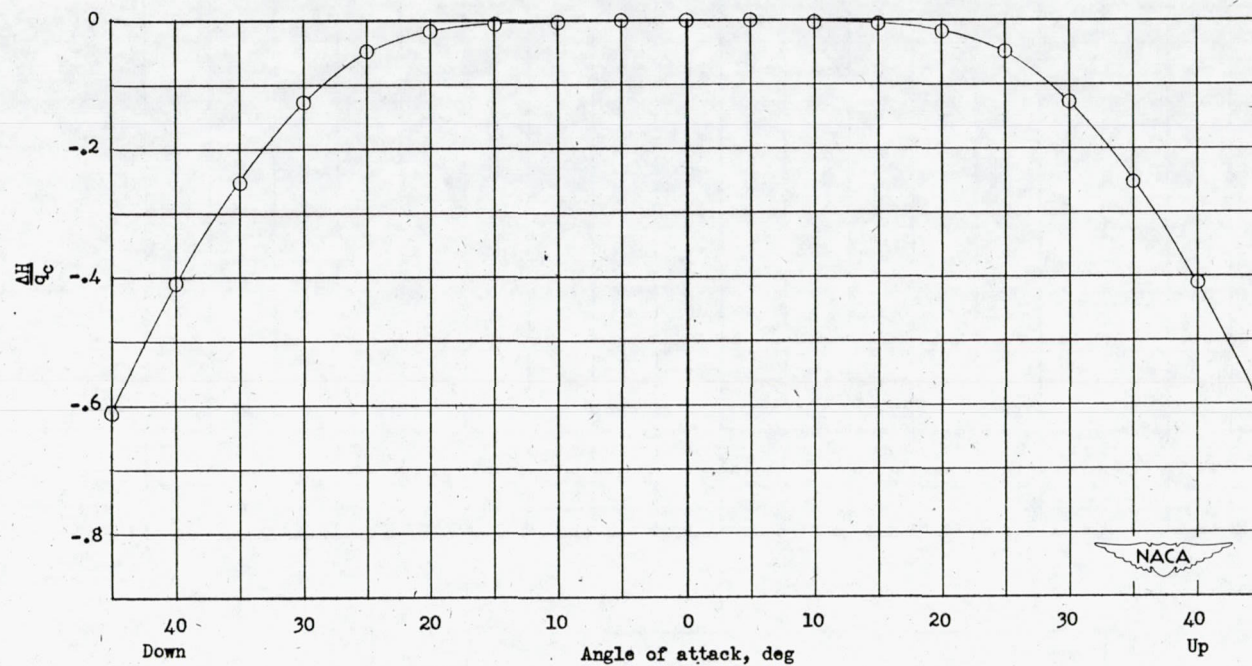
Figure 34.- Variation of total-pressure error with angle of attack. Tube C-7.
