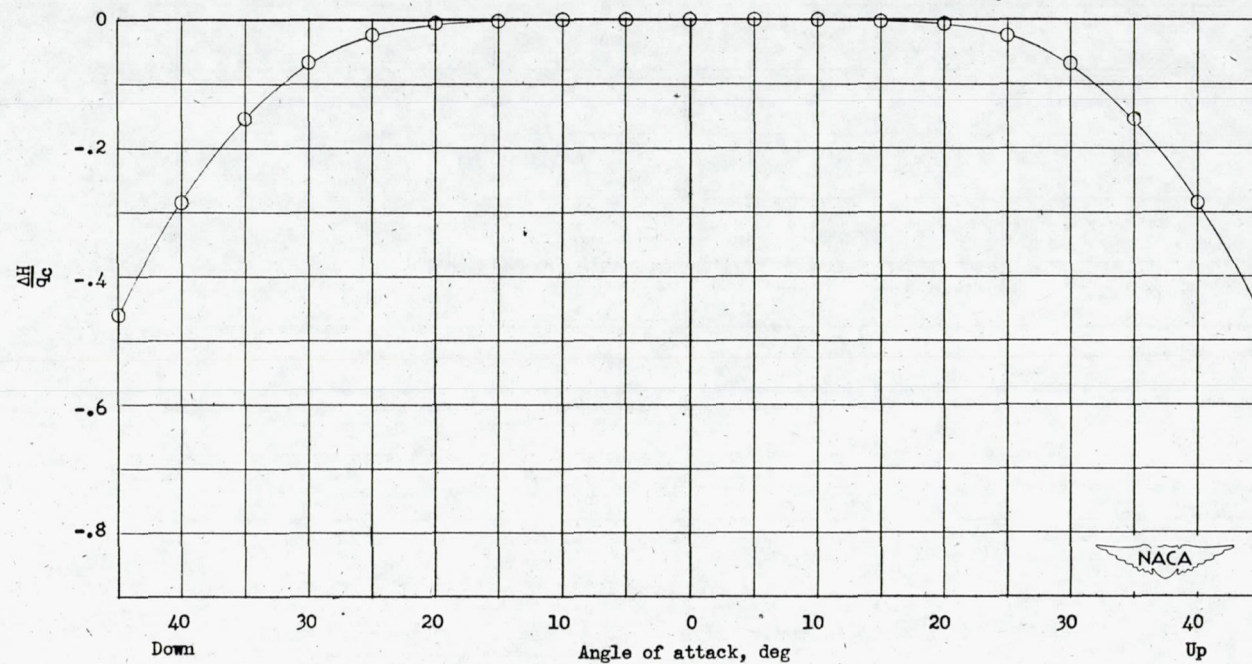
Figure 22.- Variation of total-pressure error with angle of attack. Tube B-1.
