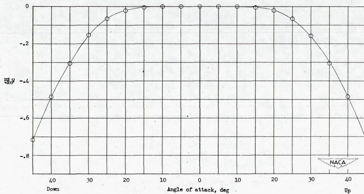
Figure 28.- Variation of total-pressure error with angle of attack. Tube C-1.
