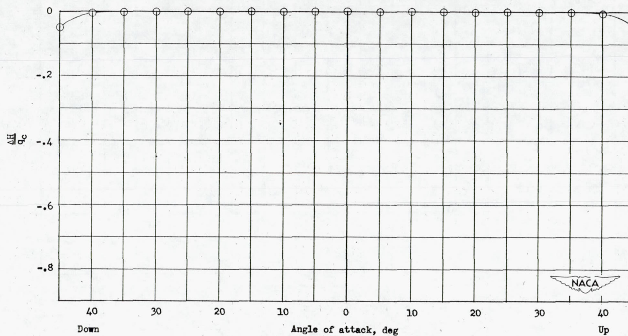
Figure 20.- Variation of total-pressure error with angle of attack. Tube A-12.
