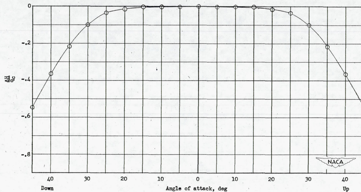
Figure 46.- Variation of total-pressure error with angle of attack. Tube E-5.
