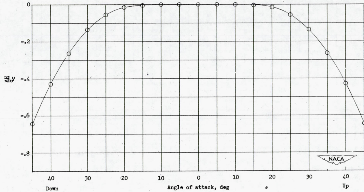
Figure 32.- Variation of total-pressure error with angle of attack. Tube C-5.
