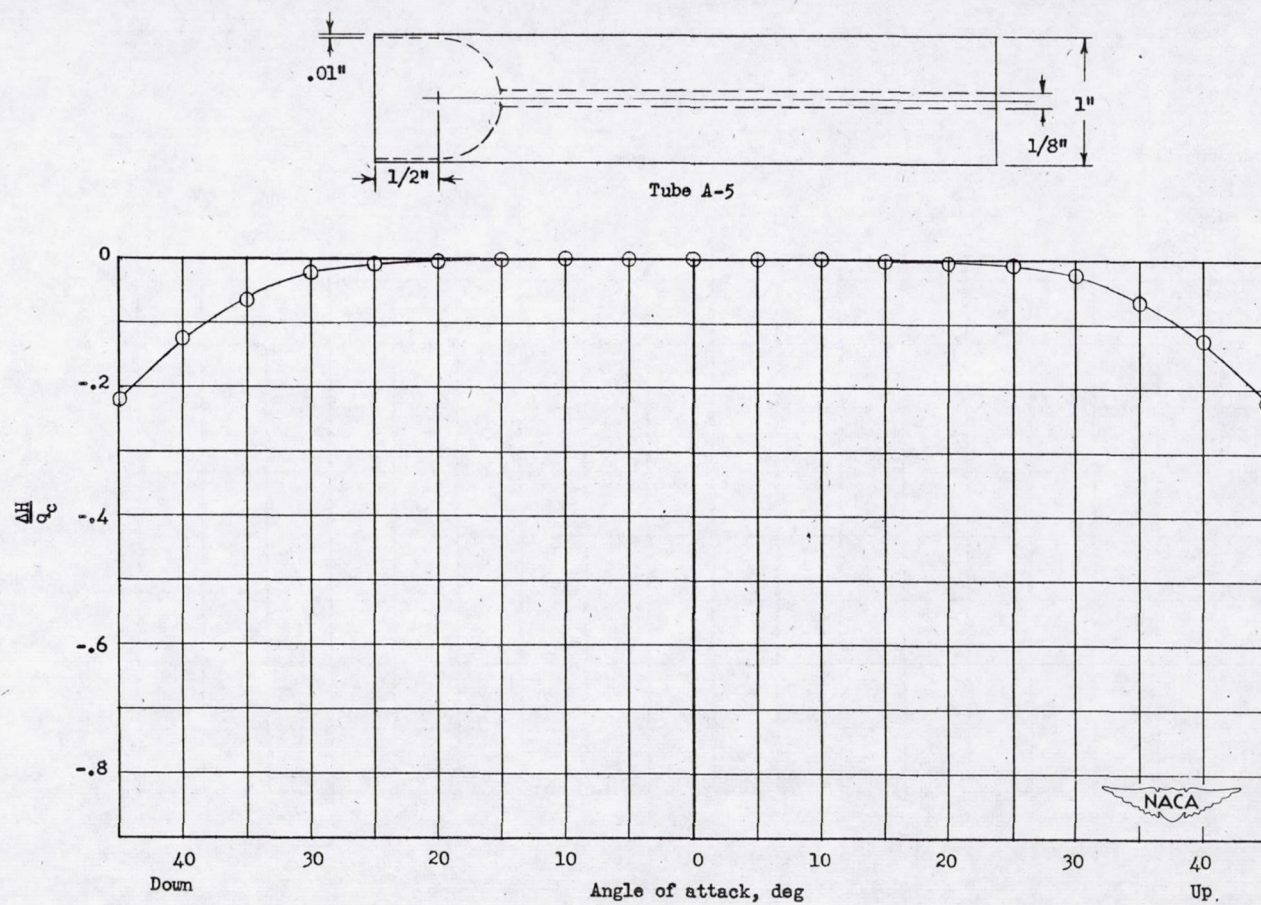
Figure 13.- Variation of total-pressure error with angle of attack. Tube A-5.
