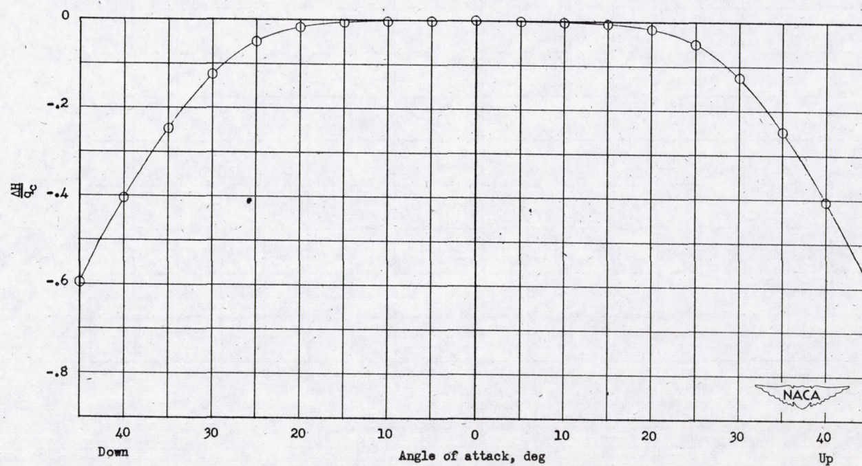
Figure 35.- Variation of total-pressure error with angle of attack. Tube C-8.
