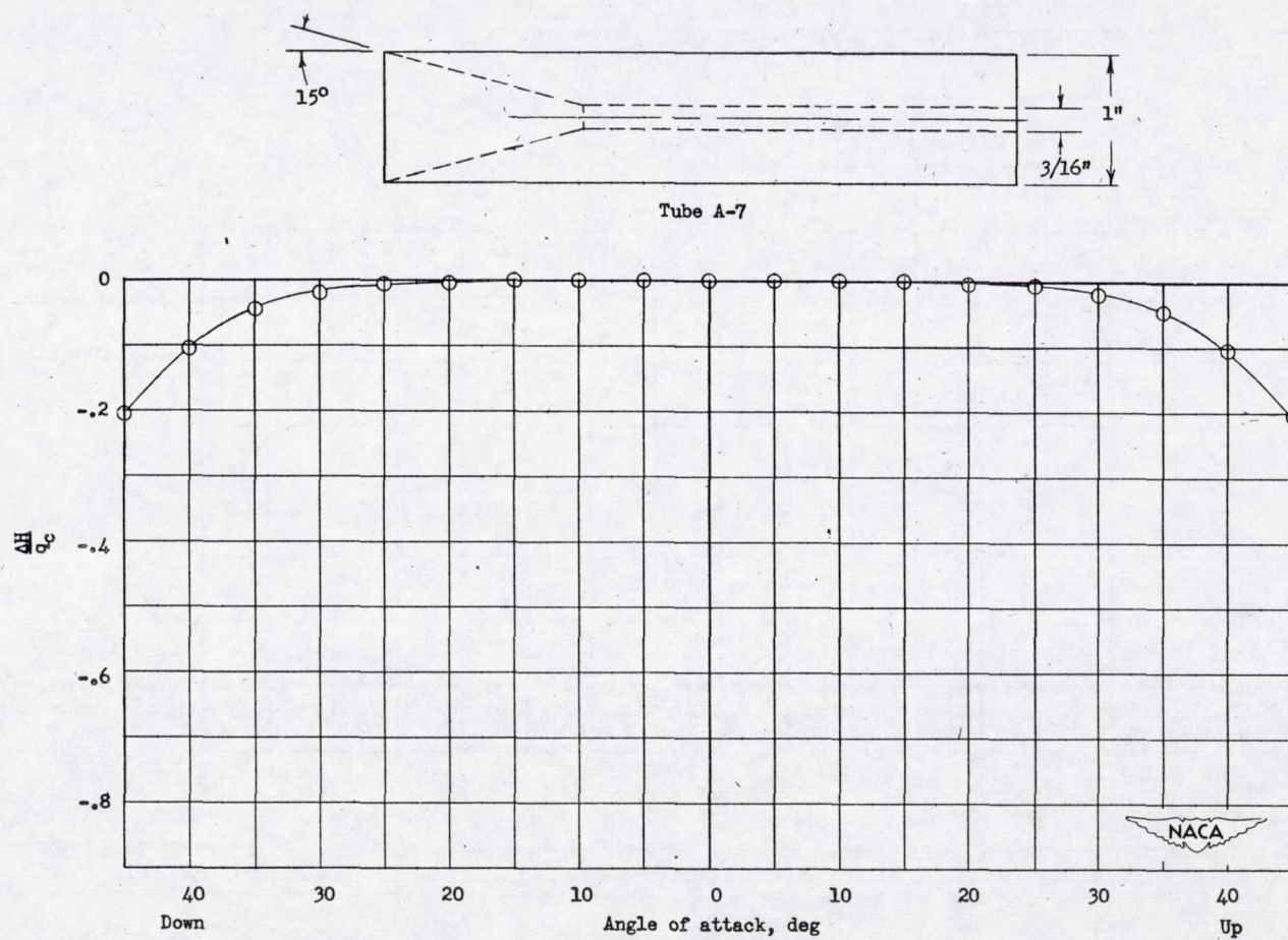
Figure 15.- Variation of total-pressure error with angle of attack. Tube A-7.
