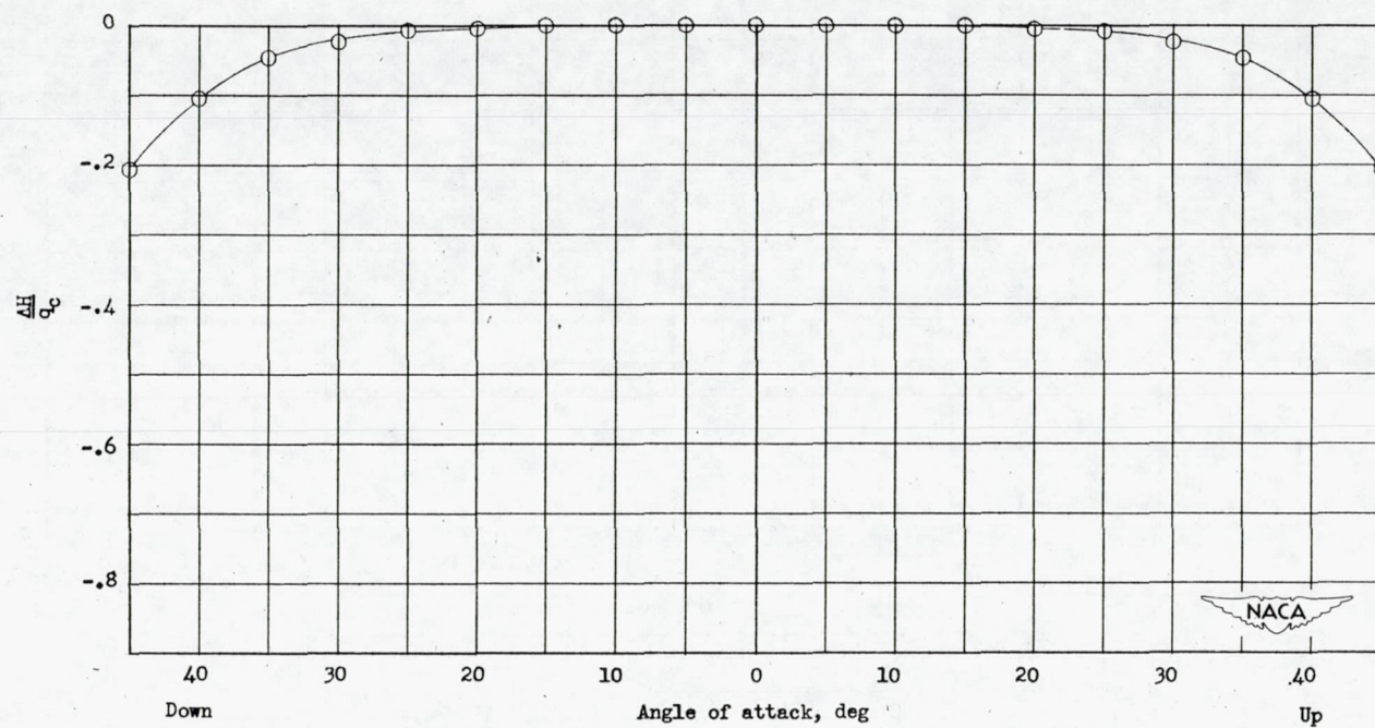
Figure 16.- Variation of total-pressure error with angle of attack. Tube A-8.
