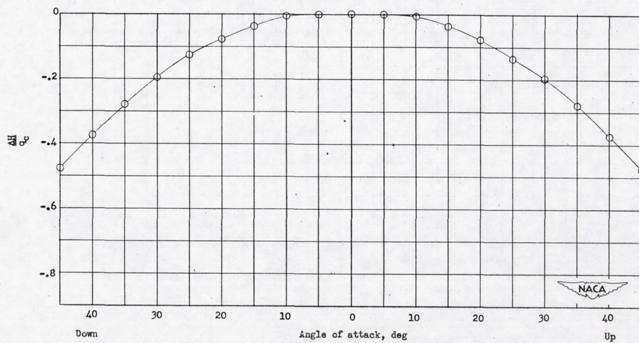
Figure 9.- Variation of total-pressure error with angle of attack. Tube A-1.
