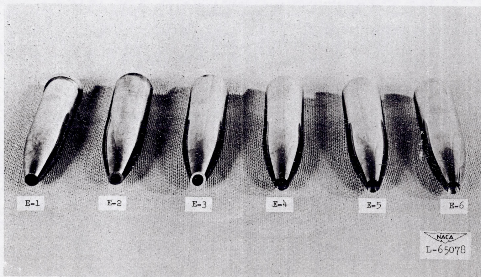
Figure 5.- Total-pressure tubes having ogival-nose sections. Series E.
