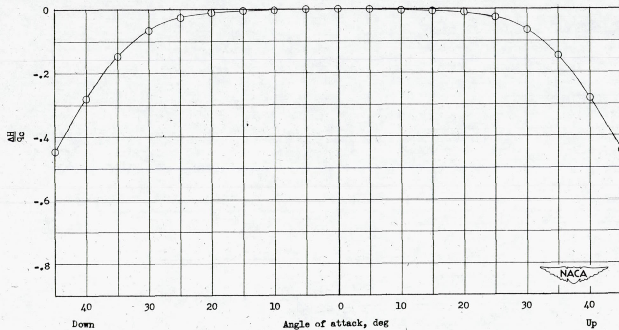
Figure 26.- Variation of total-pressure error with angle of attack. Tube B-5.
