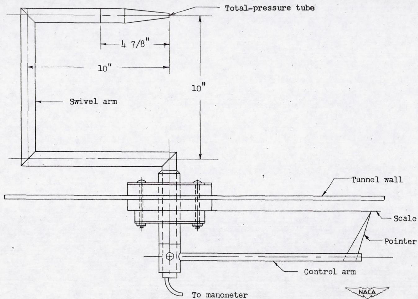
Figure 7.- Diagram of swivel mechanism used for changing angle of attack of total-pressure tubes.
