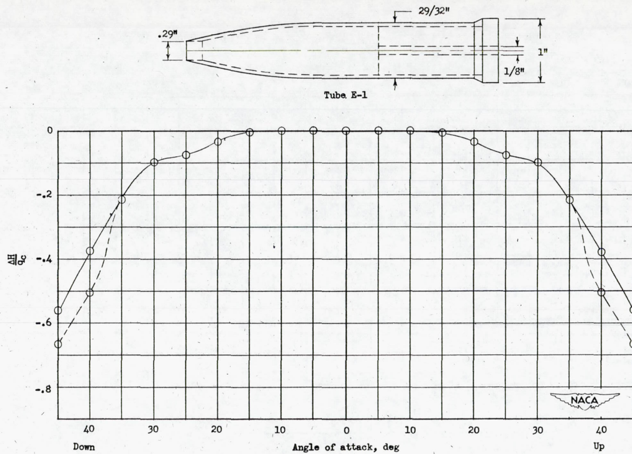
Figure 42.- Variation of total-pressure error with angle of attack. Tube E-1.
