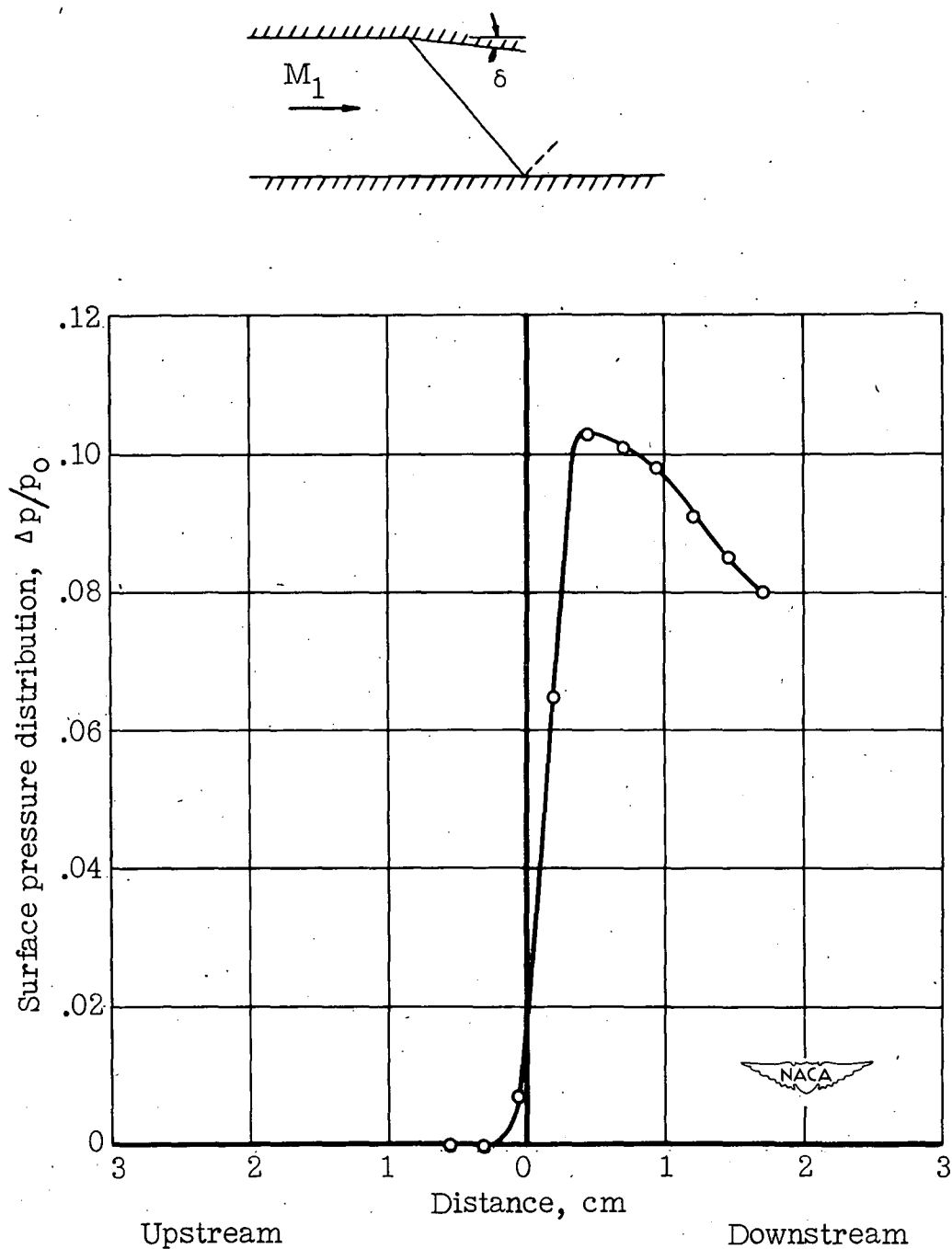
Figure 21.- Reflection of shock wave from flat surface (adapted from Fage and Sargent, reference 11, fig. 7). \delta , approx. 5^\circ ; M_1 , 1.47; R , 6 \times 10^6 ; turbulent boundary layer; theoretical \Delta p/p_0 , 0.19.
