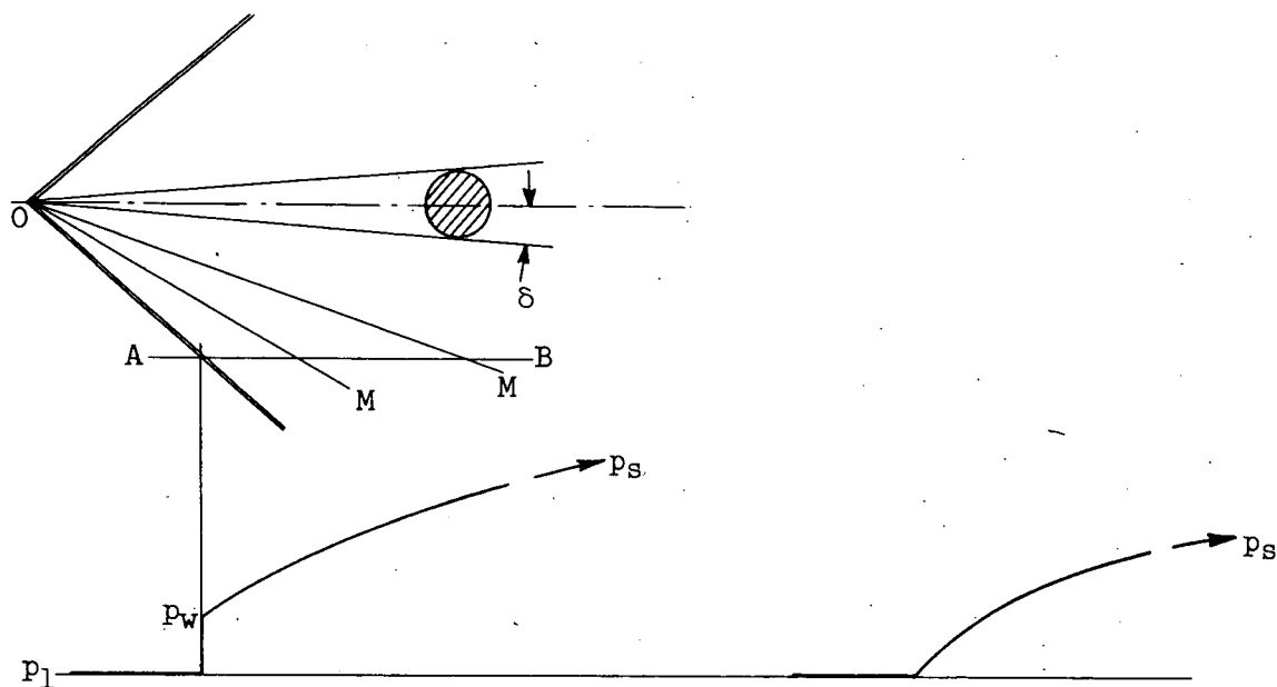
Conical pressure fields.
