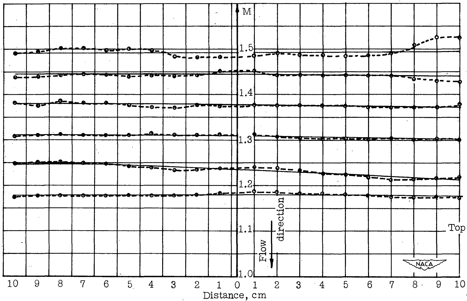
Figure 41.- Vertical Mach number distribution. Empty tunnel.
