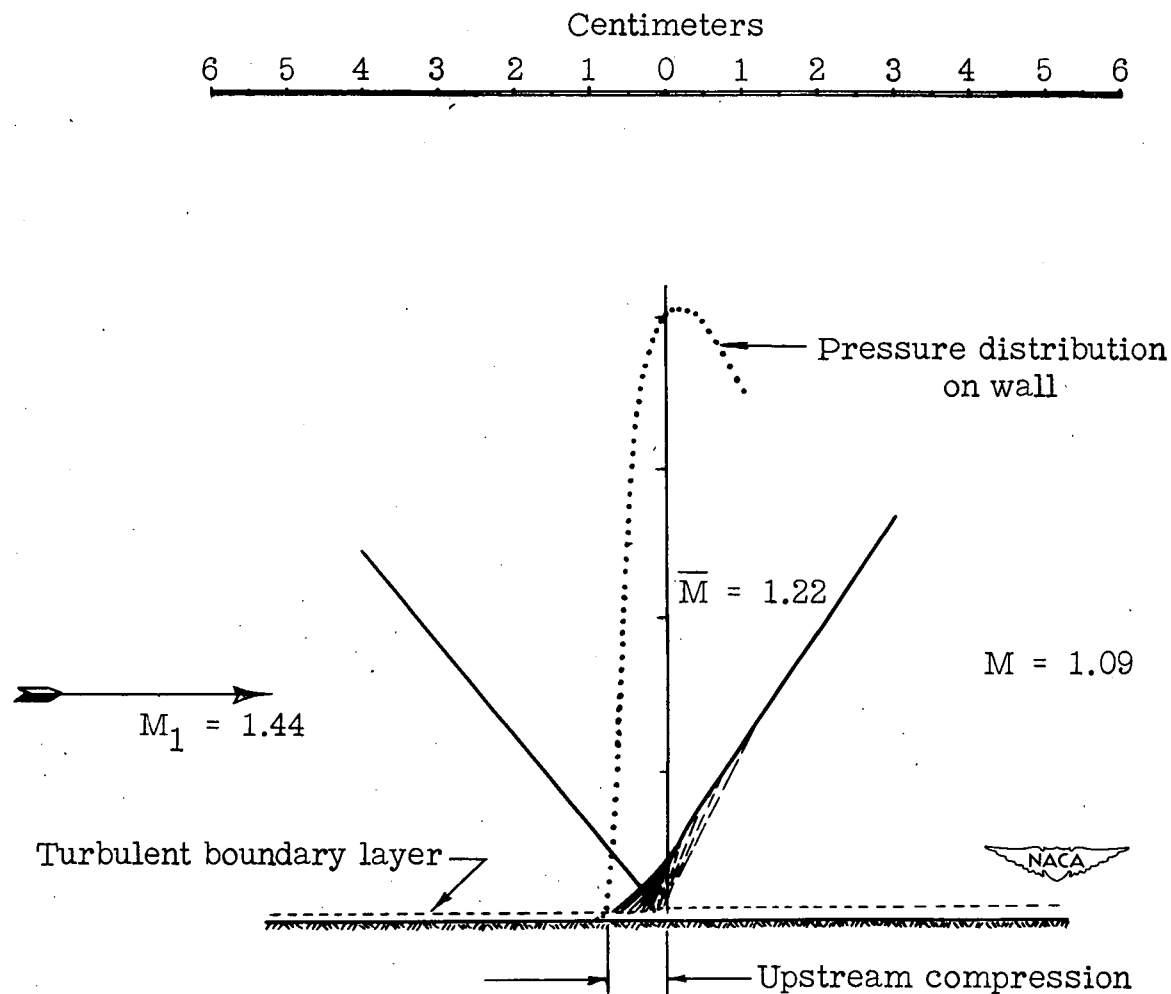
Figure 34.- Model of shock-wave reflection from flat surface with turbulent boundary layer. Full-scale; incident wave \delta, 4.5^\circ ; M_1, 1.44 ; R, 0.9 \times 10^6 .
