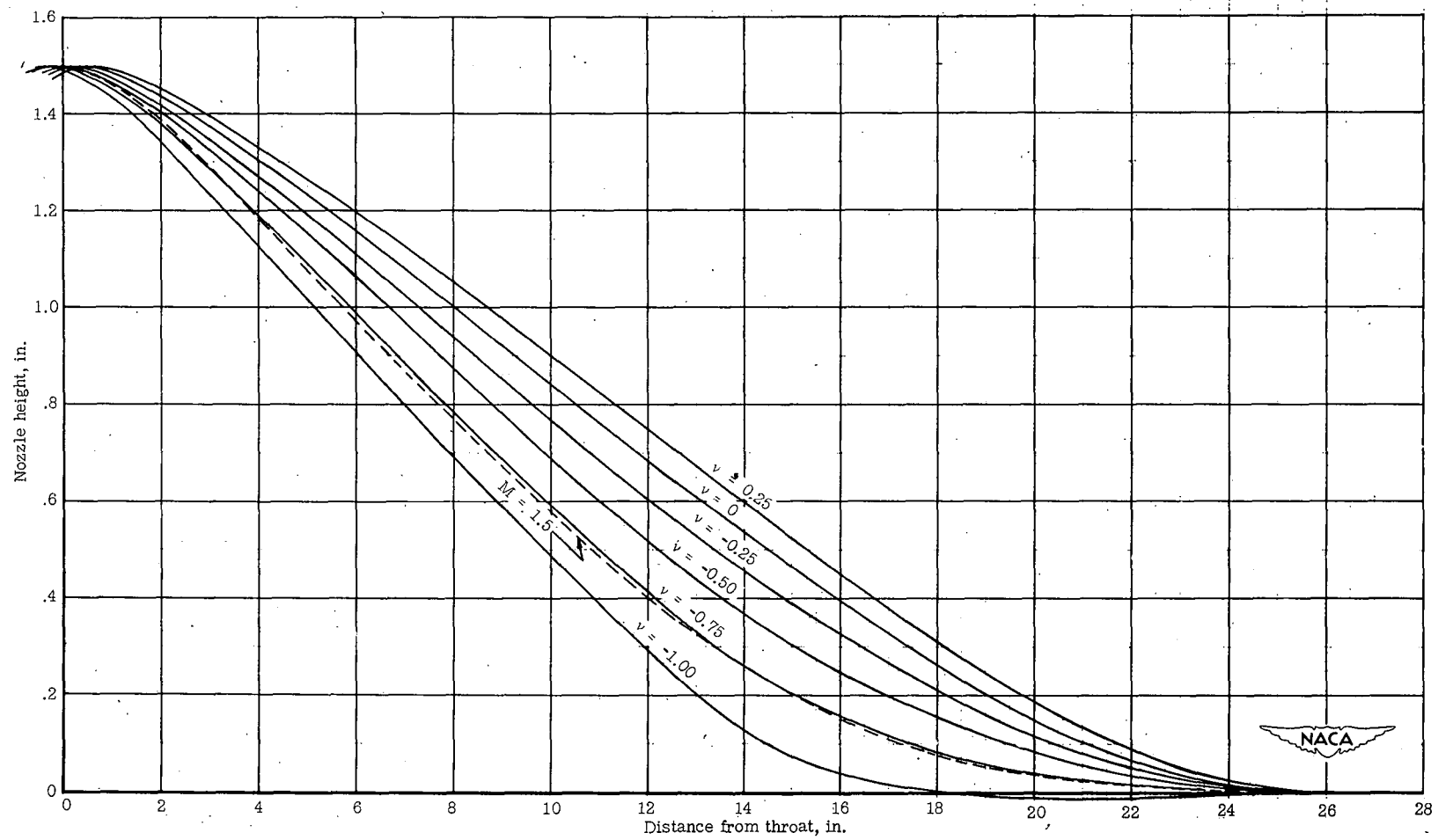
Figure 39.- Matching of aerodynamic and elastic shapes. M = 1.5 .
