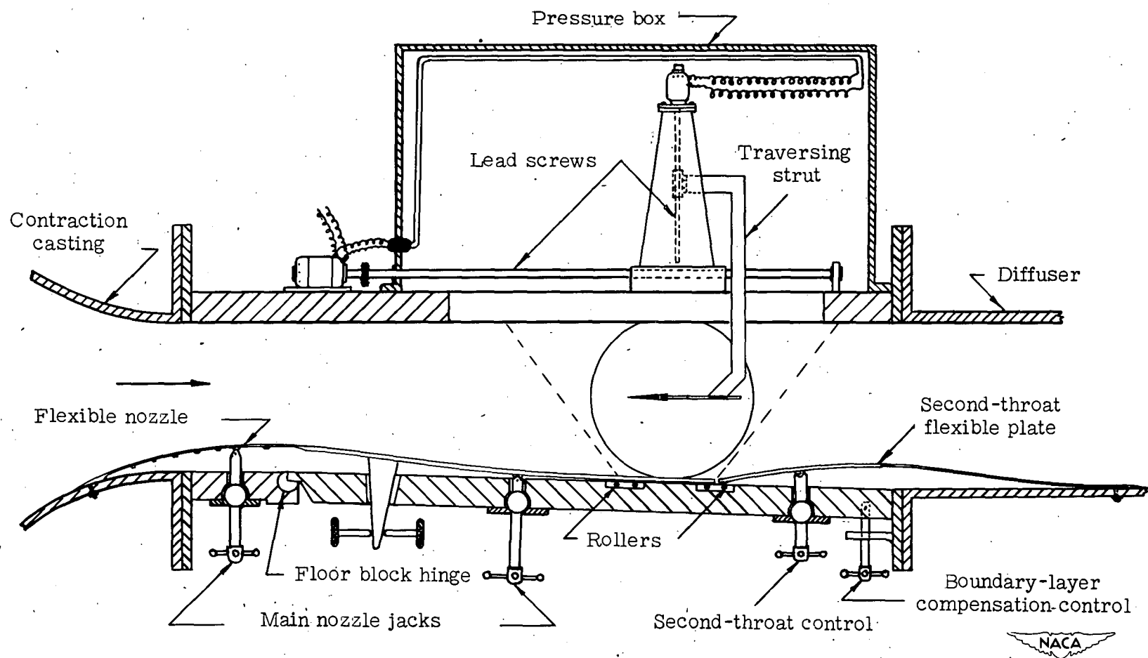
Figure 14.- Sketch of GALCIT 4-by 10-by 48-inch transonic-tunnel test section.
