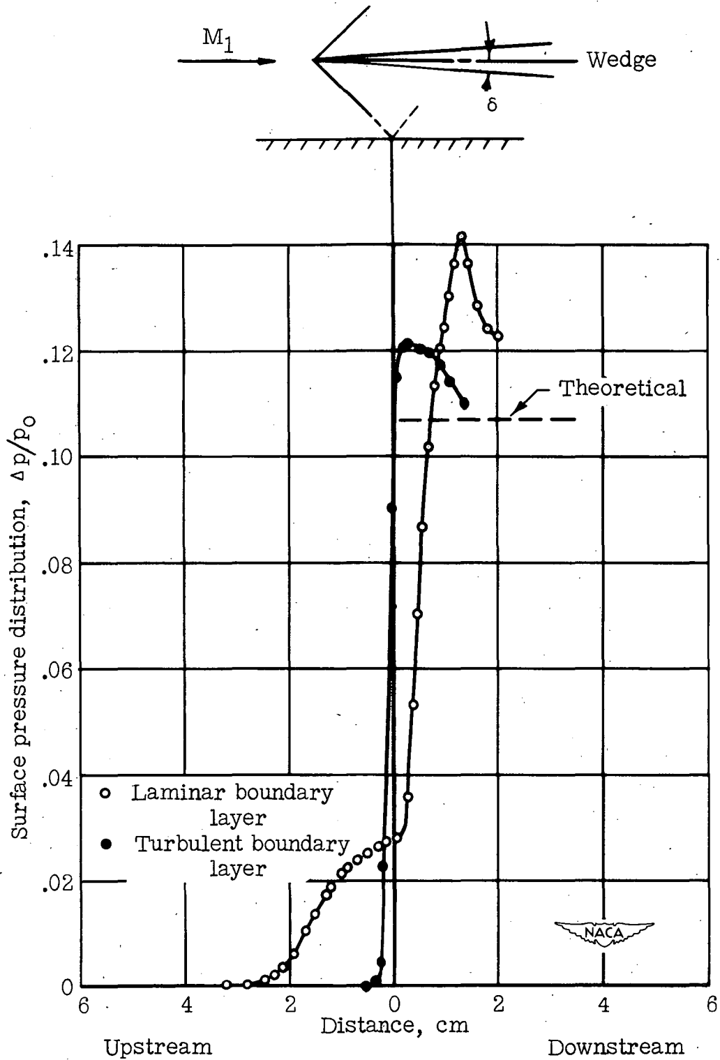
Figure 22.- Reflection of shock wave from flat surface. \delta = 3^\circ ; M_1 = 1.4 ; R = 0.9 \times 10^6 .
