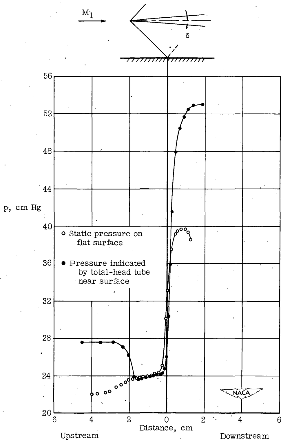
Figure 33.- Reflection of shock wave from flat surface. Conditions near surface with laminar boundary layer; \delta = 4.5^\circ ; M_1 = 1.44 ; R = 0.9 \times 10^6 .
