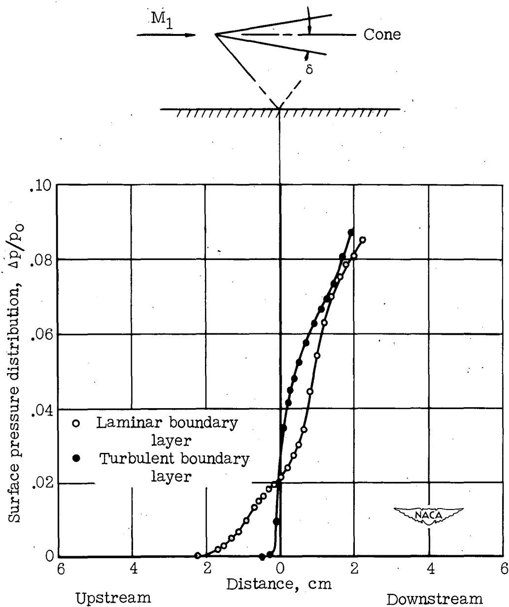
Figure 24.- Reflection of conical shock wave from flat surface. \delta = 10^\circ ; M_1 = 1.35 ; R = 0.9 \times 10^6 .
