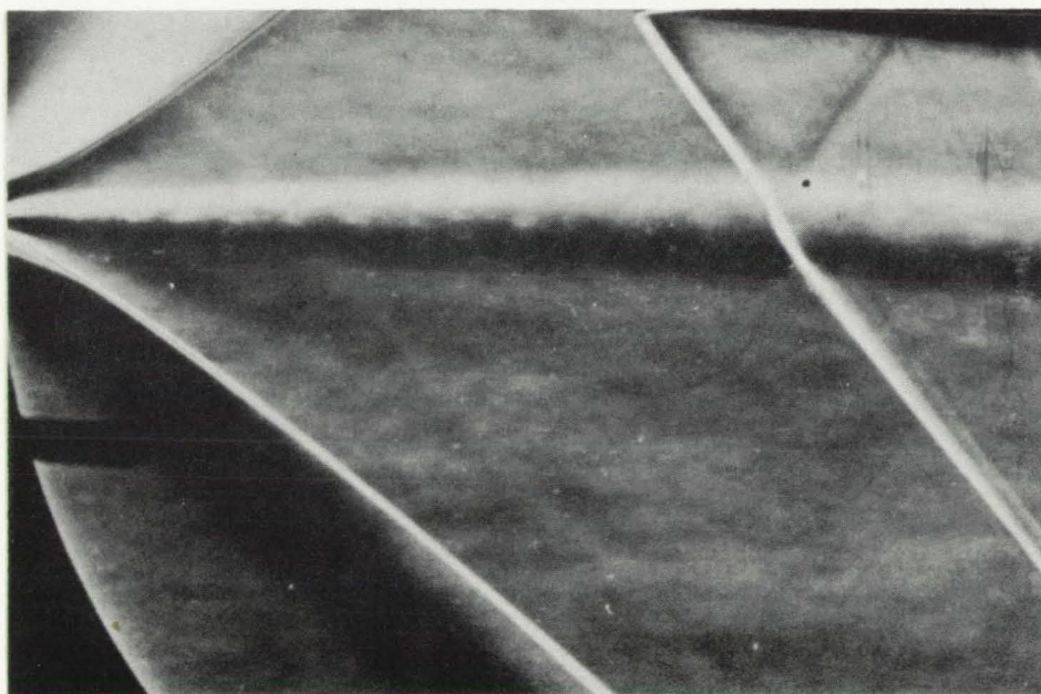
(b) Reflection 5 centimeters behind trailing edge.
