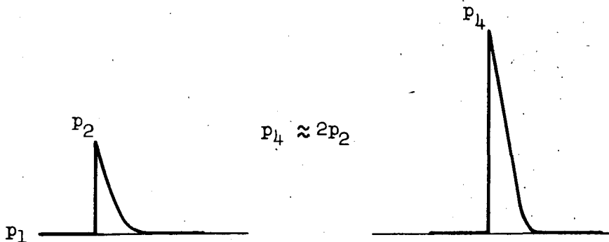
Surface pressure at reflection from flat surface.
