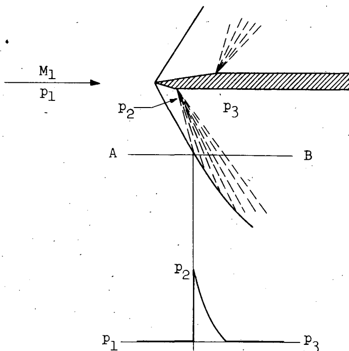
Impulse-type wave.
