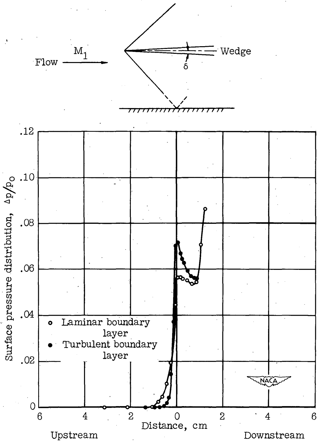
Figure 29.- Reflection of impulse-type shock wave from flat surface. \delta = 1.5^\circ ; M_1 = 1.43 ; R = 0.9 \times 10^6 .
