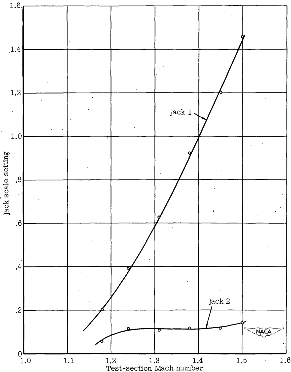
Figure 45.- Flexible-nozzle control settings.
