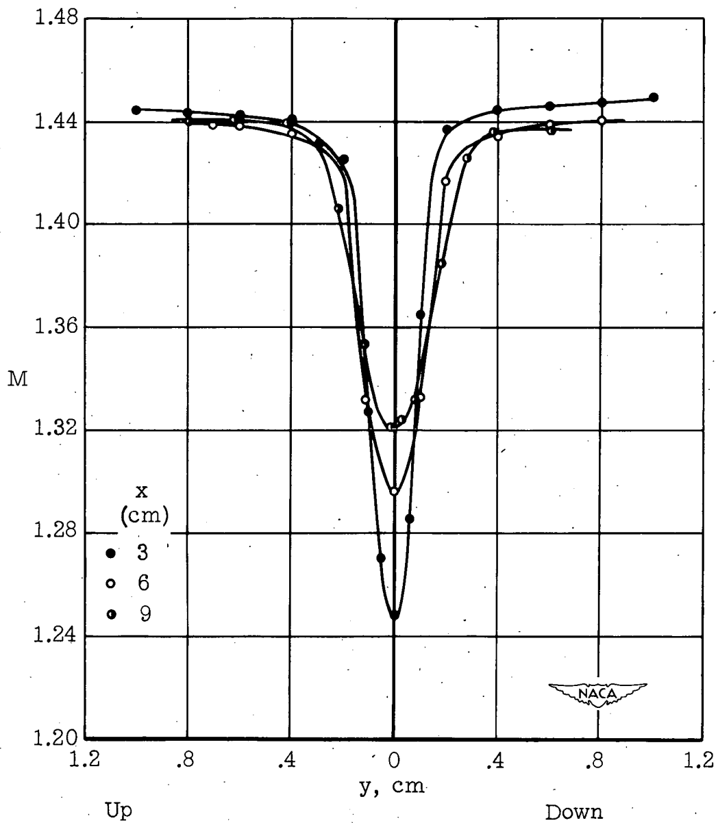
Figure 37.- Typical Mach number profiles in wake of flat plate. x , distance behind trailing edge; y , distance from center line of wake.
