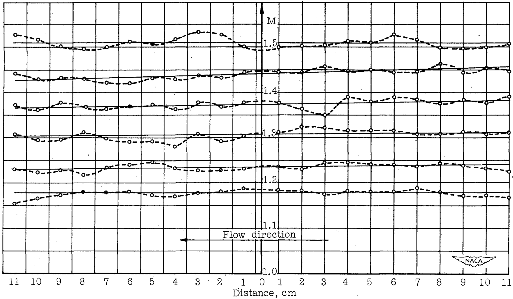
Figure 42.- Horizontal Mach number distribution. Empty tunnel.
