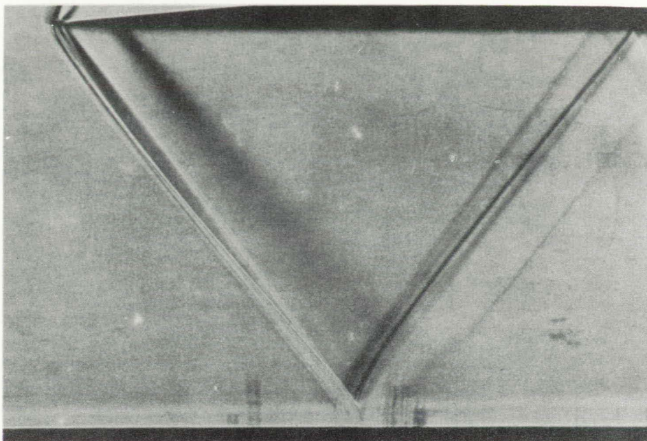
(a) Turbulent boundary layer.
