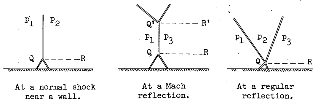
Bifurcated shocks.
