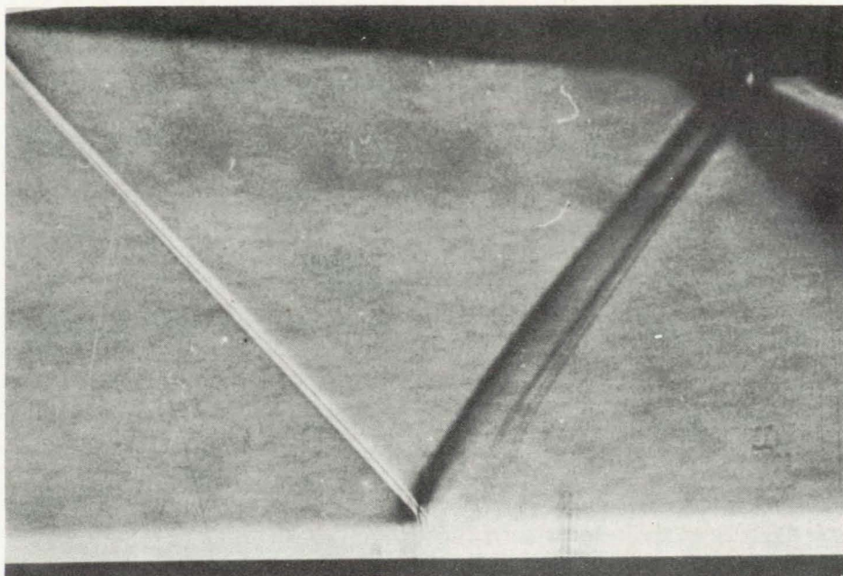
(a) Turbulent boundary layer.
