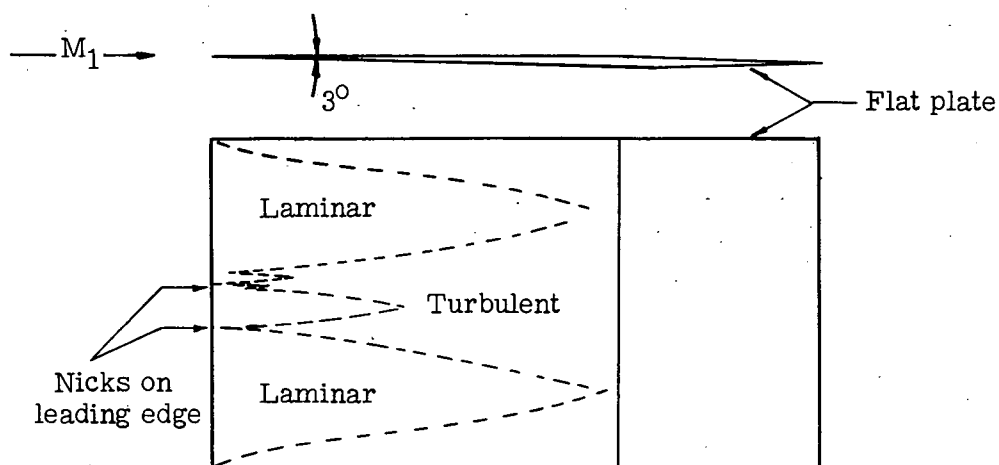
(a) Effect of leading-edge imperfections.
