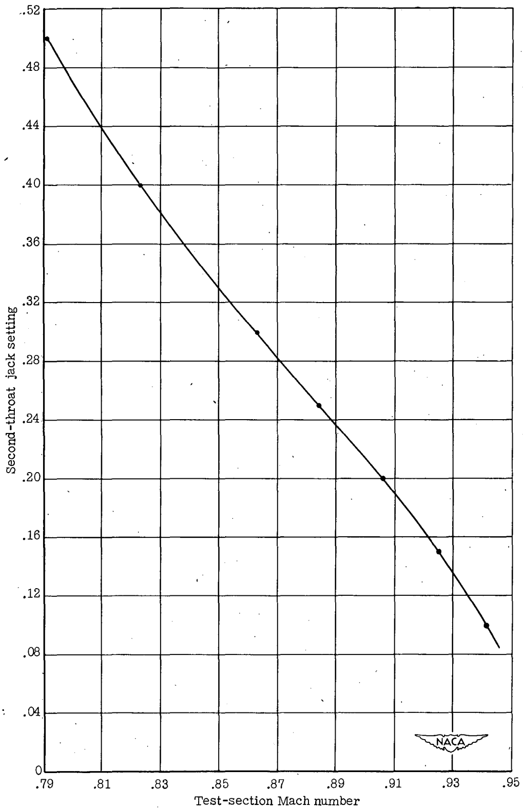
Figure 46.- Second-throat calibration for subsonic operation.
