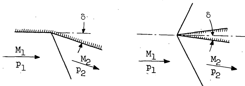
Examples of step waves.
