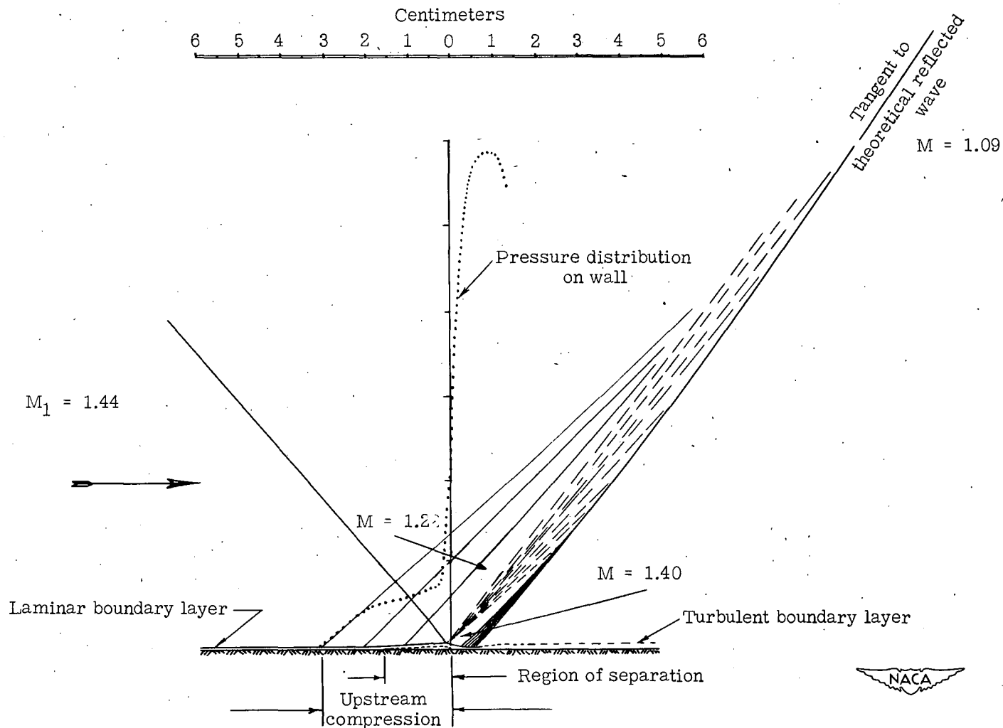
Figure 35.- Model of shock-wave reflection from flat surface with laminar boundary layer. Full-scale; incident wave \delta, 4.5^\circ ; M_1, 1.44 ; R, 0.9 \times 10^6 .
