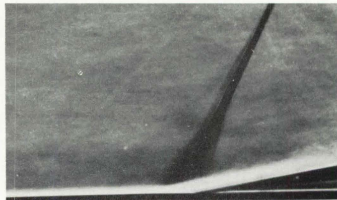
(b) Laminar boundary layer; M_1 = 1.42.
