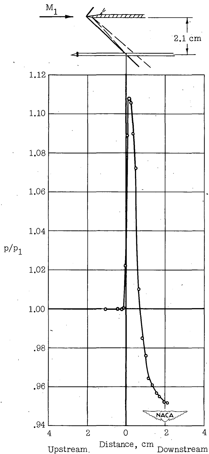
Figure 9.- Static-pressure survey through impulse-type wave. M_1 = 1.38 .
