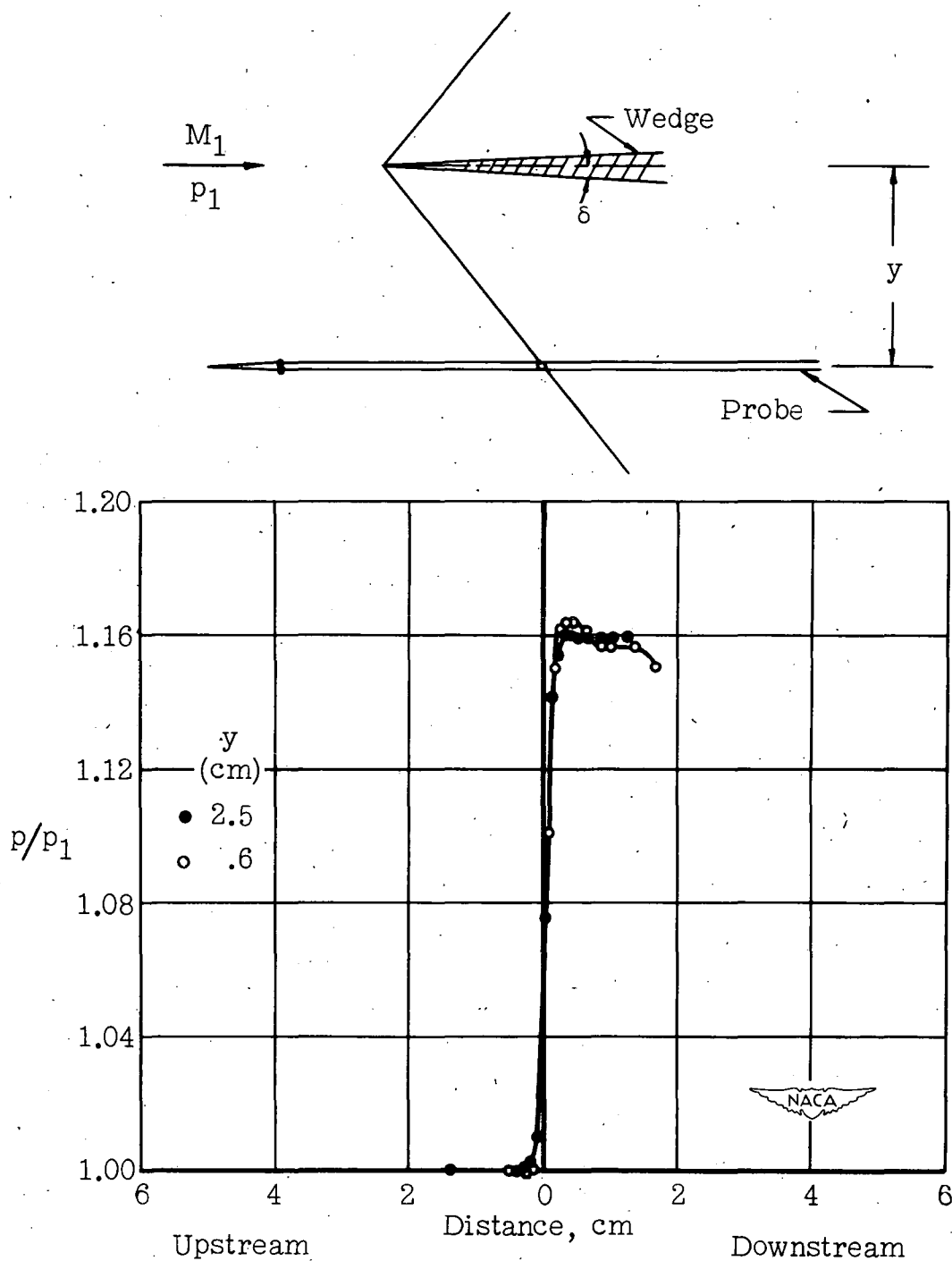
Figure 4.- Effect of distance from origin of shock wave. \delta , 3^\circ ; M_1 , 1.36; probe boundary layer, turbulent.
