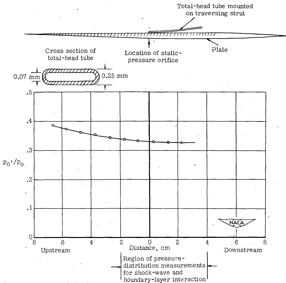
Figure 15.- Variation of total head along flat surface with laminar boundary layer. p_o' , pressure indicated by total-head tube; p_o , stagnation pressure.
