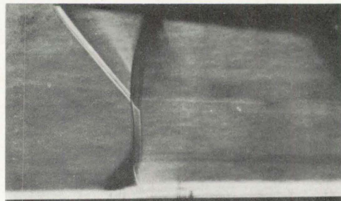
(b) Mach reflection.
