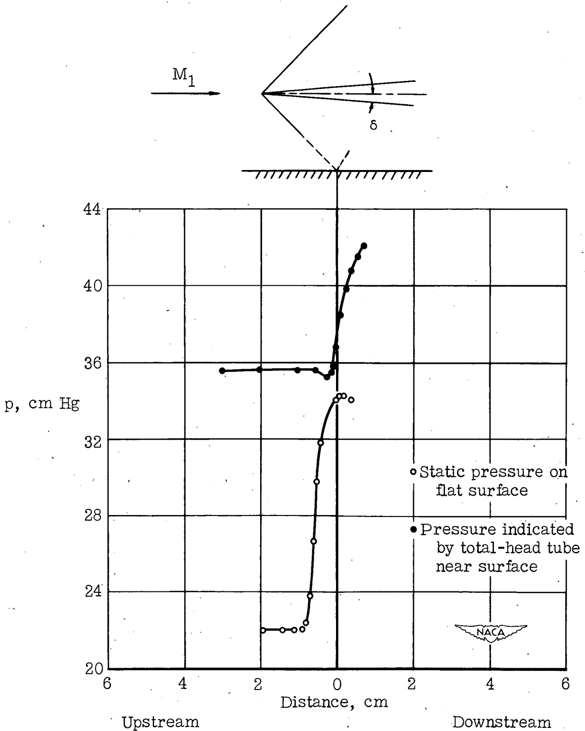
Figure 32.- Reflection of shock wave from flat surface. Conditions near surface with turbulent boundary layer; \delta = 4.5^\circ ; M_1 = 1.44 ; R = 0.9 \times 10^6 .
