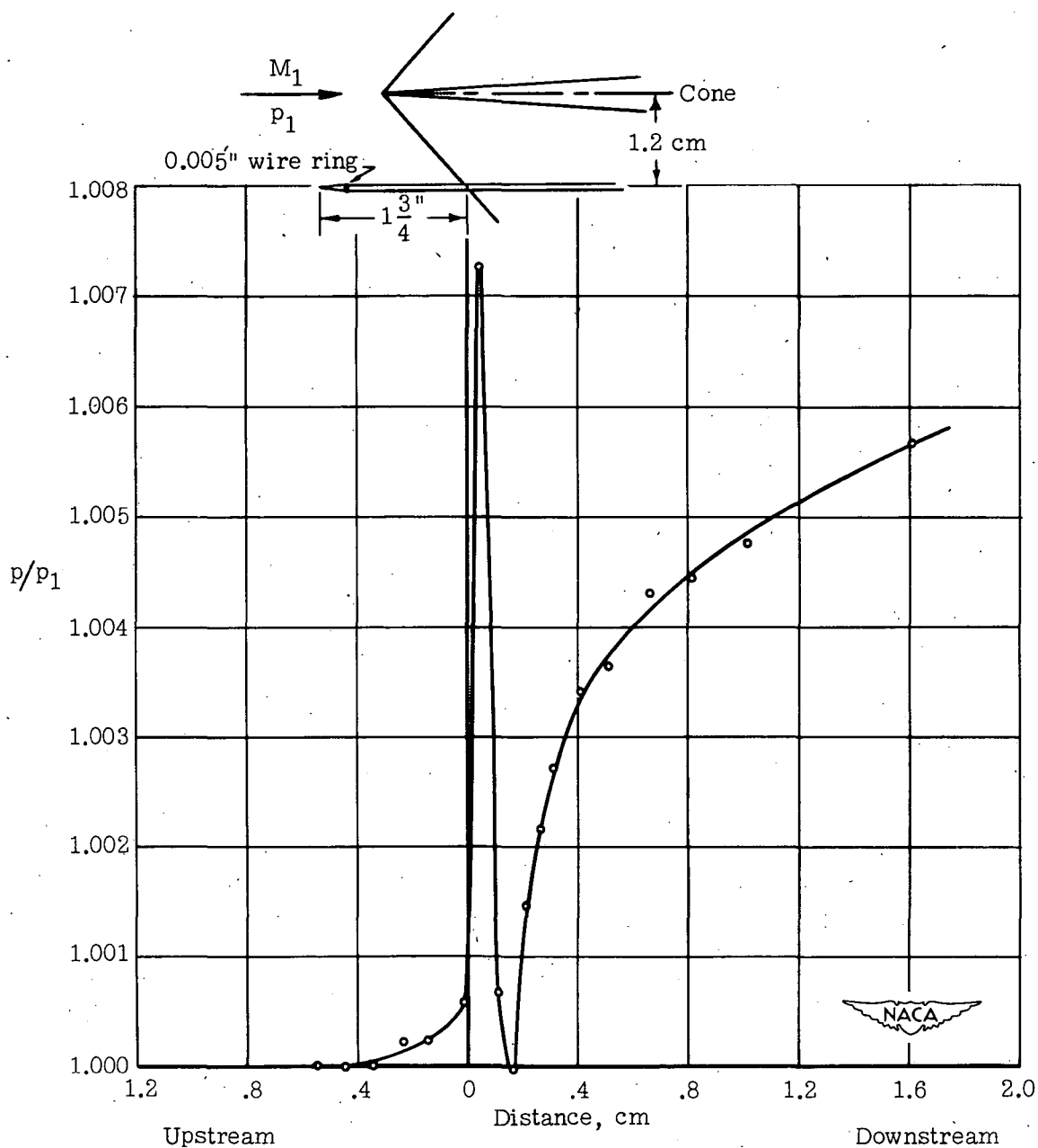
Figure 6.- Static-pressure survey through impulse-type wave from 2^\circ cone. M_1 , 1.32; cone nose radius, 0.01 centimeter.
