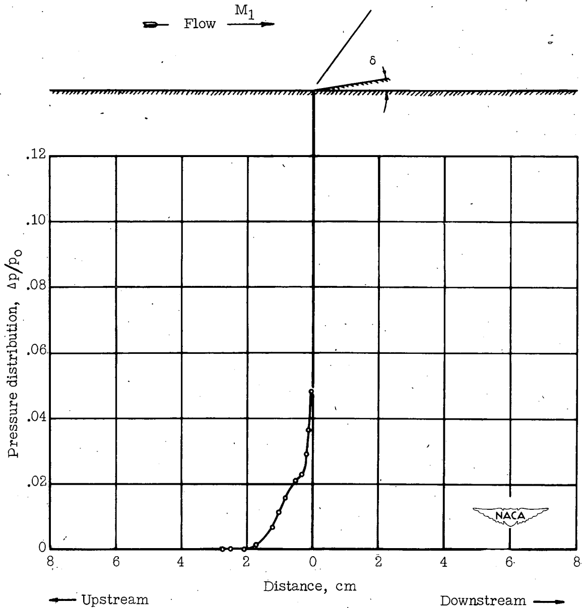
Figure 27.- Flow in corner. Laminar boundary layer; corner angle \delta, 10^\circ ; M_1, 1.55 ; R, 0.9 \times 10^6 .
