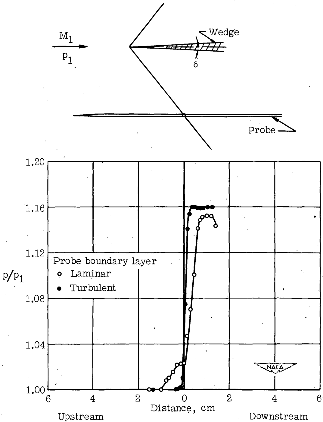
Figure 5.- Effect of probe boundary layer on static-pressure measurements through a shock wave. \delta = 30^\circ ; M_1 = 1.354 .
