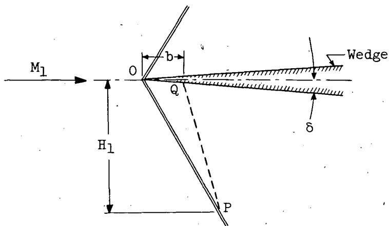
Nonviscous flow impinging on wedge.
