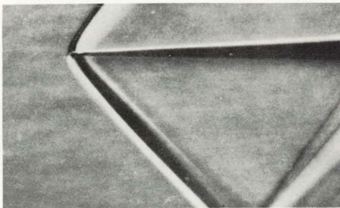
(a) Semiangle \delta , 1.5^\circ ; nose radius, 0.005 centimeter; M_1 , 1.44.
