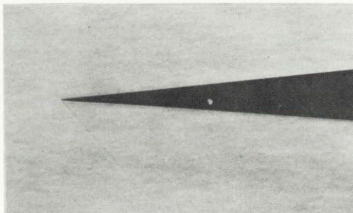
(b) Semiangle \delta , 5^\circ ; nose radius, 0.007 centimeter; M_1 , 1.32.
