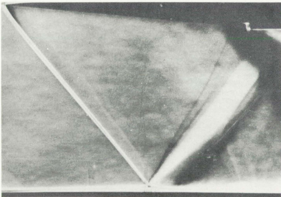
(b) Laminar boundary layer.
