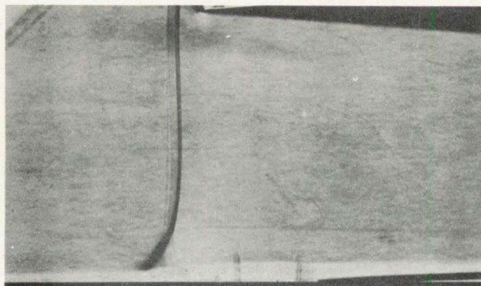
(a) Normal shock at mouth of duct.
