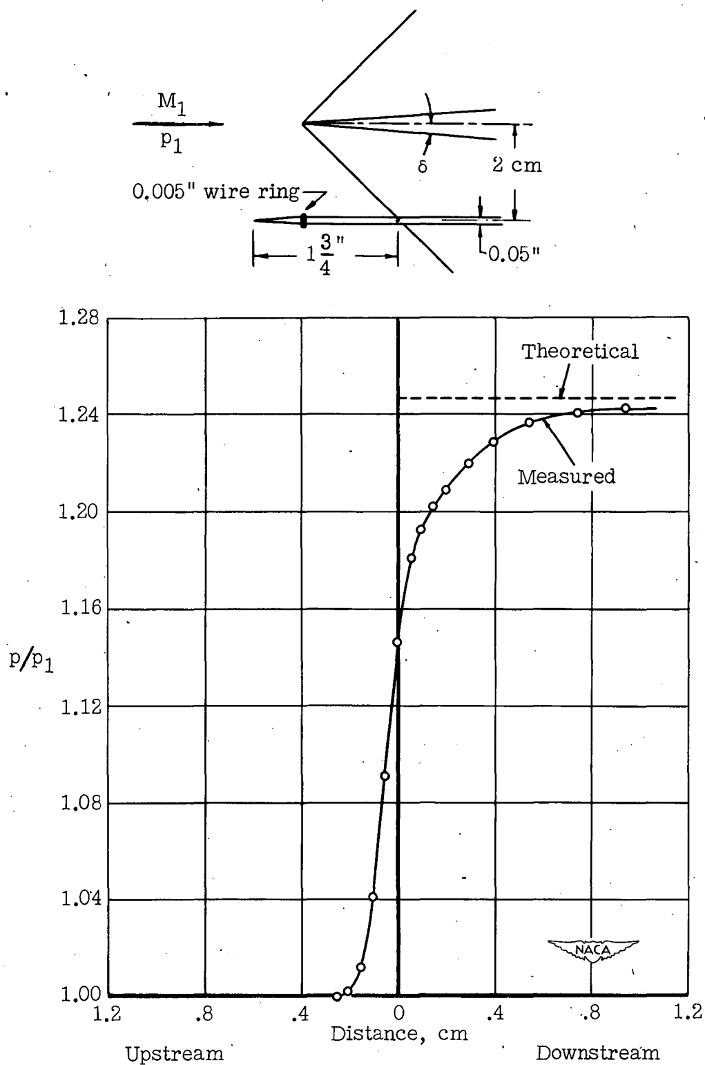
Figure 20.- Static-pressure survey through step wave from 4.5^\circ wedge. \delta = 4.5^\circ ; M_1 = 1.44..
