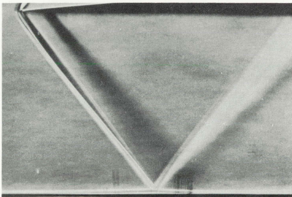
(b) Laminar boundary layer.
