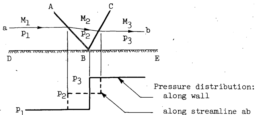
Shock reflection in nonviscous flow.
