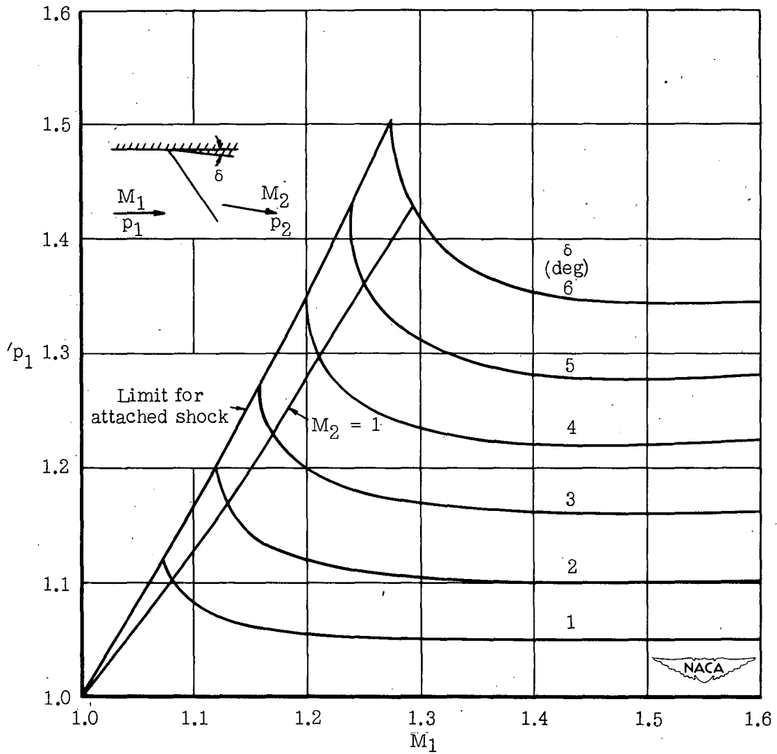
Figure 10.- Pressure ratio across inclined shock.
