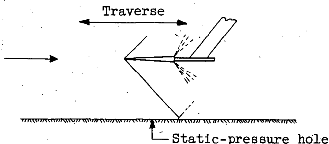
Intersection of shock wave from wedge or cone with plate.
