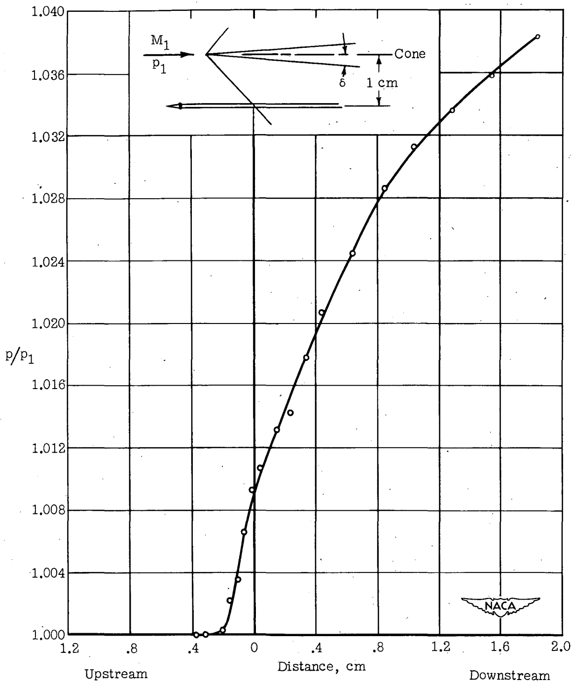
Figure 7.- Static-pressure survey through wave from 5° cone. \delta , 5°; M_1 , 1.32; cone nose radius, 0.007 centimeter.
