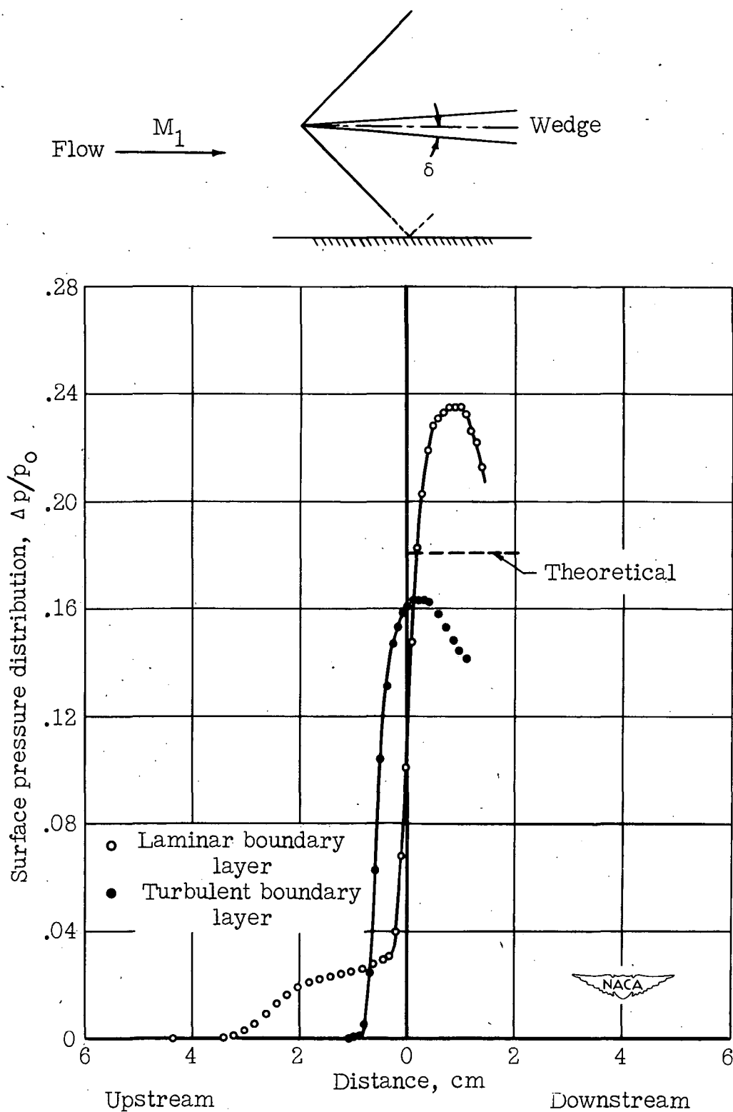
Figure 19.- Reflection of shock wave from flat surface. \delta = 4.5^\circ ; M_1 = 1.44 ; R = 0.9 \times 10^6 .
