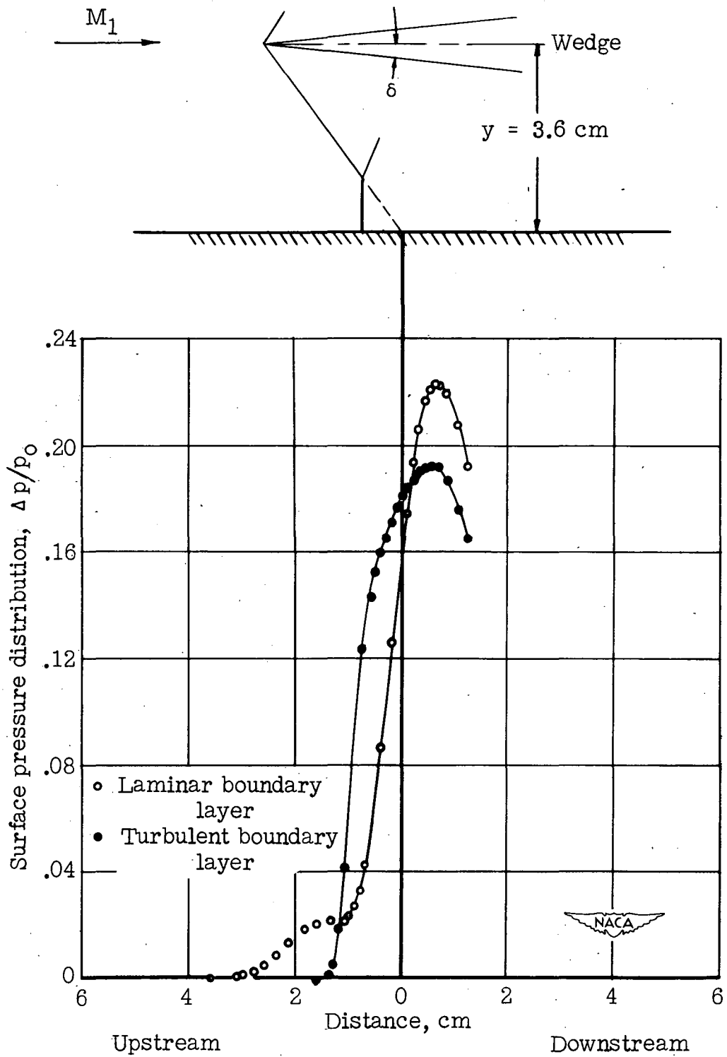
Figure 23.- Mach reflection. \delta = 6.5^\circ ; M_1 = 1.43 ; R = 0.9 \times 10^6 .
