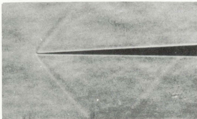
(a) Semiangle \delta , 2^\circ ; nose radius, 0.01 centimeter; M_1 , 1.32.
