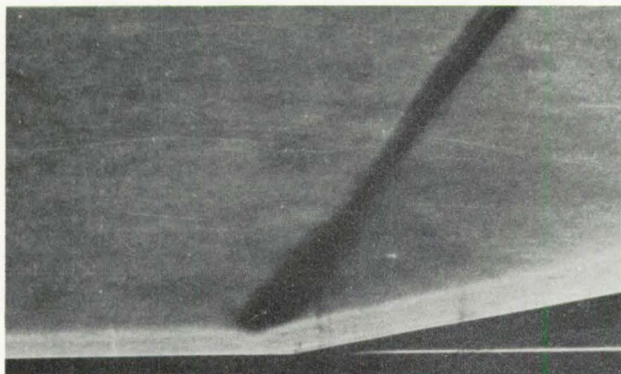
(c) Turbulent boundary layer; M_1 = 1.55.
