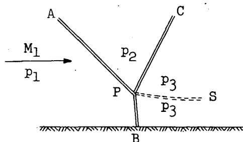
Mach reflection.
