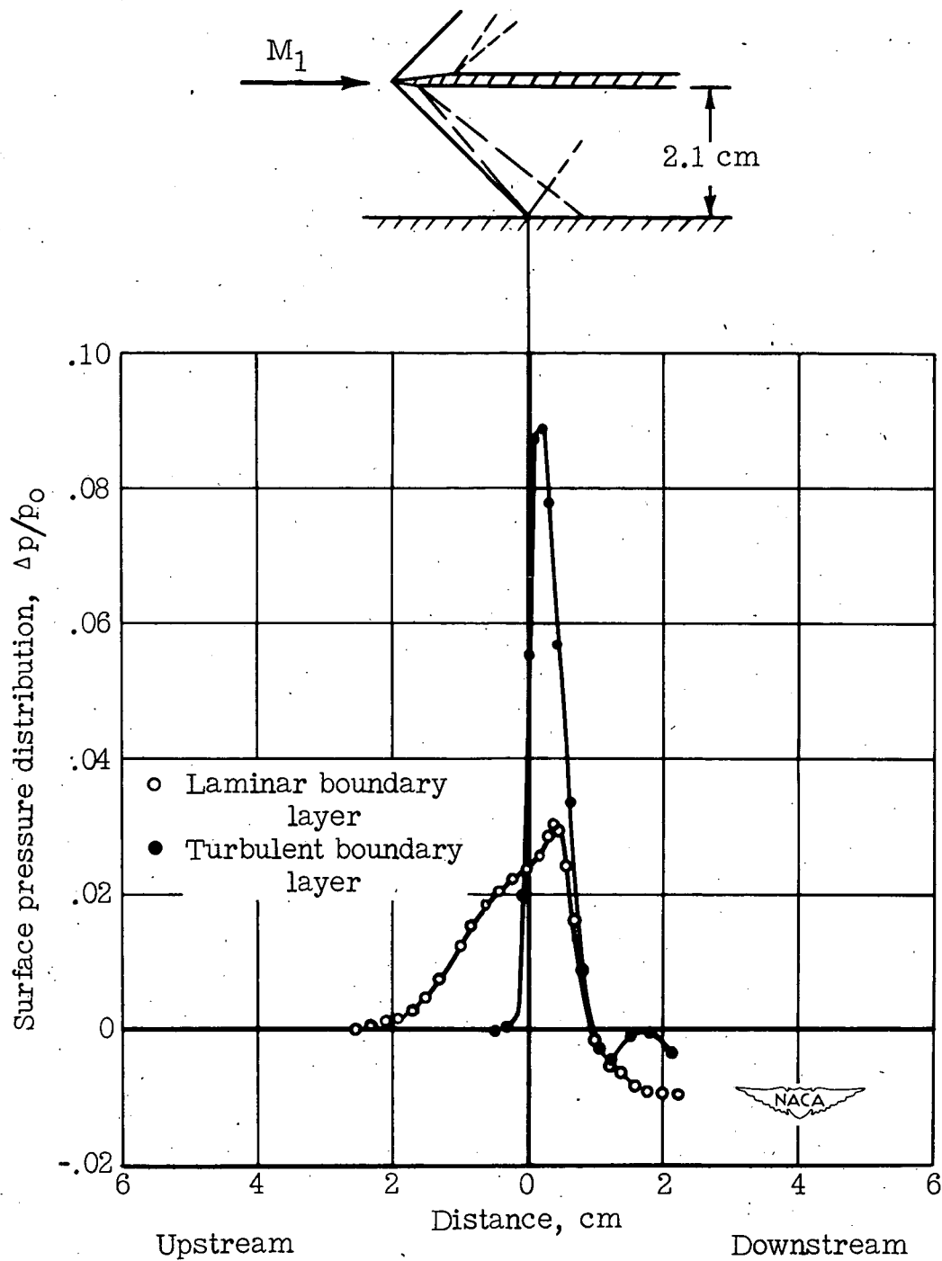
Figure 31.- Reflection of impulse-type wave from flat surface. M_1 = 1.38 ; R = 0.9 \times 10^6 .
