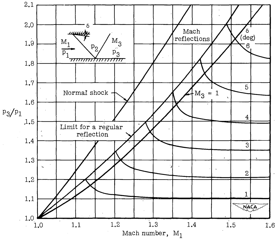
Figure 11.- Pressure ratio across regular reflection.
