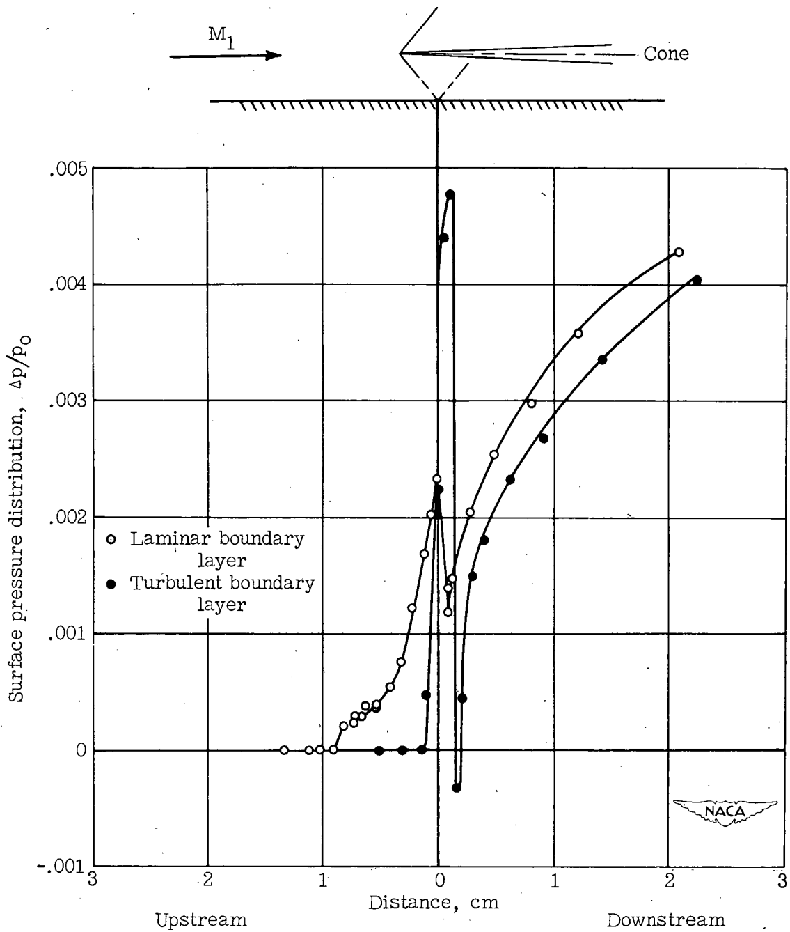
Figure 28.- Reflection of impulse-type wave. M_1 = 1.32 ; R = 0.9 \times 10^6 .
