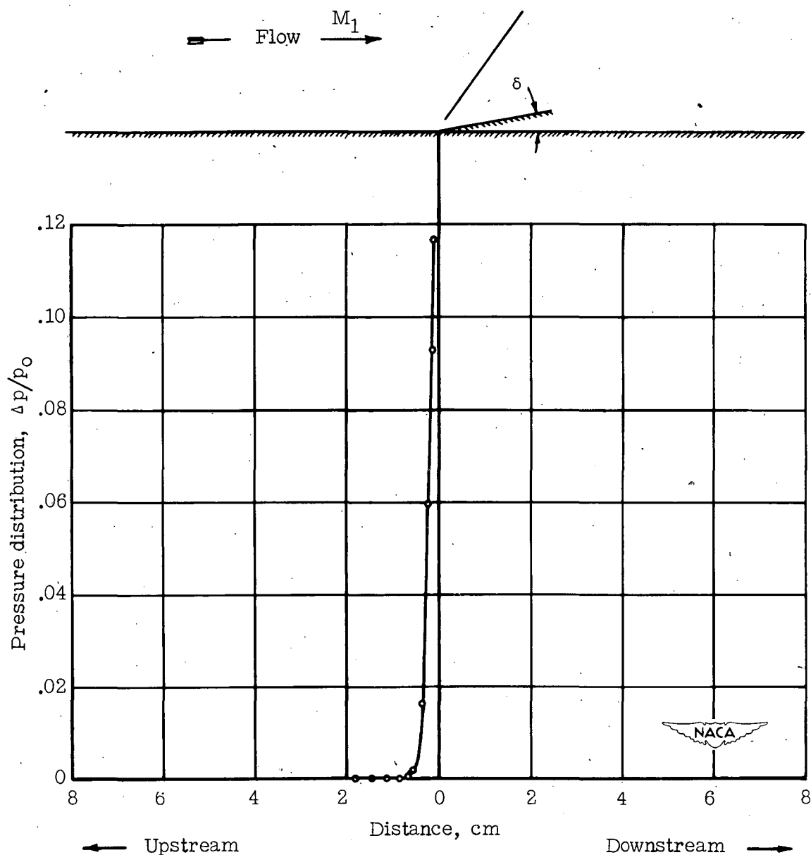
Figure 26.- Flow in corner. Turbulent boundary layer; corner angle \delta, 10^\circ ; M_1, 1.55 ; R, 0.9 \times 10^6 .
