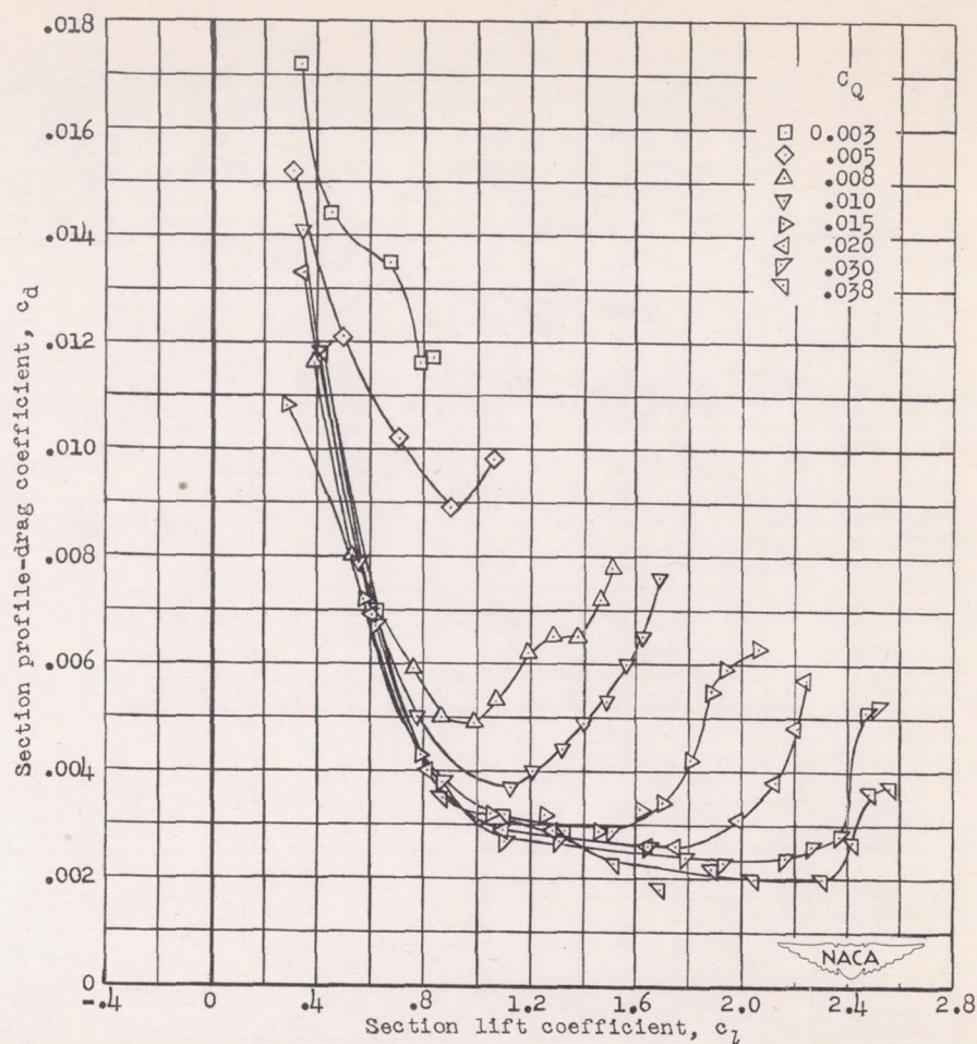
(a) Lift and profile drag.
