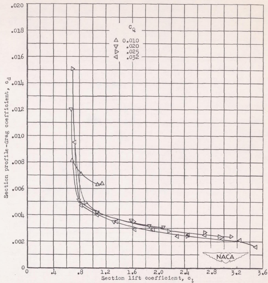
(a) Lift and profile drag.
