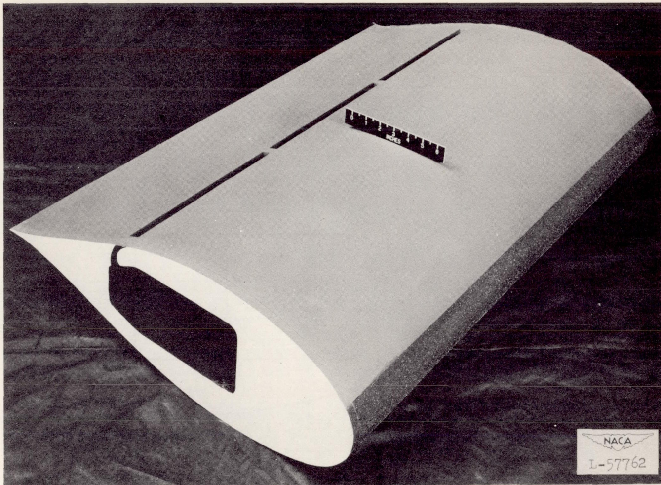
Figure 4.- Three-quarter view of the model of the NACA 64,2-432 airfoil section with a 0.016c boundary-layer-control slot at 0.60c and leading-edge roughness.
