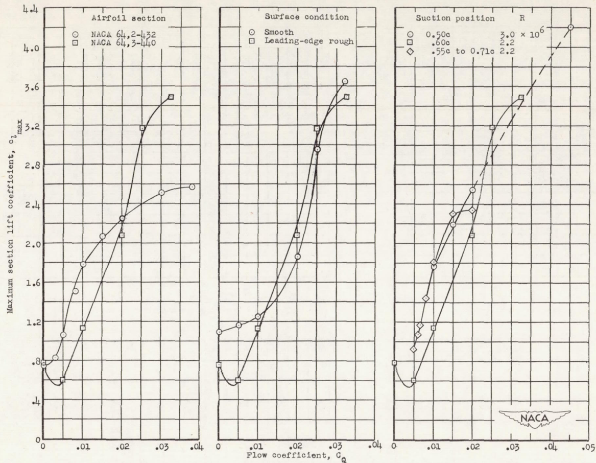
(a) Effect of airfoil thickness; slot at 0.60c; models in rough condition; R = 2.2 \times 10^6 . (b) Effect of surface condition; NACA 64,3-440 airfoil; slot at 0.60c; R = 2.2 \times 10^6 . (c) Effect of position of suction; NACA 64,3-440 airfoil; rough condition.
