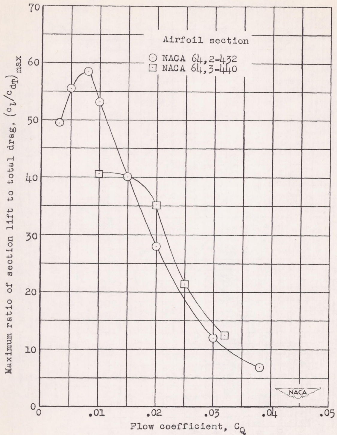
Figure 15.- Effect of flow coefficient on the maximum ratio of section lift to total drag of the NACA 64,2-432 and 64,3-440 airfoil sections. Suction slot at 0.60c ; R = 2.2 \times 10^6 .
