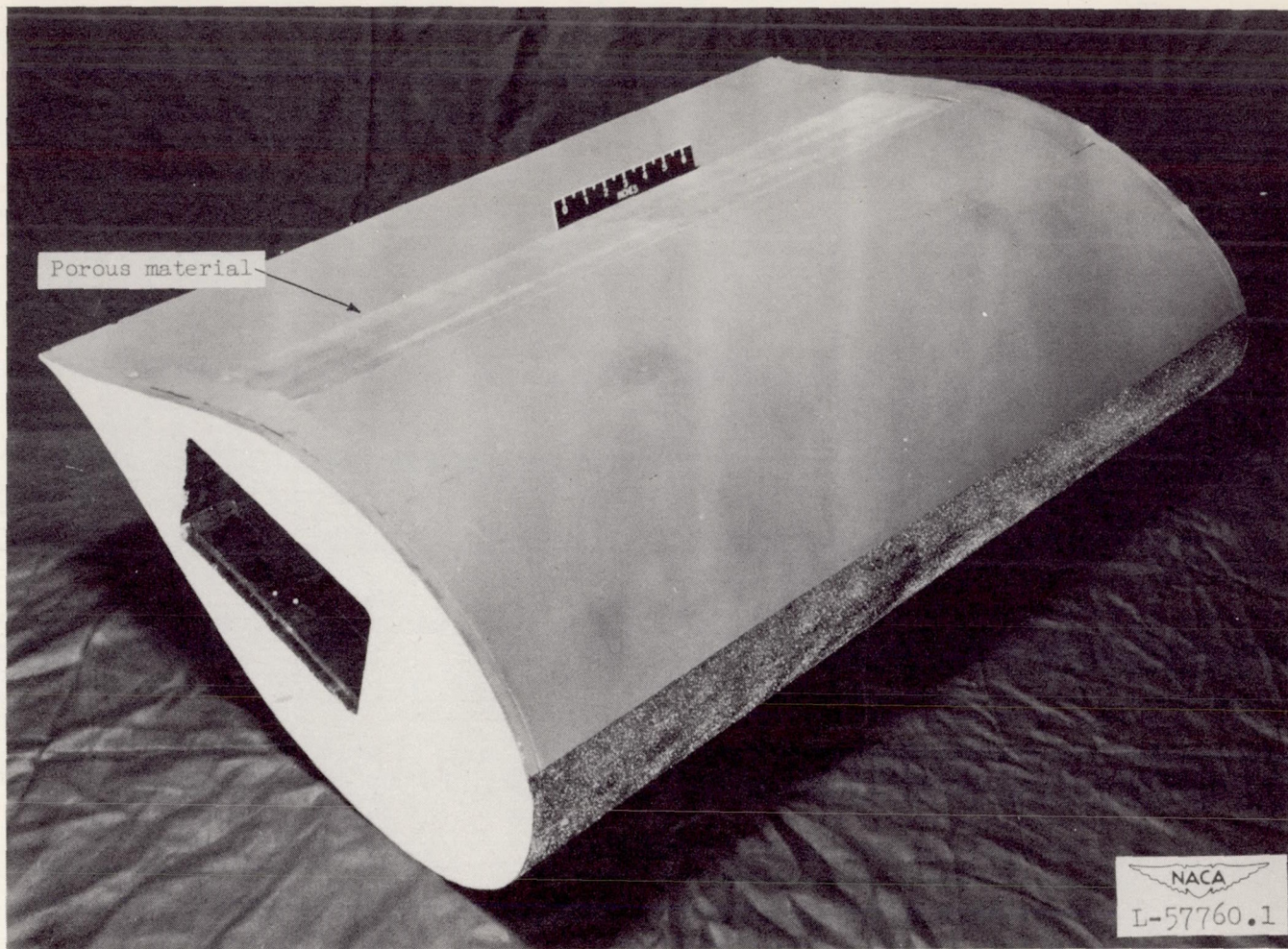
Figure 6.- Three-quarter view of the model of the NACA 64,3-440 airfoil section with a porous upper surface from 0.55c to 0.71c and leading-edge roughness.
