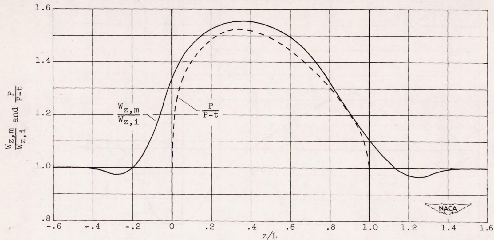
Figure 10. - Comparison between axial velocity along mean streamline and channel-width ratio for incompressible solution.
