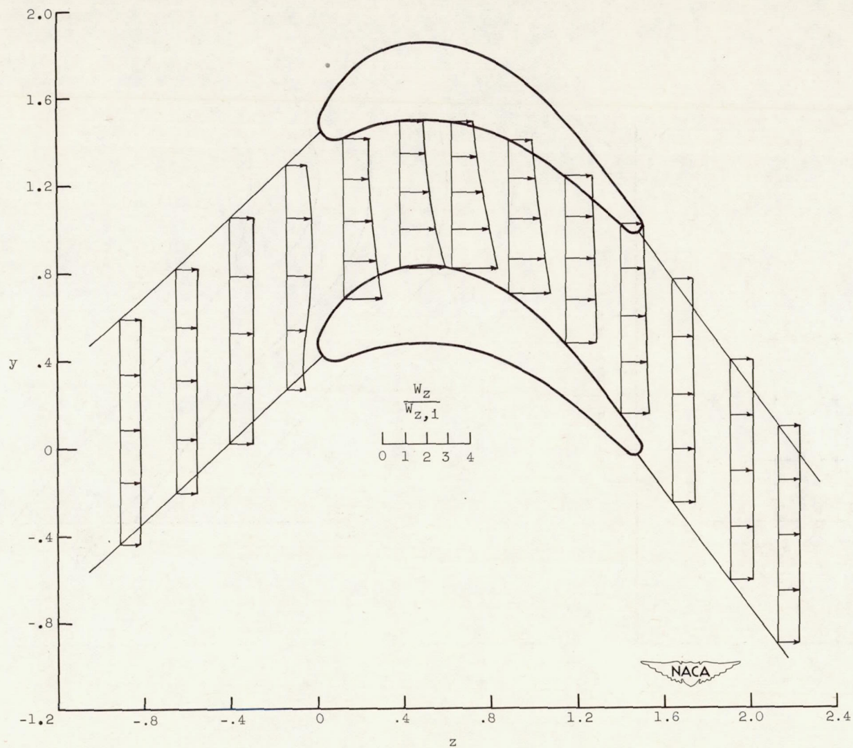
Figure 5. - Variation of axial velocity across channel for incompressible solution.
