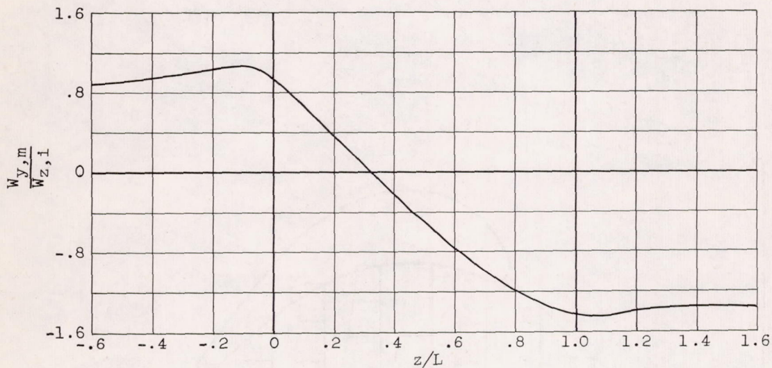
Figure 12. - Variation of tangential velocity on mean streamline with respect to axis for incompressible solution.
