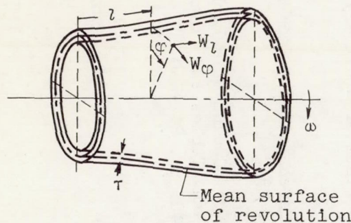
(a) Stream filament of revolution.
