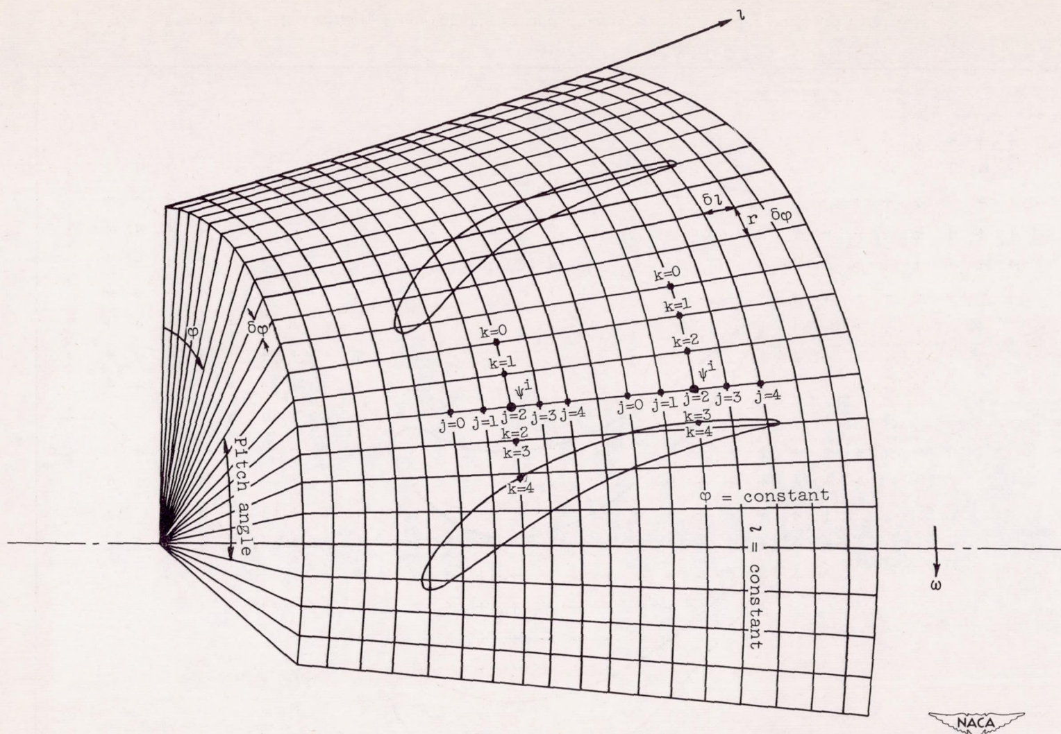
Figure 2. - Values of j and k for two grid points near boundary using five-point system.
