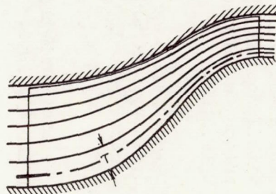
(b) Mean stream surface of revolution.
