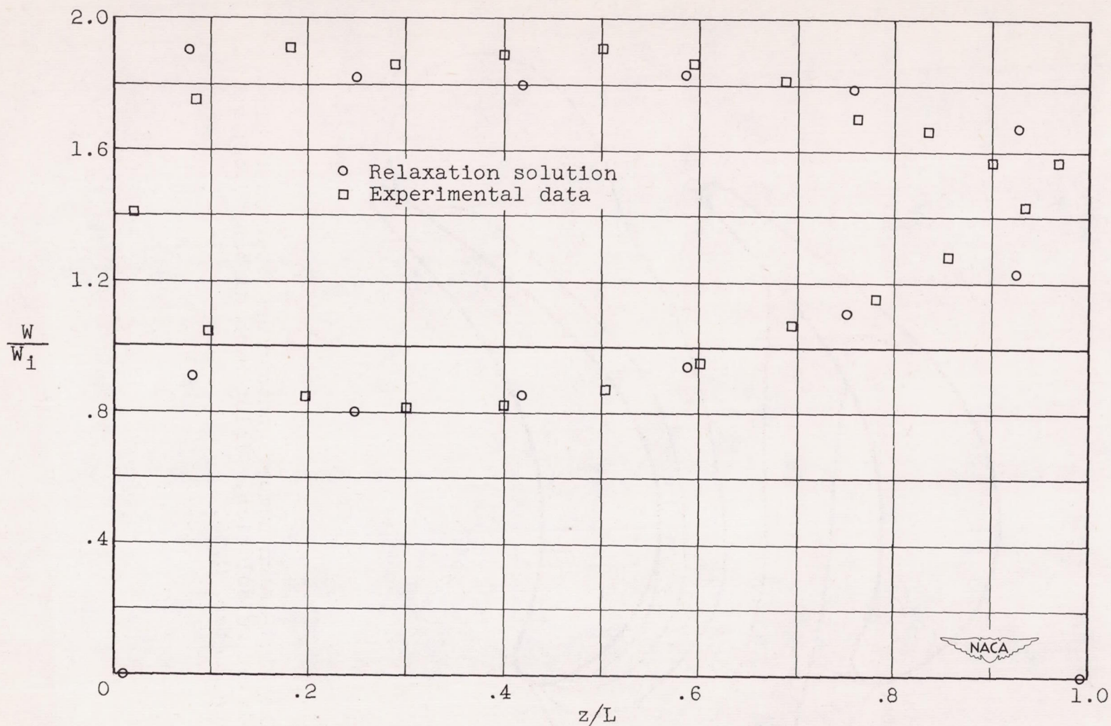
Figure 22. - Comparison of velocity distribution on blade obtained in numerical solution with experimental data. Inlet Mach number, 0.42.
