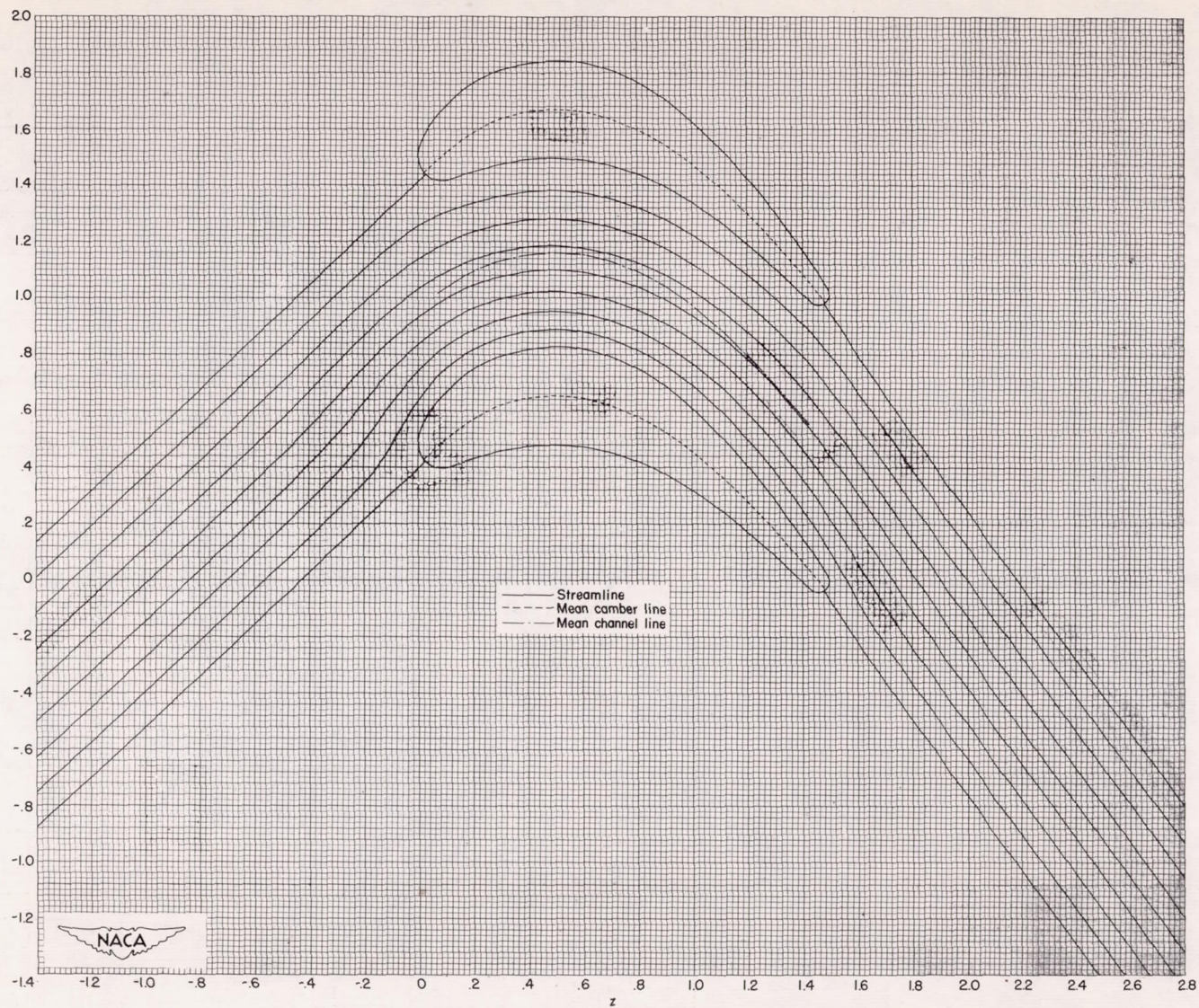
Figure 8. - Streamlines obtained in incompressible solution.
