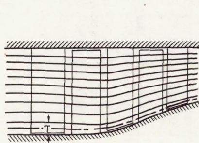
(a) Stream filament of revolution.
