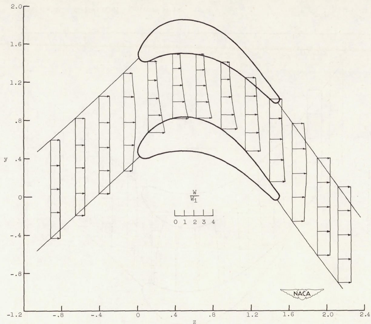
Figure 7. - Variation of magnitude of resultant velocity across channel for incompressible solution.
