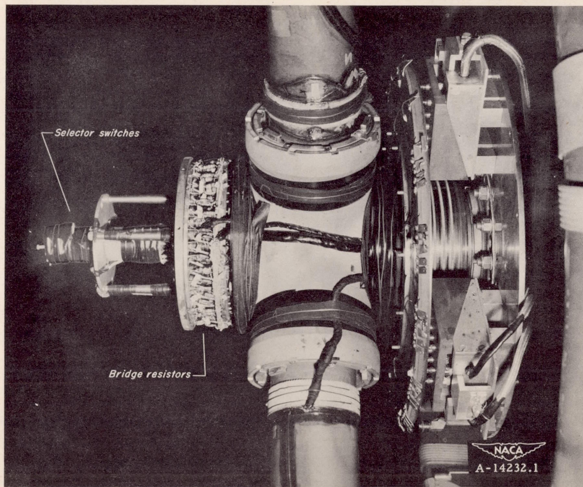
(c) Gage selector switches, bridge resistors, slip rings, and brush assemblies.
