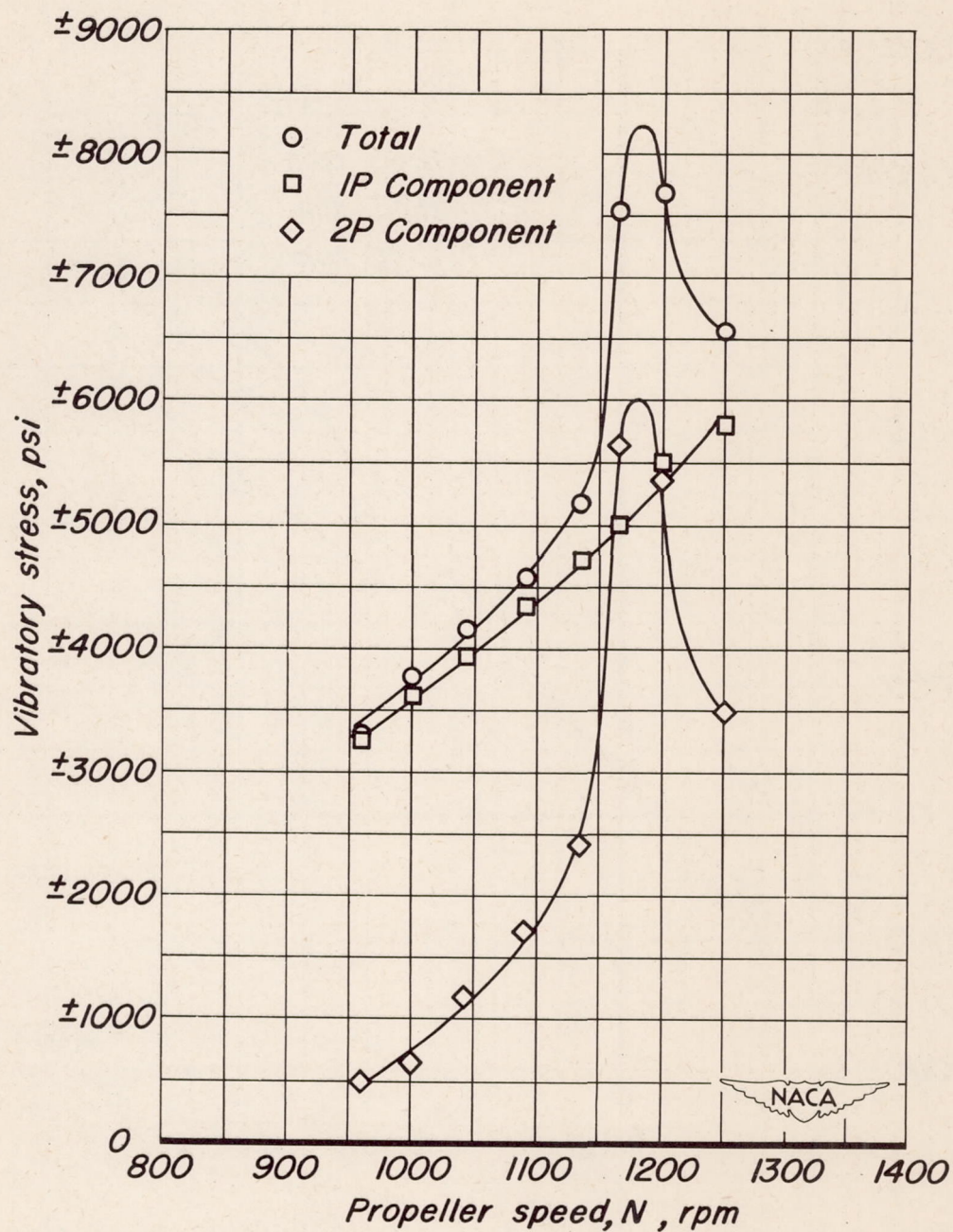
Figure 11. - Vibratory stress measured at shank (11-inch station) V_0 , 165 mph; \alpha_6 , 8^\circ ; \beta_{.75R} , 20^\circ ; four-blade propeller.
