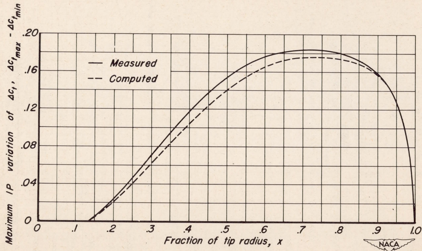
Figure 9. - Comparison of the computed and measured distributions of the maximum variations of the first-order (IP) incremental section thrust coefficient. V_0 , 165 mph; N , 1250 rpm; \alpha_6 , 8^\circ ; \beta_{.75R} , 20^\circ ; four-blade propeller.
