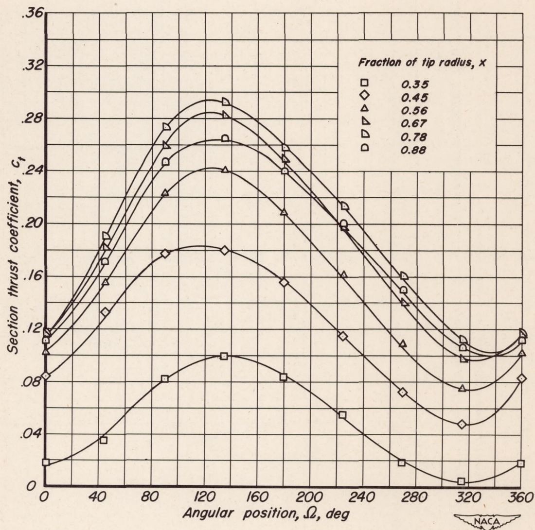
Figure 7.- Measured variation of the section thrust coefficient c_t with angular position \Omega . V_0 , 165 mph; \alpha_0 , 8^\circ ; N , 1250 rpm; \beta , 75^\circ ; R , 20^\circ ; four-blade propeller.
