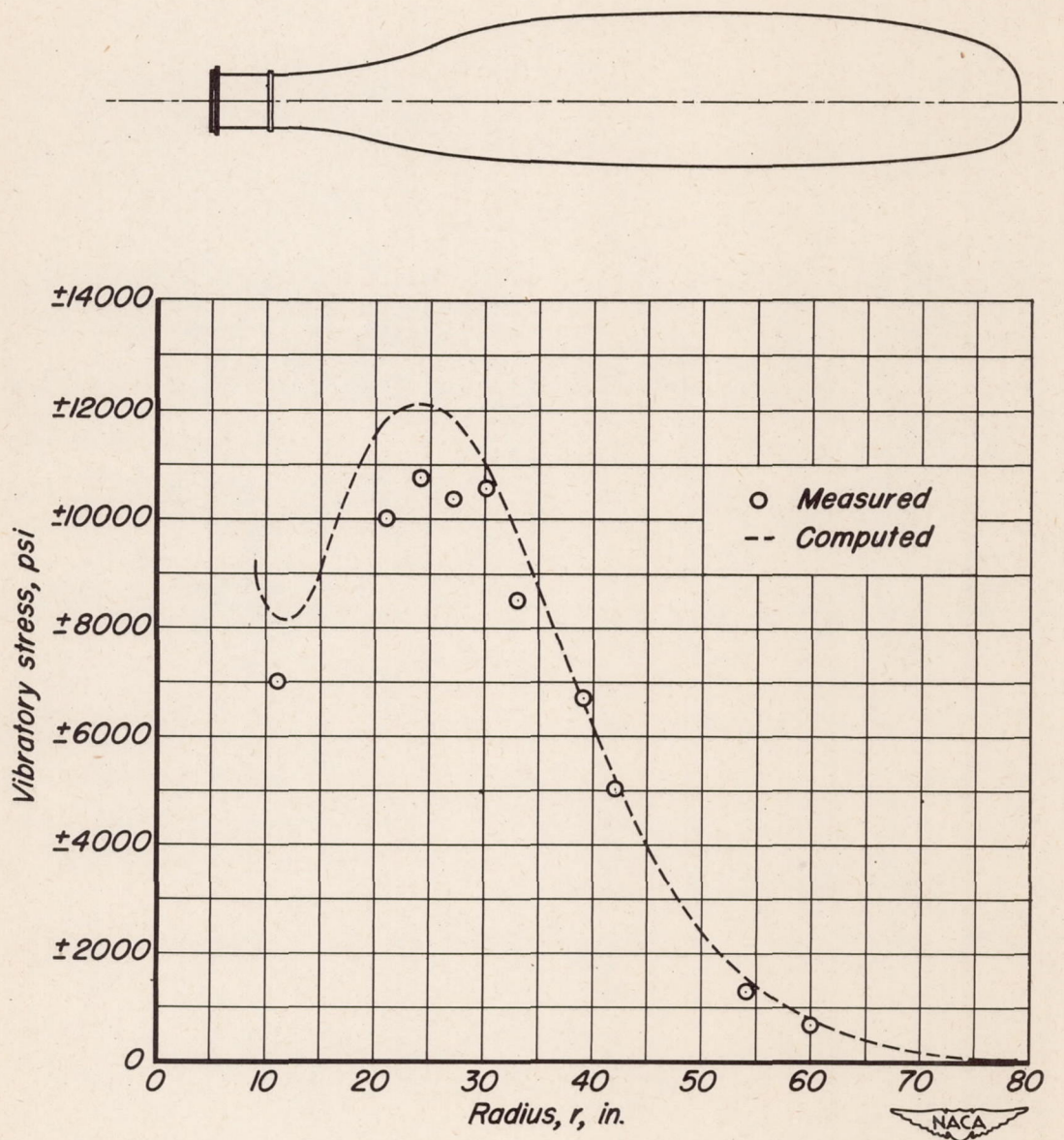
Figure 15. - Comparison of the computed and measured stress distributions for the three-blade propeller. V_0 , 165 mph; N , 1250 rpm; \alpha_6 , 8^\circ ; \beta_{.75R} , 20^\circ .
