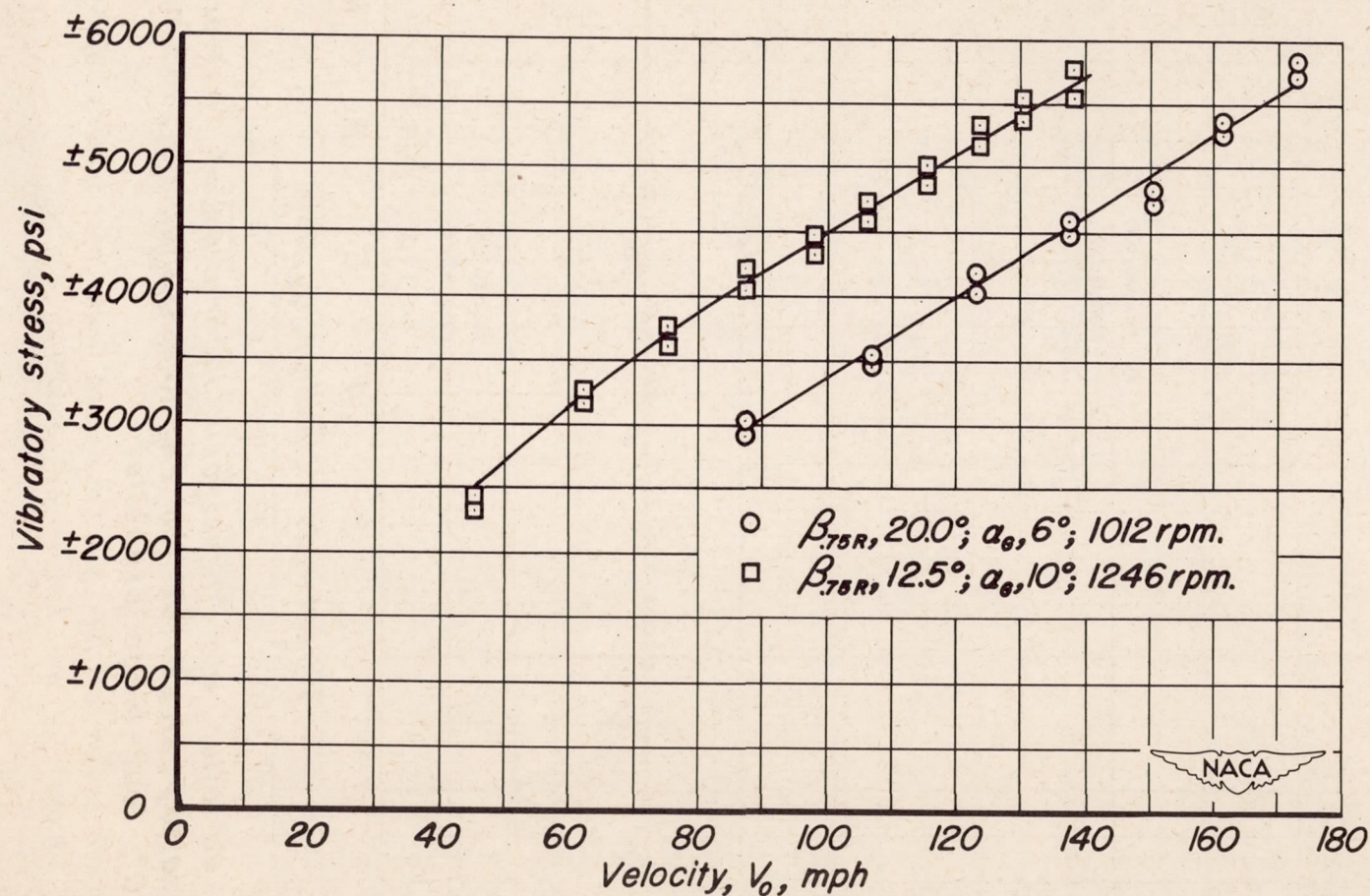
Figure 13.- Variation with stream velocity of first-order (IP) vibratory stress at the 24-inch station. Four-blade propeller.
