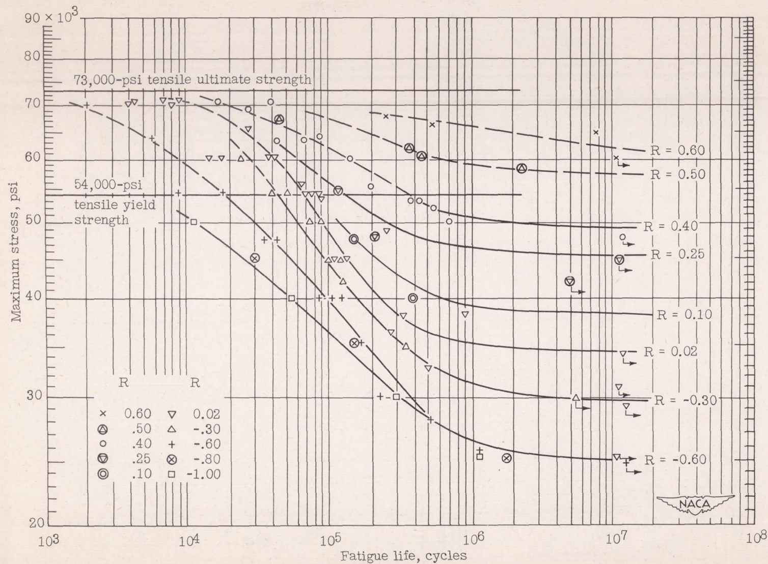
Figure 8.- Results of fatigue tests at 1100 cycles per minute on 24S-T3 aluminum alloy.
