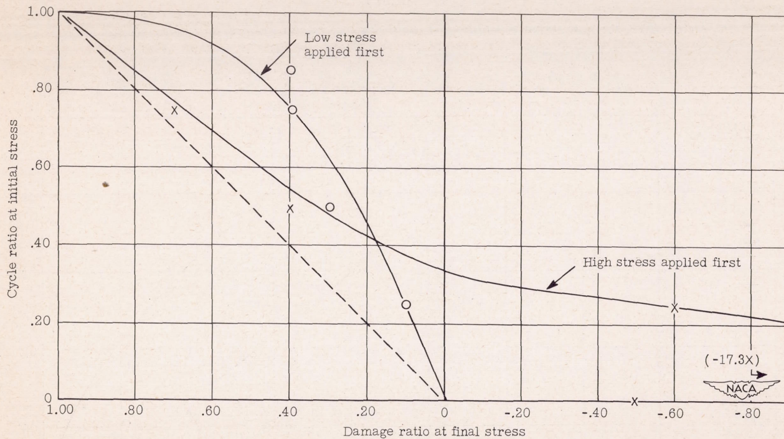
Figure 16.- Results of fatigue loading 75S-T6 aluminum sheet specimens at two stress levels. High stress, 65,000-psi maximum; low stress, 45,000-psi maximum; for both, mean stress, 20,625 psi.
