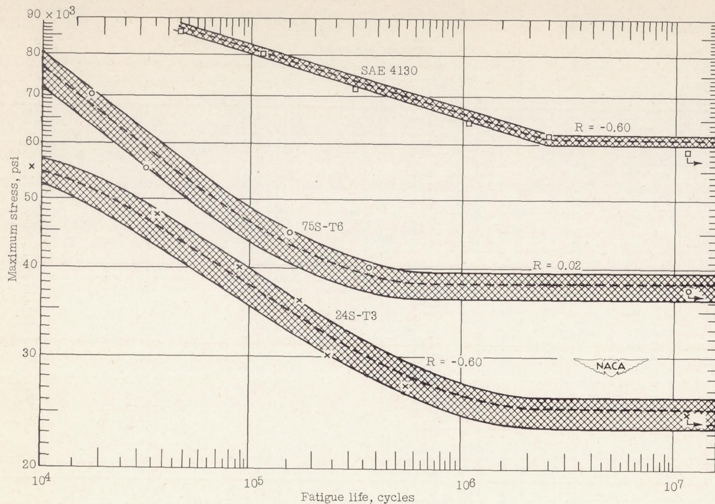
Figure 11.- Representative scatter bands. Dashed lines correspond to solid lines in figures 8, 9, and 10. The ratio shown for 75S-T6 is R = 0.02 to avoid confusion with the scatter bands at R = -0.60 for 24S-T3 and 4130.
