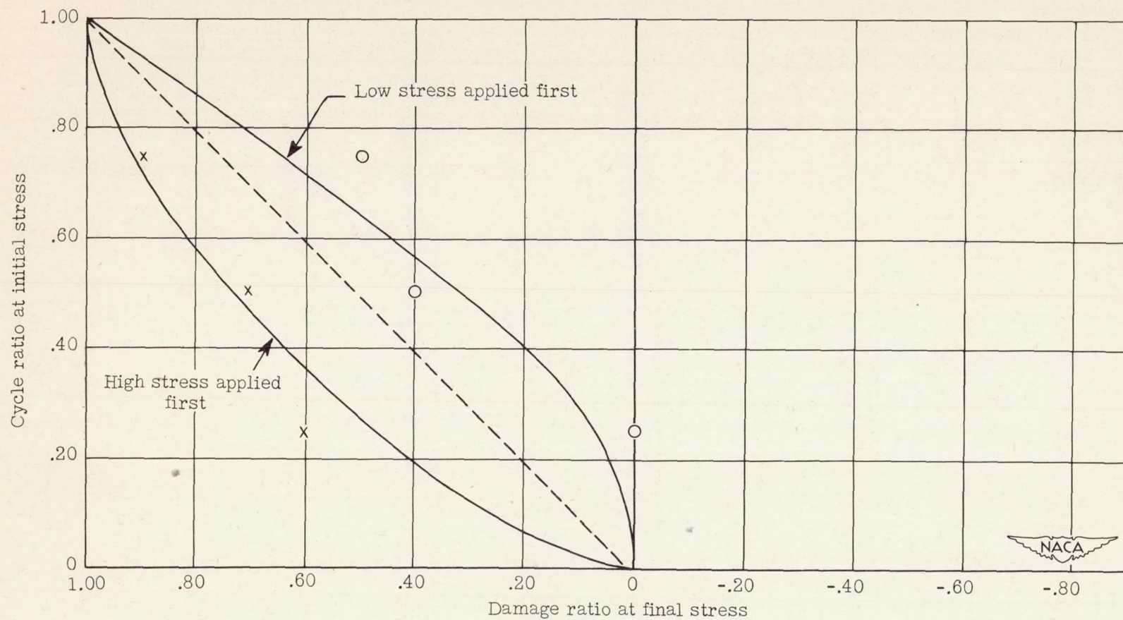
Figure 17.- Results of fatigue loading SAE 4130 steel sheet specimens at two stress levels. High stress, 95,000-psi maximum; low stress, 82,500-psi maximum; for both, mean stress, 29,250 psi.
