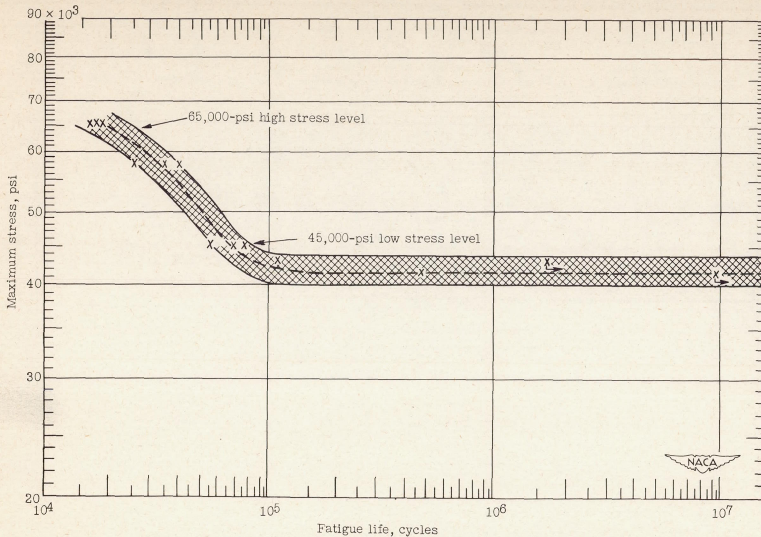
Figure 13.- S-N base-line curve for damage tests on 75S-T6 aluminum. Mean stress constant at 20,625 psi (one-fourth of ultimate strength).
