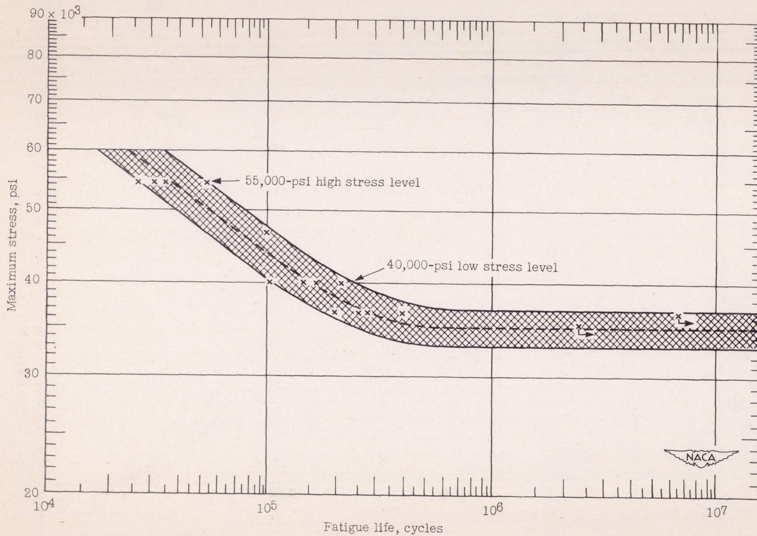
Figure 12.- S-N base-line curve for damage tests on 24S-T3 aluminum. Mean stress constant at 18,250 psi (one-fourth of ultimate strength).
