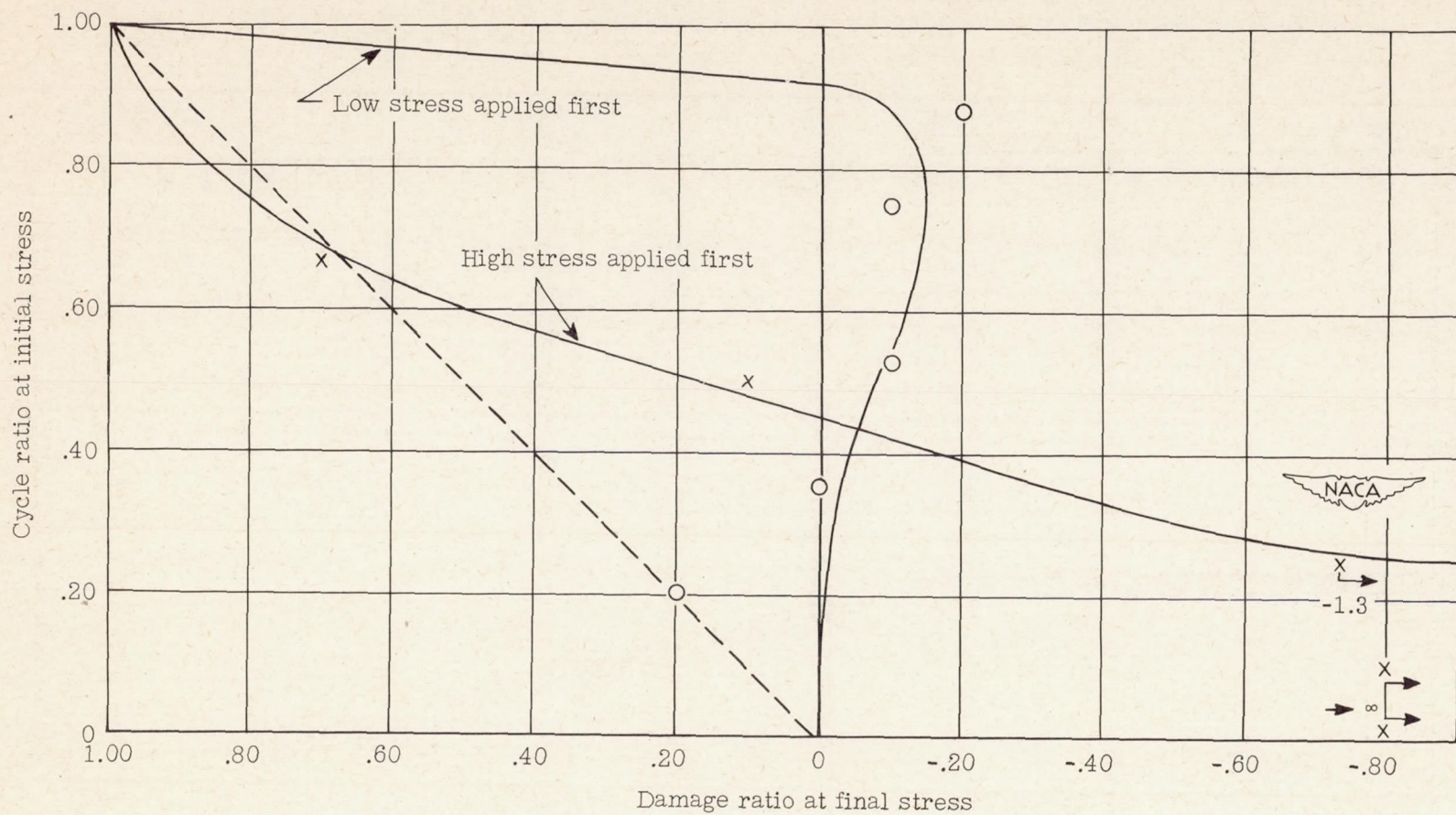
Figure 15.- Results of fatigue loading 24S-T3 aluminum sheet specimens at two stress levels. High stress, 55,000-psi maximum; low stress, 40,000-psi maximum; for both, mean stress, 18,250 psi.
