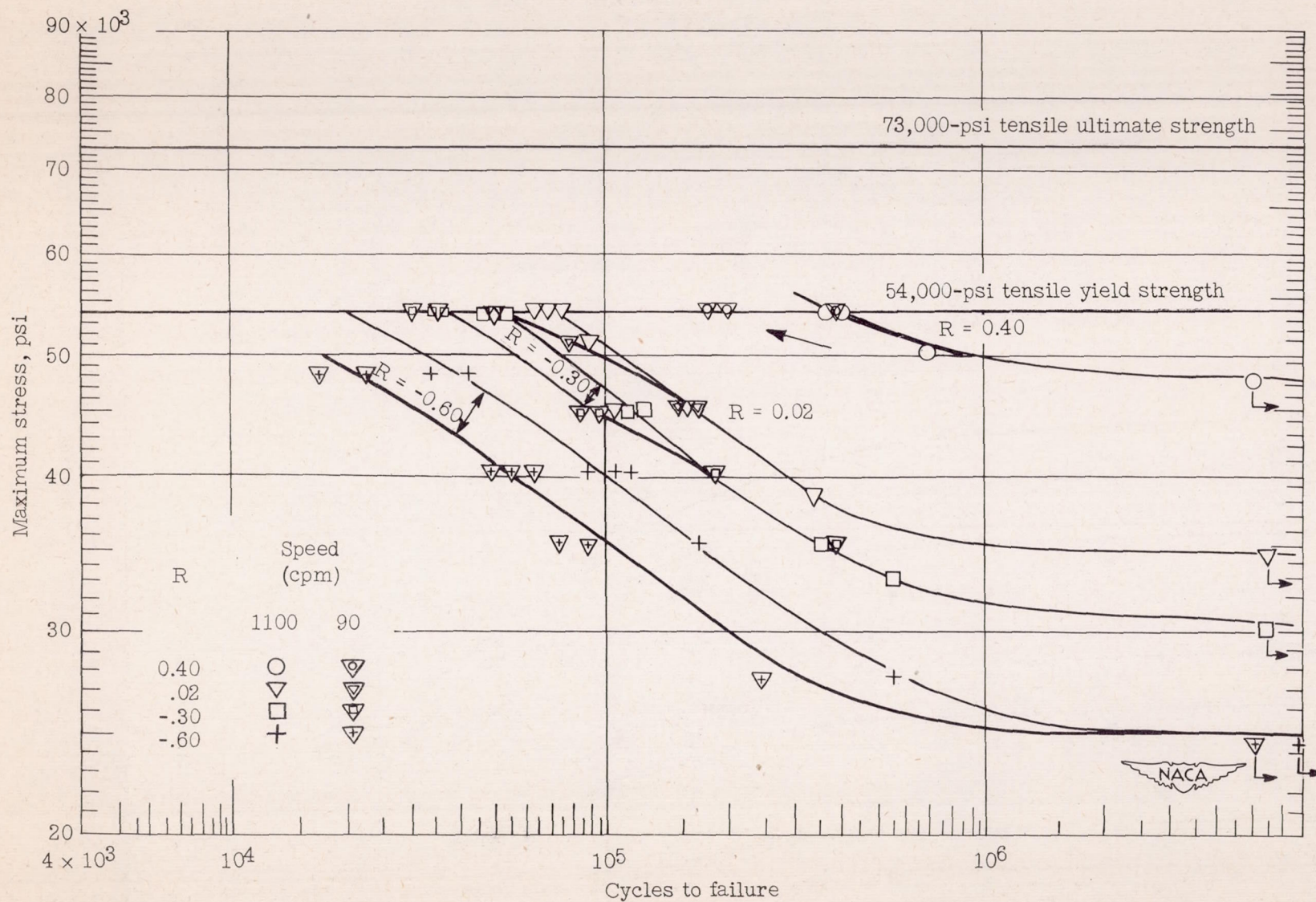
Figure 18.- Results of fatigue tests, at different speeds, on unnotched 24S-T3 aluminum alloy.
