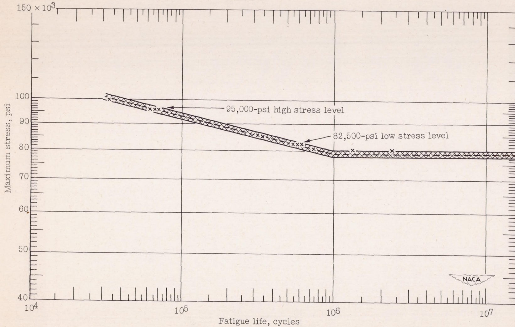
Figure 14.- S-N base-line curve for damage tests on SAE 4130 steel. Mean stress constant at 29,250 psi (one-fourth of ultimate strength).
