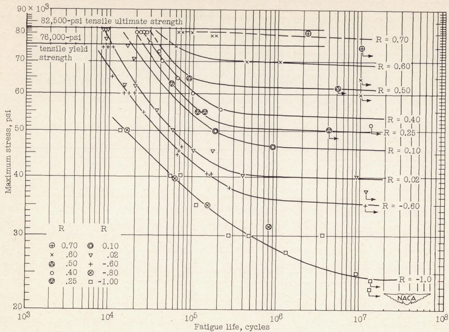
Figure 9.- Results of fatigue tests at 1100 cycles per minute on 75S-T6 aluminum alloy.
