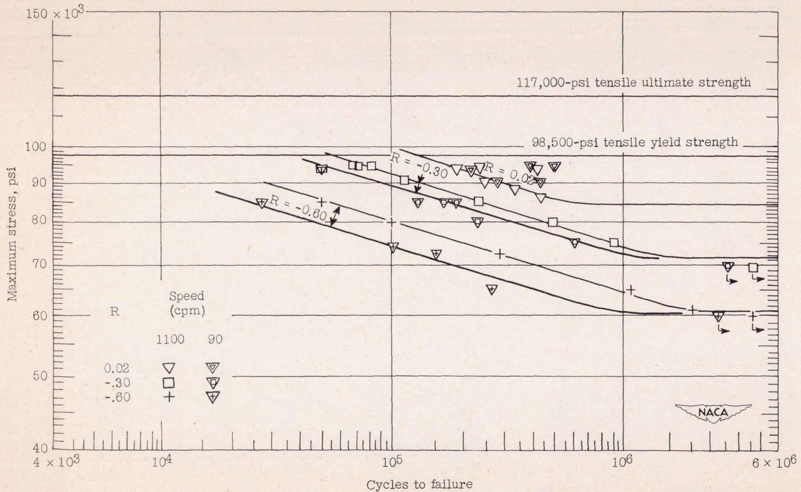
Figure 20.- Results of fatigue tests, at different speeds, on normalized unnotched SAE 4130 steel.
