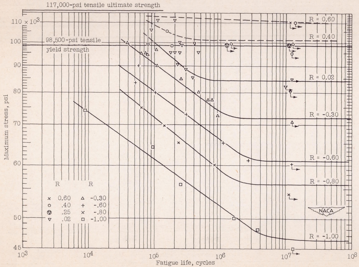
Figure 10.- Results of fatigue tests at 1100 cycles per minute on normalized SAE 4130 steel.
