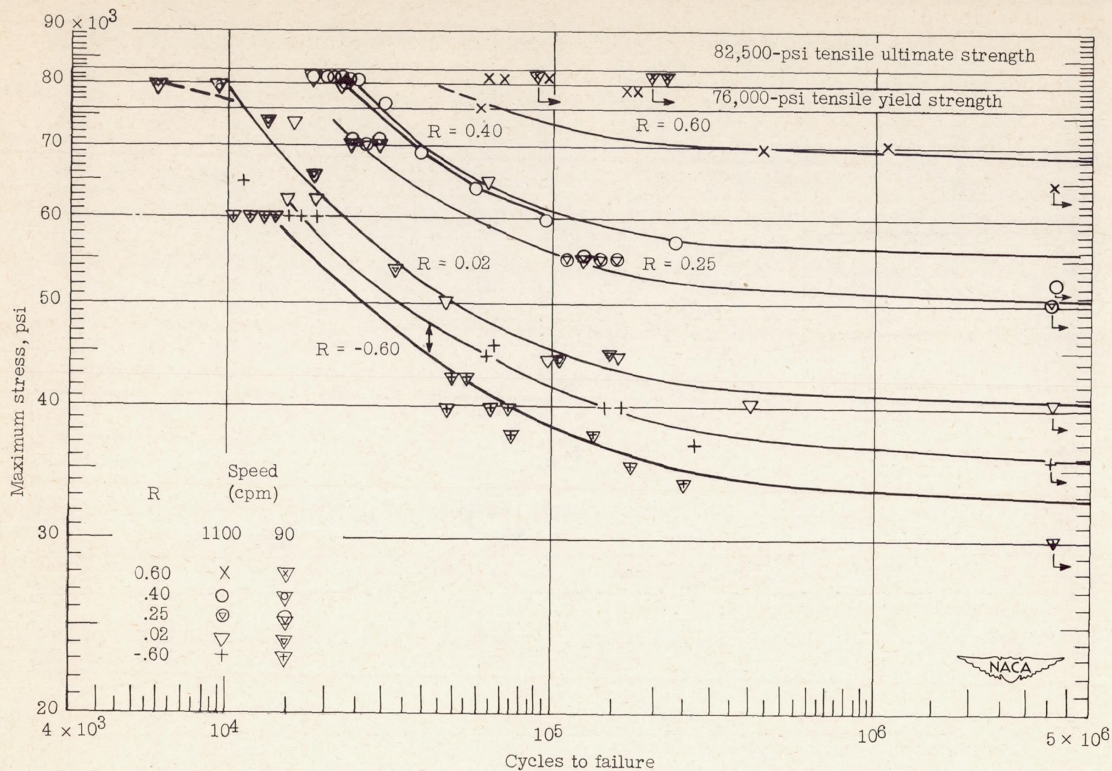
Figure 19.- Results of fatigue tests, at different speeds, on unnotched 75S-T6 aluminum alloy.
