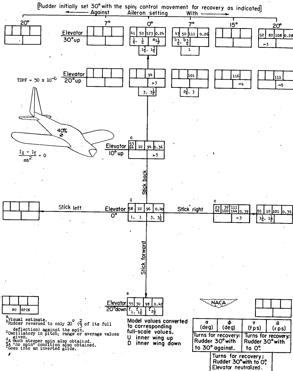
CHART 28.- SPIN AND RECOVERY CHARACTERISTICS OF MODEL FOR TEST CONDITION 28 LISTED IN TABLE III
