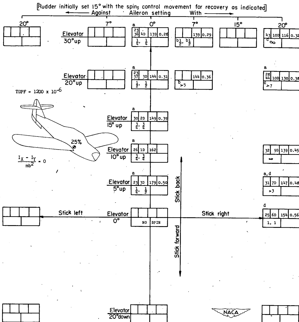
CHART 6.-SPIN AND RECOVERY CHARACTERISTICS OF MODEL FOR TEST CONDITION 6 LISTED IN TABLE III
