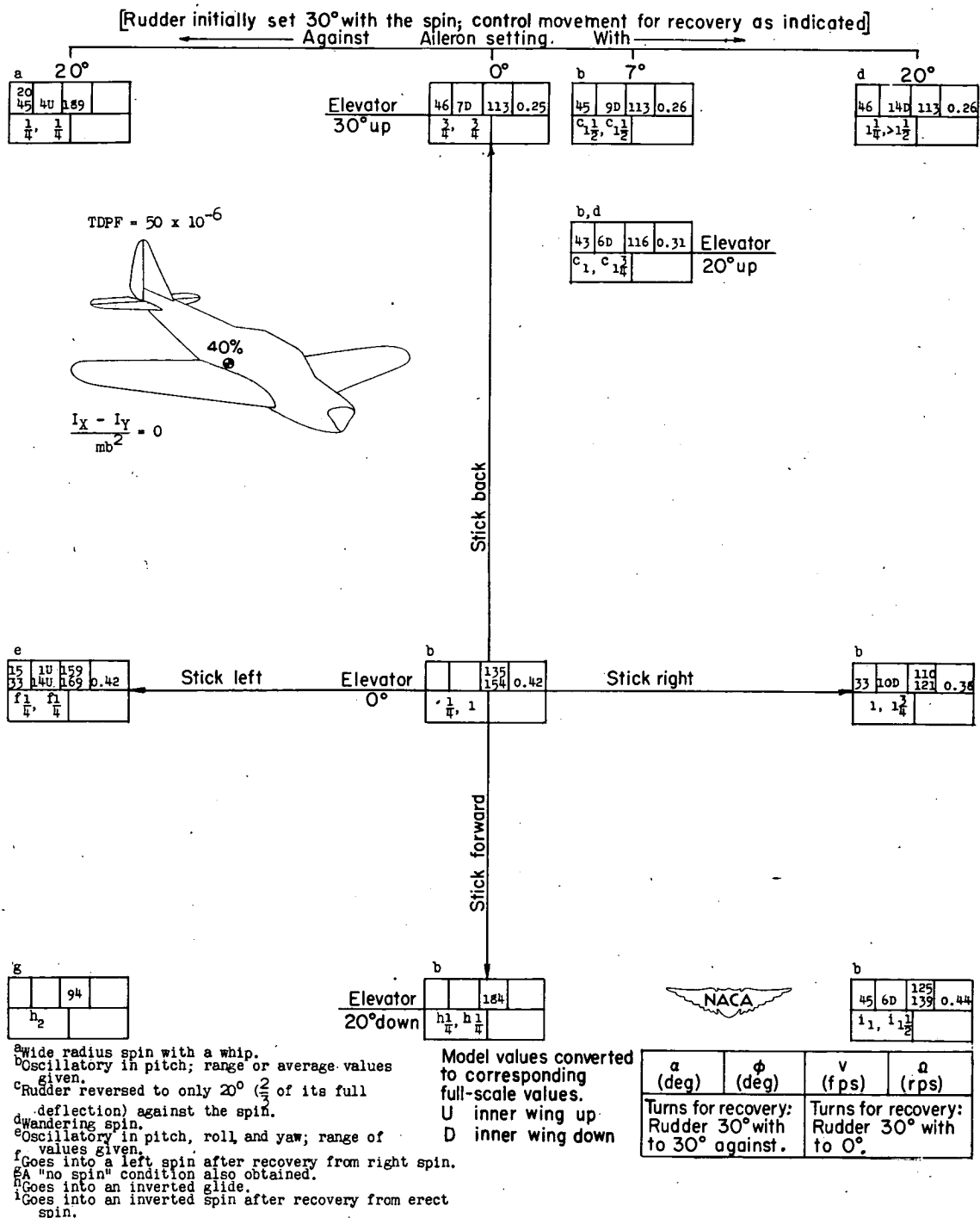
CHART 65.-SPIN AND RECOVERY CHARACTERISTICS OF MODEL FOR TEST CONDITION 66 LISTED IN TABLE III
