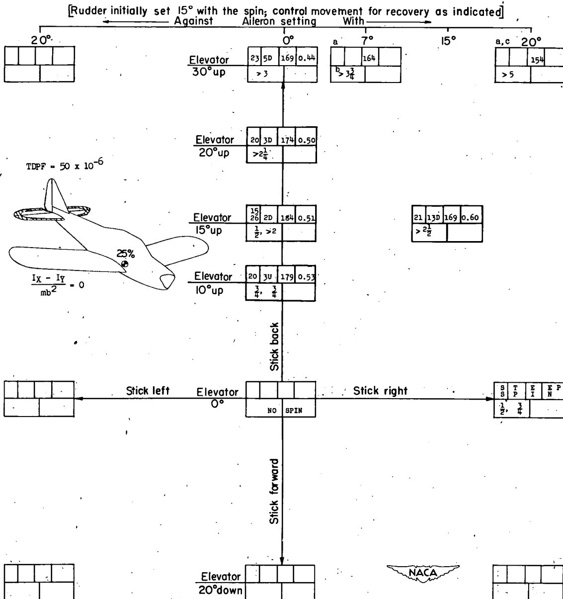
CHART 45.-SPIN AND RECOVERY CHARACTERISTICS OF MODEL FOR TEST CONDITION 45 LISTED IN TABLE III
