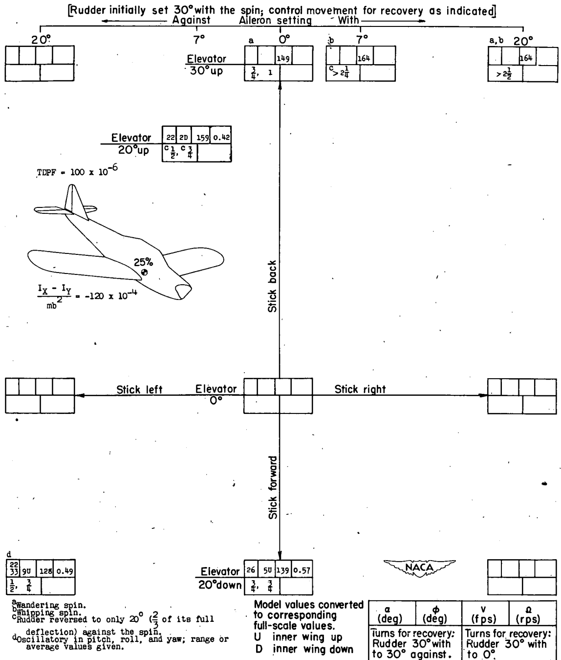
CHART 62.- SPIN AND RECOVERY CHARACTERISTICS OF MODEL FOR TEST CONDITION 62 LISTED IN TABLE III
