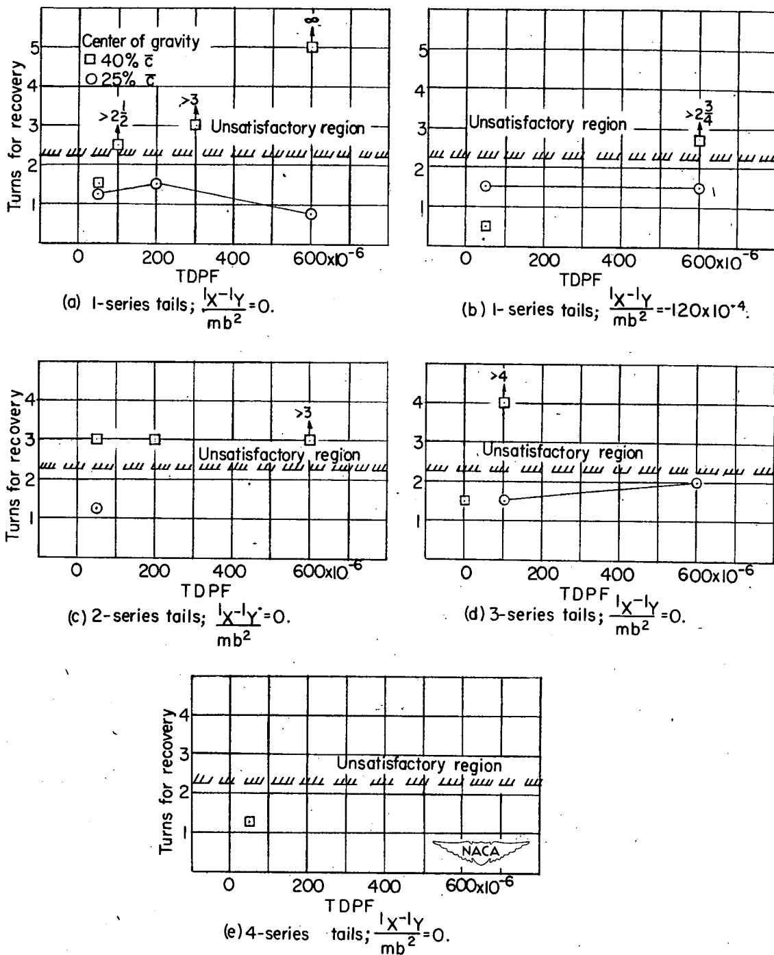
Figure 17.- Effect of tail-damping power factor on turns required for recovery by simultaneous rudder and elevator neutralization. (See table V.)
