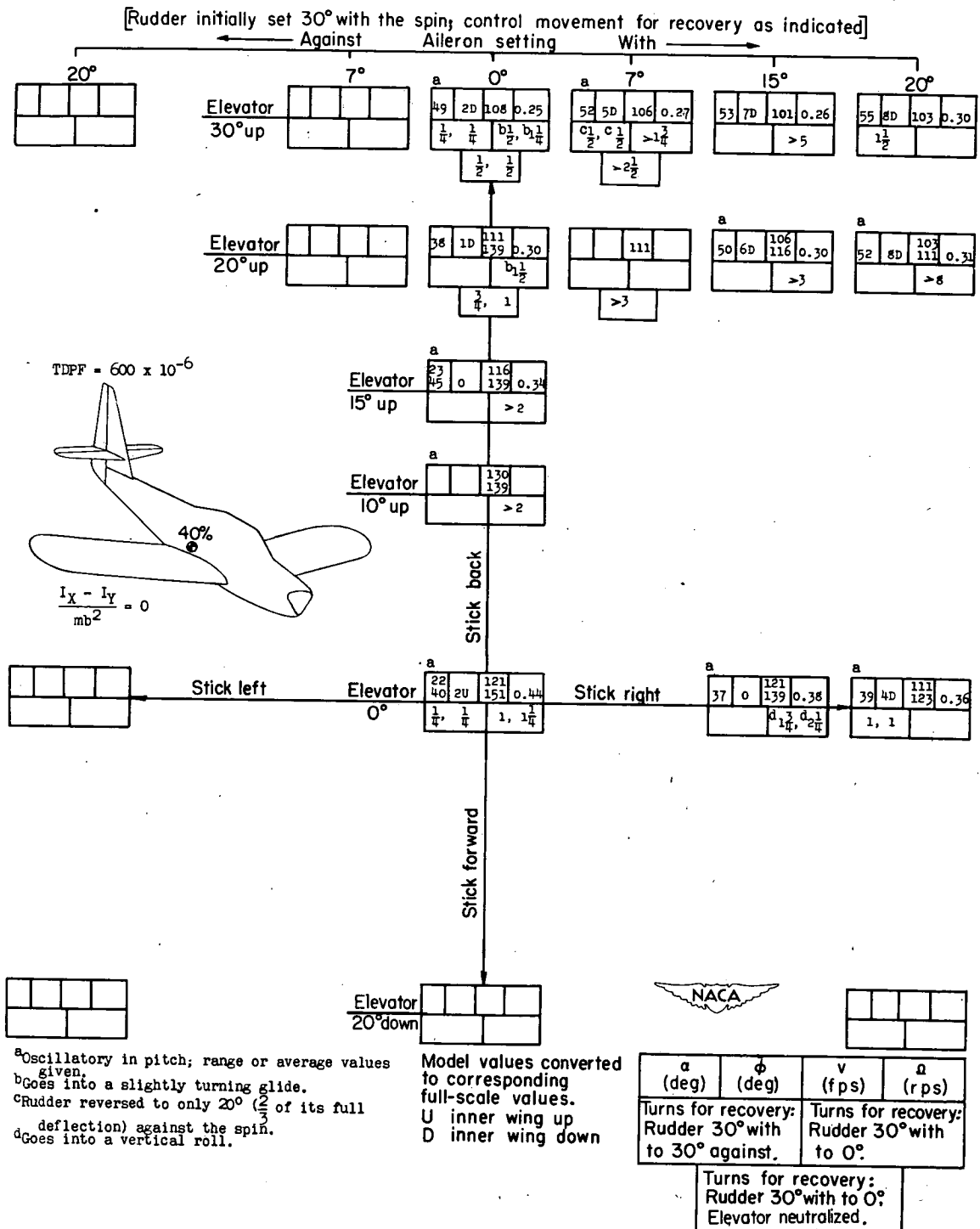
CHART 32.-SPIN AND RECOVERY CHARACTERISTICS OF MODEL FOR TEST CONDITION 32 LISTED IN TABLE III
