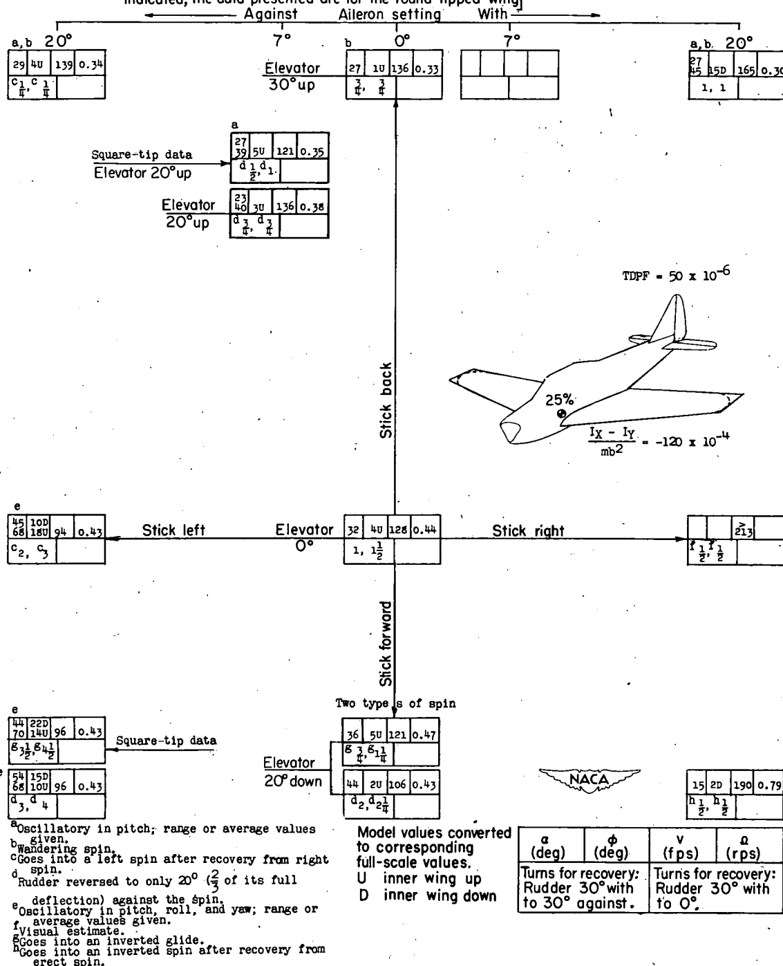
Chart 67:-SPIN AND RECOVERY CHARACTERISTICS OF MODEL FOR TEST CONDITIONS 68 AND 75 LISTED IN TABLE III [Rudder initially set 30° with the spin; control movement for recovery as indicated; unless otherwise indicated, the data presented are for the round-tipped wing]
