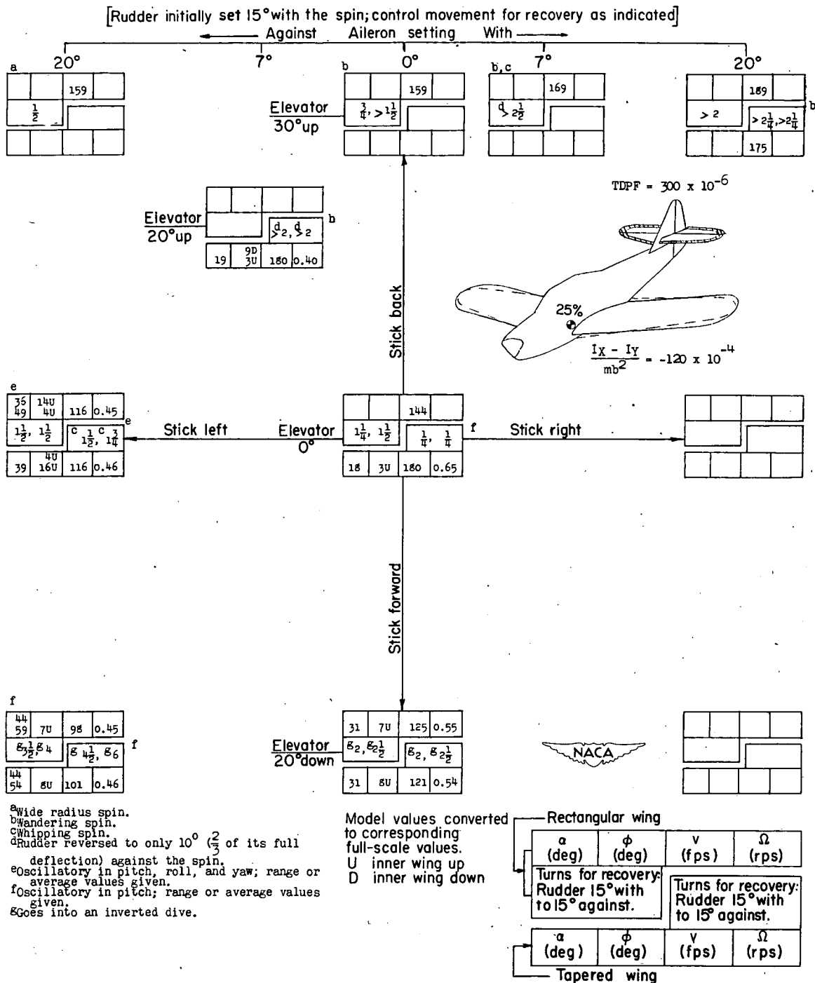
CHART 53.-SPIN AND RECOVERY CHARACTERISTICS OF MODEL FOR TEST CONDITIONS 53 AND 73 LISTED IN TABLE III
