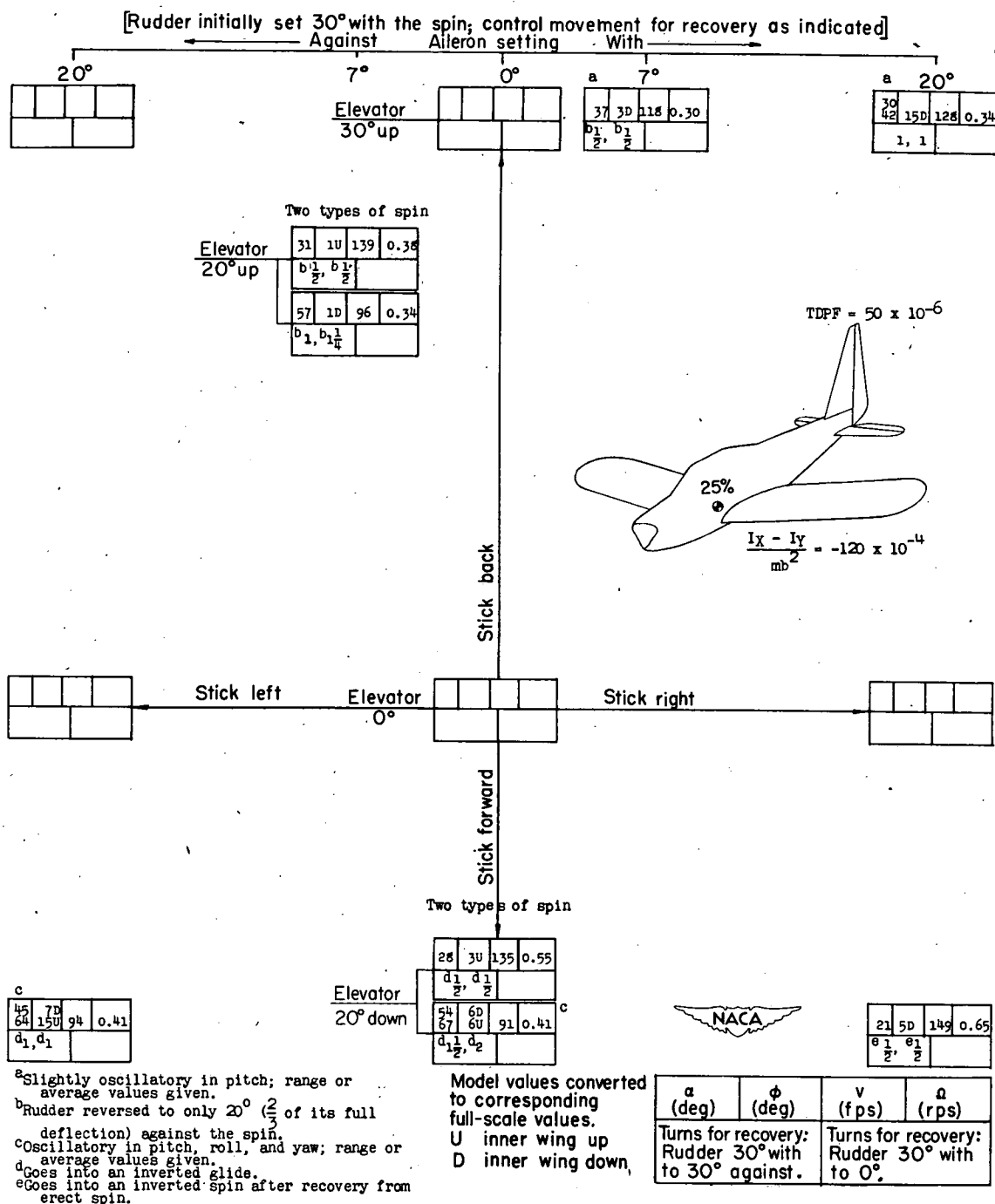
CHART 30.-SPIN AND RECOVERY CHARACTERISTICS OF MODEL FOR TEST CONDITION 30 LISTED IN TABLE III
