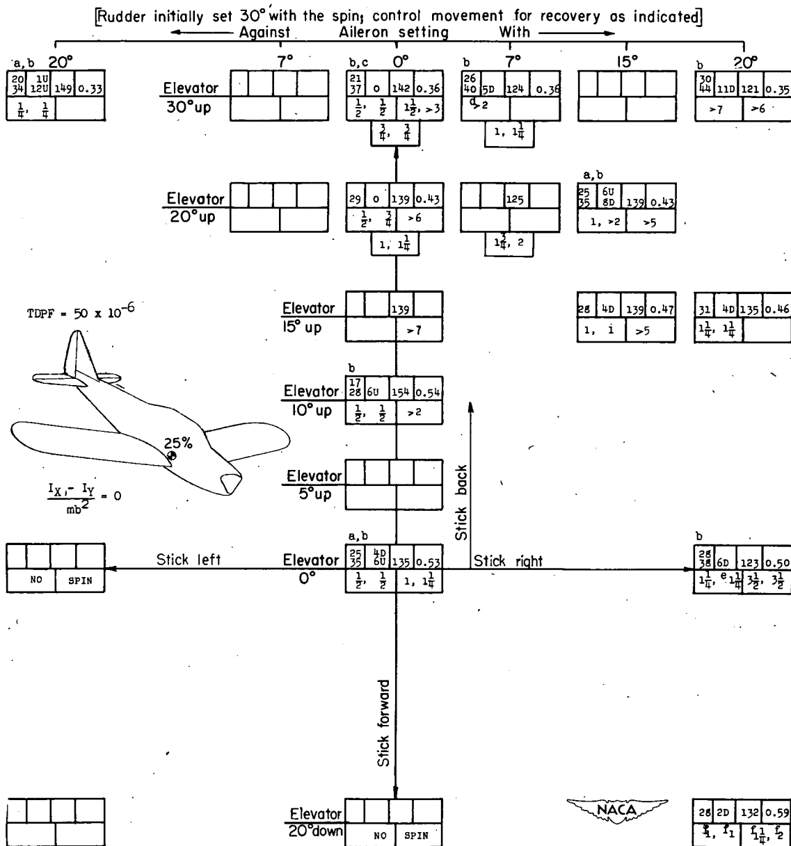
CHART 1.- SPIN AND RECOVERY CHARACTERISTICS OF MODEL FOR TEST CONDITION 1 LISTED IN TABLE III
