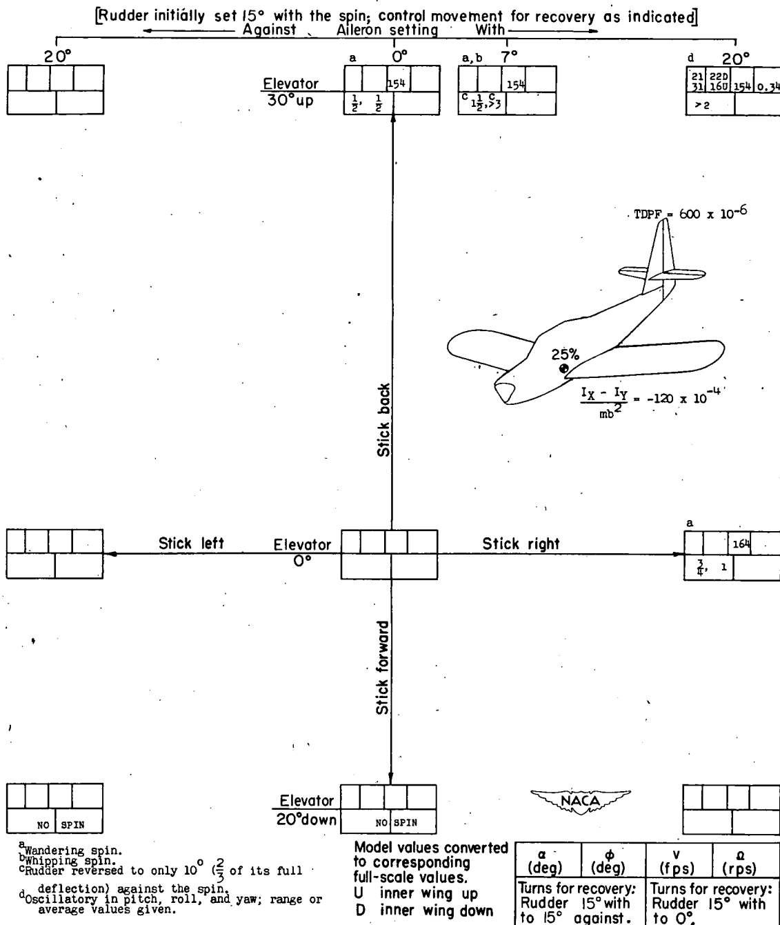
CHART 35.-SPIN AND RECOVERY CHARACTERISTICS OF MODEL FOR TEST CONDITION 35 LISTED IN TABLE III
