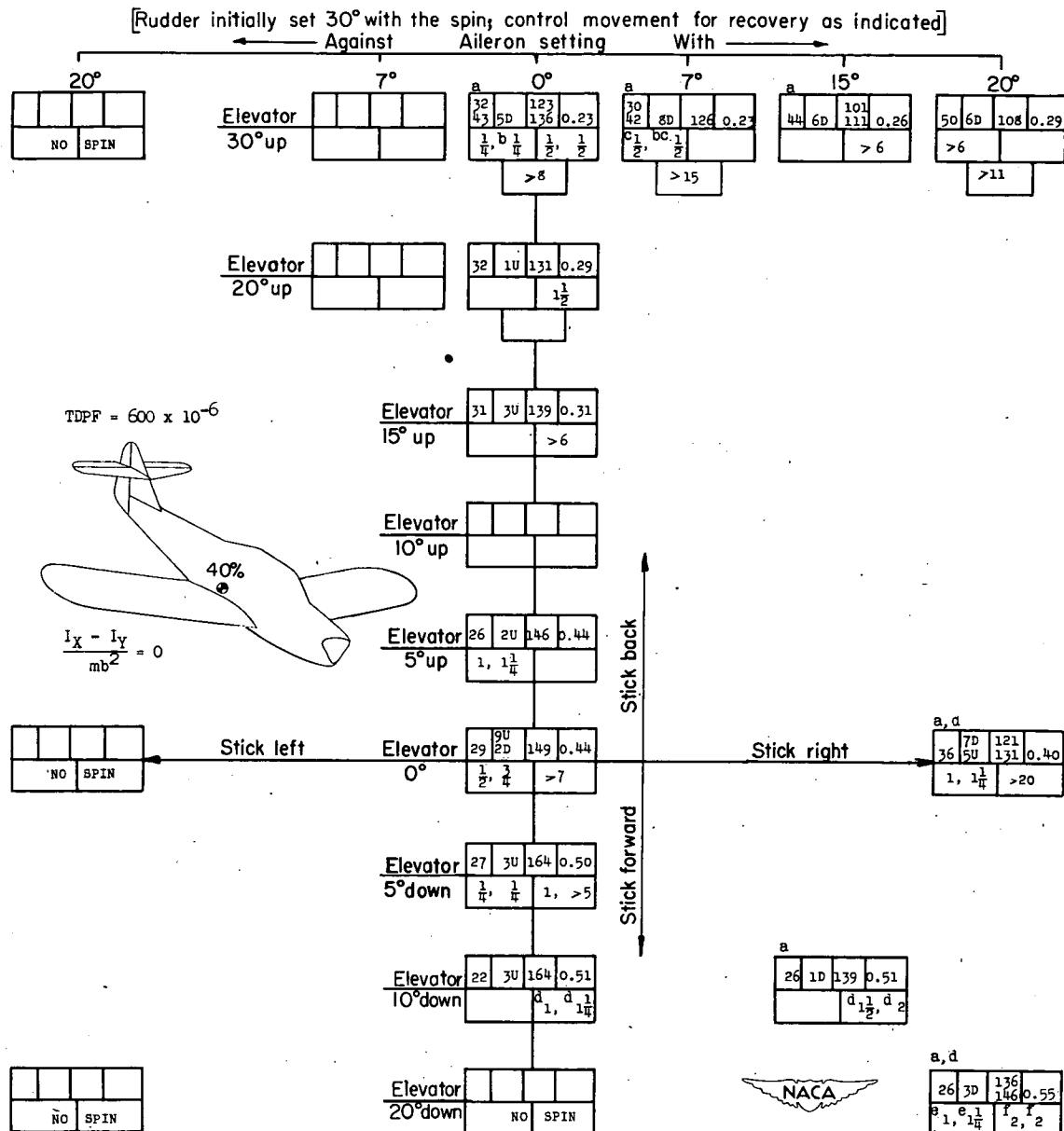
CHART 19: SPIN AND RECOVERY CHARACTERISTICS OF MODEL FOR TEST CONDITION 19 LISTED IN TABLE III
