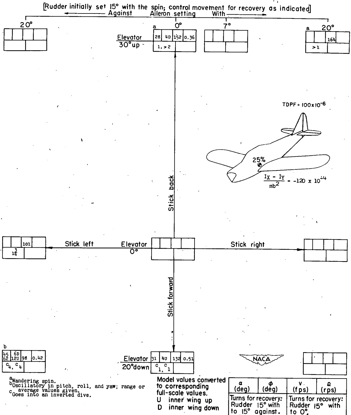
CHART 10.-SPIN AND RECOVERY CHARACTERISTICS OF MODEL FOR TEST CONDITION 10 LISTED IN TABLE III
