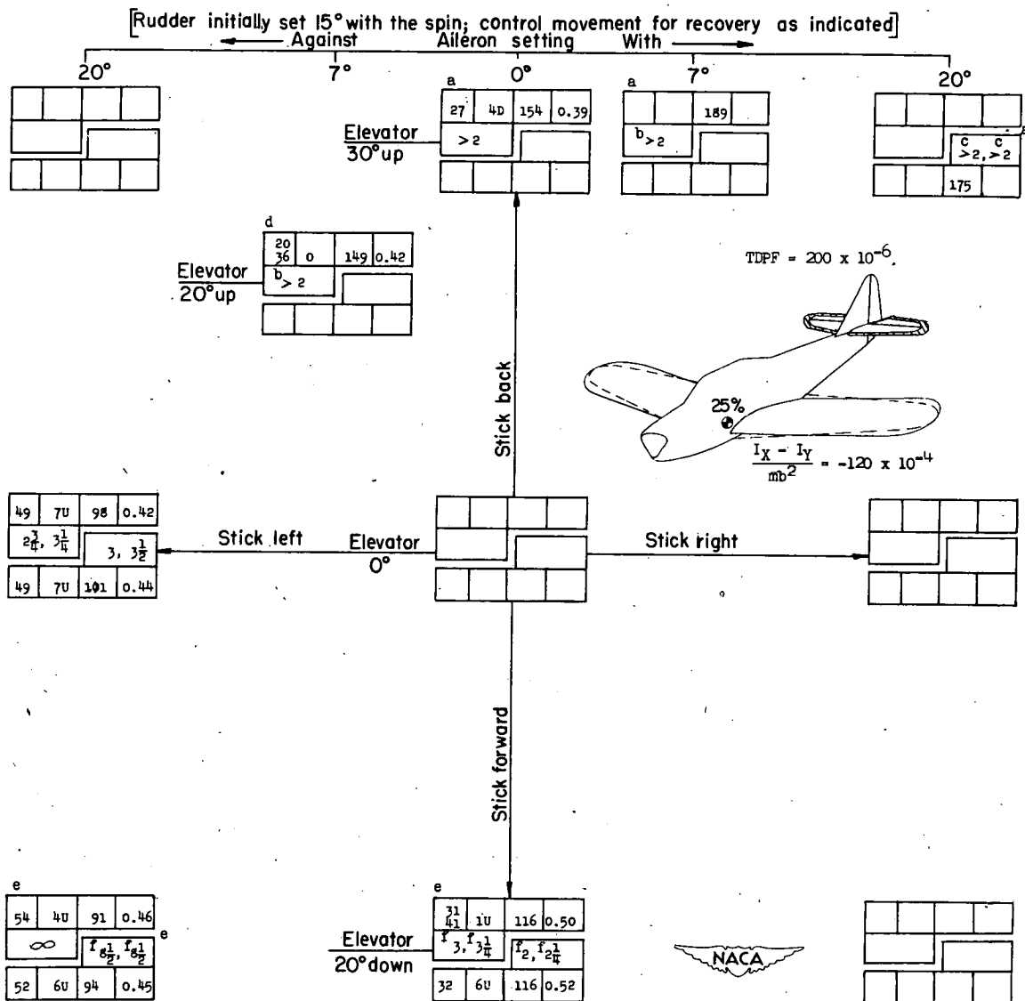
CHART 51.-SPIN AND RECOVERY CHARACTERISTICS OF MODEL FOR TEST CONDITIONS 51 AND 71 LISTED IN TABLE III
