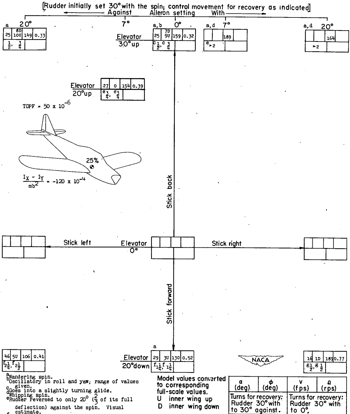
CHART 38.-SPIN AND RECOVERY CHARACTERISTICS OF MODEL FOR TEST CONDITION 38 LISTED IN TABLE III
