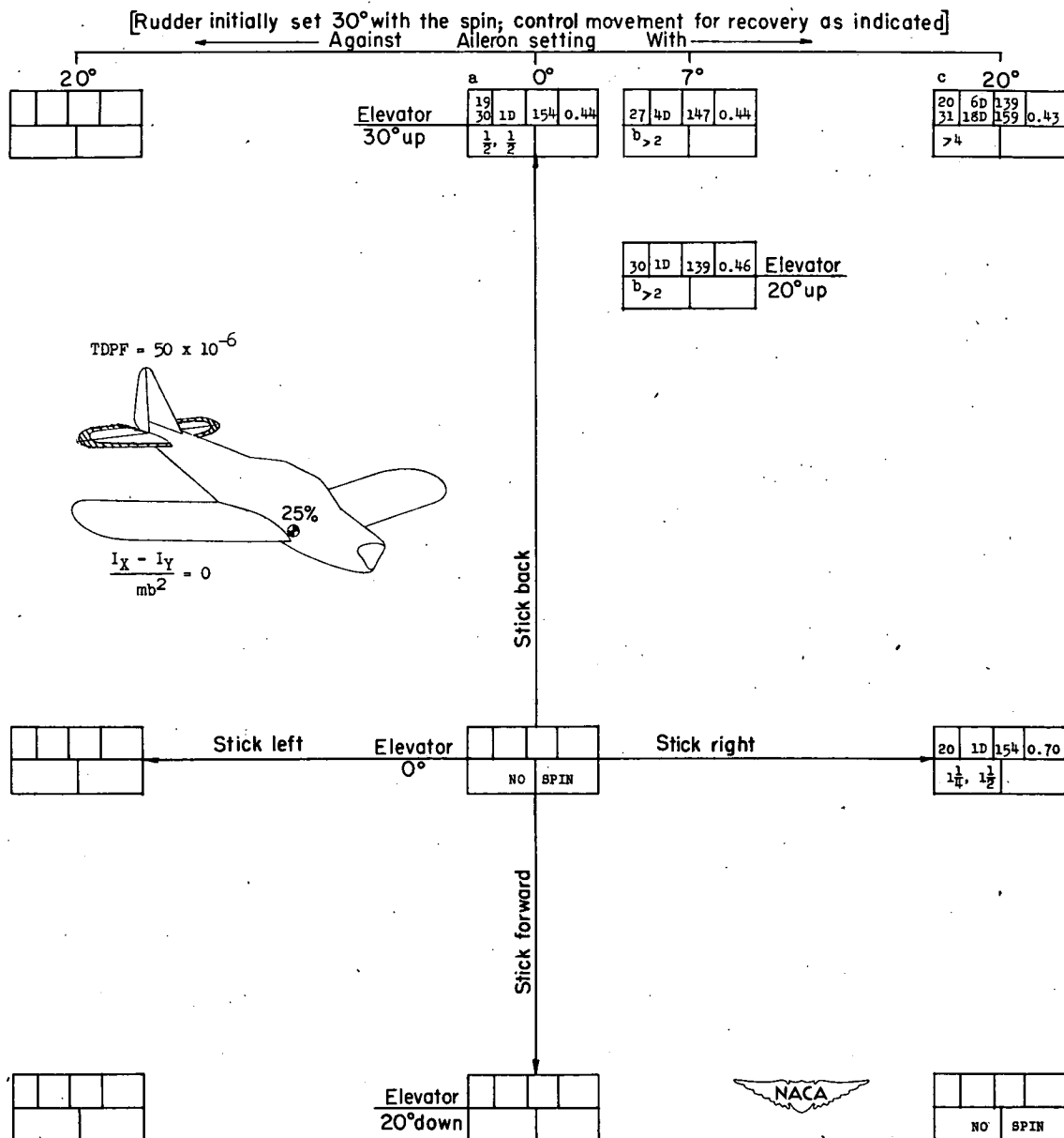
CHART 44.-SPIN AND RECOVERY CHARACTERISTICS OF MODEL FOR TEST CONDITION 44 LISTED IN TABLE III
