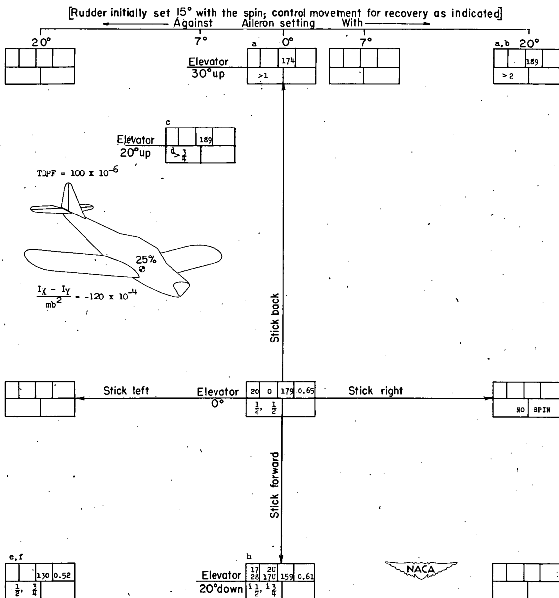
CHART 63--SPIN AND RECOVERY CHARACTERISTICS OF MODEL FOR TEST CONDITION 63 LISTED IN TABLE III
