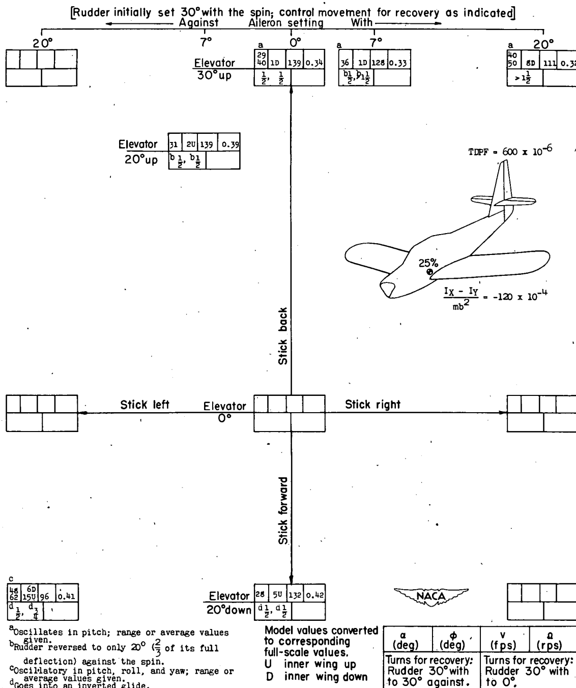
CHART 34.-SPIN AND RECOVERY CHARACTERISTICS OF MODEL FOR TEST CONDITION 34 LISTED IN TABLE III
