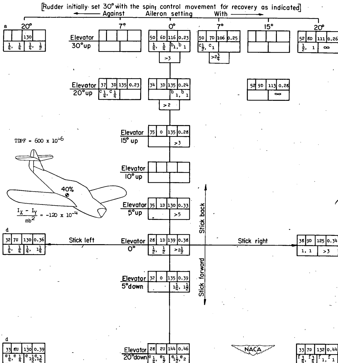
CHART 24.- SPIN AND RECOVERY CHARACTERISTICS OF MODEL FOR TEST CONDITION 24 LISTED IN TABLE III
