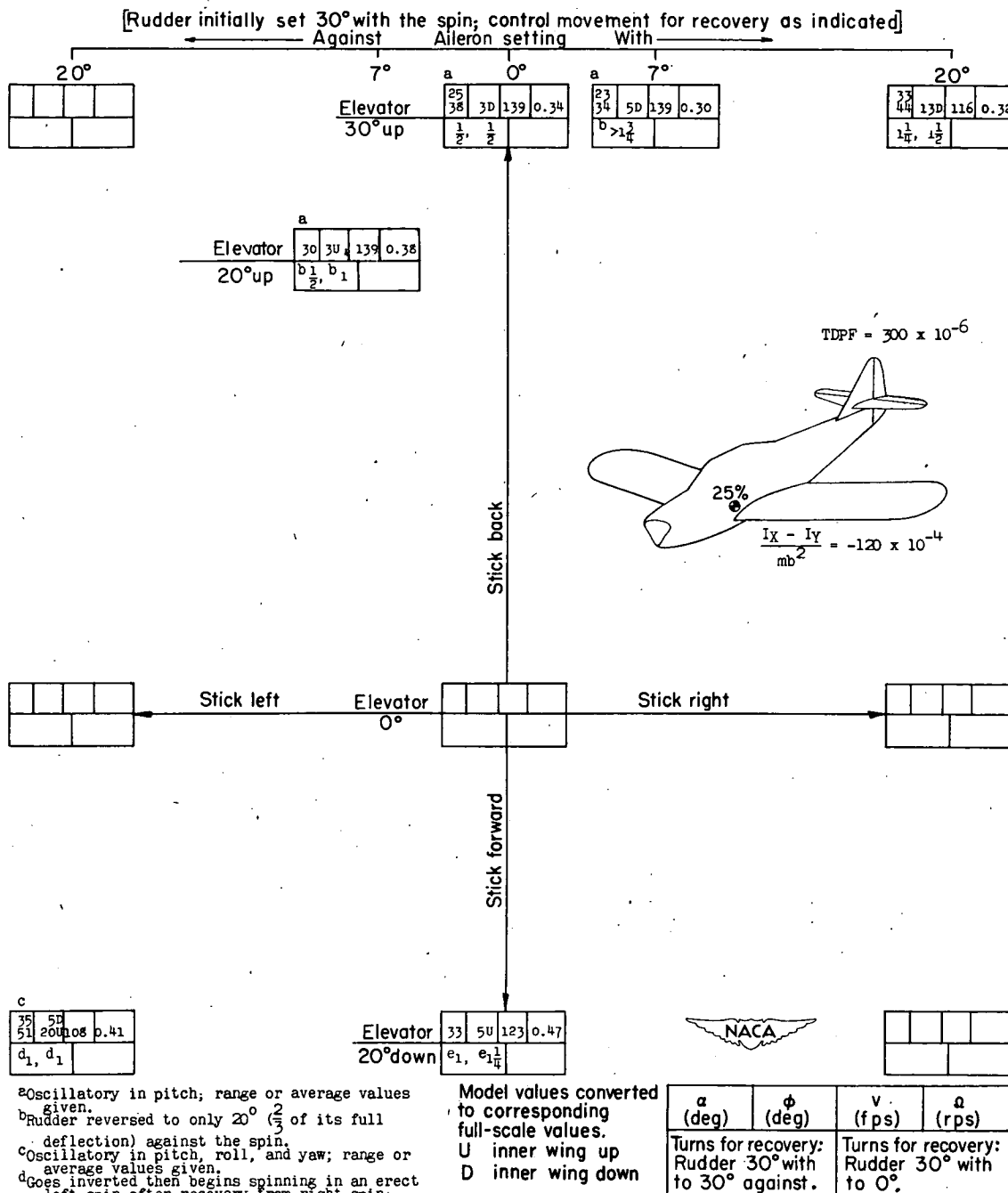
CHART 13.-SPIN AND RECOVERY CHARACTERISTICS OF MODEL FOR TEST CONDITION 13 LISTED IN TABLE III
