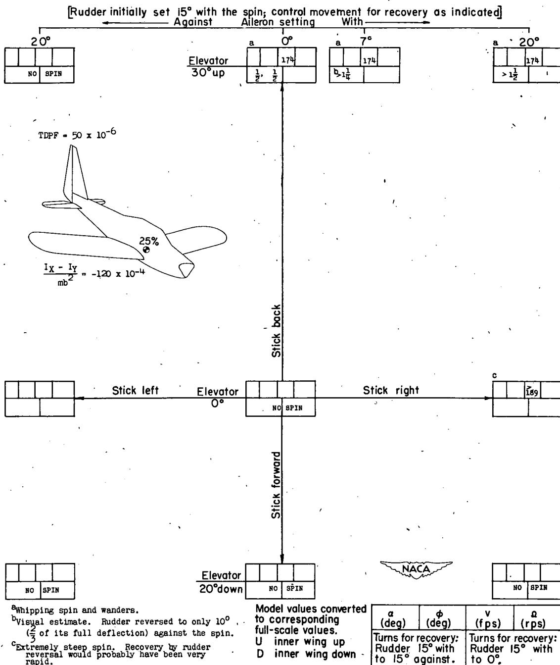
CHART 31.- SPIN AND RECOVERY CHARACTERISTICS OF MODEL FOR TEST CONDITION 31 LISTED IN TABLE III
