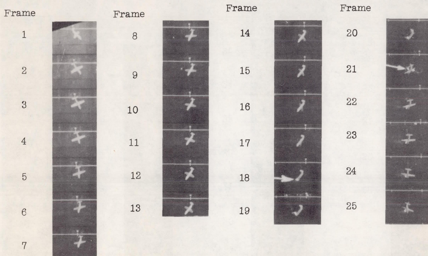
Figure 6.- Moving-picture strips of pilot release from outboard side. Model 20; right spin. (Arrows indicate pilot.)
