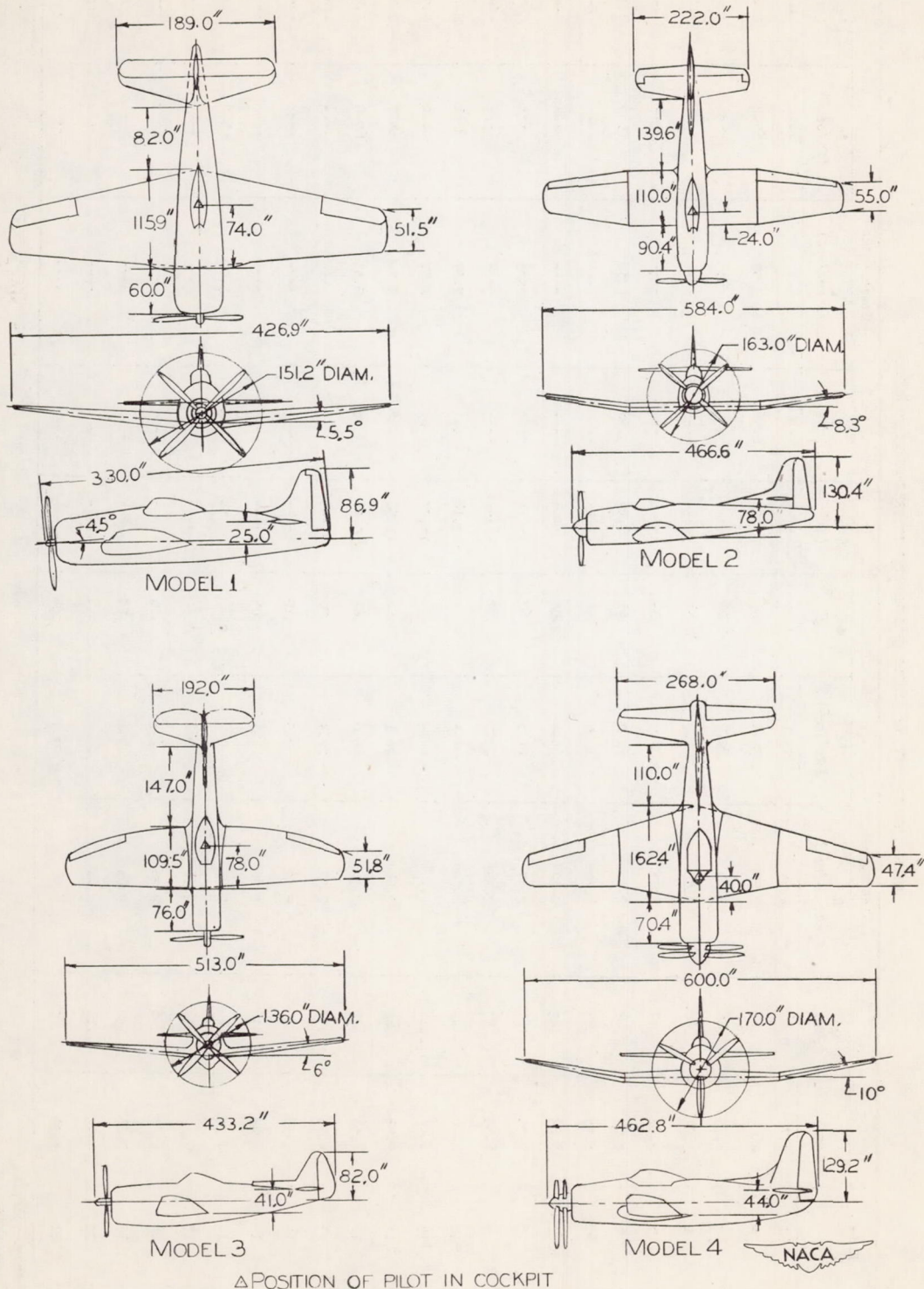
FIGURE 1.- THREE-VIEW SKETCHES OF THE MODELS FOR WHICH PILOT-RELEASE TESTS WERE MADE. DIMENSIONS ARE FULL-SCALE.
