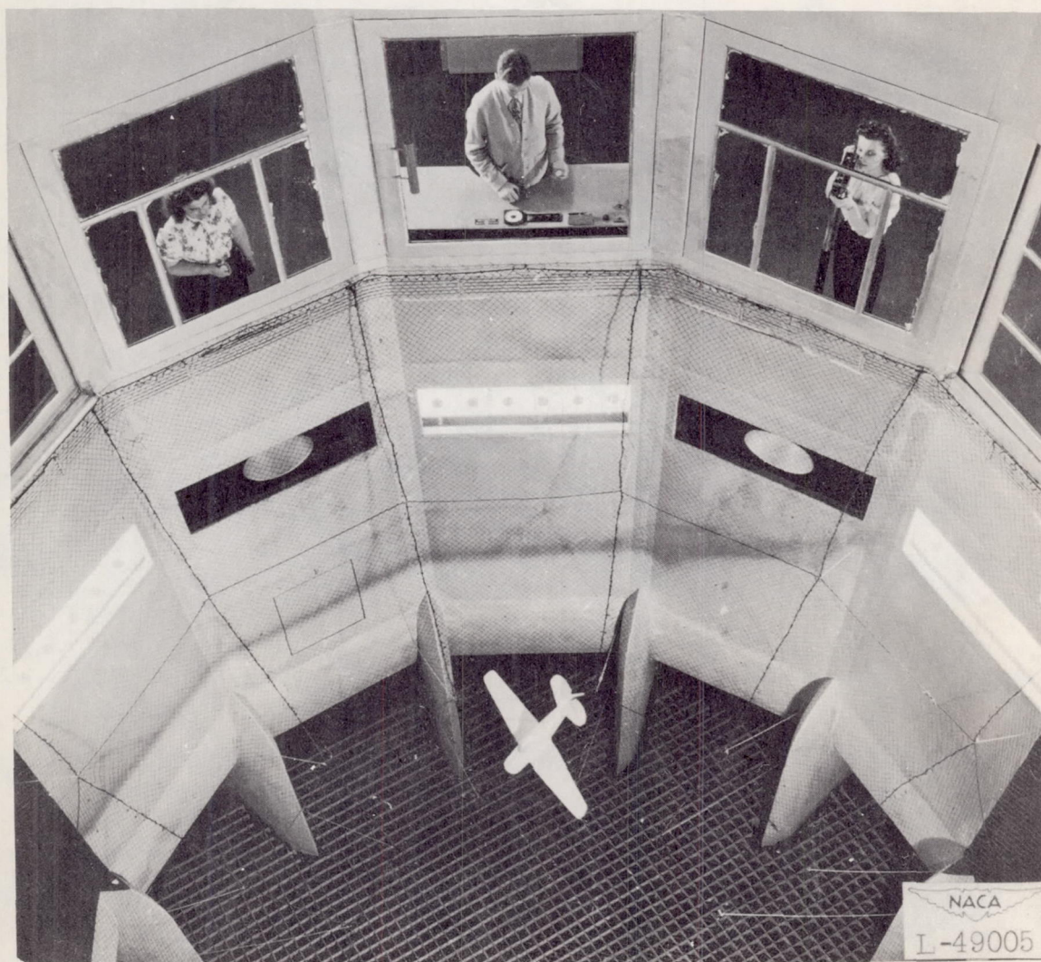
Figure 2.- Photograph of a model spinning in the Langley 20-foot free-spinning tunnel.
