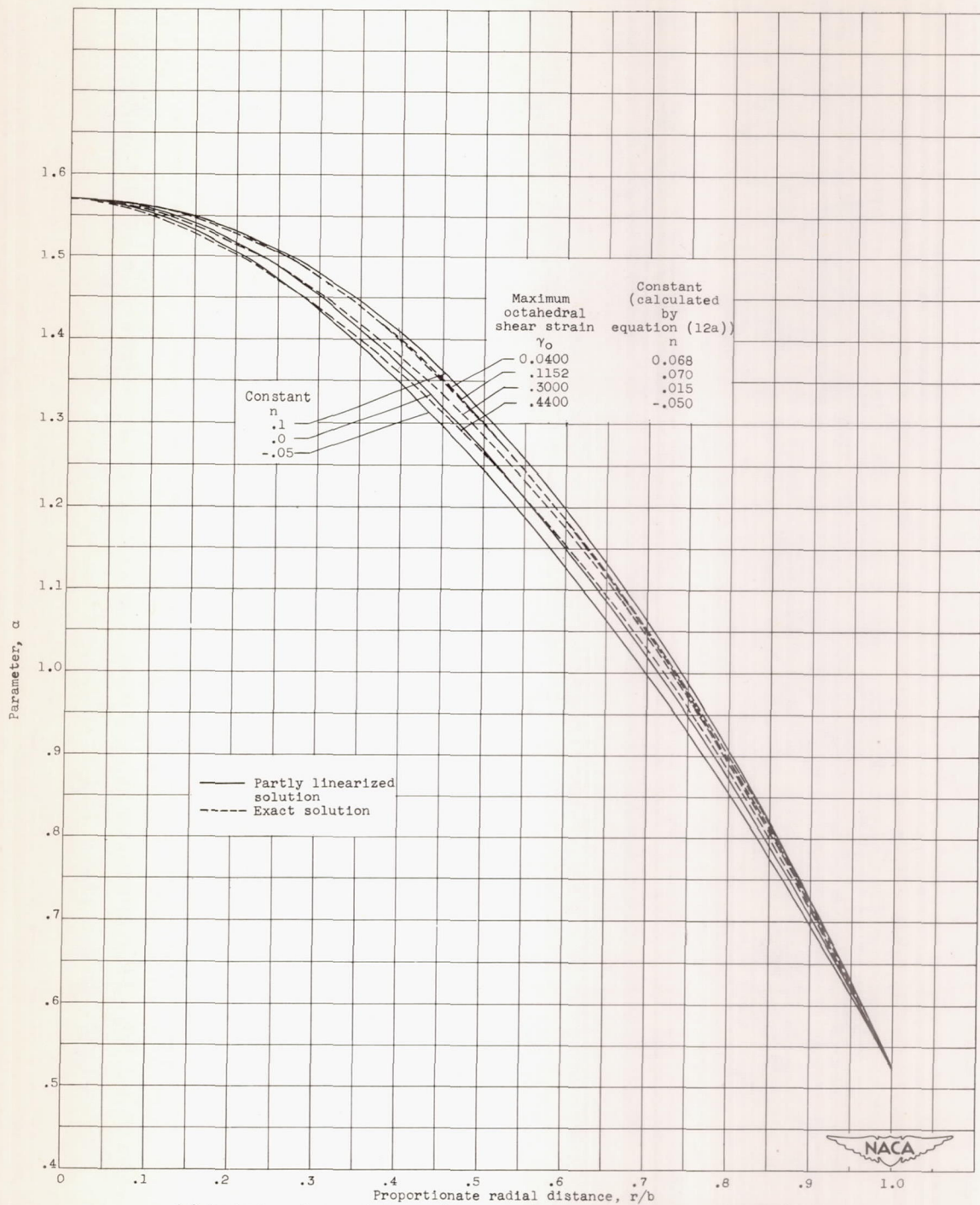
(a) Variation of parameter \alpha with proportionate radial distance for 16-25-6.
