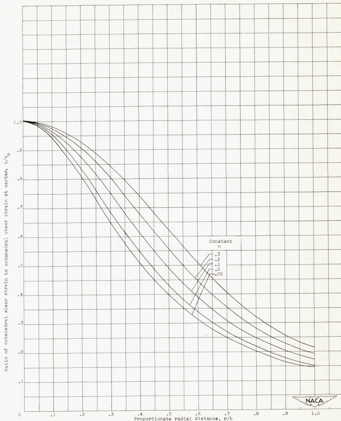
(b) Variation of ratio of octahedral shear strain to octahedral shear strain at center \gamma/\gamma_0 with proportionate radial distance.
