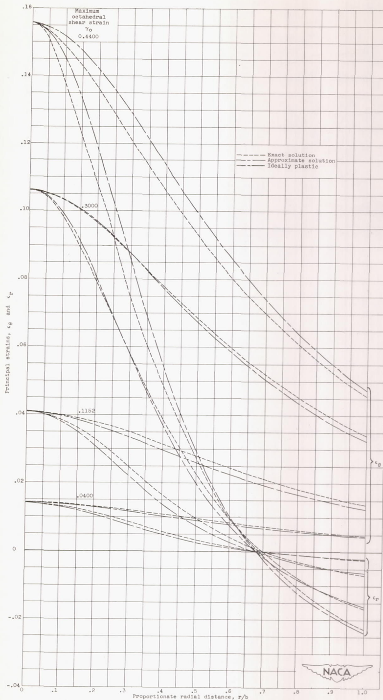
(a) Variation of principal strain with proportionate radial distance, 16-25-6.
