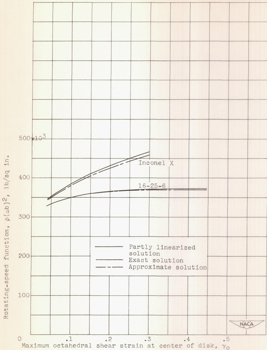
Figure 9. - Comparison of relations between rotating-speed function \rho(\omega b)^2 and maximum octahedral shear strain at center of disk obtained by exact, partly linearized, and approximate solutions for Inconel X and 16-25-6.
