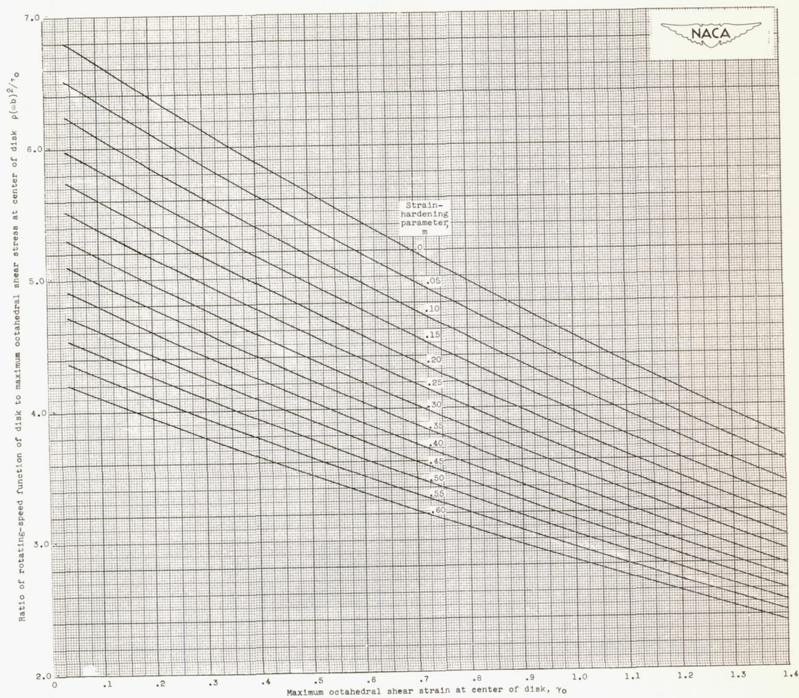
Figure 10. - Variation of ratio of rotating-speed function to maximum octahedral shear stress at center of disk \rho(\omega b)^2/\tau_0 with maximum octahedral shear strain at center of disk for different values of parameter m . (A 14- by 15-in. print of this fig. is attached.)
