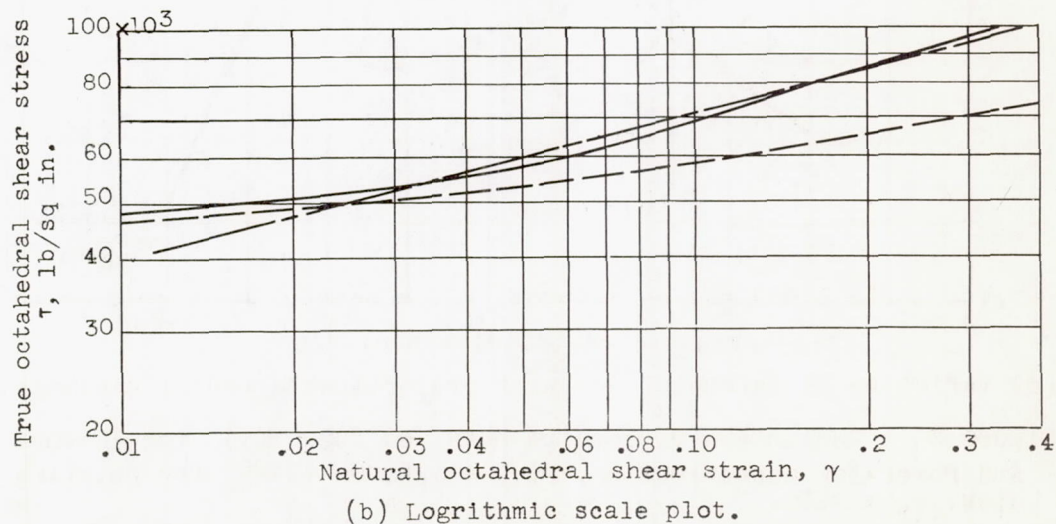
Figure 2. - Octahedral shear stress-strain curves.
