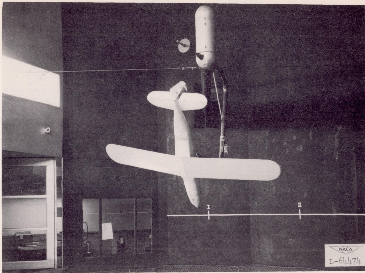
Figure 4.- Photograph of the model mounted on the rotary balance.
