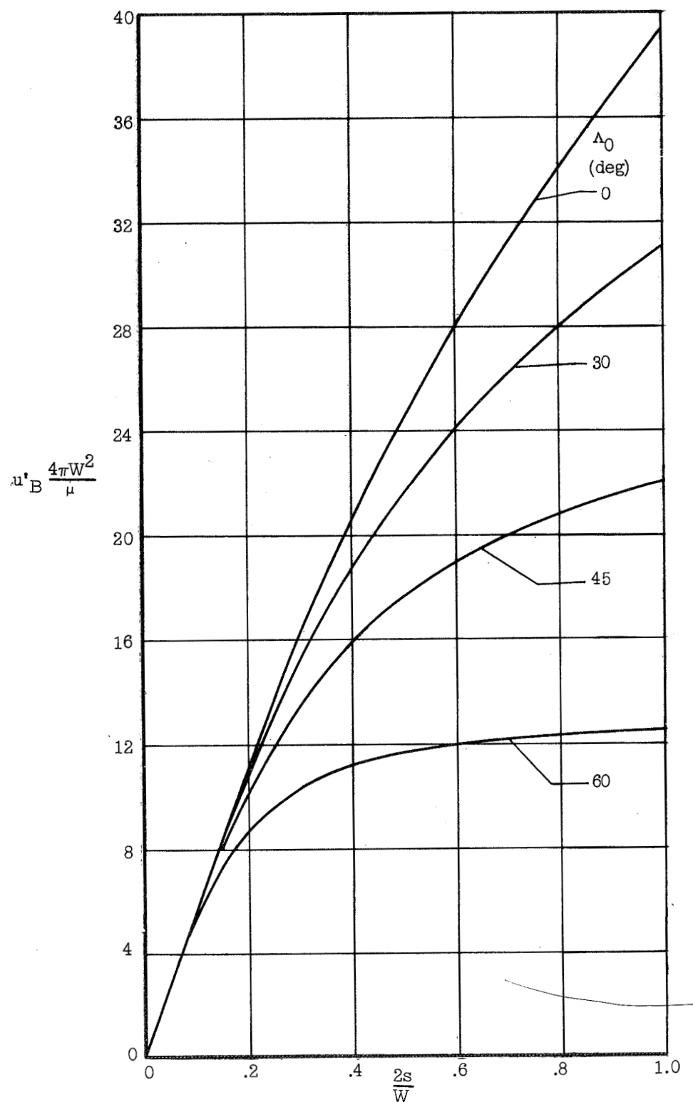
Figure 8.- Nondimensional velocity at B due to a line doublet as a function of span.
