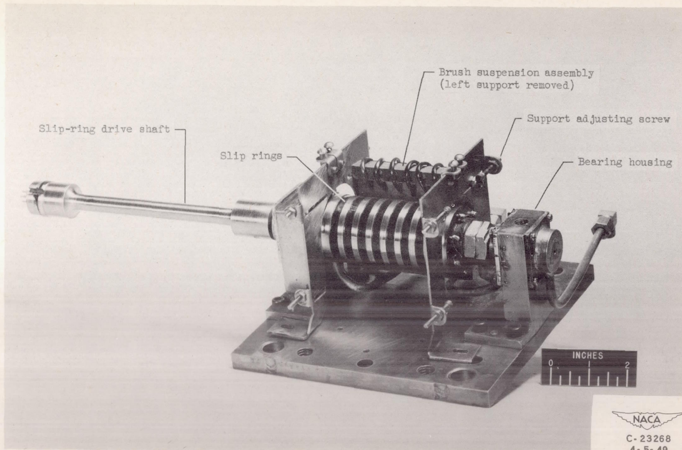
Figure 3. - Slip-ring assembly.
