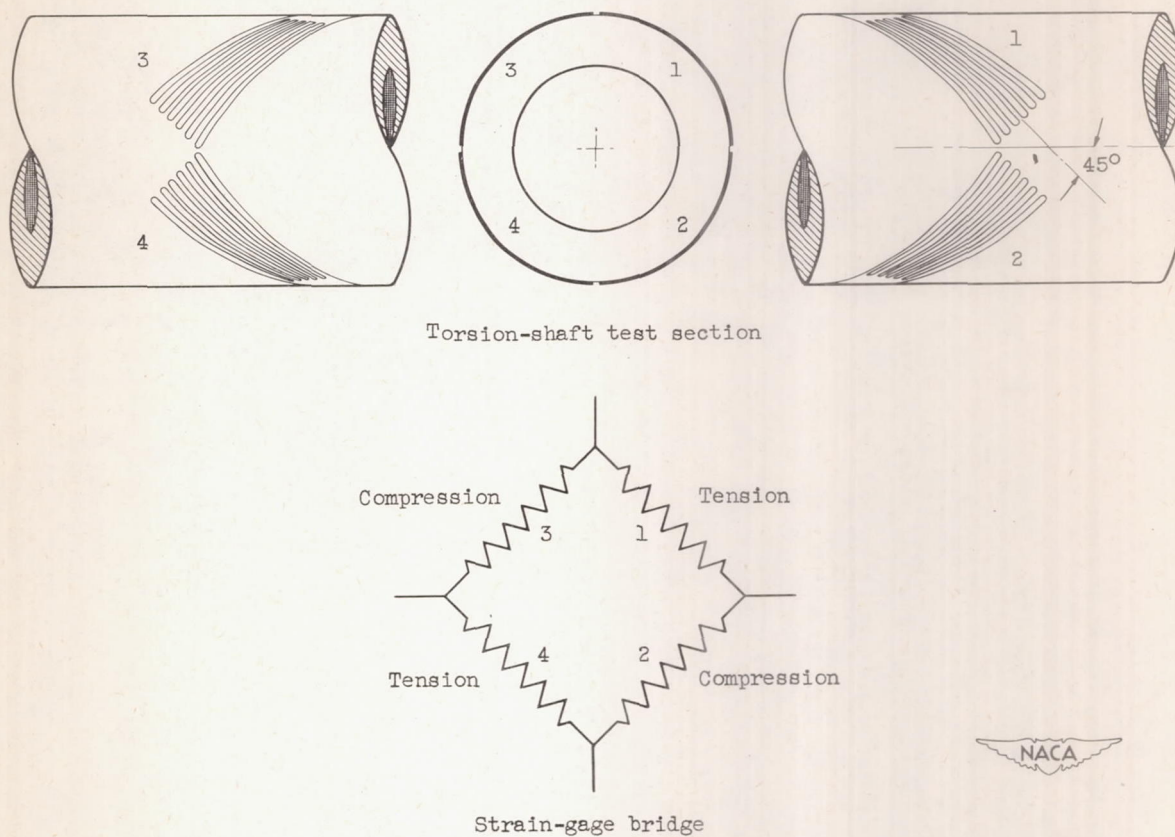
Figure 2. - Orientation of strain gages on torsion-shaft test section. Advance wire strain gages 1,2,3, and 4 are 350 ohms.
