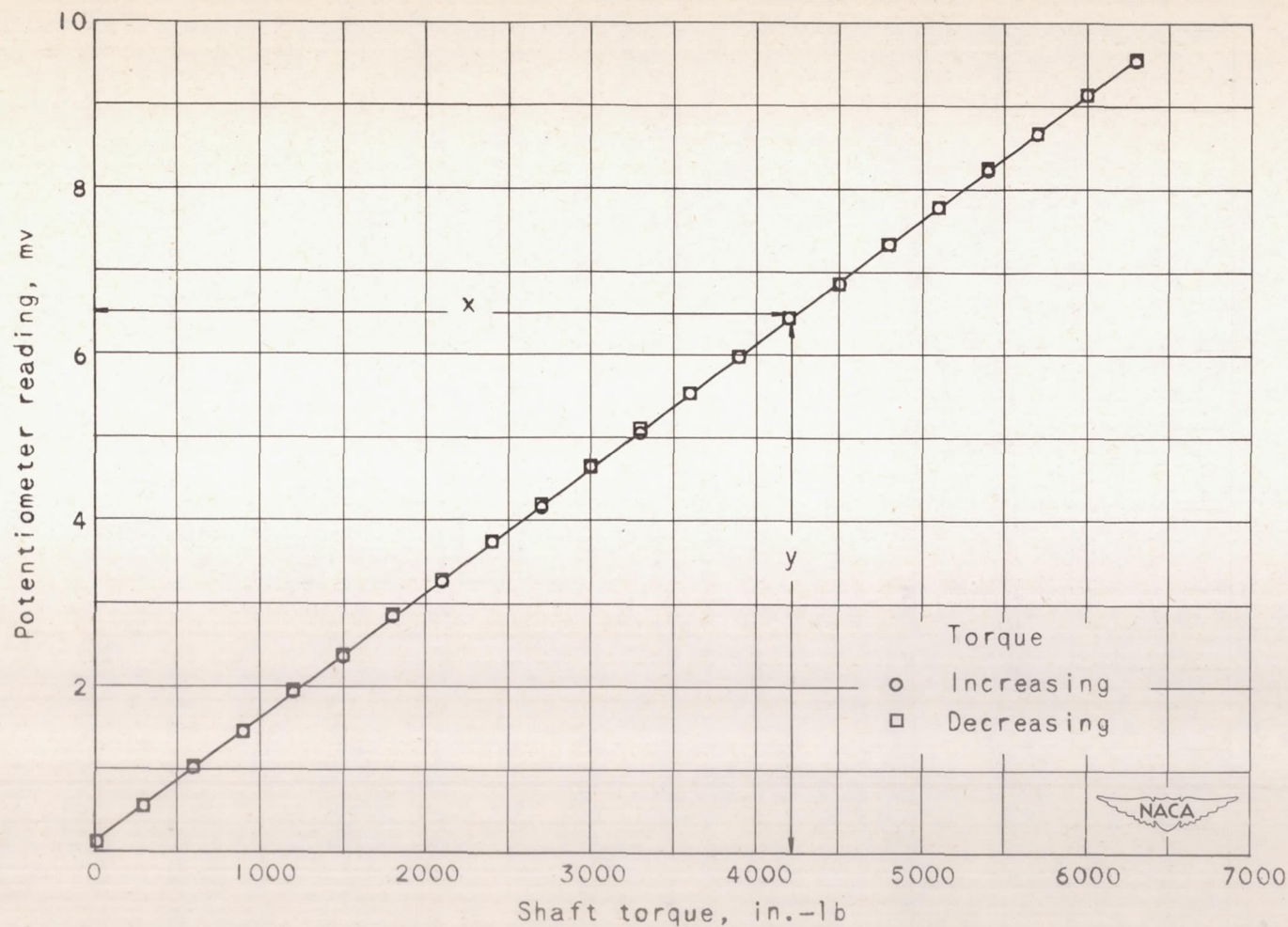
Figure 10.— Static calibration of strain-gage torquemeter (torsion-shaft temperature, 73° F) when contact resistance is present in circuit.
