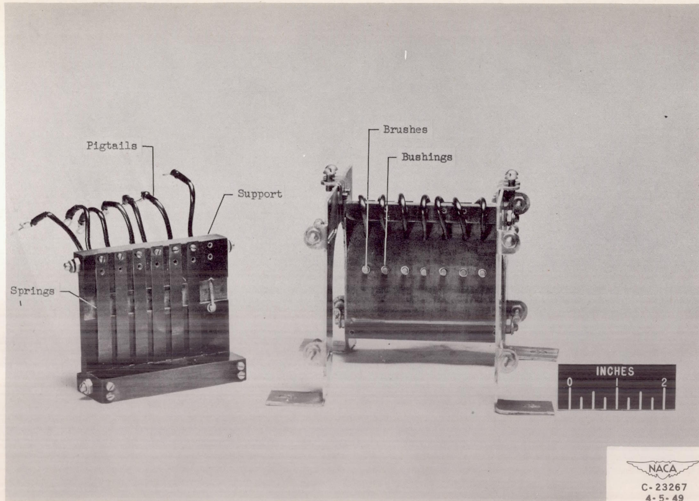
Figure 4. - Brush-suspension assembly.
