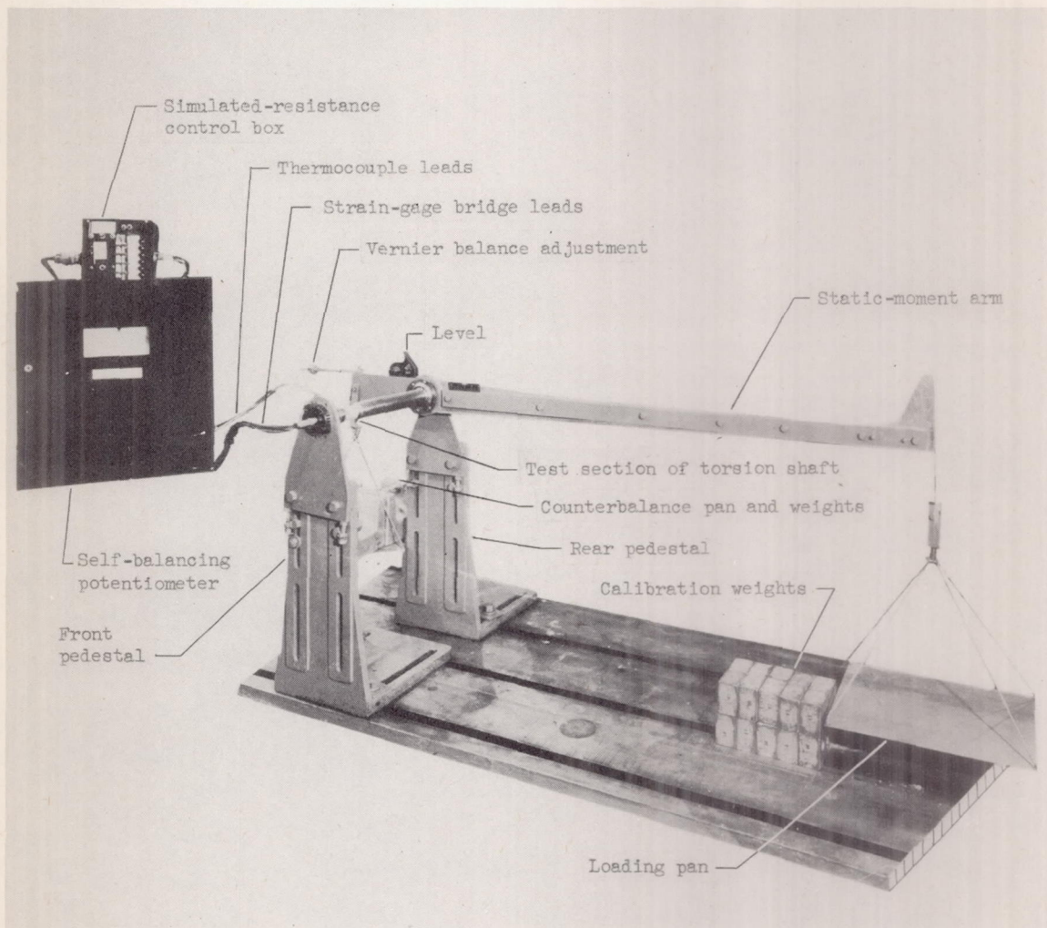
Figure 8. - Torsion-shaft apparatus for static calibration.
