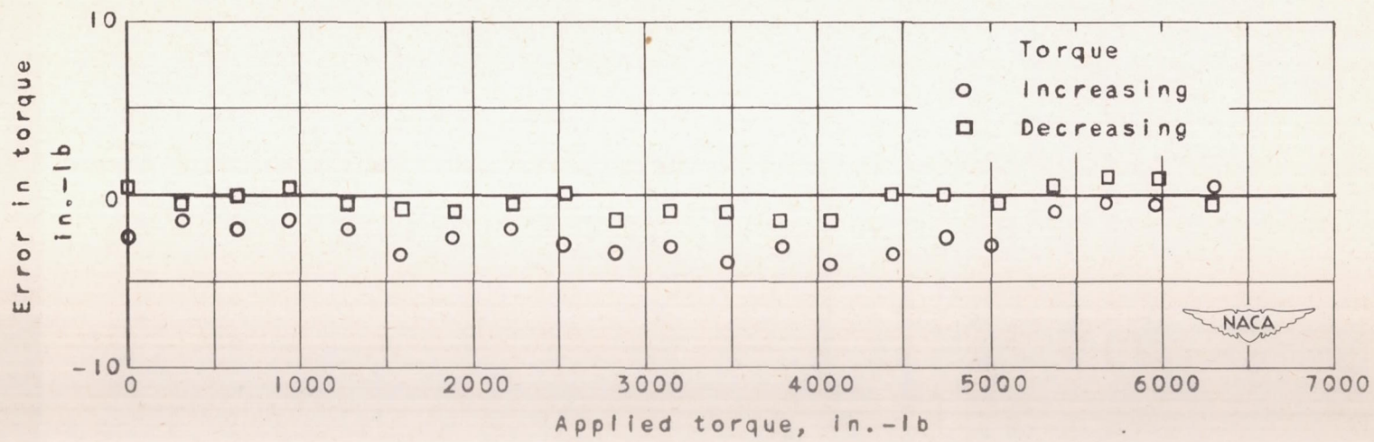
Figure 7. - Results of typical dynamometer static calibration..
