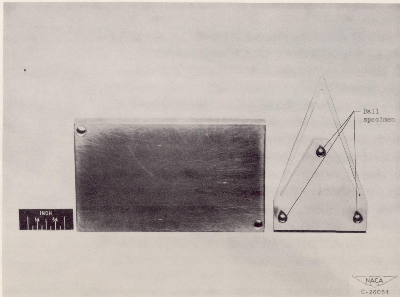
(c) Plate specimen and rider specimens in rider assembly.
