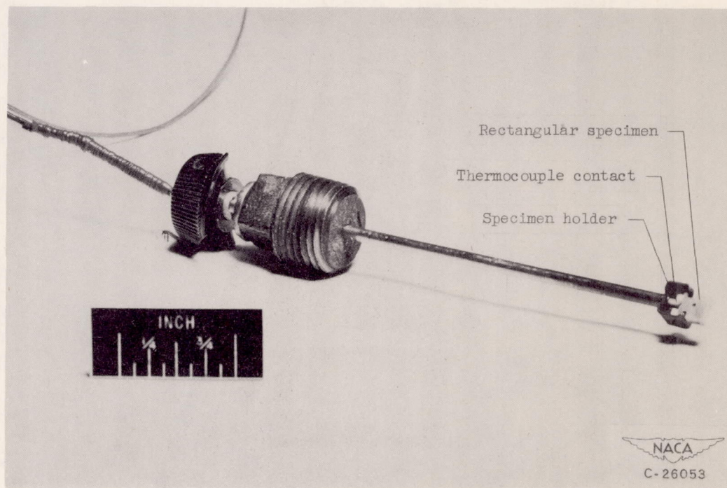
(b) Specimen and specimen holder with thermocouple and leads passing through the hollow shaft.
