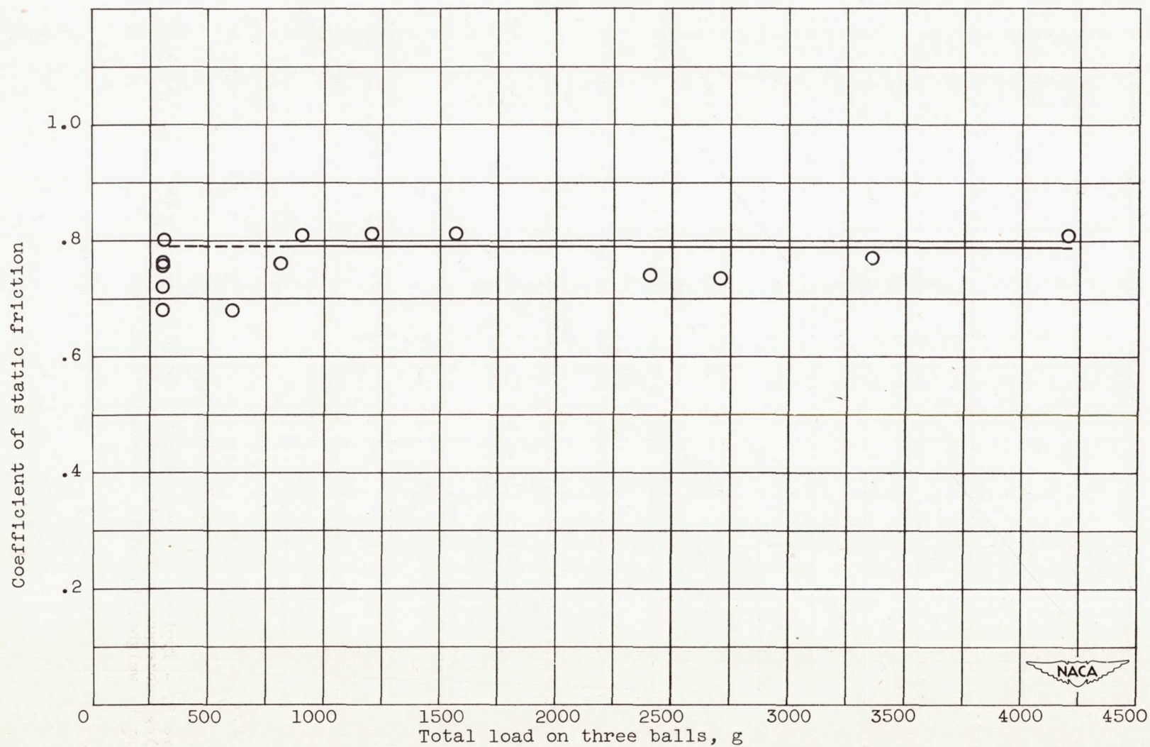
Figure 6. - Effect of load on coefficient of static friction of clean hardened steel balls sliding on dry mild steel plate.
