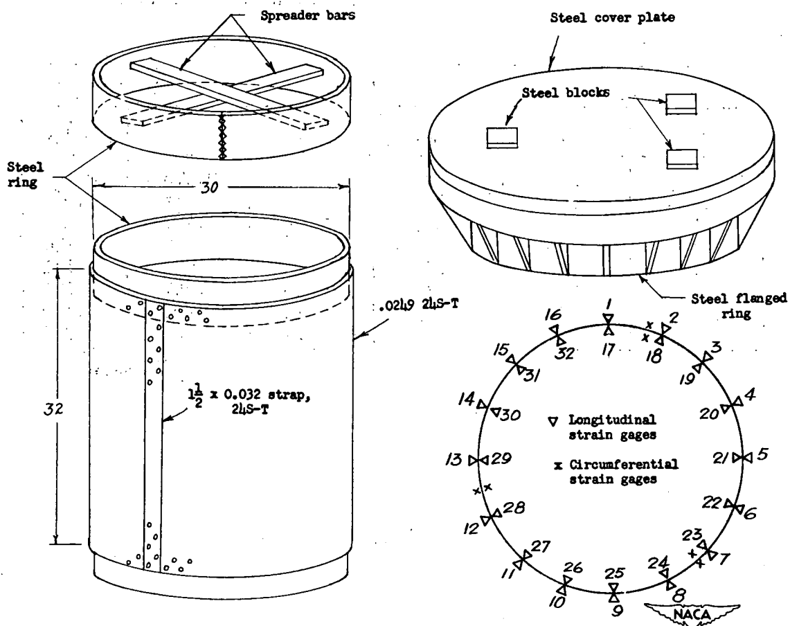
Figure 1.- Test specimen and strain-gage positions.
