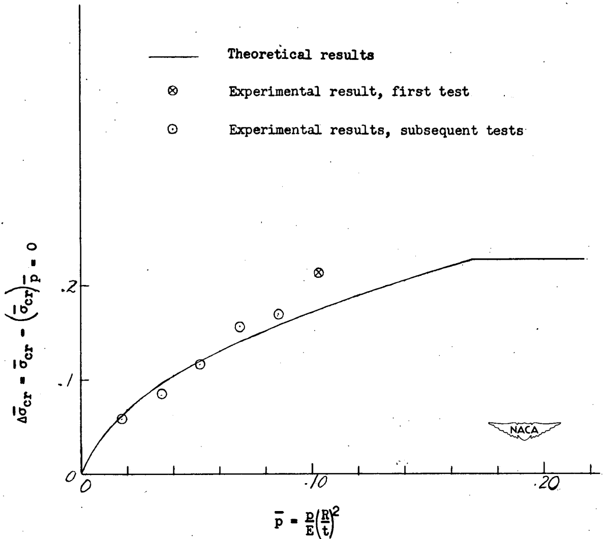
Figure 4.- Theoretical and experimental results showing the increment of buckling stress due to internal pressure.
