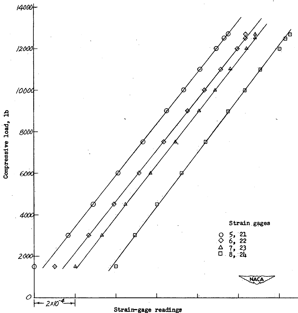
(a) Linear part of load-strain curve for four typical pairs of strain gages.
