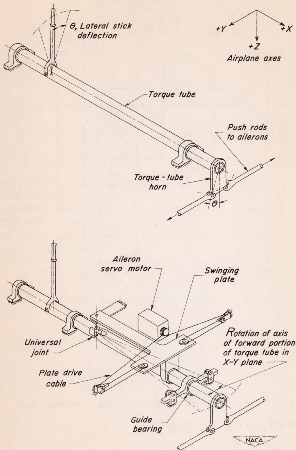
Figure 3.-Sketch of original and modified aileron control system.
