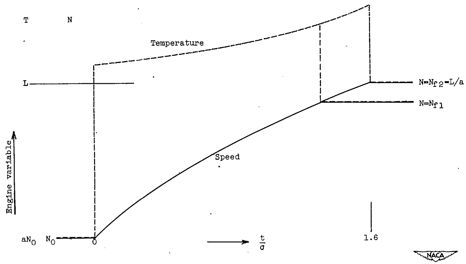
Figure 10. - Typical transients for controlled system for minimum rise time with temperature-limiting criterions (case C).
