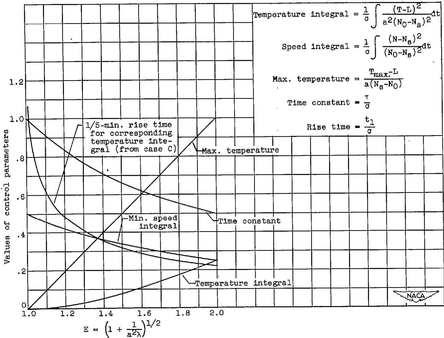
Figure 4. - Various control parameters as functions of E for speed control with temperature-limiting criterions (case B), when accelerating to limiting temperature.
