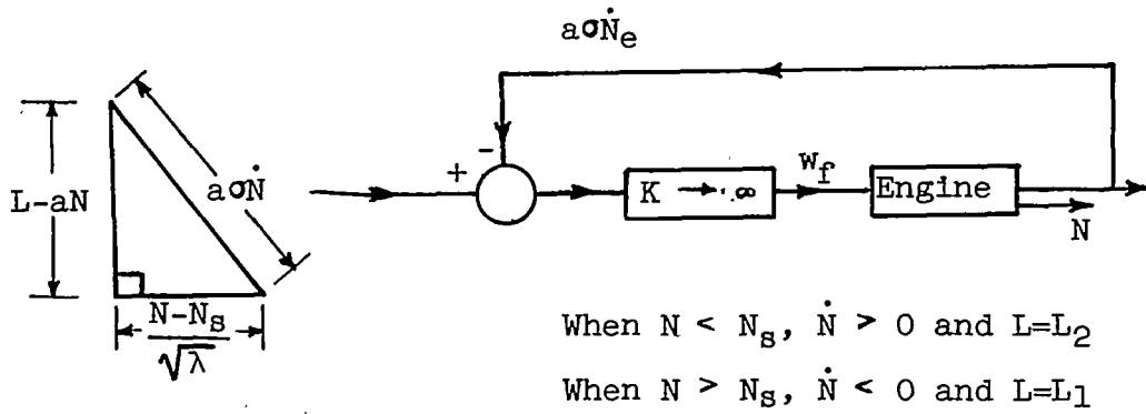
Figure 3. - Schematic diagram of control for turbojet engine for case of speed control with temperature-limiting criterions (case B). Stability device must be added to this system.
