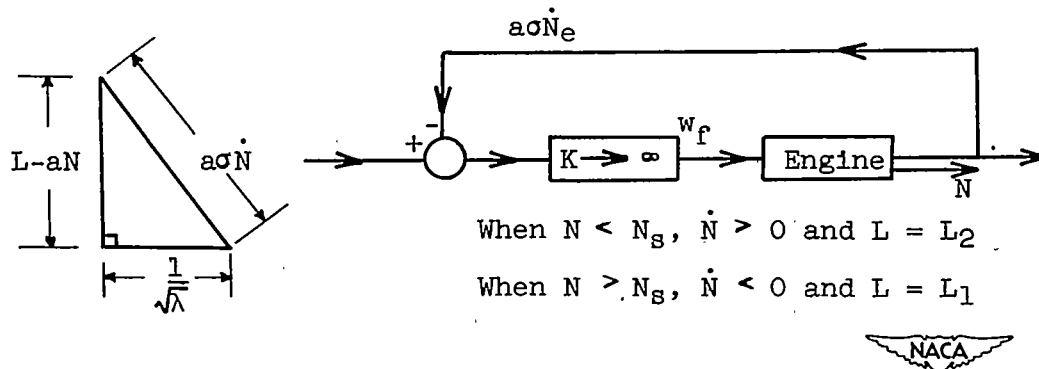
Figure 7. - Schematic diagram of control for turbojet engine for minimum rise time with temperature-limiting criterions (case C). Stability device must be added to this system.
