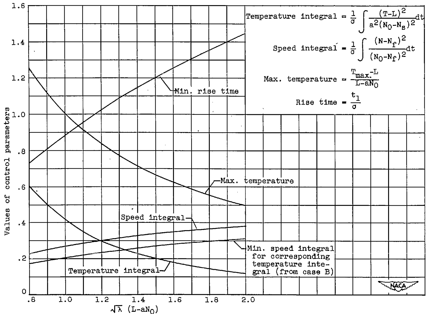
Figure 8. - Various control parameters as function of \lambda for minimum rise time with temperature-limiting criterions (case C), when accelerating to limiting temperature.
