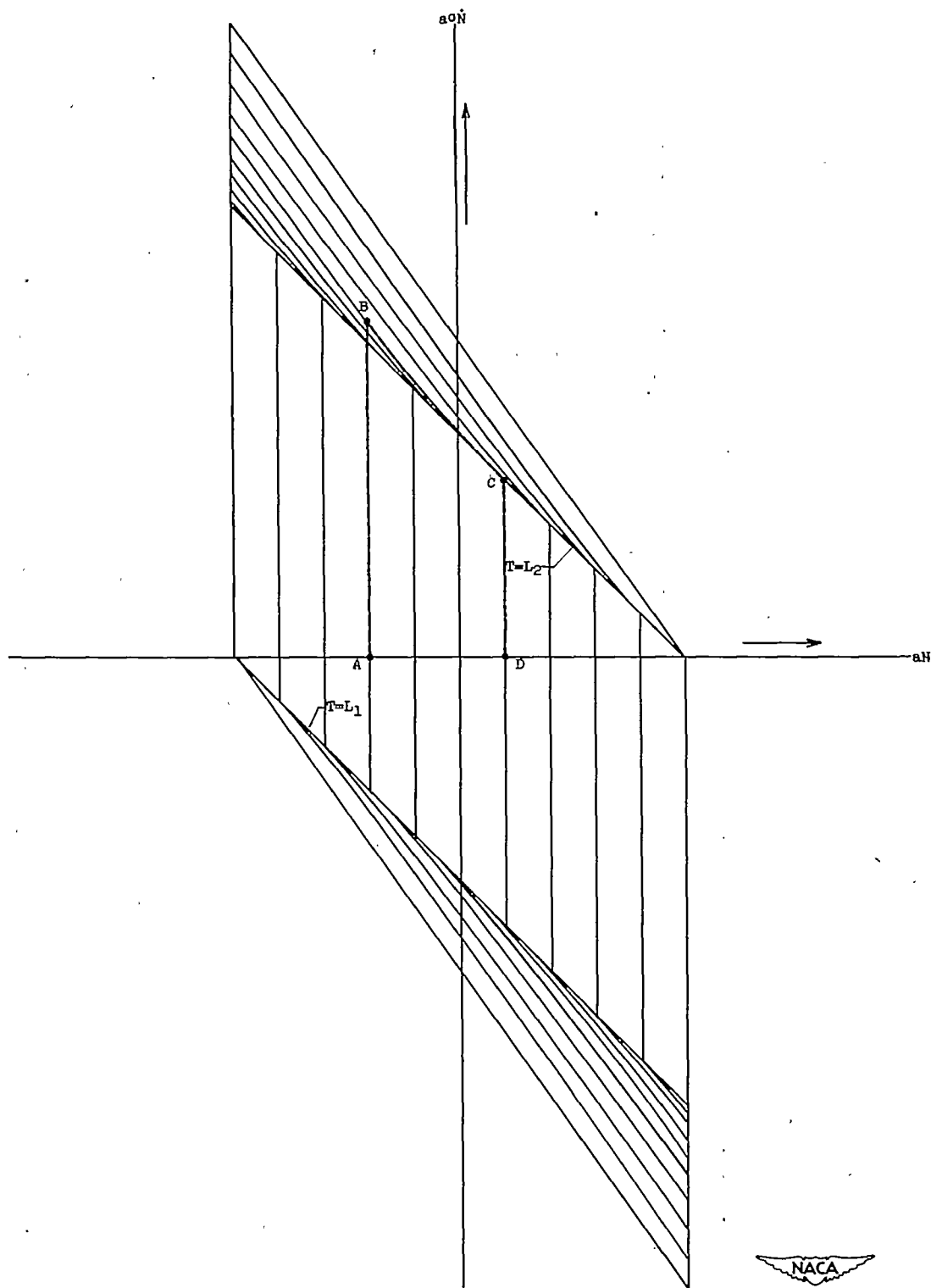
Figure 5. - Phase plane showing dynamics of controlled system for speed control with temperature-limiting criteria (case B), where a^2\lambda = 1 .
