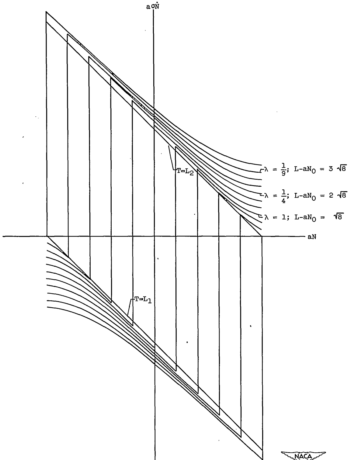
Figure 9. - Phase plane showing dynamics of controlled system for minimum rise time with temperature-limiting criterions (case C), where \sqrt{\lambda} (L-aN_0) = \sqrt{8} .
