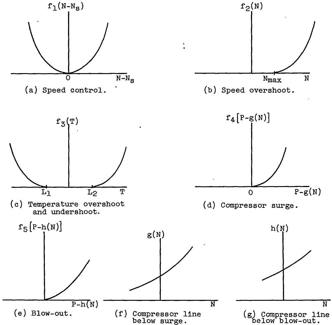
Figure 2. - Arbitrary weighting functions for various control criteria and pertinent engine characteristics involved.
