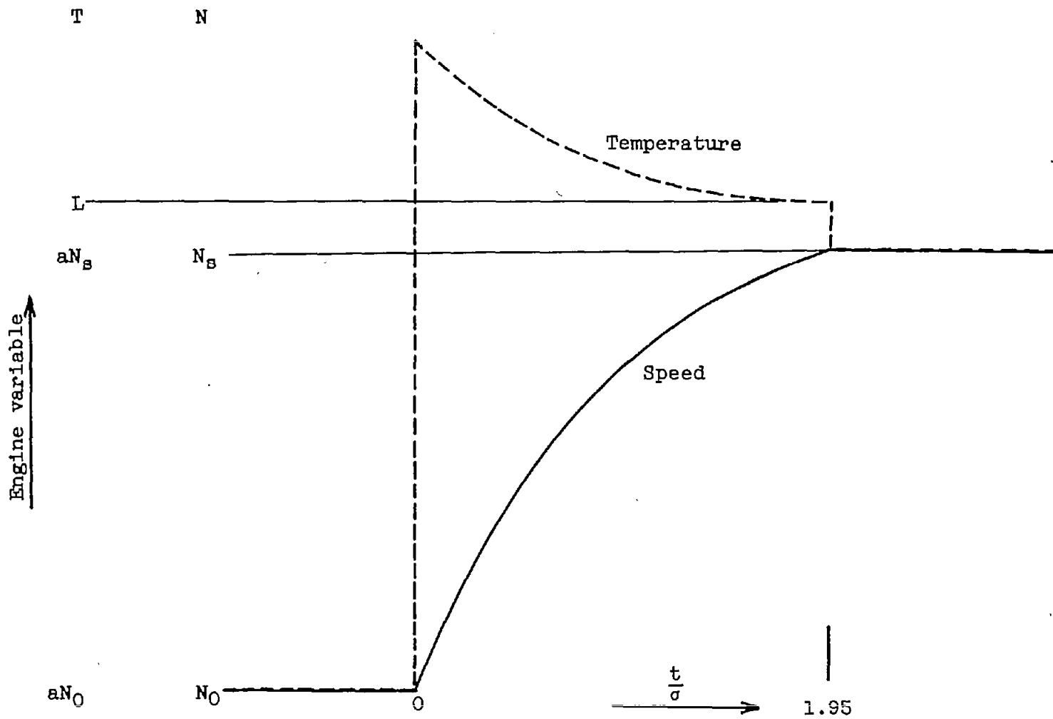
Figure 6. - Typical transient of controlled system for speed control with temperature-limiting criteria (case B), where E = \sqrt{2} .
