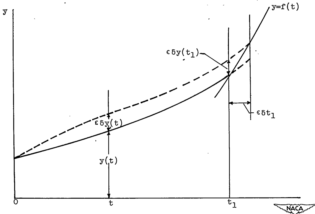
Figure 1. - Illustration of curves for minimization of \int_0^{t_1} F(y, \dot{y}) dt .
