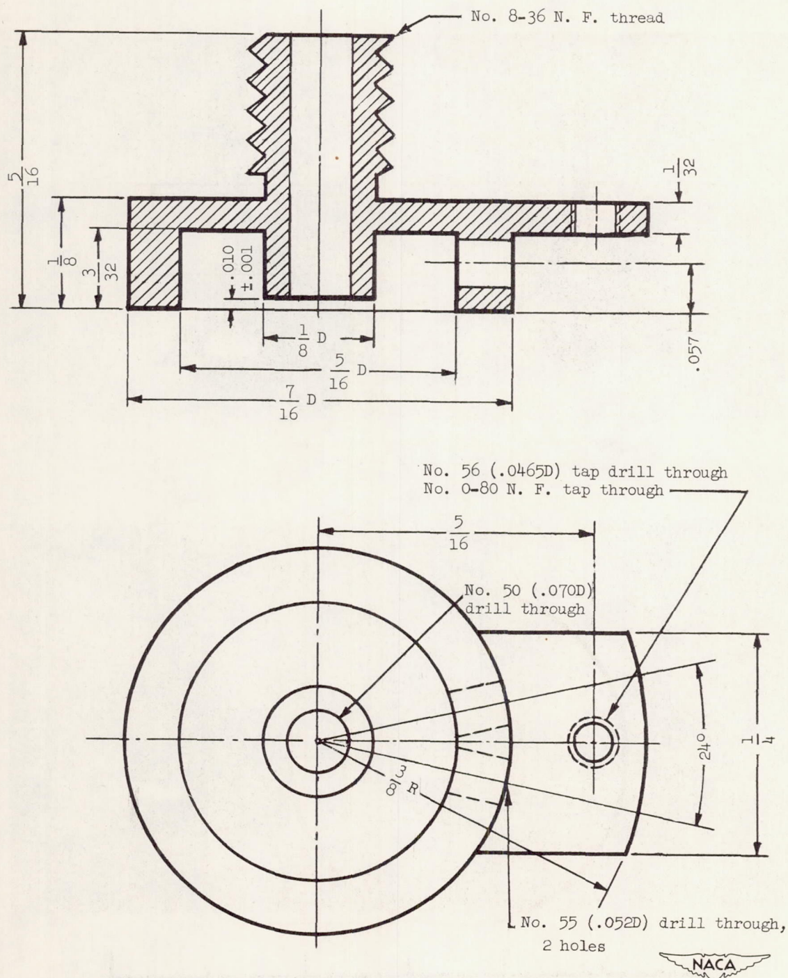
Figure 13.- Detailed drawings of the main components of the NACA miniature electrical pressure gage model 49-NC. (Notations are in accordance with standard drafting practice.)
