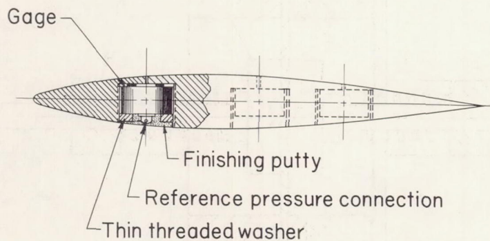
(c) Small solid airfoil.
