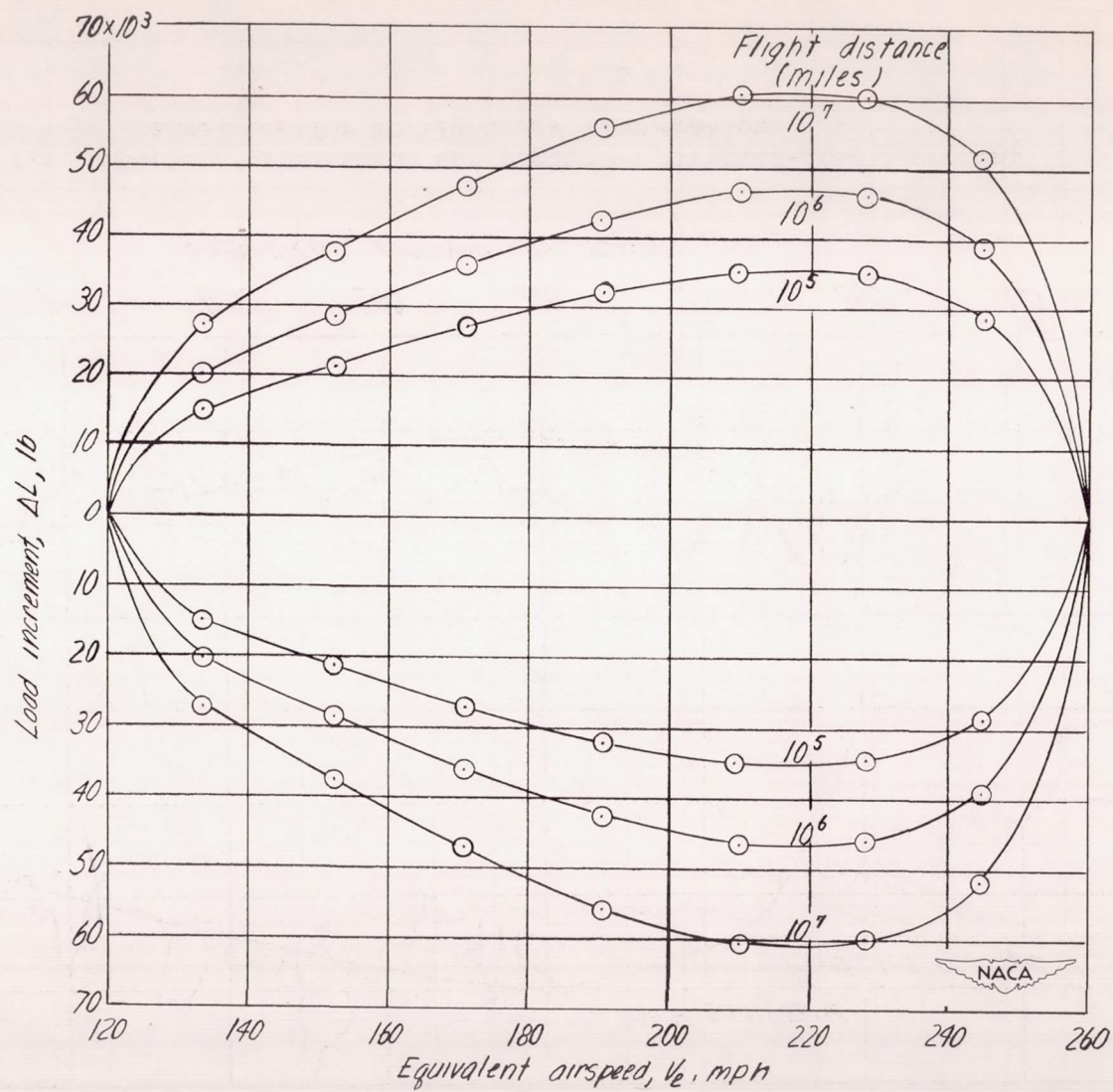
Figure 8.- Airspeed-load-increment envelopes for given flight distances.
