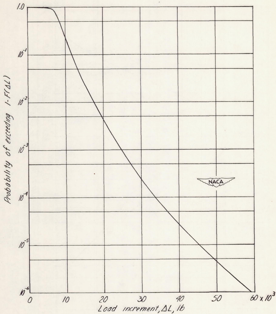
Figure 5.- Probability that a value of load increment will be greater than indicated value.
