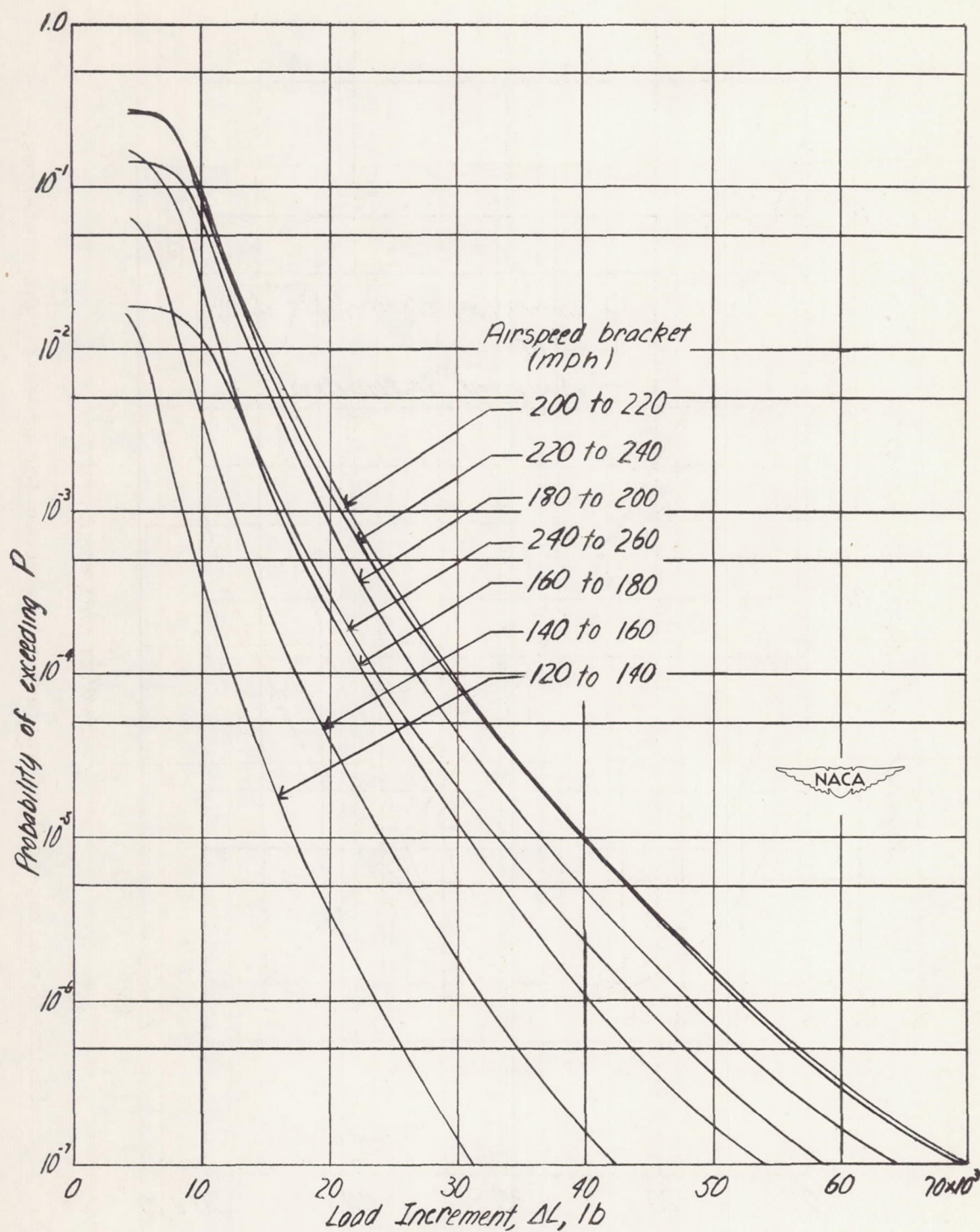
Figure 7.- Probability that a value of load increment will occur in a given airspeed bracket and exceed indicated value.
