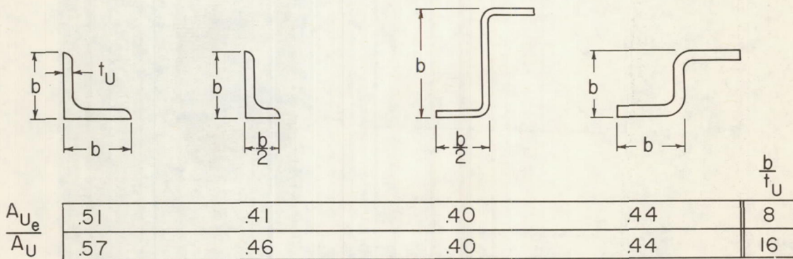
Figure 7.- Ratio of effective to actual area of uprights.
