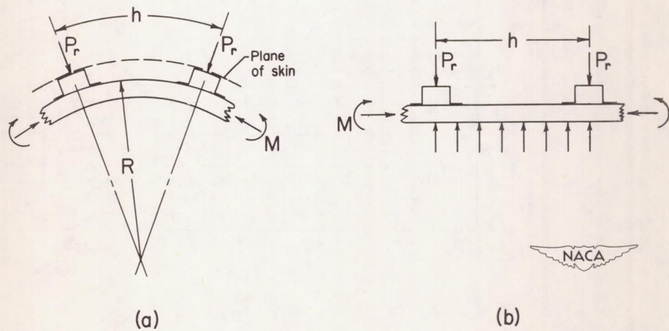
Figure 29.- Forces on floating rings.
