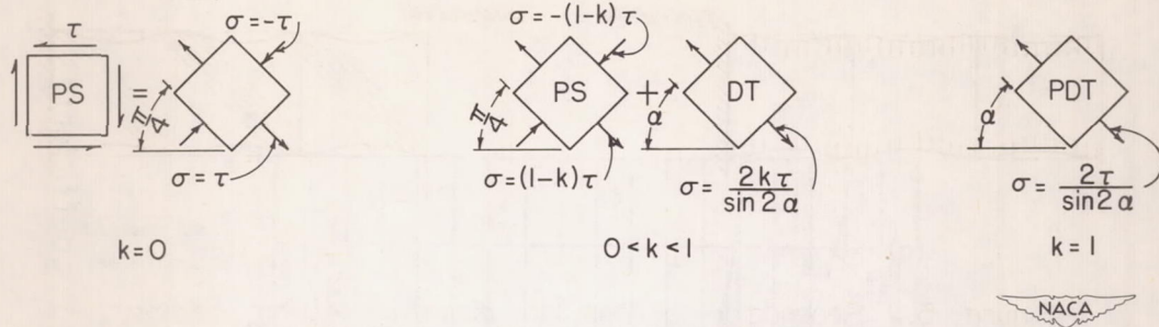
Figure 8.—Stress systems in diagonal-tension webs.
