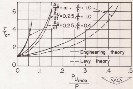
Figure 10.—Upright forces by two theories. P_{Umax} = \sigma_{Umax} A_U
