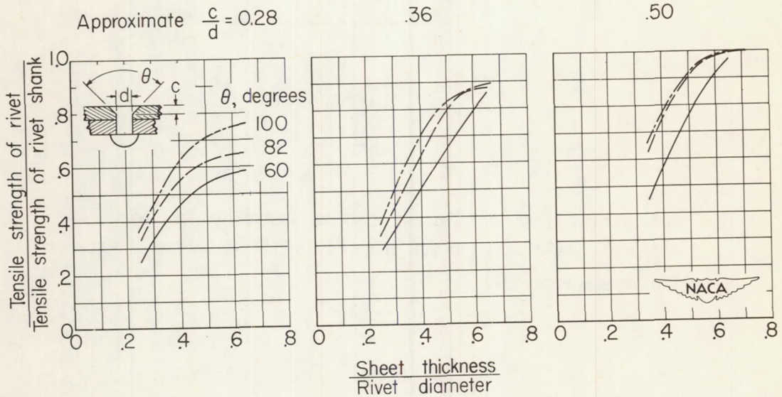
Figure 36.- Tensile strength of NACA machine-countersunk flush rivets of Al7S-T3 aluminum-alloy in 24S-T3 aluminum alloy sheet.
