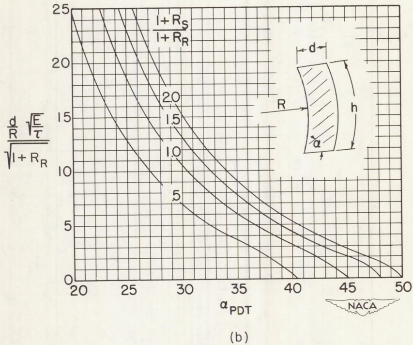
Figure 28.—Angle of pure diagonal tension.
