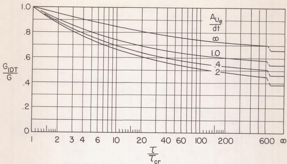
(a) Modulus ratio for elastic web.
