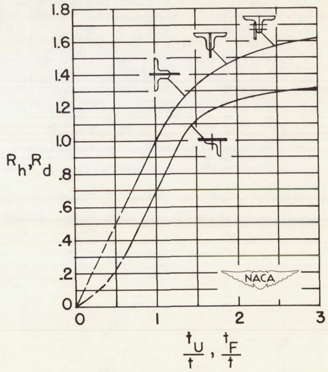
(a) Theoretical coefficients for plates with simply supported edges. (b) Empirical restraint coefficients.
