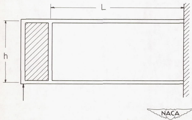
Figure 38. - Portal frame.
