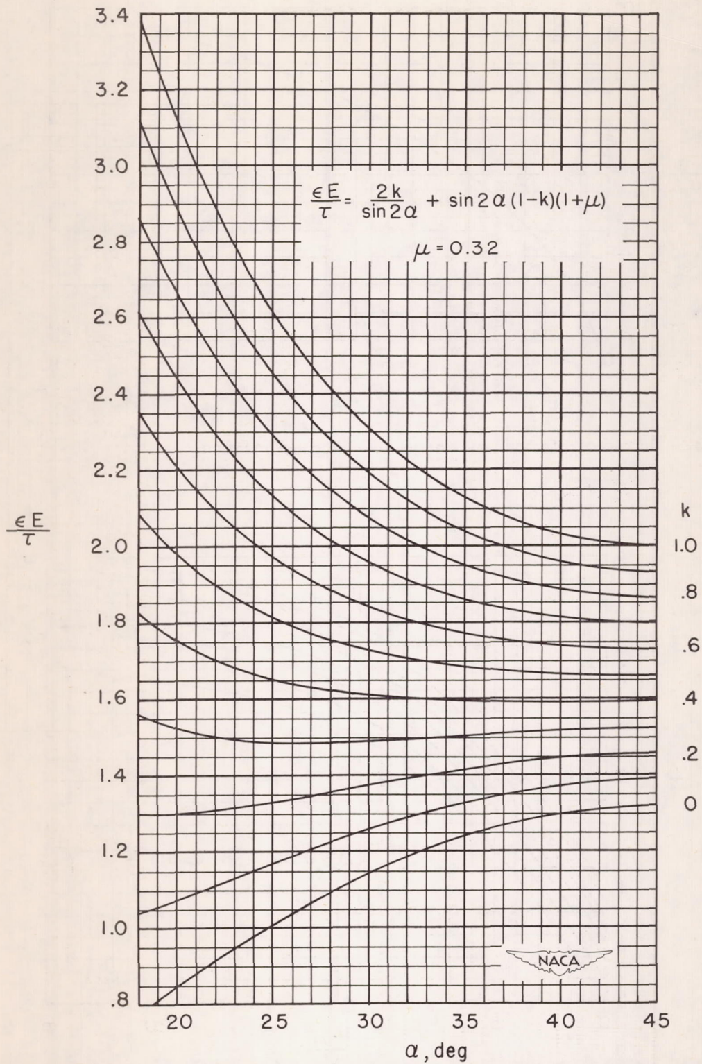
Figure 31.—Graph for calculating web strain .
