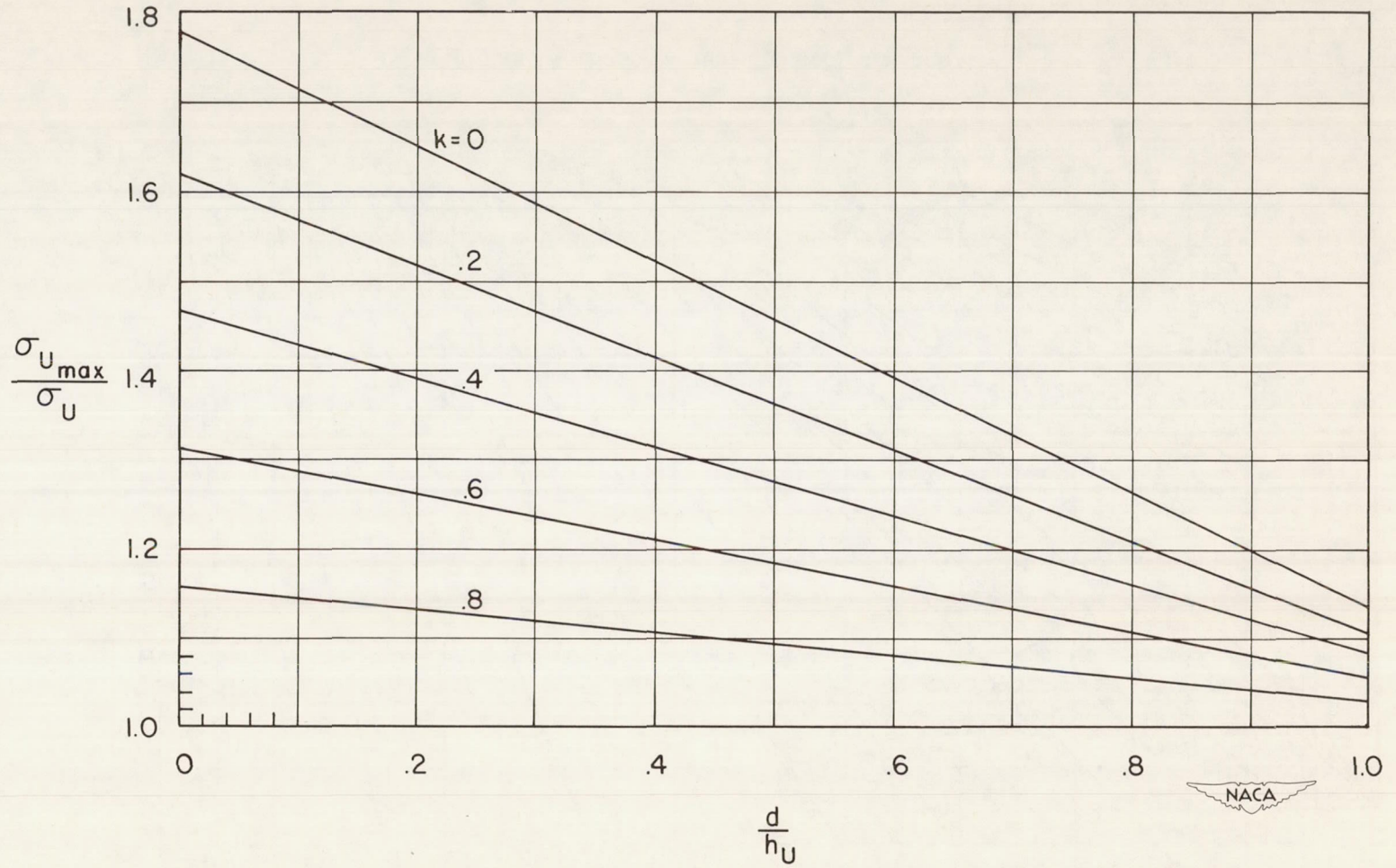
Figure 15.— Ratio of maximum stress to average stress in web stiffener .
