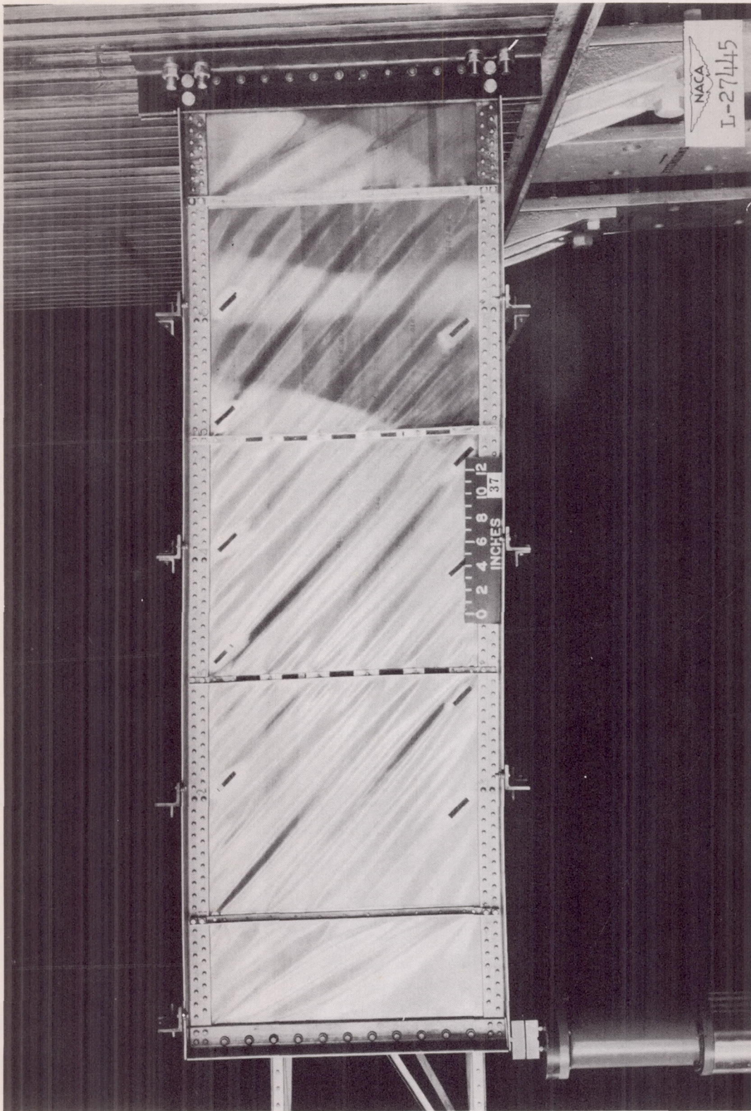
Figure 2.- Diagonal-tension beam.
