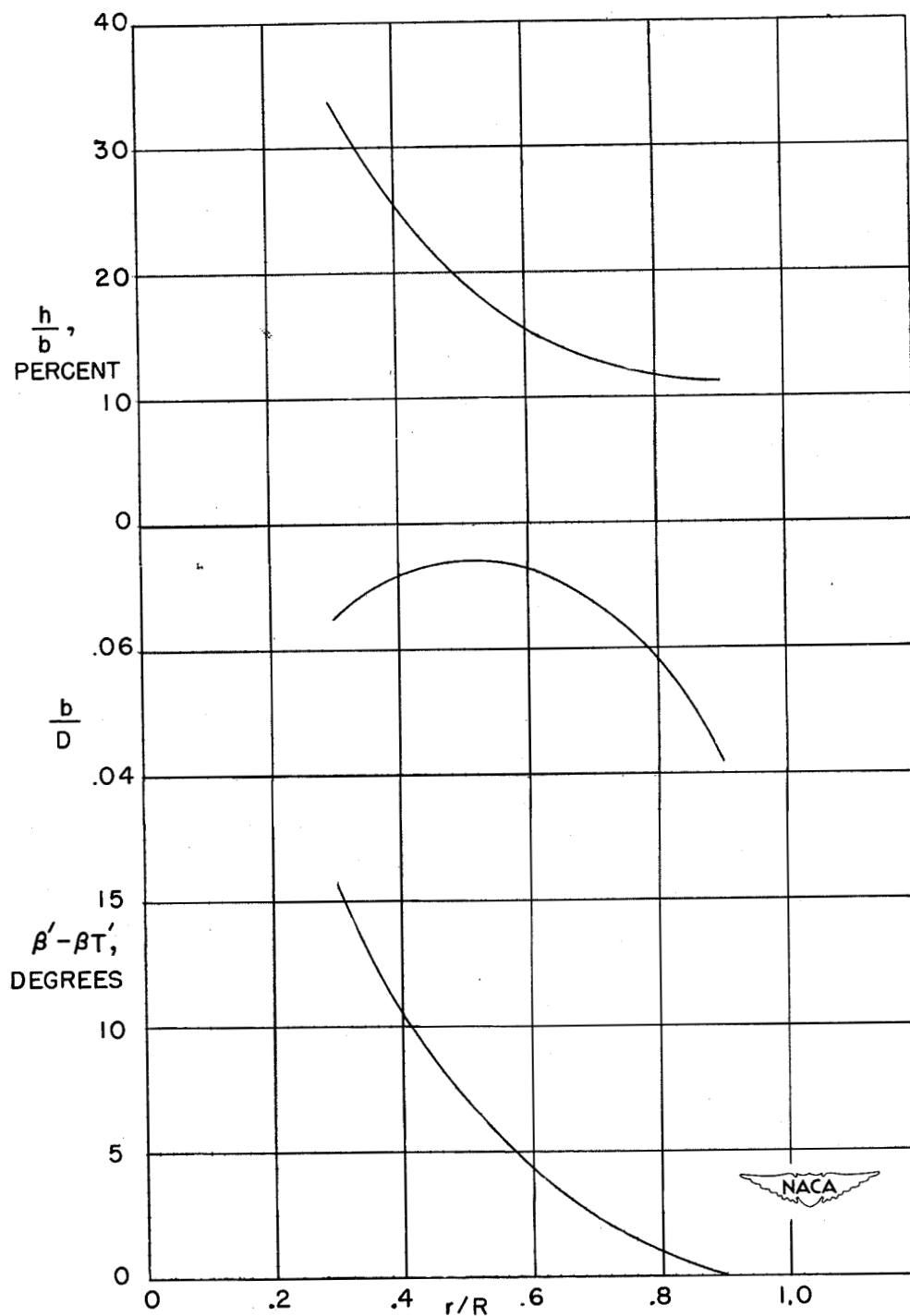
Figure 8.- Blade-form curves for propeller used on both versions of CAA Cub (configurations 2M and 2U) and on standard Cub (configuration 4). D , diameter of propeller; R , tip radius; r , radius of element; b , width (chord) of element; h , maximum thickness of element; \beta' , pitch angle of element; \beta T' , pitch angle of tip element.
