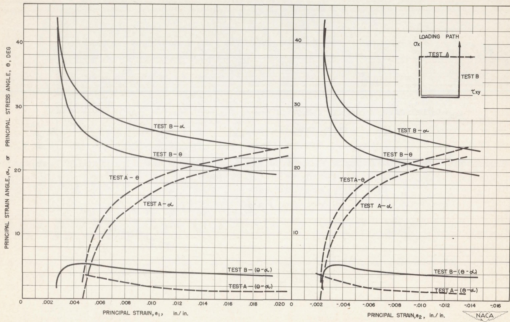
Figure 21.- Comparison of principal strain and stress directions.
