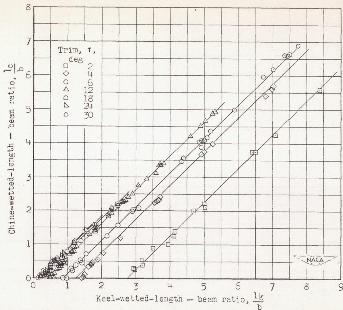
Figure 10.- Variation of chine-wetted-length-beam ratio with keel-wetted-length-beam ratio.
