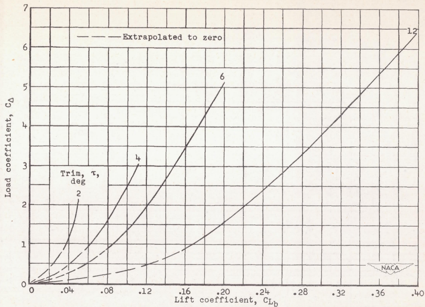
Figure 18.- Curves defining the variation of minimum load coefficient for pure planing.
