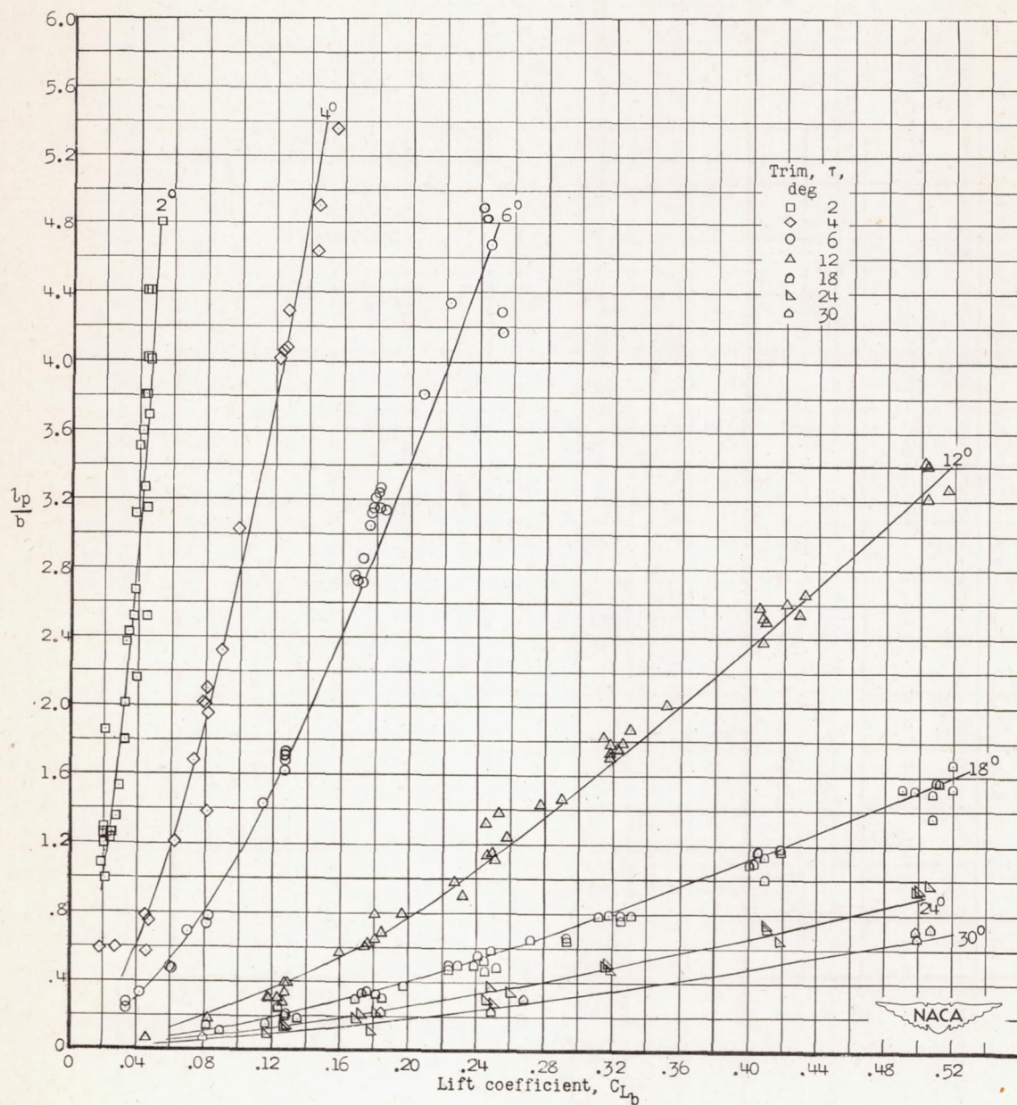
Figure 12.- Variation of nondimensional center-of-pressure location l_p/b with lift coefficient C_{L_b} .
