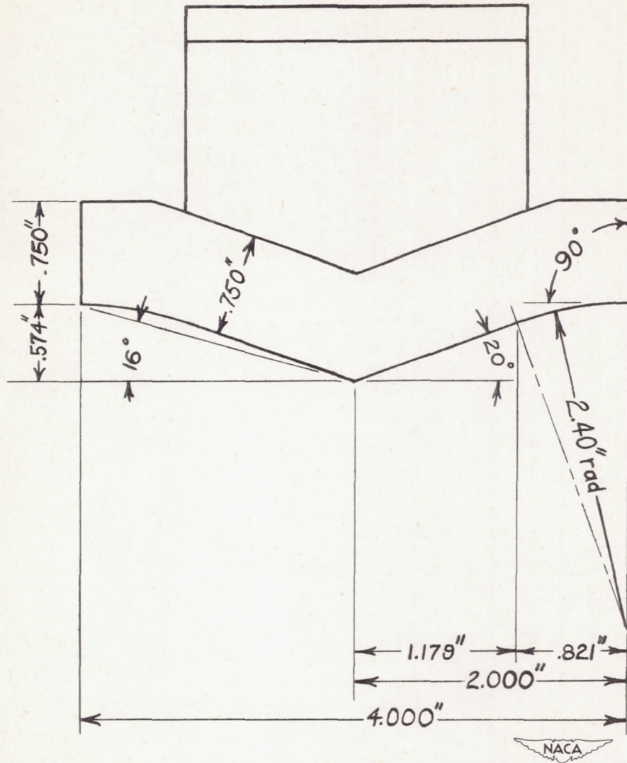
Figure 2.- Cross section of model.
