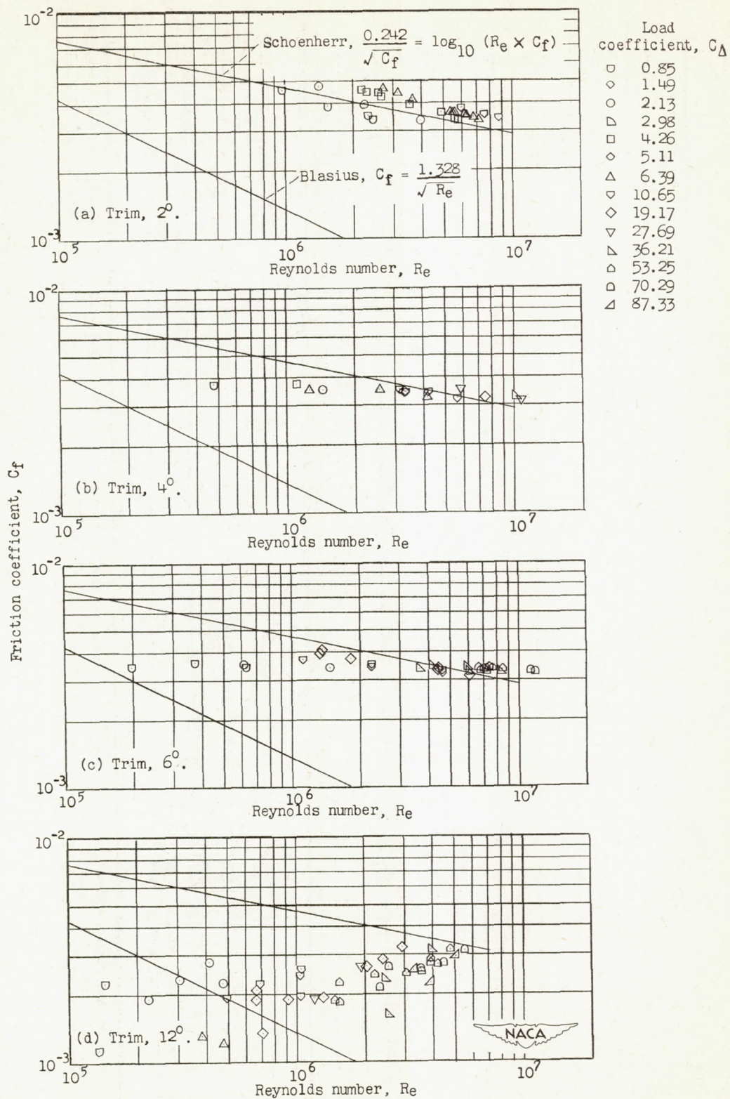
Figure 20.- Variation of friction coefficient with Reynolds number.
