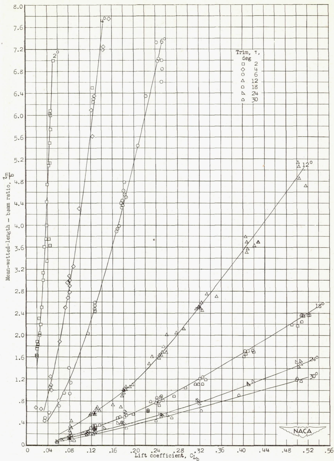
Figure 9.- Variation of mean-wetted-length-beam ratio \frac{l_m}{b} with lift coefficient C_{Lb} .
