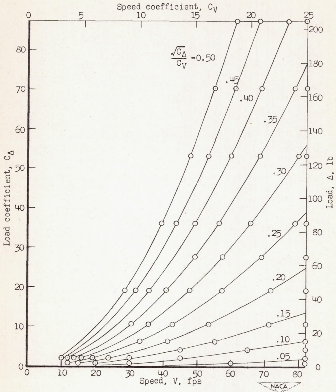
Figure 8.- Load-speed schedule for test program.
