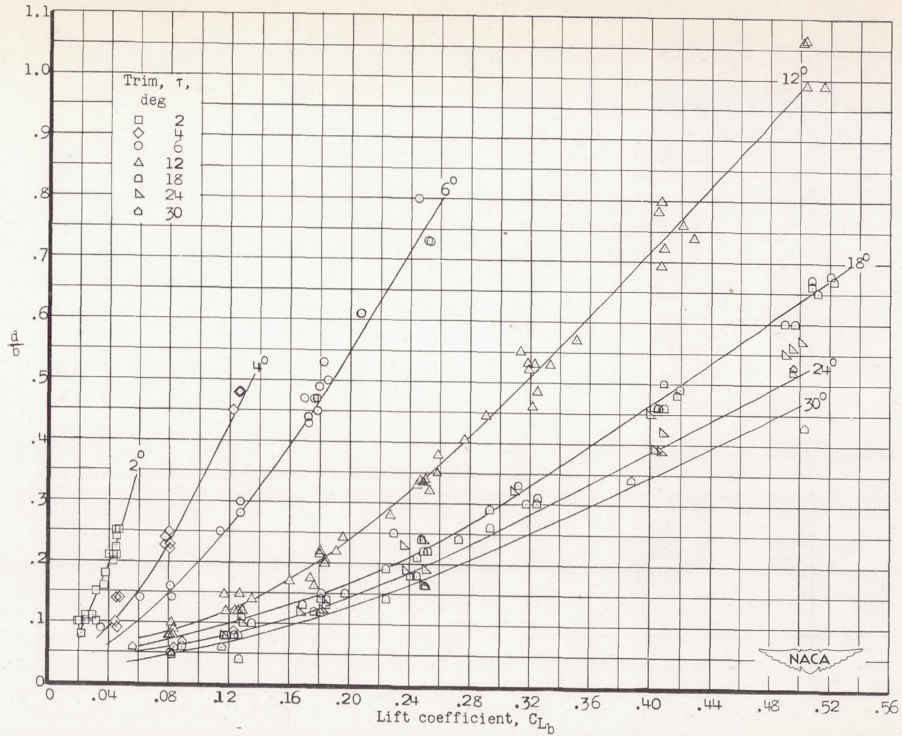
Figure 14.- Variation of d/b with C_{Lb} .
