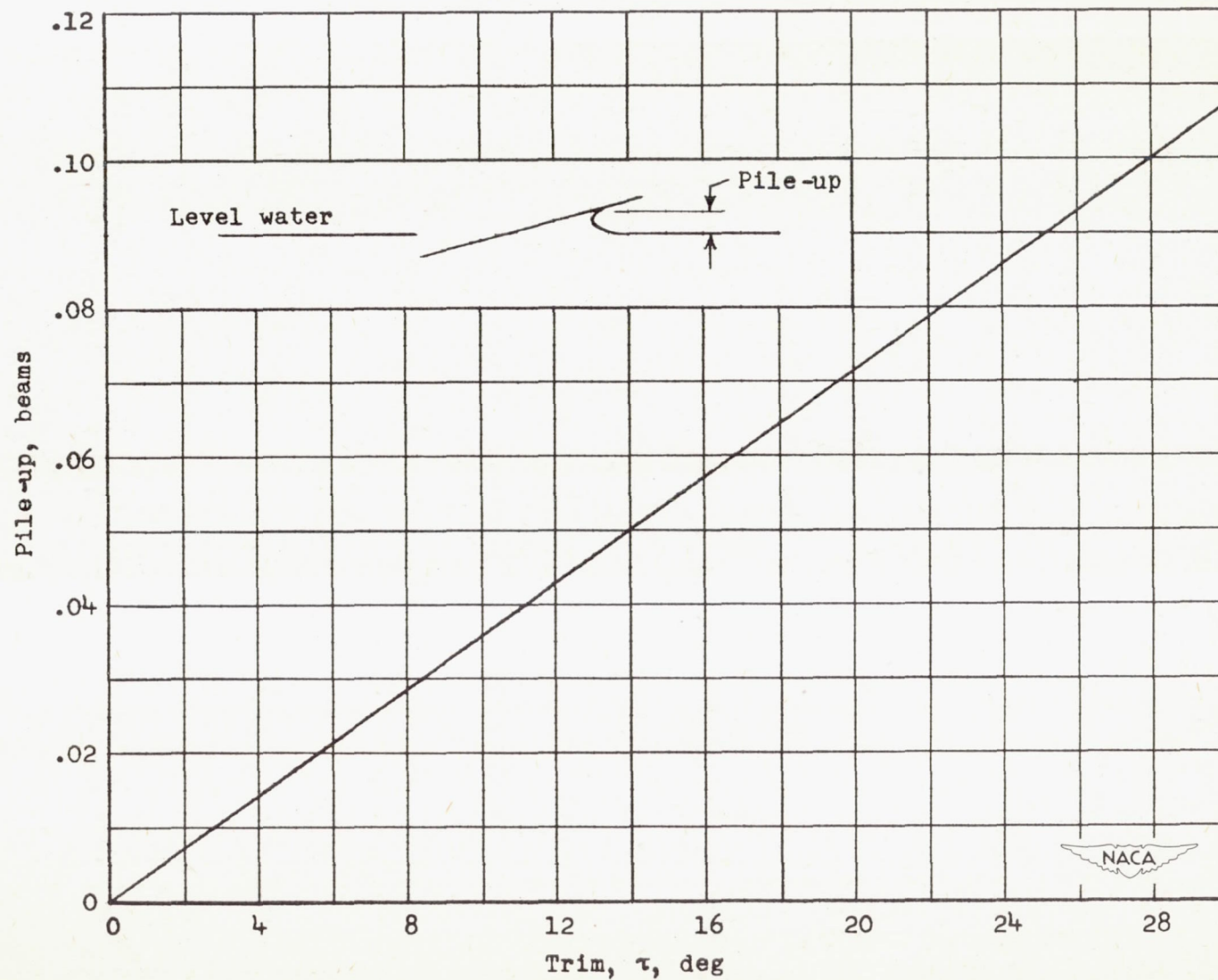
Figure 16.- Variation of pile-up with trim angle.
