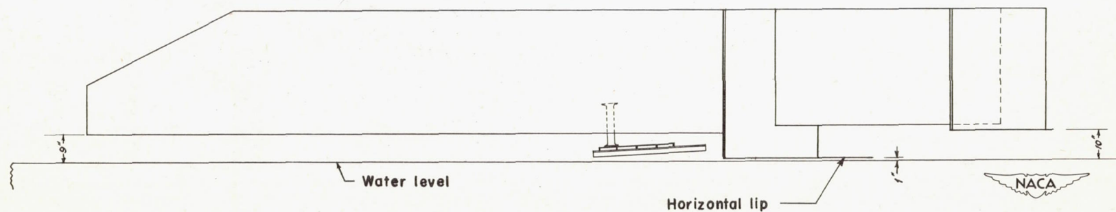
Figure 7.- Details of windscreen.
