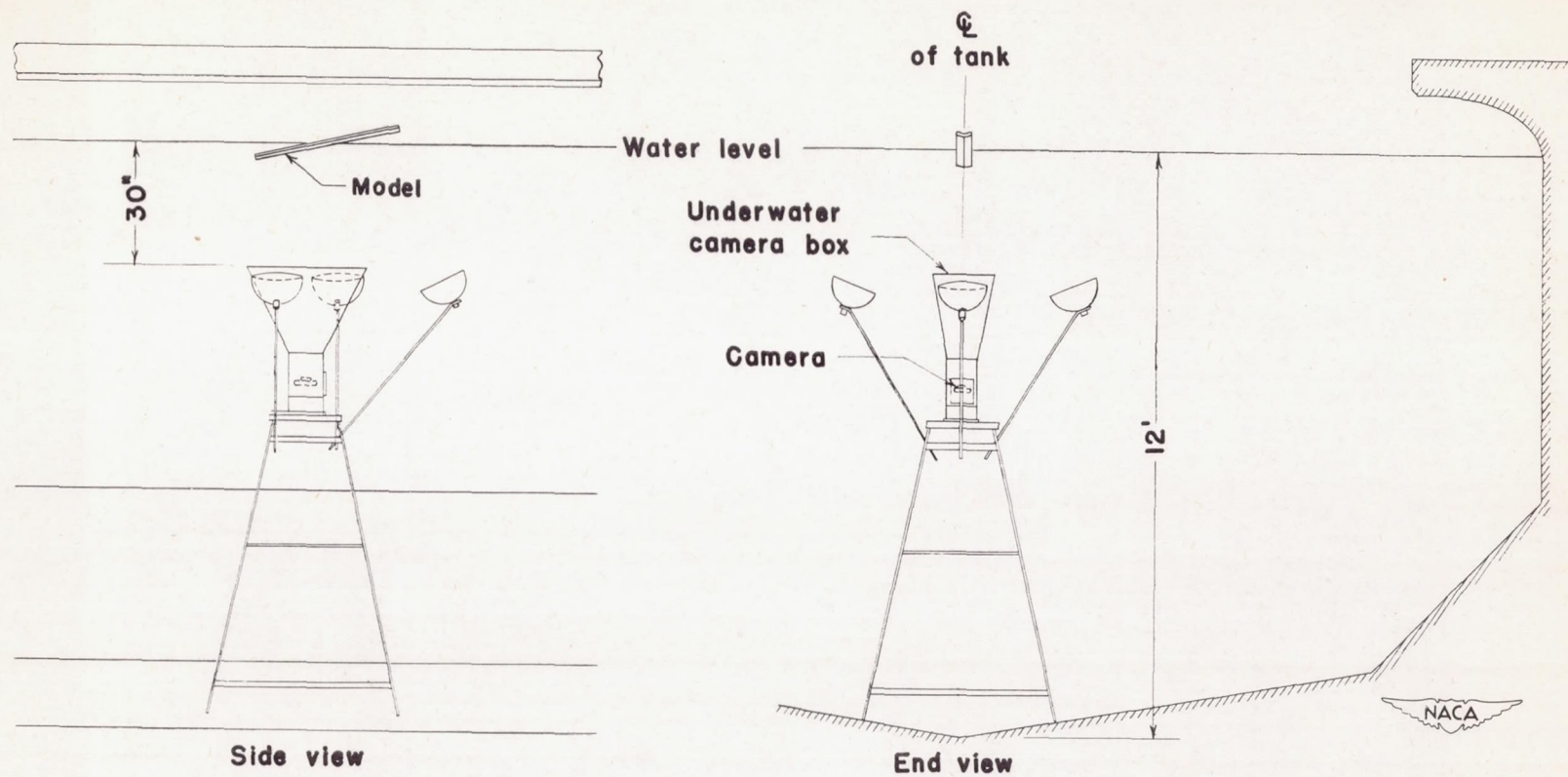
Figure 4.- Setup used for obtaining underwater photographs.
