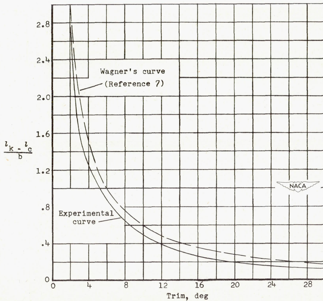
Figure 11.- Variation of \frac{l_k - l_c}{b} with trim.
