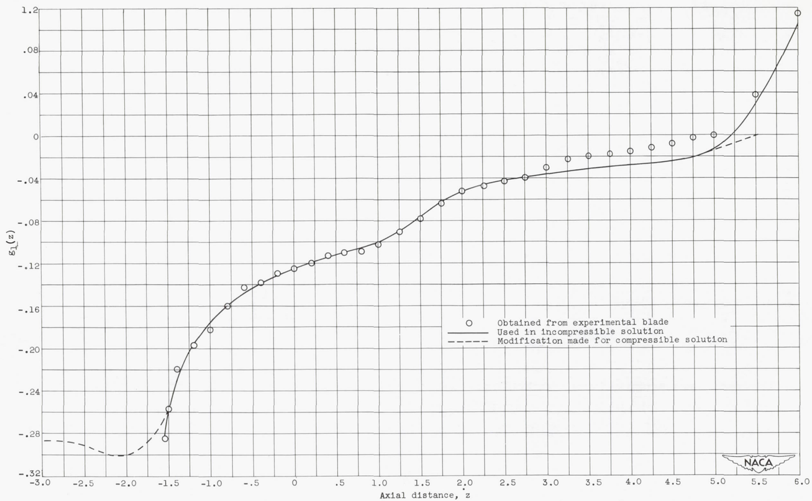
Figure 3. - Function g_1(z) .
