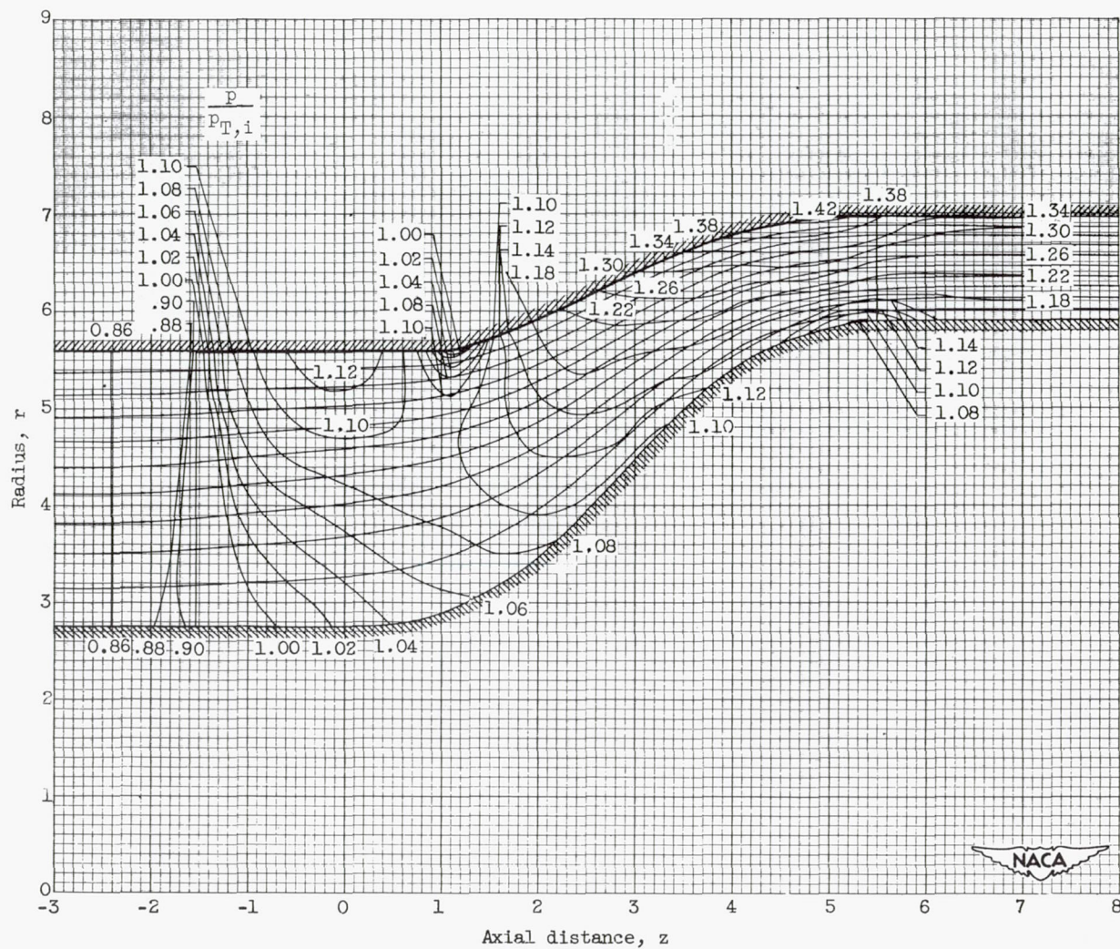
Figure 14.- Meridional projection of contours of constant pressure superposed on streamlines for compressible solution. (An overlay of this fig. is enclosed.)
