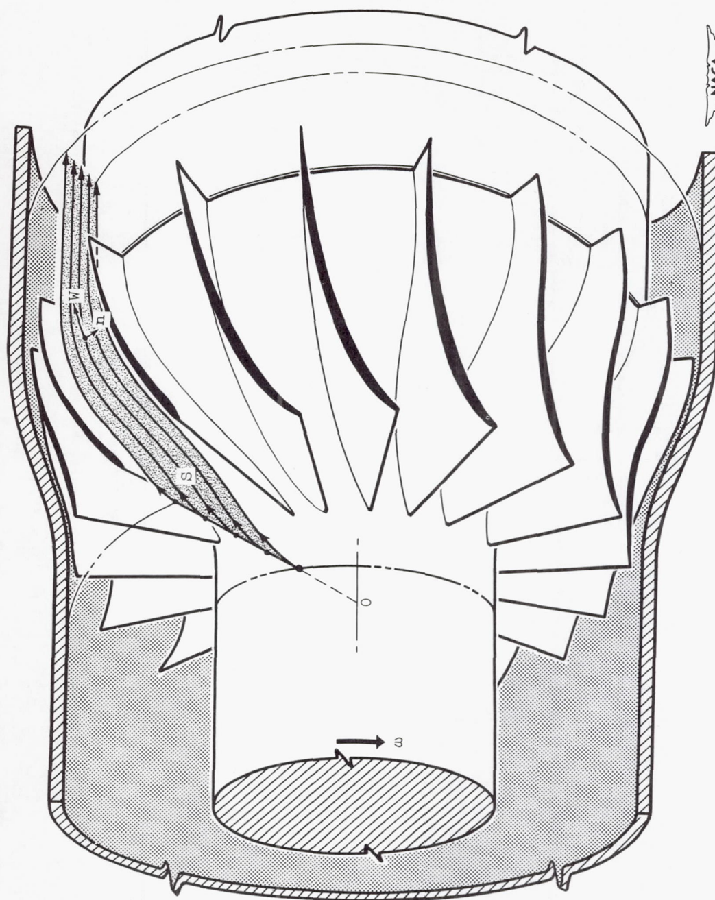
Figure 1. - Mean stream surface S.
