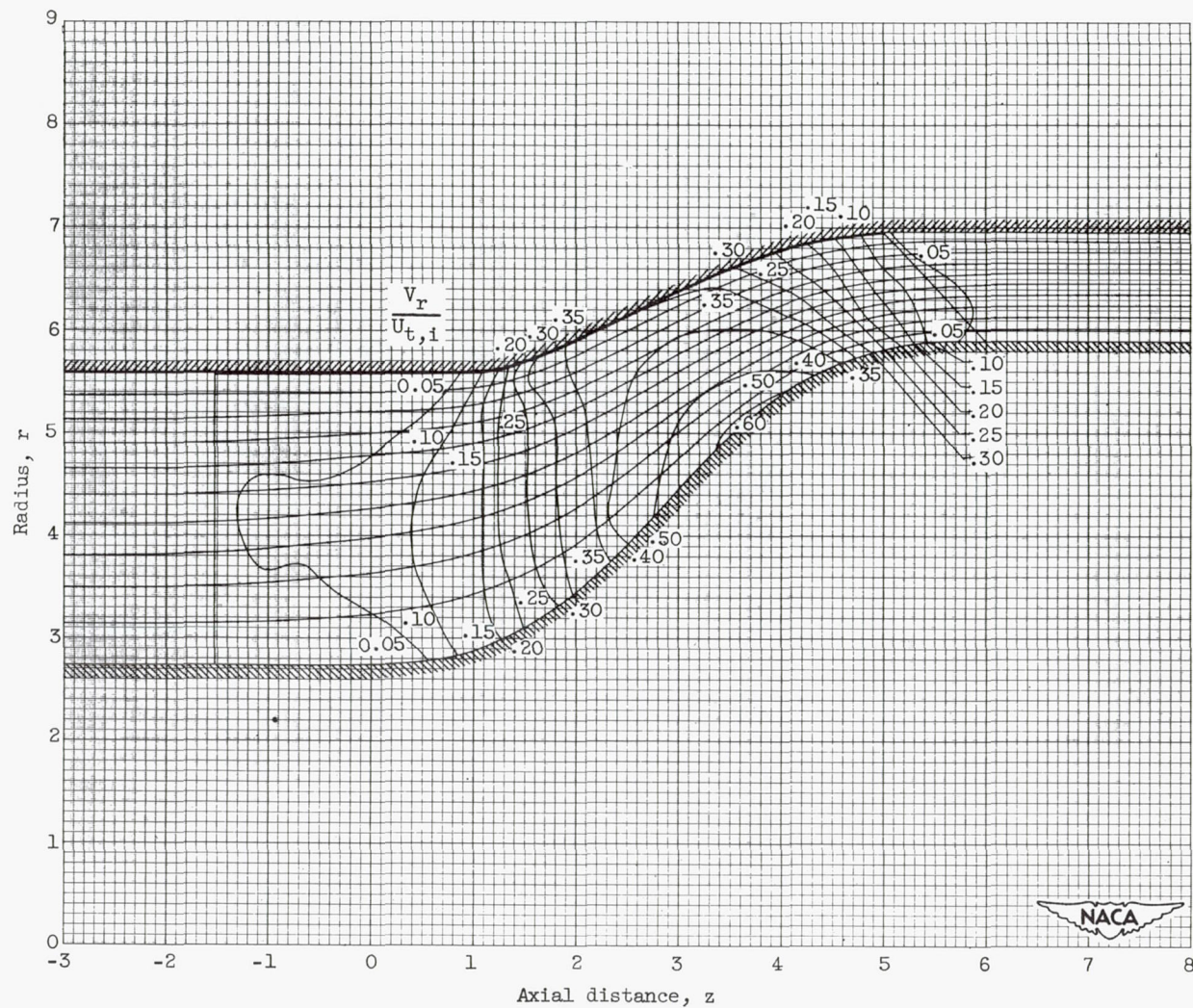
(b) Radial component.
