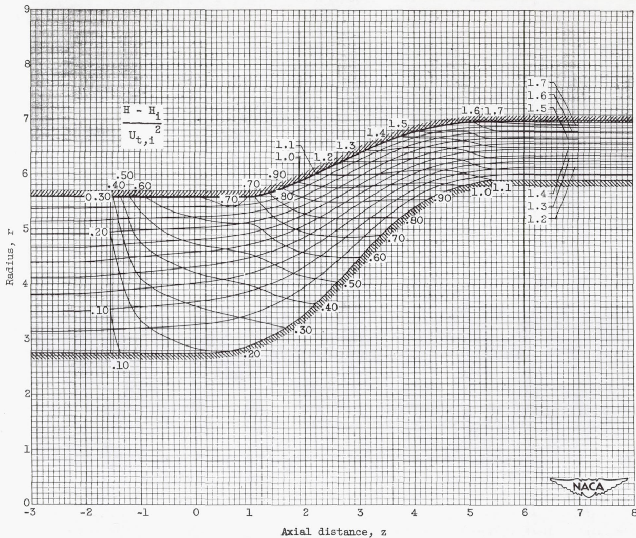
Figure 13.- Meridional projection of contours of constant total enthalpy superposed on streamlines for compressible solution. (An overlay of this fig. is enclosed.)
