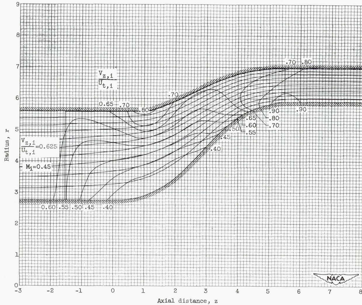
(a) Axial component.
