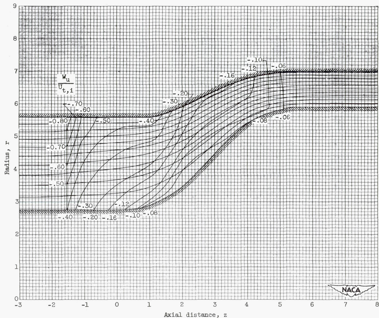
(c) Tangential component.
