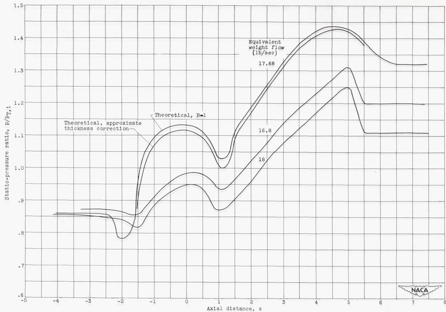
Figure 17. - Comparison of theoretical and experimental variation of static pressure along casing wall for compressible solution. M_1 , 0.45; U_{t,e}/\theta , 987 feet per second.
