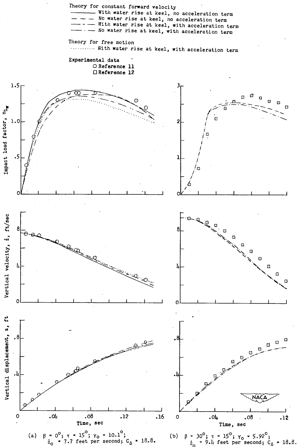
Figure 10.- Comparisons of theoretical and experimental impact time histories for 0^\circ and 30^\circ angles of dead rise.
