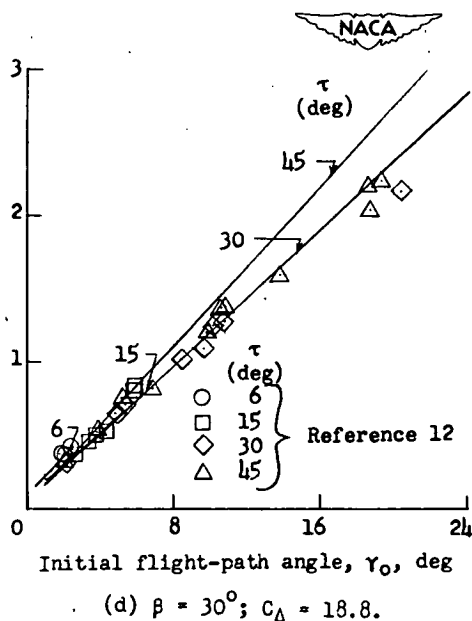
Figure 13.- Comparisons of theoretical and experimental maximum drafts for 0^\circ and 30^\circ angles of dead rise.
