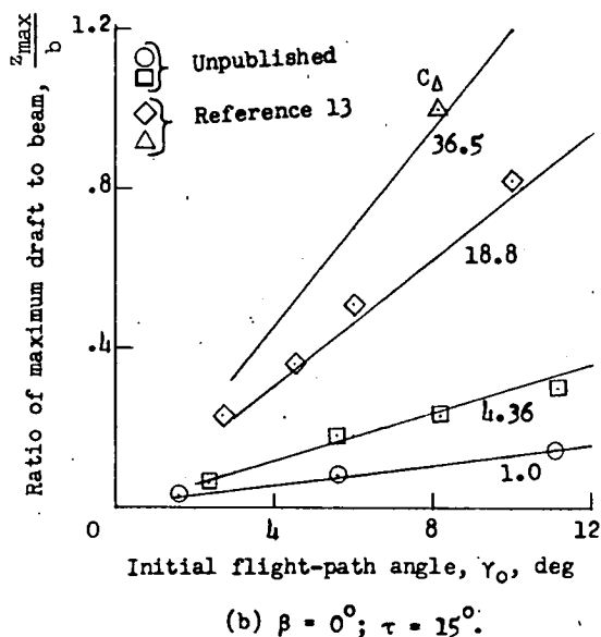
Figure 13.- Comparisons of theoretical and experimental maximum drafts for 0^\circ and 30^\circ angles of dead rise.
