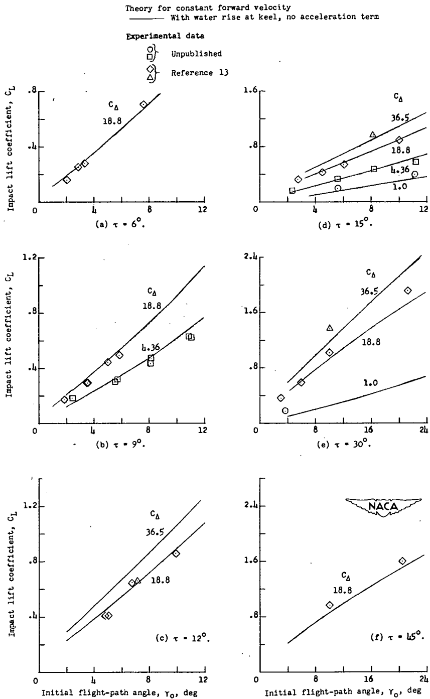
Figure 11.- Comparisons of theoretical and experimental impact lift coefficients C_L for a flat plate at various beam loadings.
