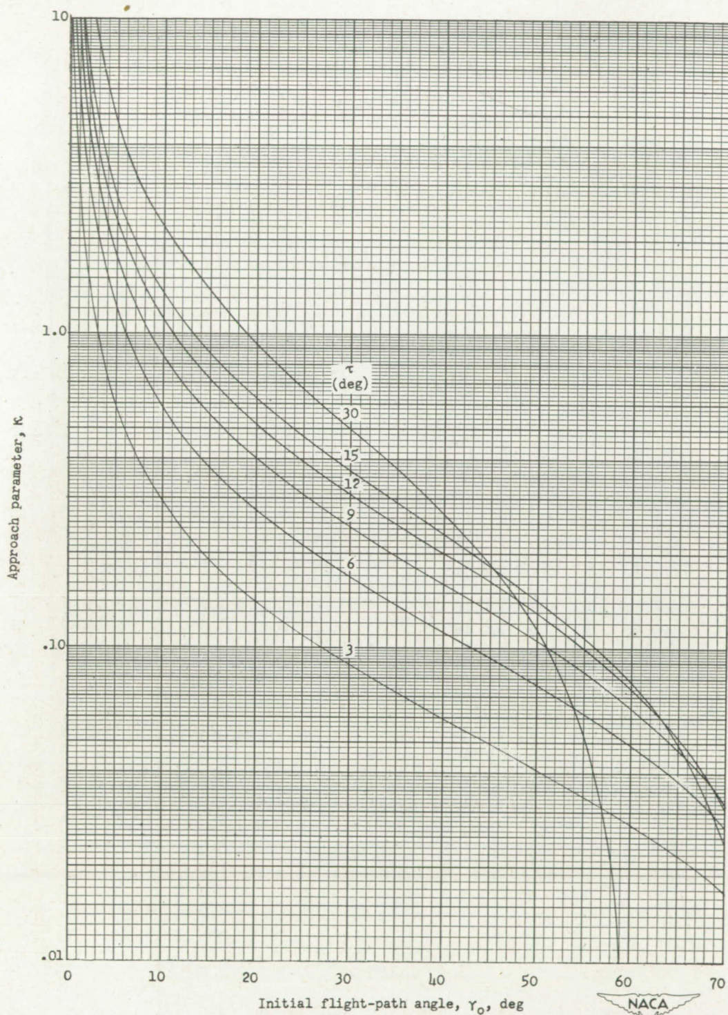
Figure 4.- Variation of approach parameter with trim and flight-path angle.
