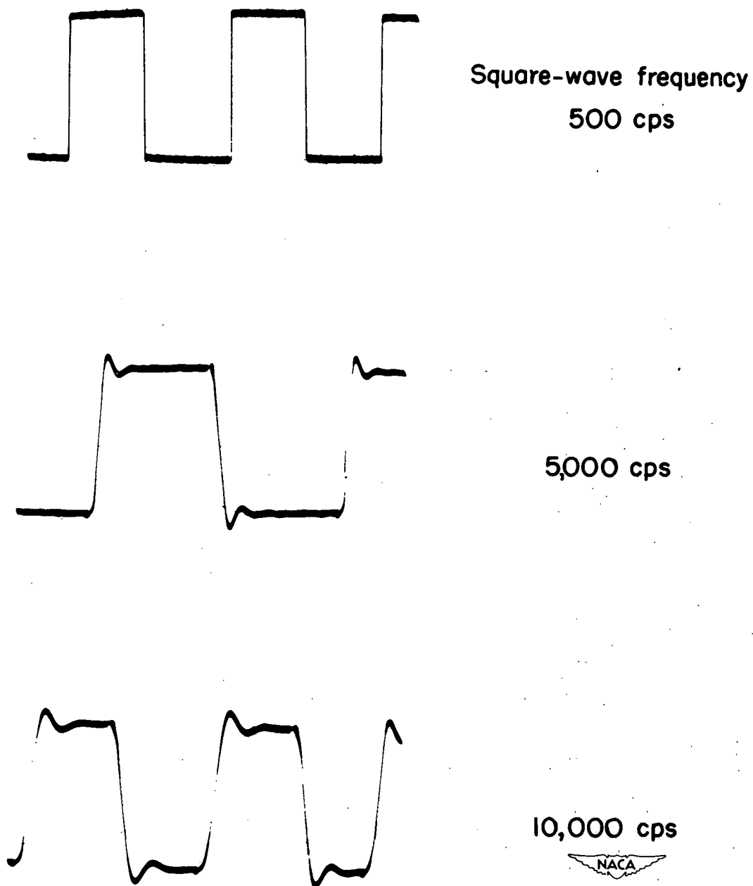
Figure 32.- Compensated output at various square-wave frequencies.
