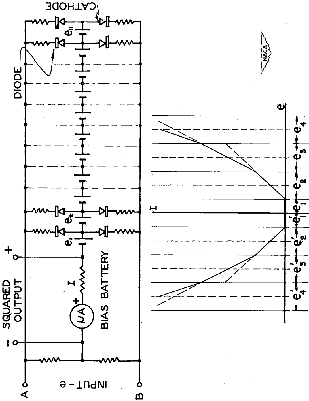
Figure 39.- Biased-diode square-law detector.
