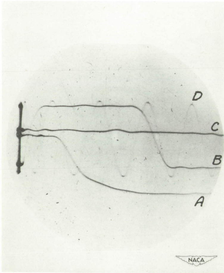
Figure 48.- Ultimate resolution of hot-wire method. A, shock-wave record - compensated; B, 10-kilocycle square-wave record - compensated; C, no signal; D, sine wave, 50-kilocycle, 75 millivolt root-mean-square value. Shock-wave indication rises sharply, then becomes less steep, probably because shock reflection from wedge-shaped holder becomes significant. R_w = 33.3 ohms; I = 13.56 milliamperes; time constant M = 0.205 millisecond.
