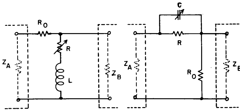
(a) Inductance resistance. (b) Capacitance resistance.
