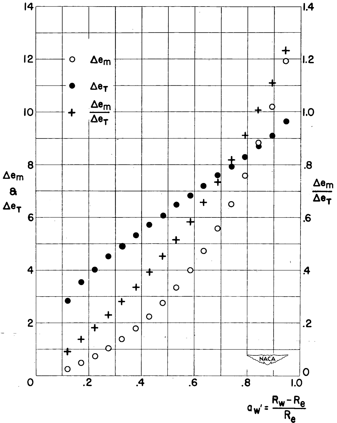
Figure 8.- Variation of fluctuation sensitivities with wire temperature in supersonic flow. Tungsten wire with 0.0015-inch diameter was used. Flow conditions: M = 1.73 , T_0 = 293^\circ K , and pressure at stagnation temperature was 40 centimeters of mercury.
