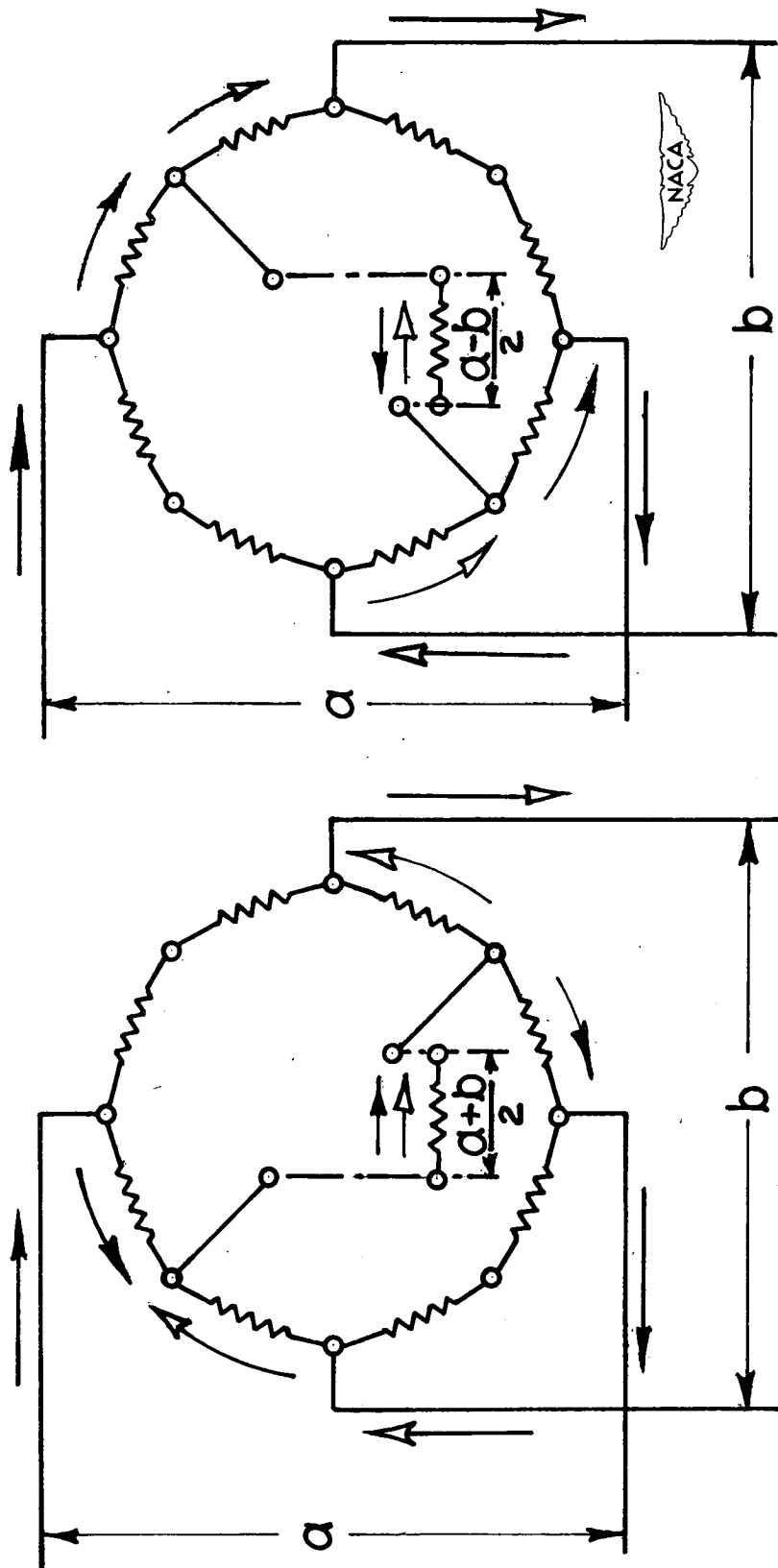
Figure 36.- Sum-difference circuit.
