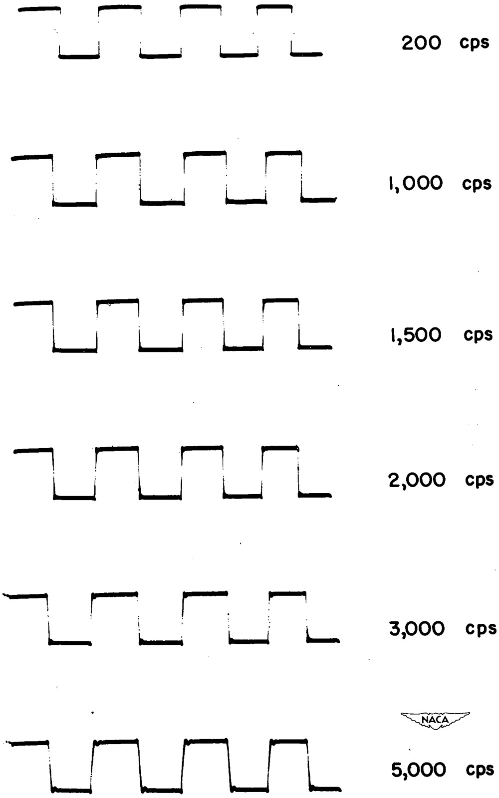
Figure 30.- Square-wave response of compensation.
