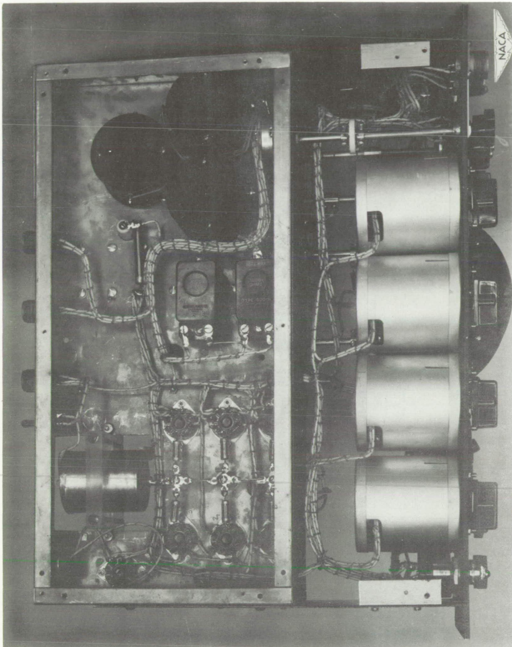
Figure 14.- Control unit, bottom view.
