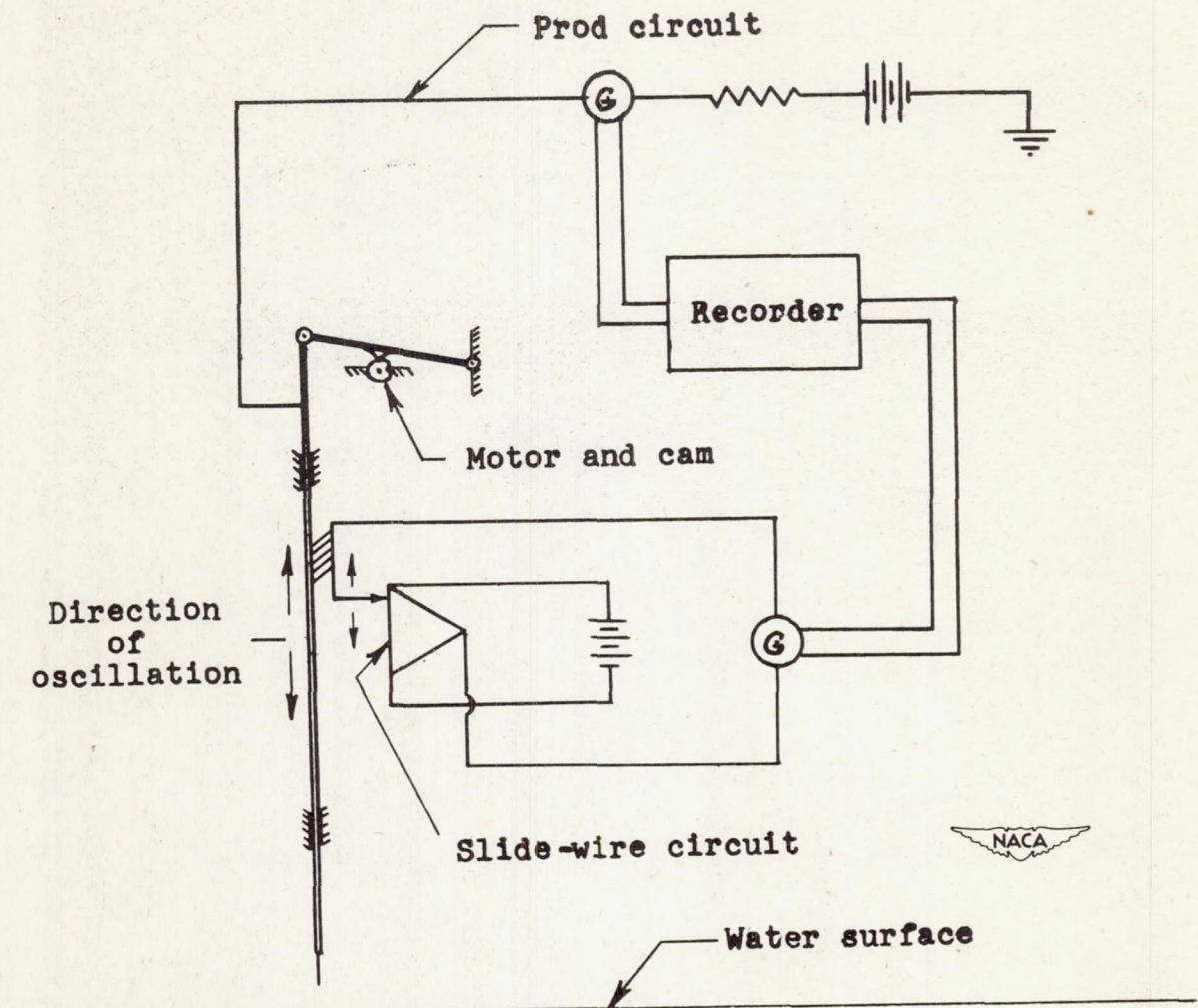
Figure 4.- Schematic drawing of water-level recorder.
