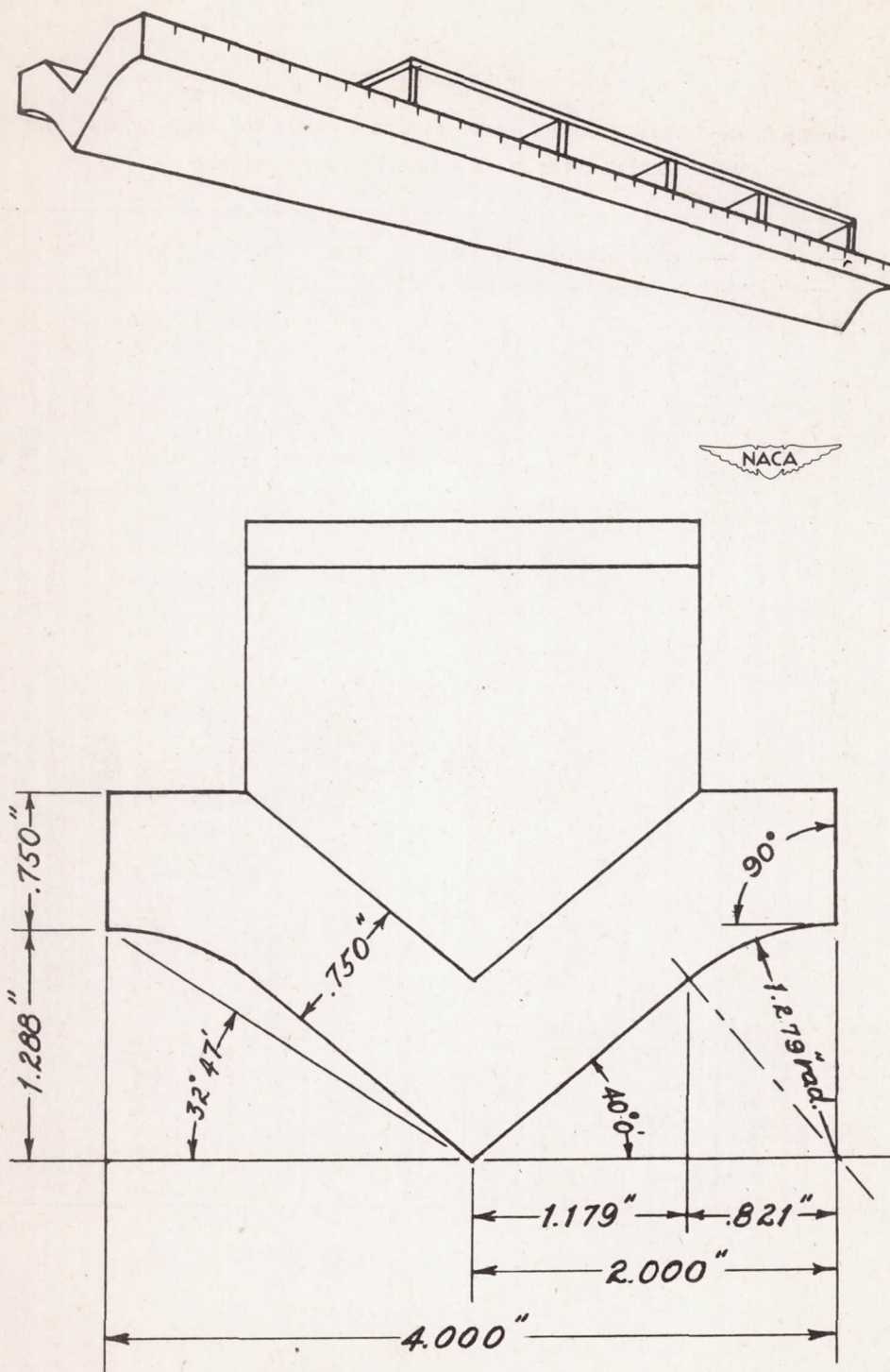
Figure 1.- Sketch and cross section of Langley tank model 277A.
