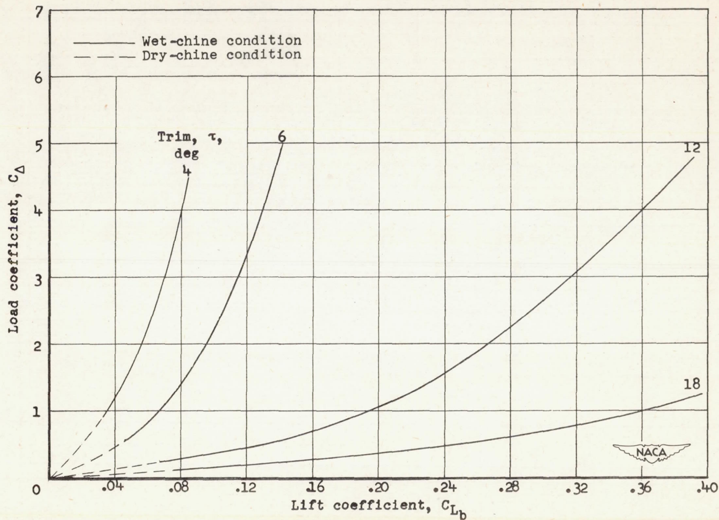
Figure 12.- Variation of minimum C_{\Delta} for pure planing, based on 20-percent buoyancy.
