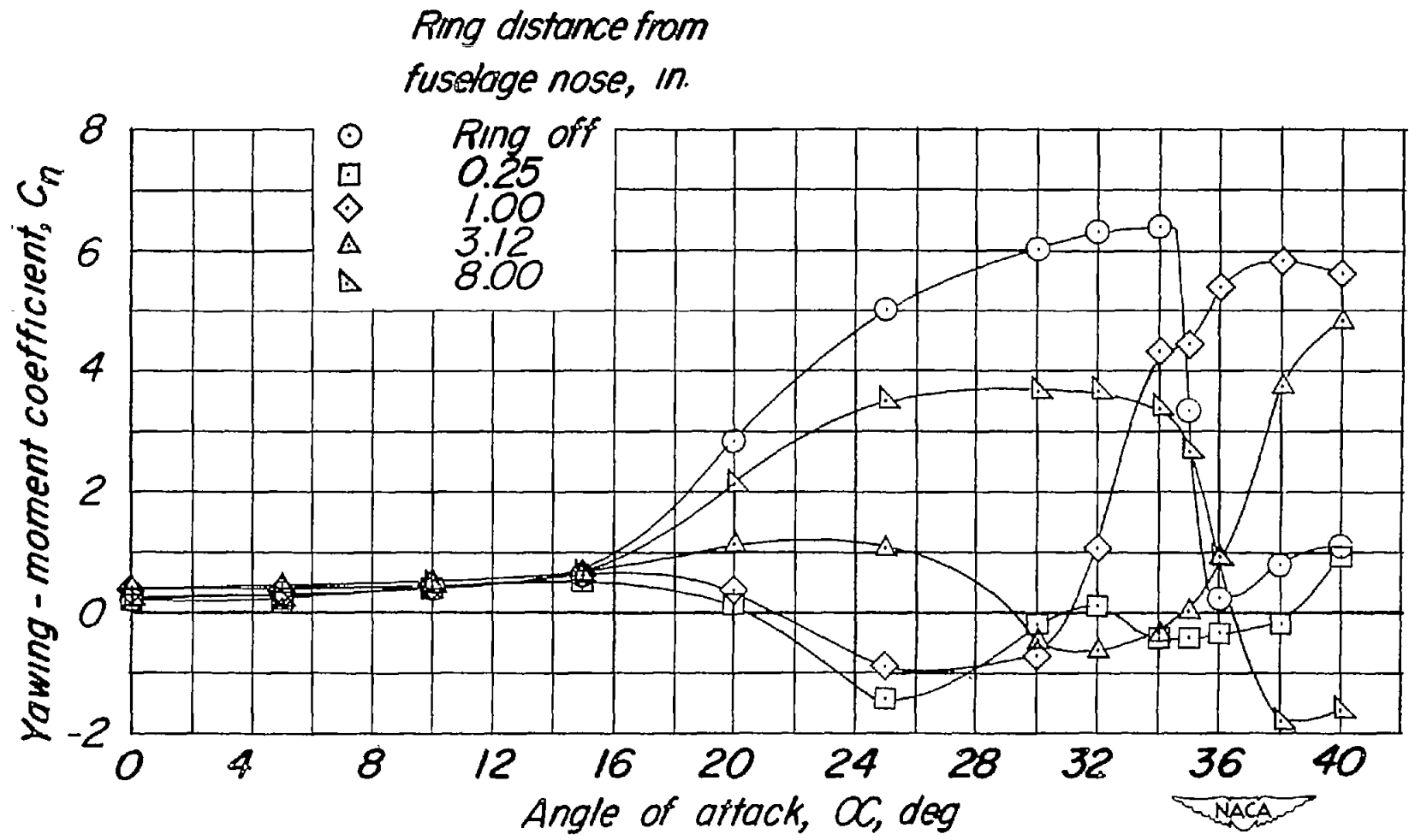
Figure 12.- Effect of location of \frac{1}{16} -inch-diameter ring on the variation of yawing-moment coefficient with angle of attack. \beta = 0^\circ ; q = 98.3 pounds per square foot.
