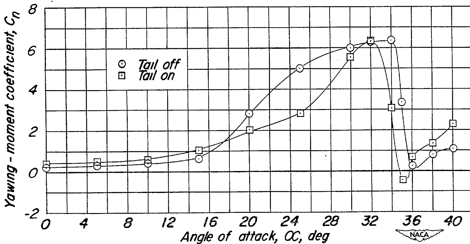
Figure 15.- Variation of the yawing-moment coefficient with angle of attack for the plain fuselage alone and for the plain fuselage with tail of aspect ratio 2. \beta = 0^\circ ; q = 98.3 pounds per square foot.
