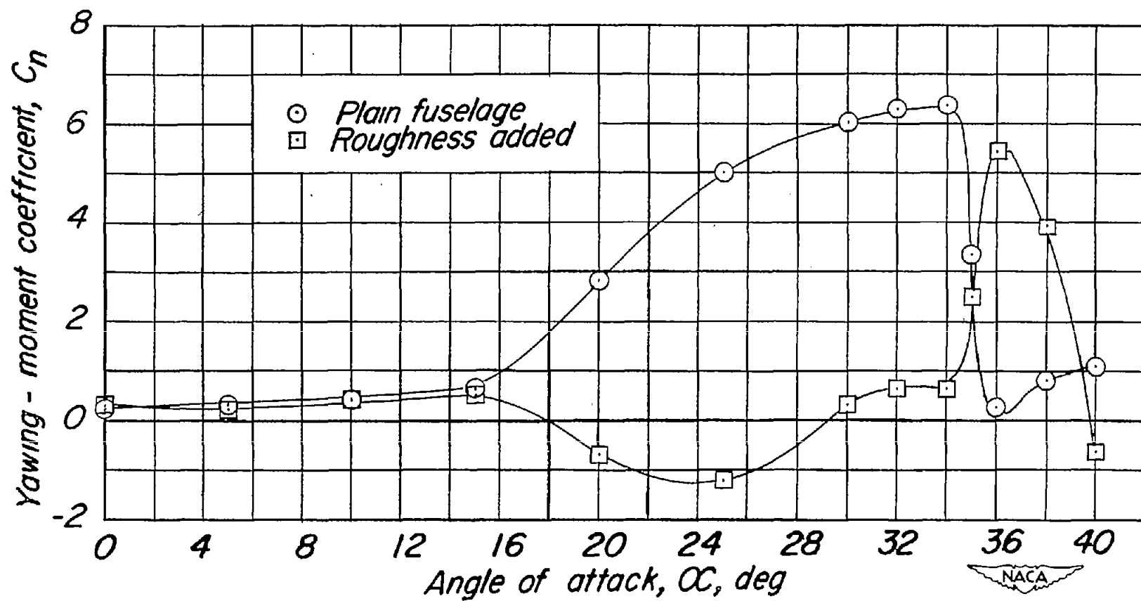
Figure 14.- Variation of the yawing-moment coefficient with angle of attack for the plain fuselage and for the fuselage with first 2 inches coated with carborundum grains. \beta = 0^\circ ; q = 98.3 pounds per square foot.
