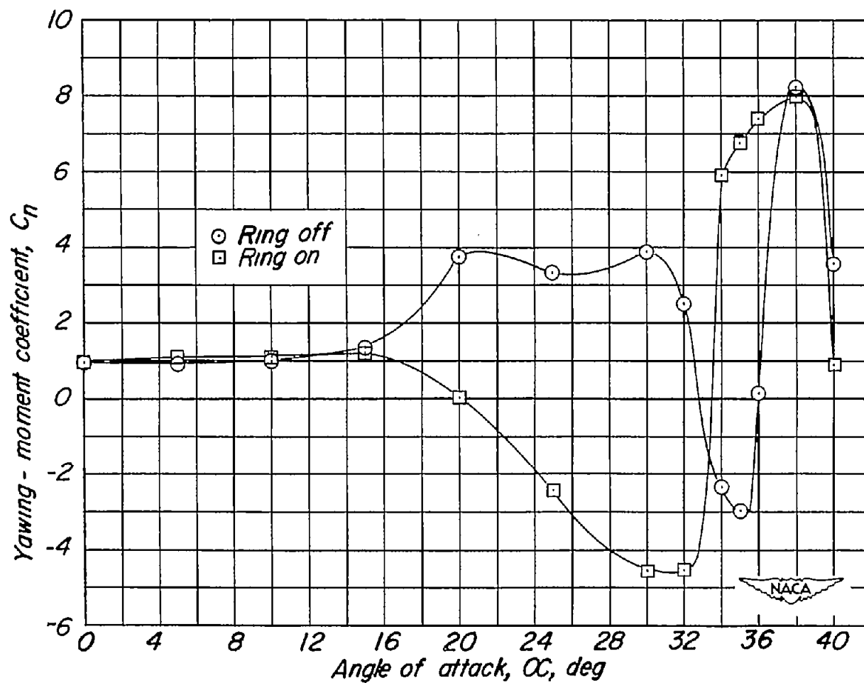
Figure 9.- Effect of small sideslip angle on the variation of the yawing-moment coefficient with angle of attack for the plain fuselage and for the fuselage with \frac{1}{16} -inch-diameter ring located 1 inch from the nose. \beta = -6^\circ ; q = 98.3 pounds per square foot.
