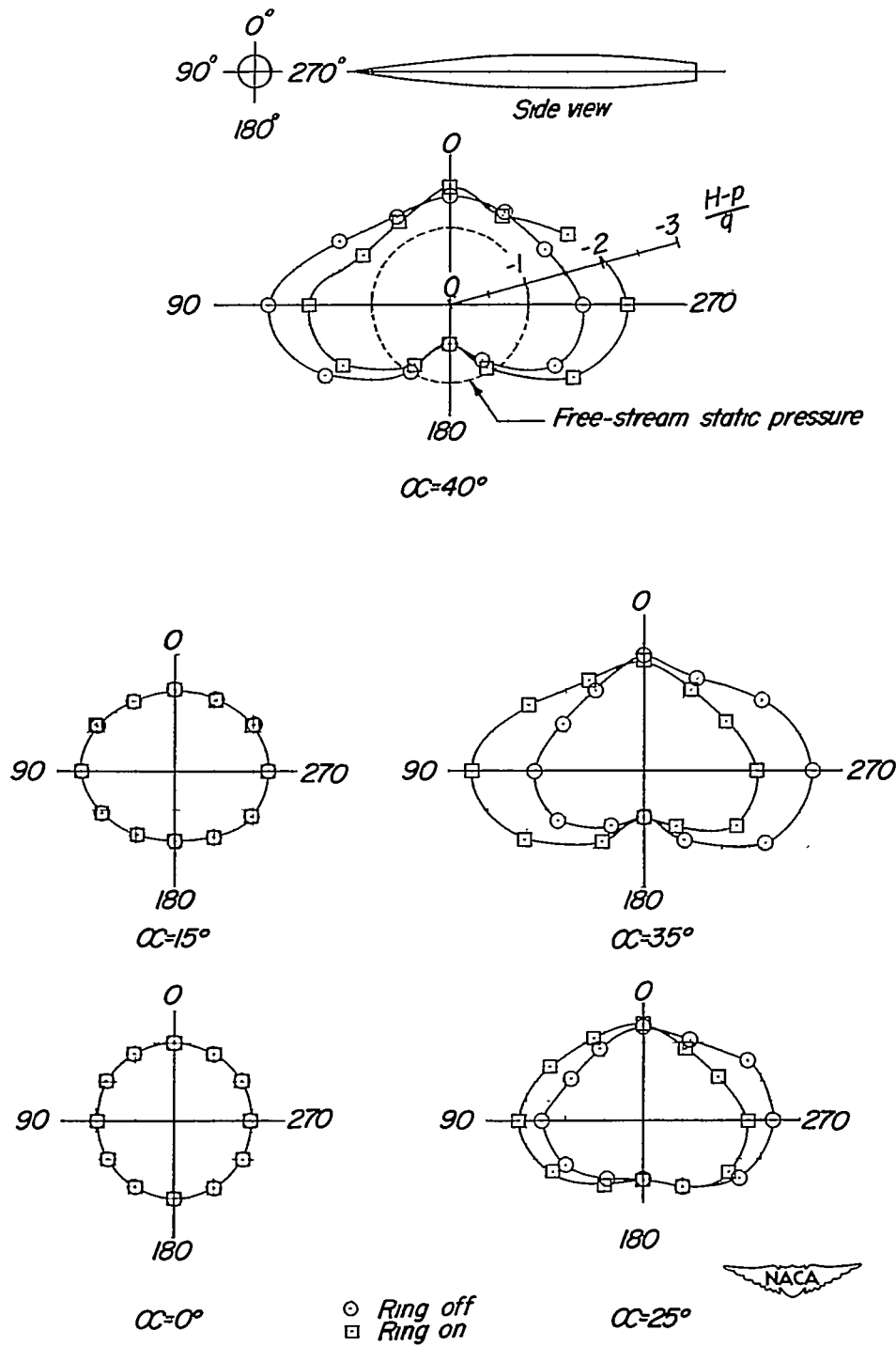
Figure 7.- Comparison of the peripheral pressure distributions 17\frac{1}{2} inches from the nose for the plain fuselage and for the fuselage with ring located 1 inch from the nose. \beta = 0^\circ ; q = 64.3 pounds per square foot.
