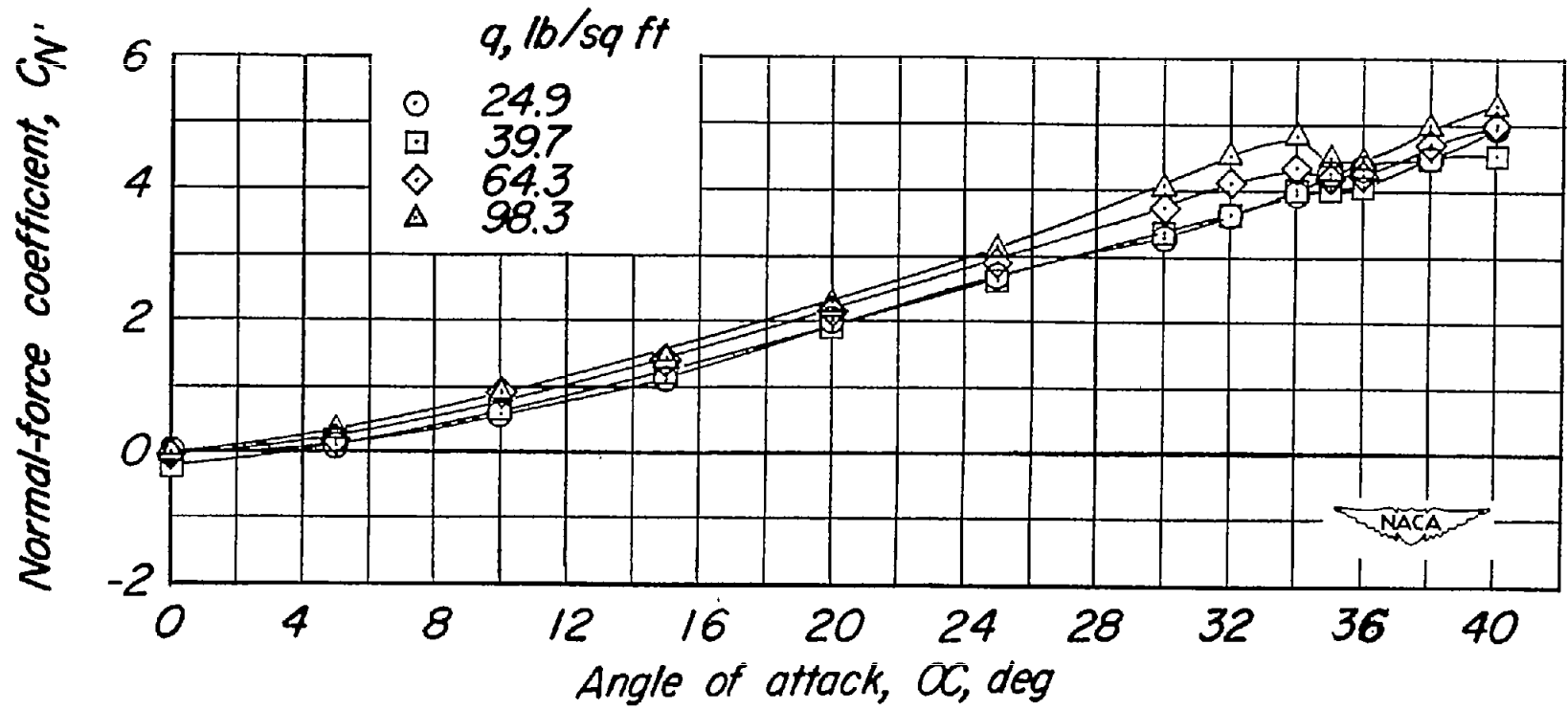
Figure 4.- Effect of dynamic pressure on the variation of fuselage normal-force coefficient with angle of attack. \beta = 0^\circ .
