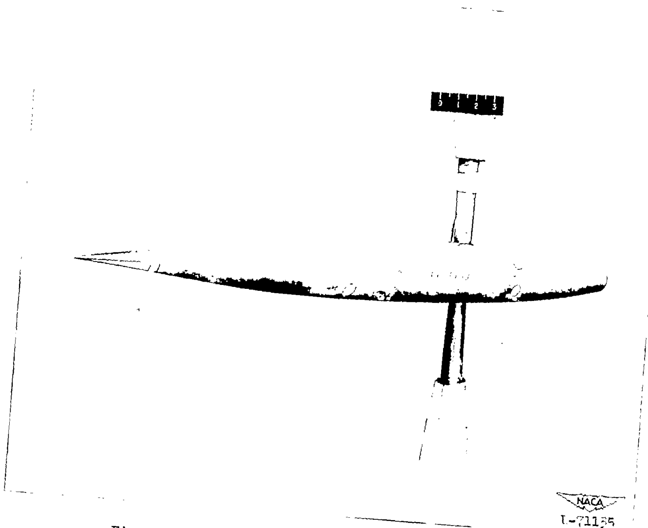
Figure 3.- Model mounted in Langley stability tunnel.
