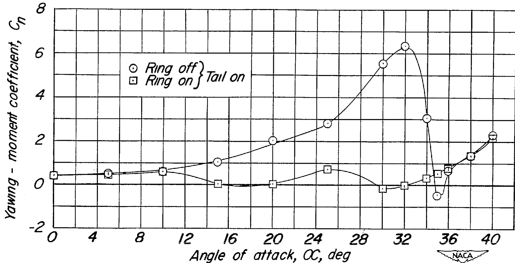
Figure 16.- Variation of the yawing-moment coefficient with angle of attack for the plain fuselage with tail and for the ringed fuselage with tail ( \frac{1}{16} -inch-diameter ring 1 inch from nose). \beta = 0^\circ ; q = 98.3 pounds per square foot.
