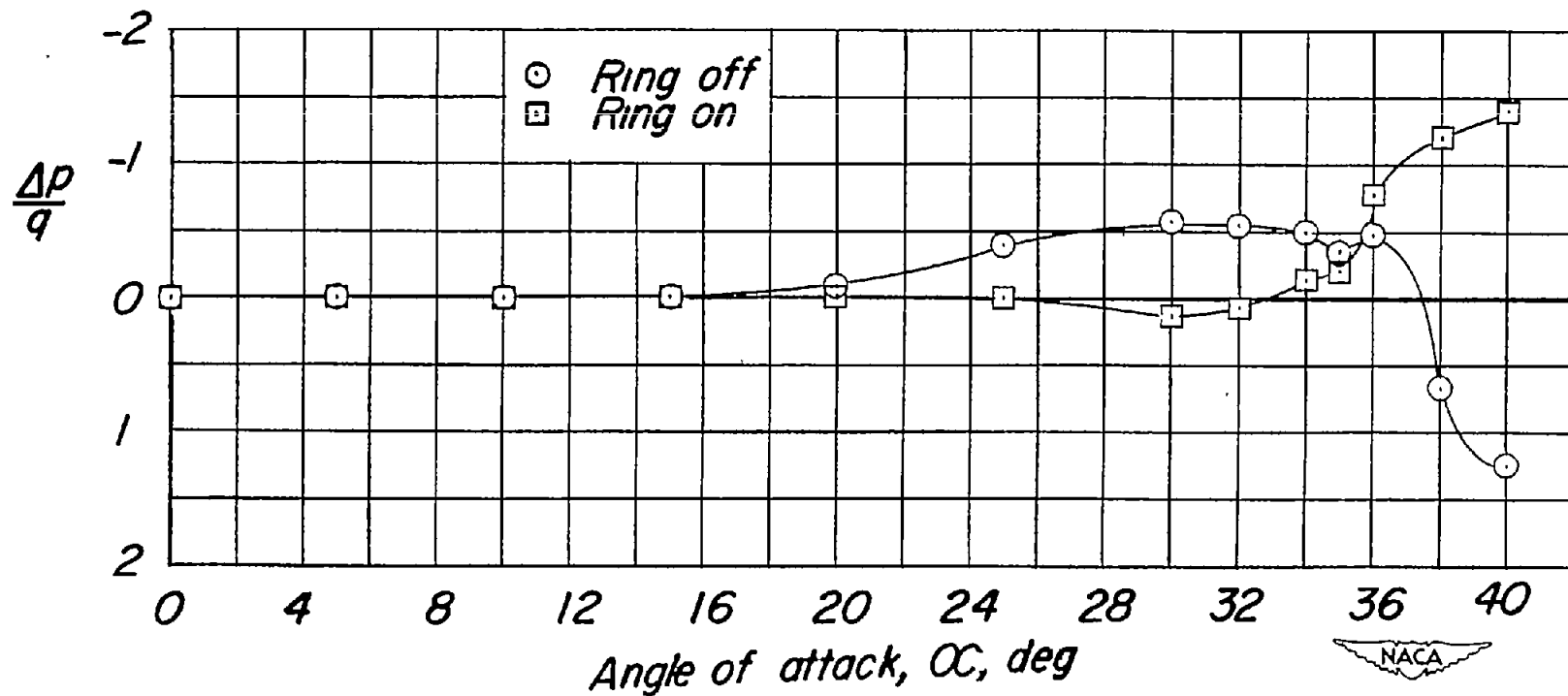
Figure 8.- Variation with angle of attack of the pressure difference measured by yaw orifices for the plain fuselage and for the fuselage with \frac{1}{16} -inch-diameter ring located 1 inch from the nose. \beta = 0^\circ ; q = 98.3 pounds per square foot.
