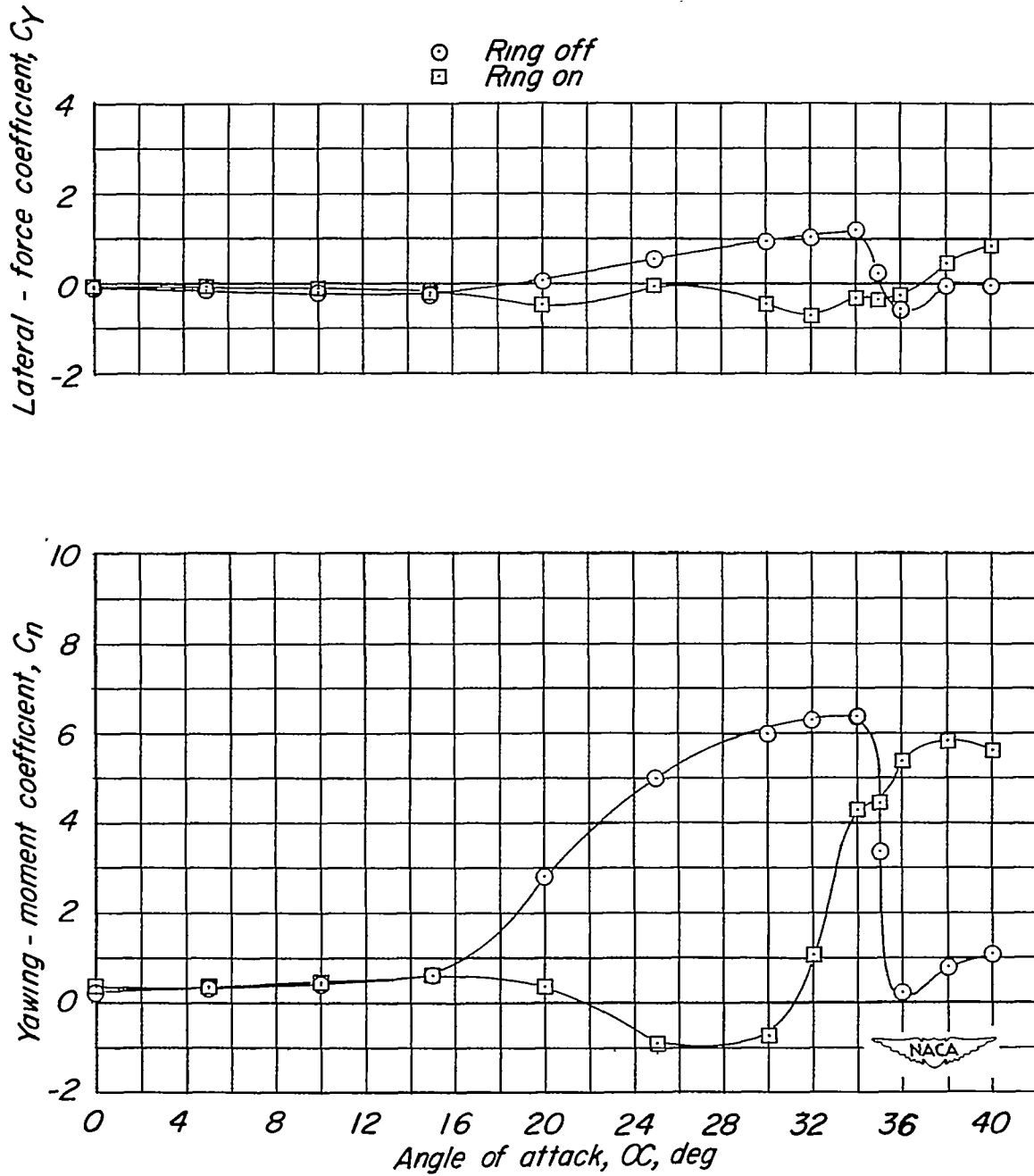
Figure 6.- Variation with angle of attack of the yawing-moment and lateral-force coefficients of the plain fuselage and the fuselage with \frac{1}{16} -inch-diameter ring located 1 inch from the nose. \beta = 0^\circ ; q = 98.3 pounds per square foot.
