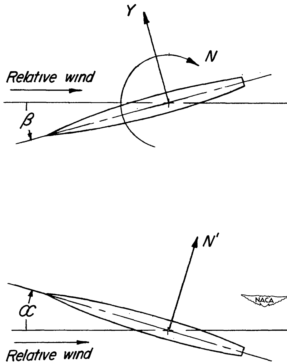
Figure 1.- System of axes used. Arrows indicate positive directions of forces, moments, and angular displacements.
