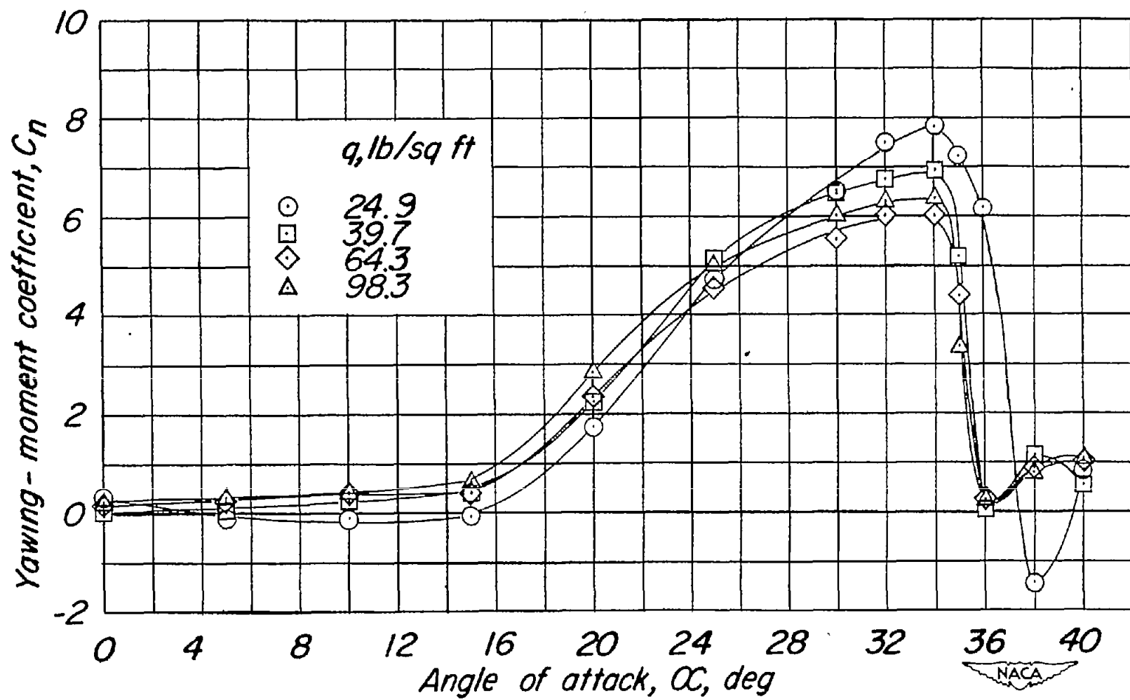
Figure 5.- Effect of dynamic pressure on the variation of fuselage yawing-moment coefficient with angle of attack. \beta = 0^\circ .
