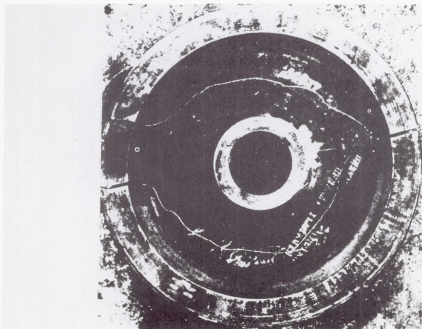
(b) Wheel fracture produced in the laboratory.
