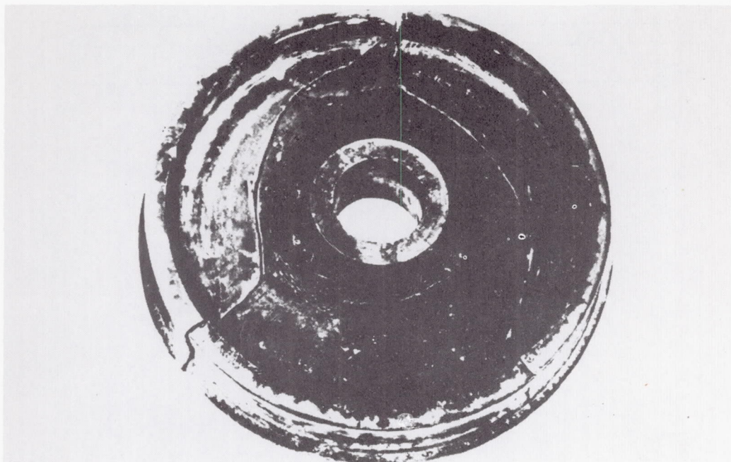
(a) Wheel fracture produced in service.
