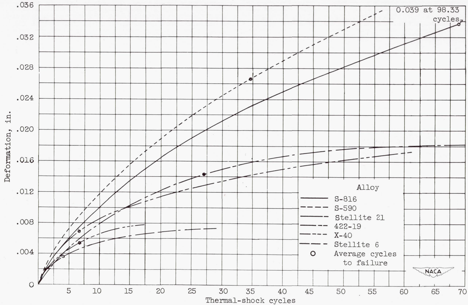
Figure 17. - Composite curves for progressive deformation of six alloys.
