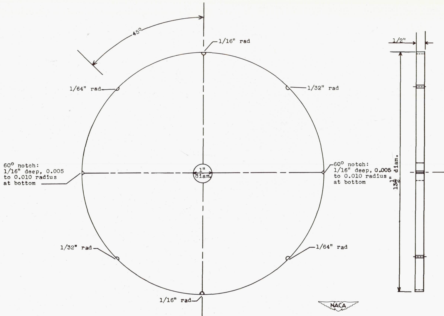
Figure 32. - Notched-rim disk used in thermal stress investigation.
