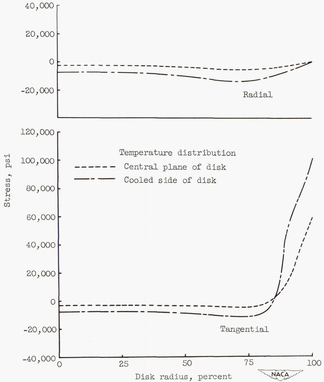
Figure 26. - Residual stresses after operation.
