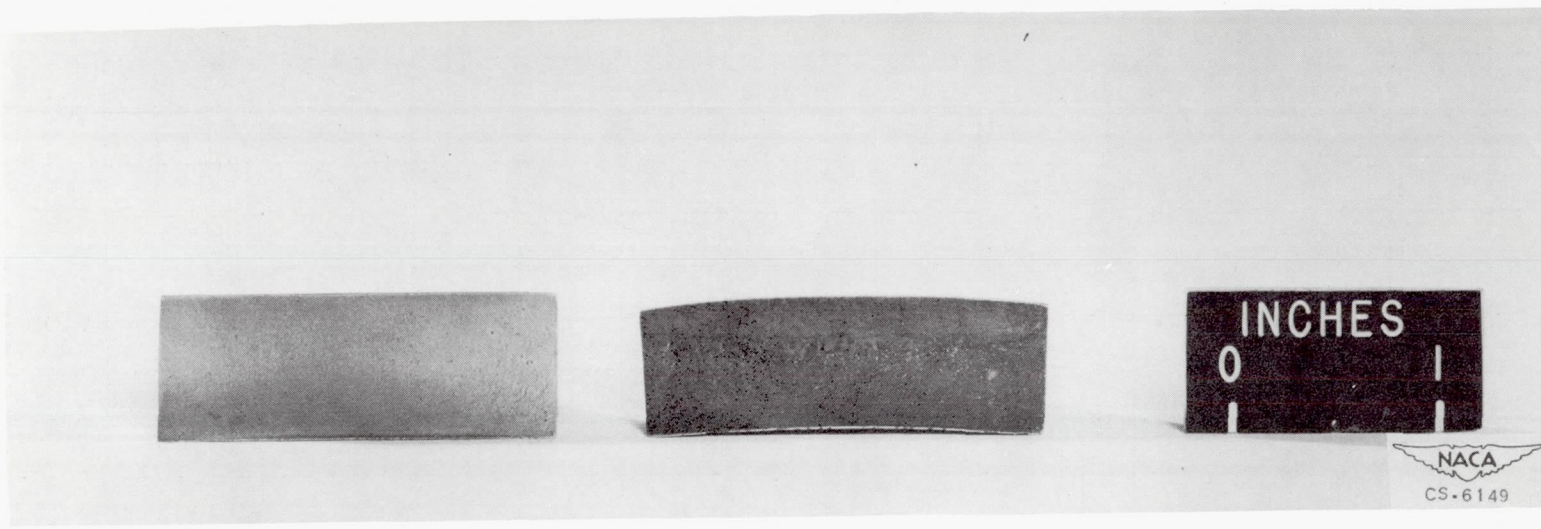
Figure 18. - Specimens before and after repeated thermal-shock cycles. Note curvature produced by thermal stress.
