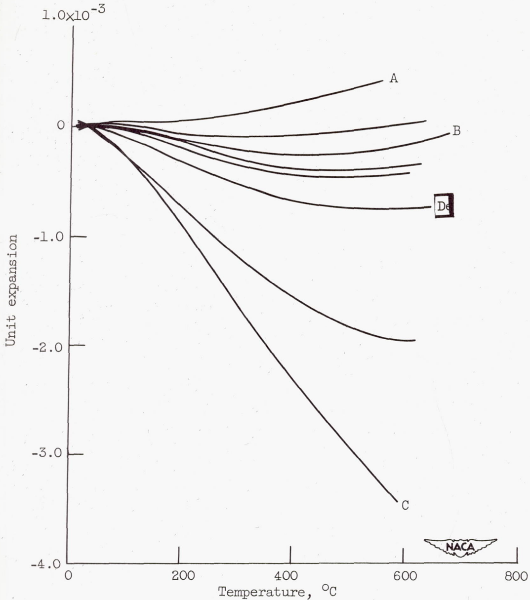
Figure 53. - Typical thermal expansion curves of various Stupalith compositions.
