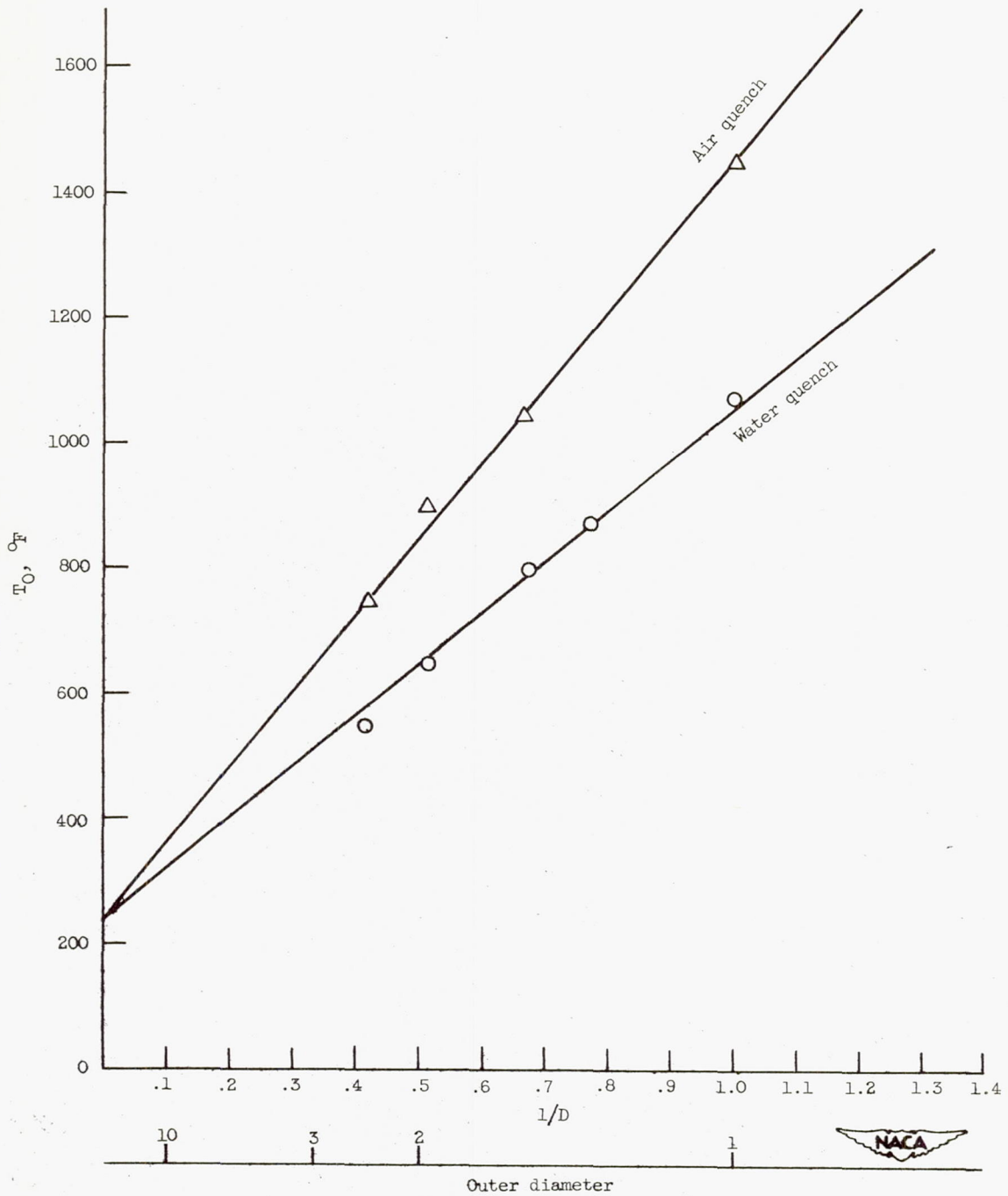
Figure 38. - Size effect in thermal shock of steatite.
