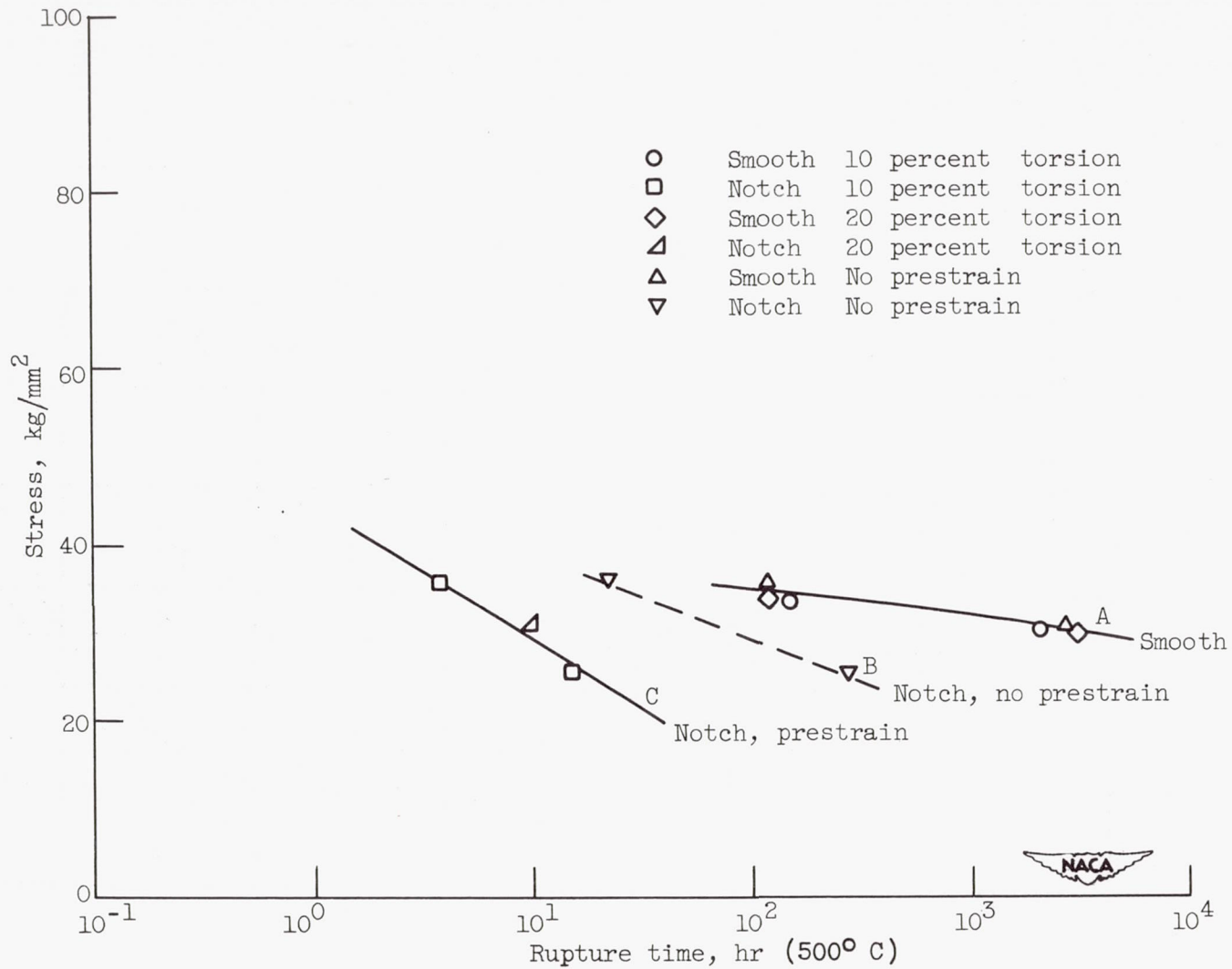
Figure 13. - Effect of working on strength of steel.
