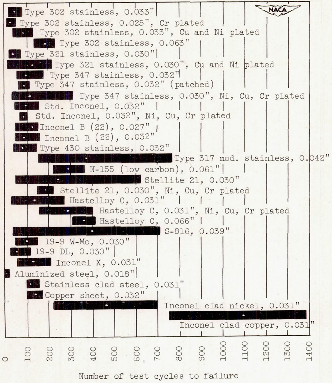
Figure 52. - Summarized results of flame impingement test.
