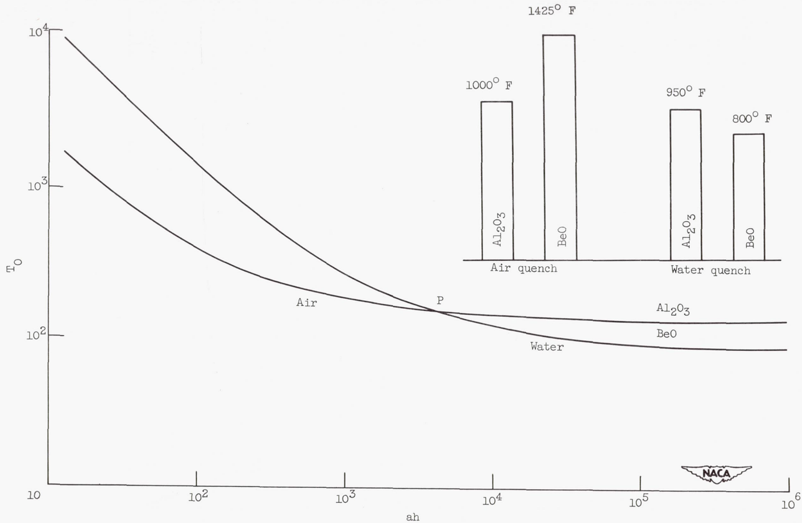
Figure 7. - Thermal shock tests of BeO and Al_2O_3 .
