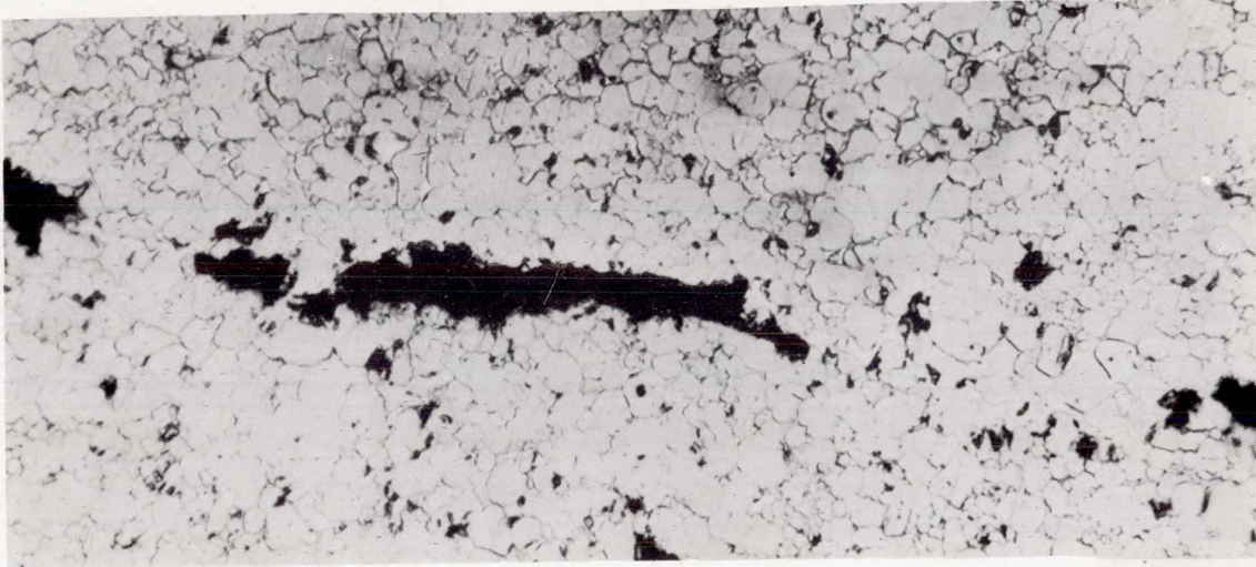
Figure 50. - Thermal shock crack in 11.8 weight percent (7.8 volume percent) iron plus titanium carbide ceramal.
