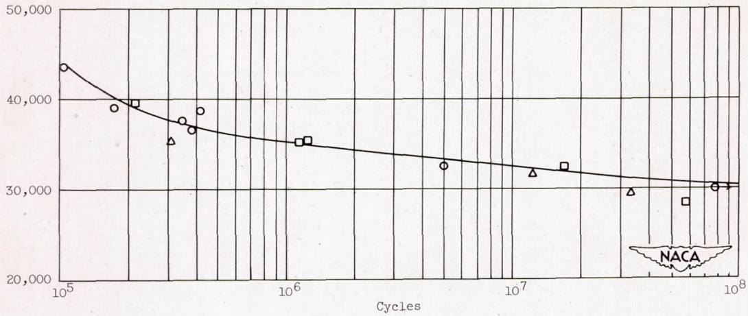
Figure 49. - Effect of surface treatment on fatigue properties of low-carbon N-155.
