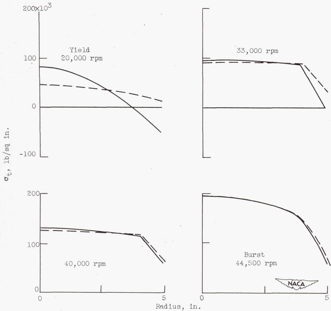
Figure 29. - Comparison of total tangential stress with centrifugal tangential stress.
