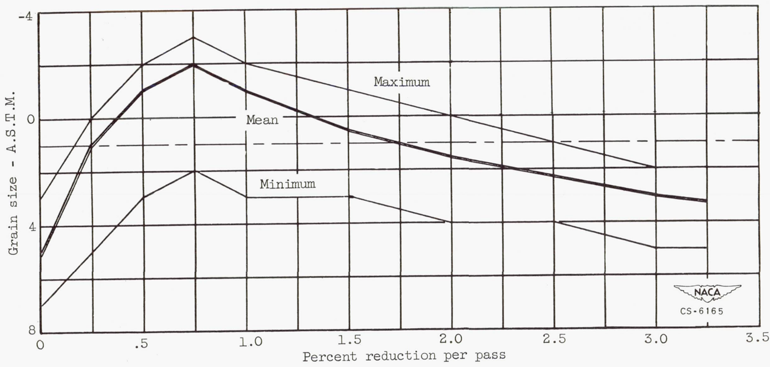
Figure 14. --Effect of prior critical deformation on grain size of S-816 alloy.
