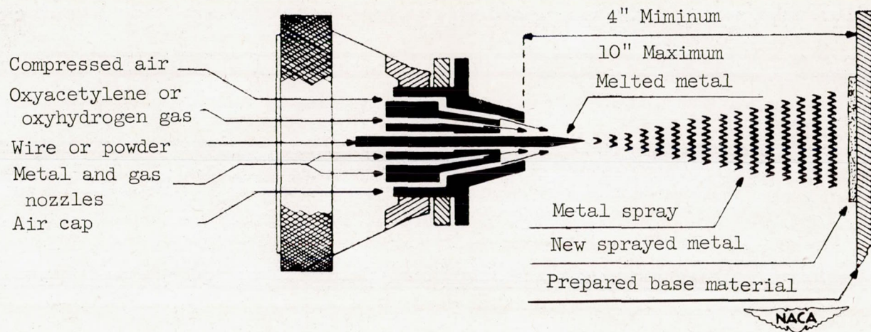
Figure 46. - Schematic drawing showing action of wire-type metal spray gun.
