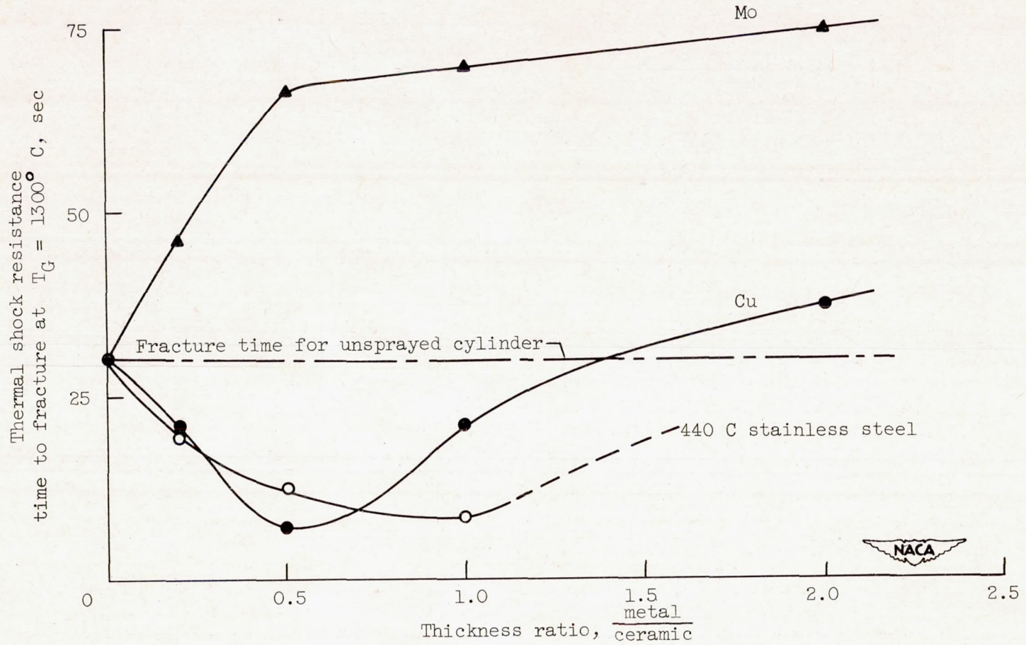
Figure 48. - Effect of metal/ceramic thickness ratio on thermal shock resistance of metal-sprayed cylinders.
