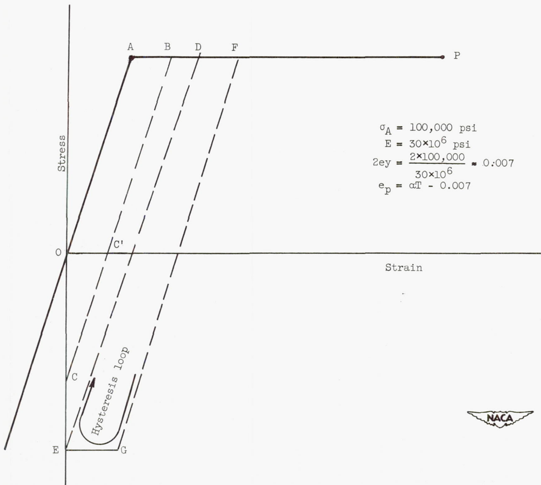
Figure 10. - Cyclic plastic strain in constrained bar due to heating and cooling.
