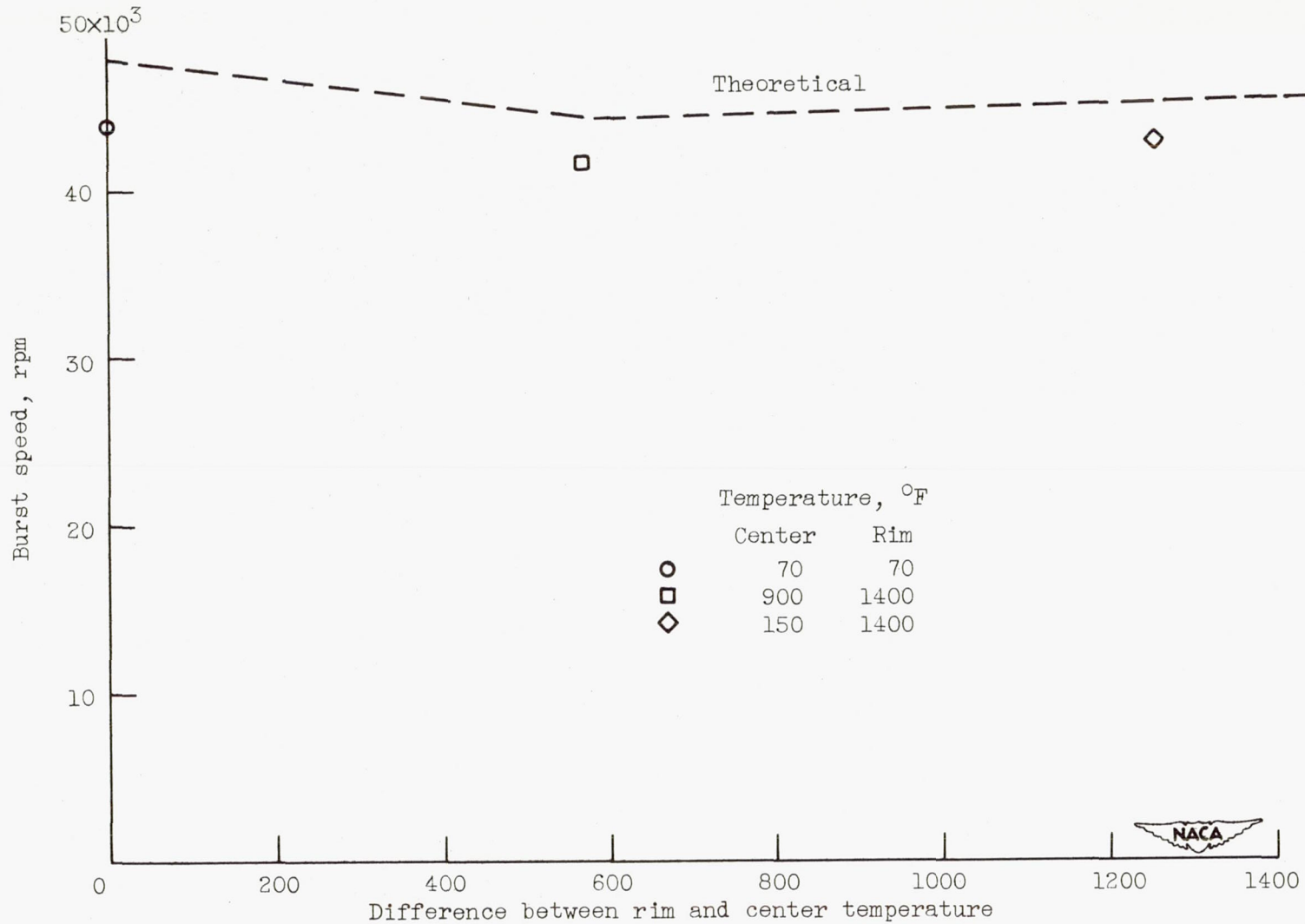
Figure 30. - Burst speeds of disks with temperature gradient.
