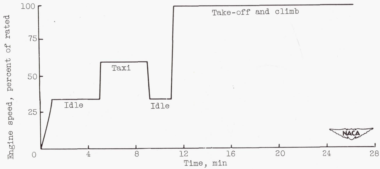
Figure 21. - Take-off sequence for turbojet engine.
