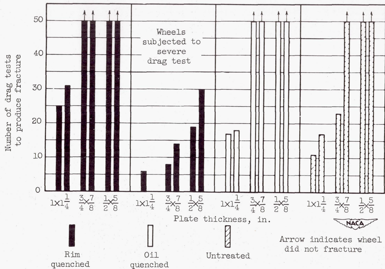
Figure 41. - Effect of plate thickness on number of drag tests required to produce fracture.
