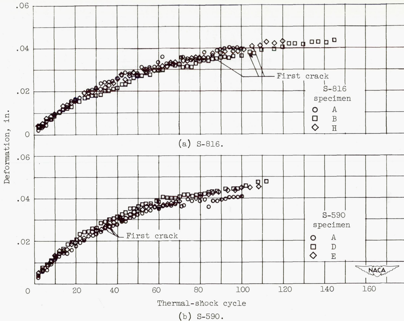
Figure 16. - Deformation produced in specimens by thermal shock.
