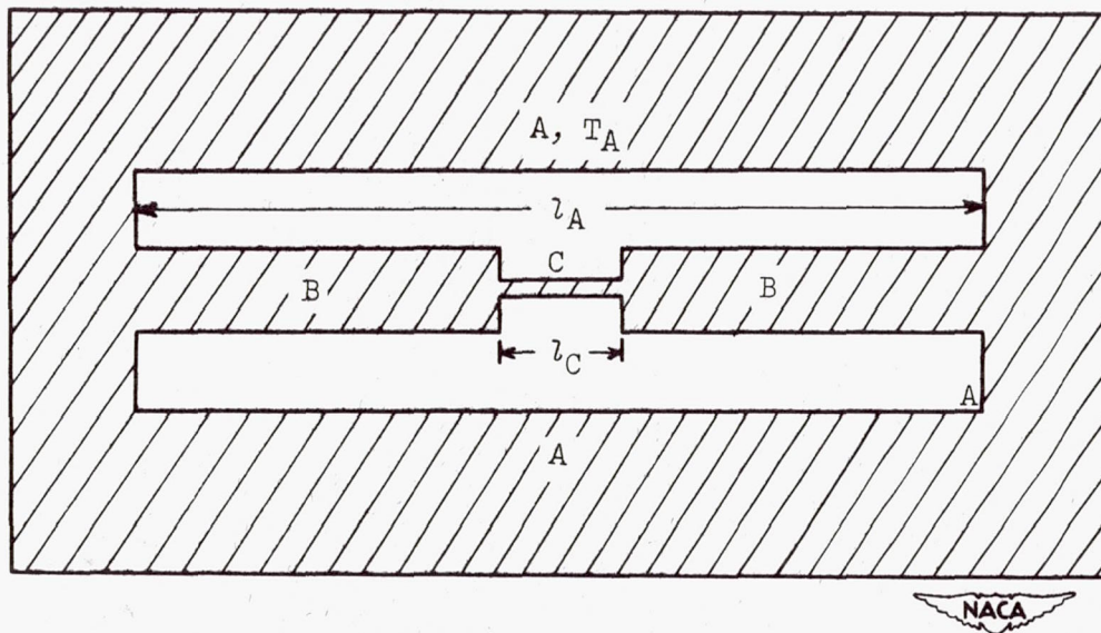
Figure 43. - Cross section of body in which large stress and strain are induced in small member as a result of temperature change in large member.
