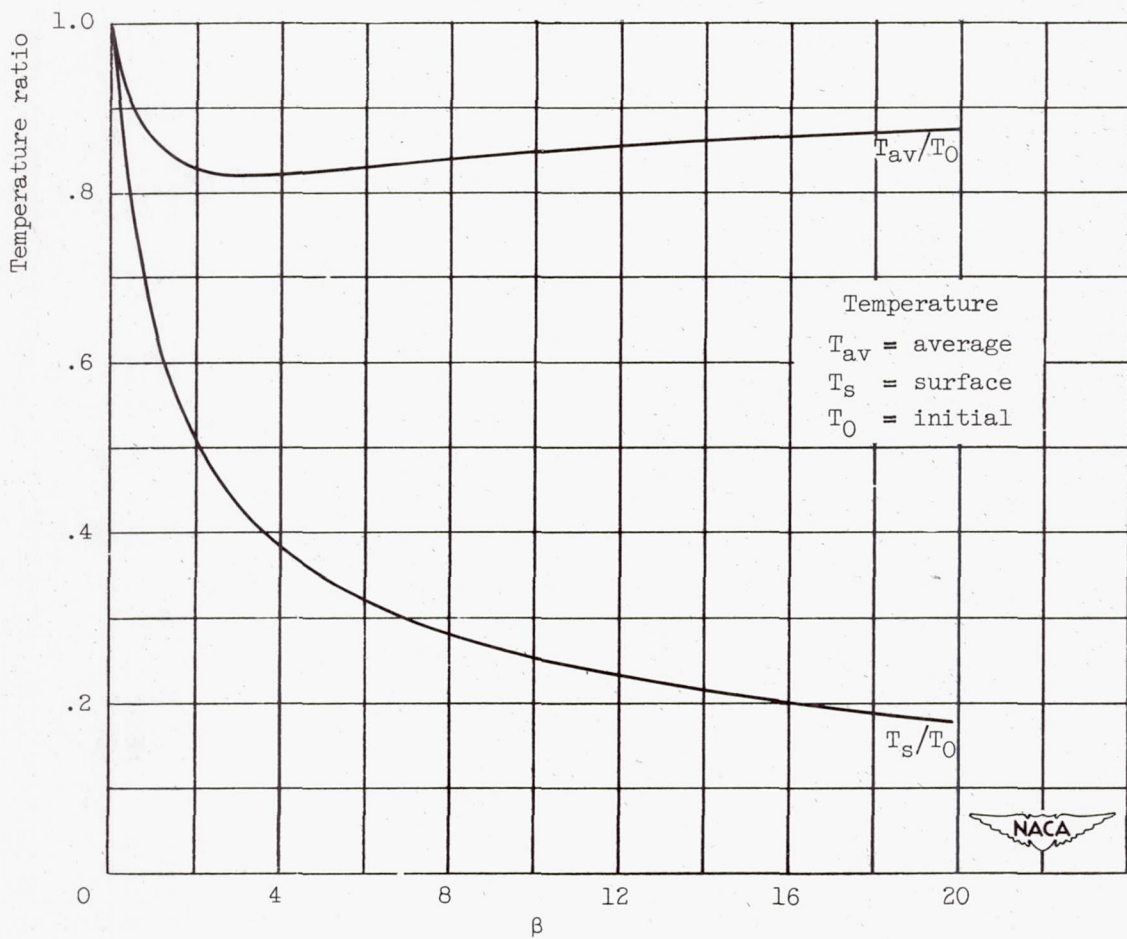
Figure 9. - Temperature ratio at time of maximum surface stress.
