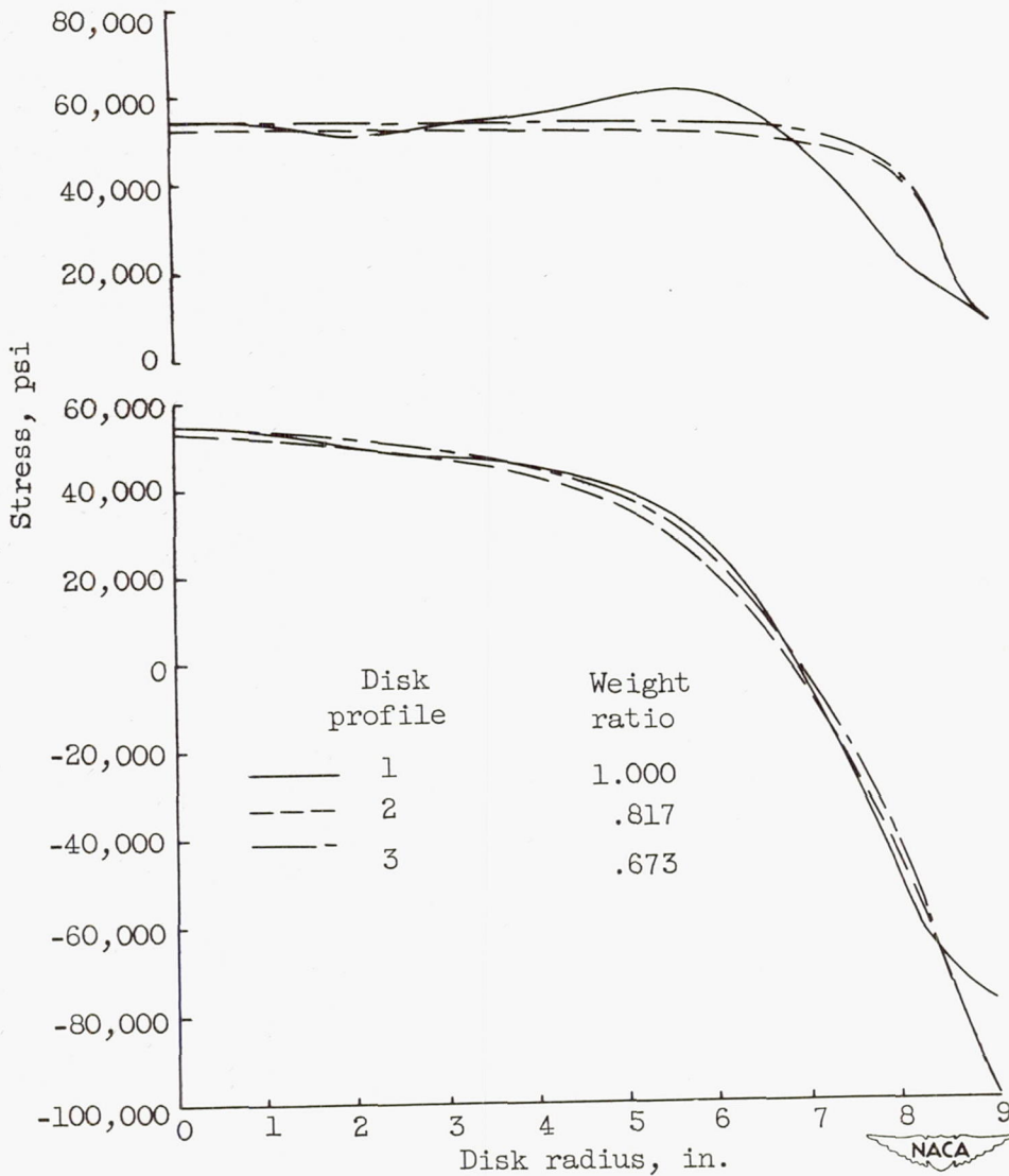
Figure 42. - Elastic stress distribution for various disk profiles.
