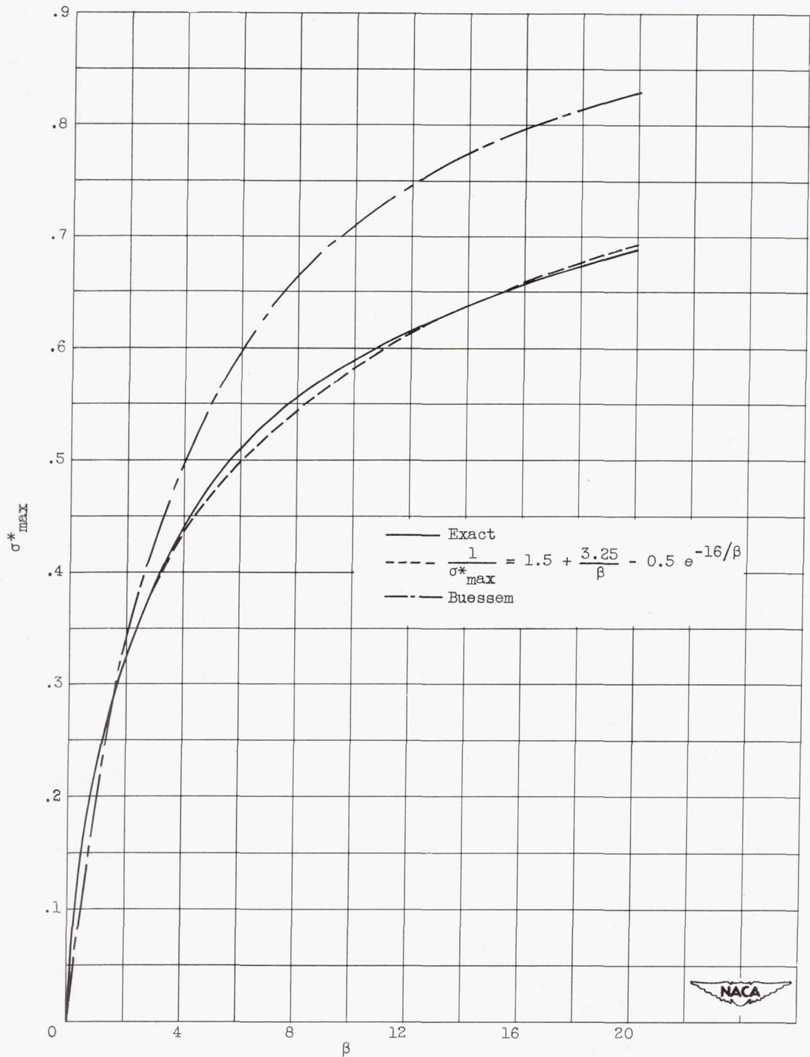
Figure 5. - Correlation of approximate formulas with exact solution for maximum stress.
