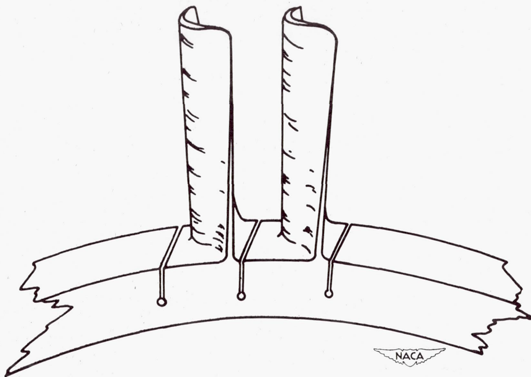
Figure 35. - Welded blade attachment with keyhole slots.
