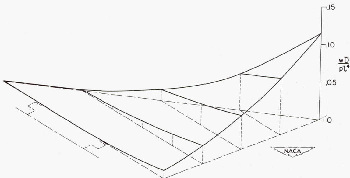
(b) Uniform-load deflections computed from experimental influence coefficients of table 2.
