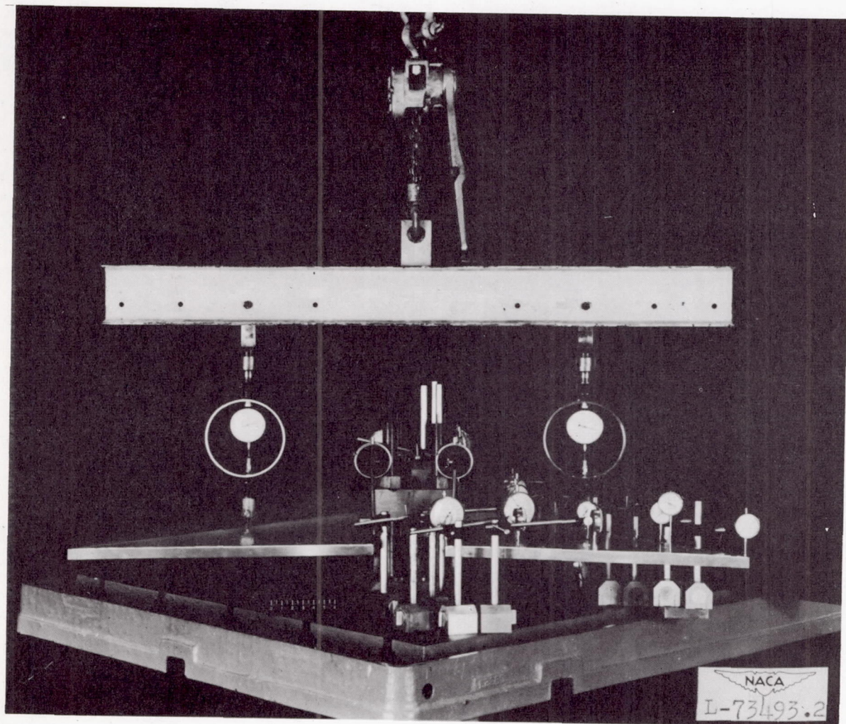
Figure 4.- Test setup.
