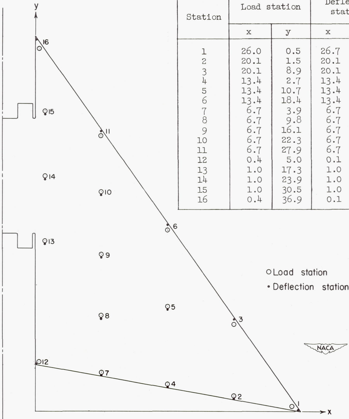
Figure 3.- Location of load and deflection stations.
