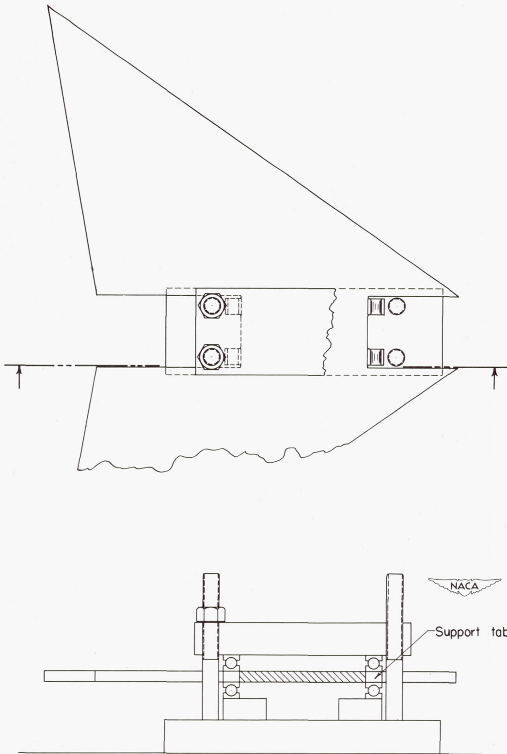
Figure 2.- Method of supporting the delta wings.
