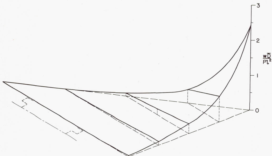
(a) Tip-load deflections.
