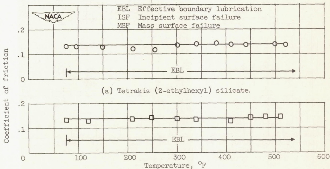
Figure 10. - Effect of temperature on friction of steel specimens boundary-lubricated with silicate ester. Load, 1000 grams; sliding velocity, 120 feet per minute.
