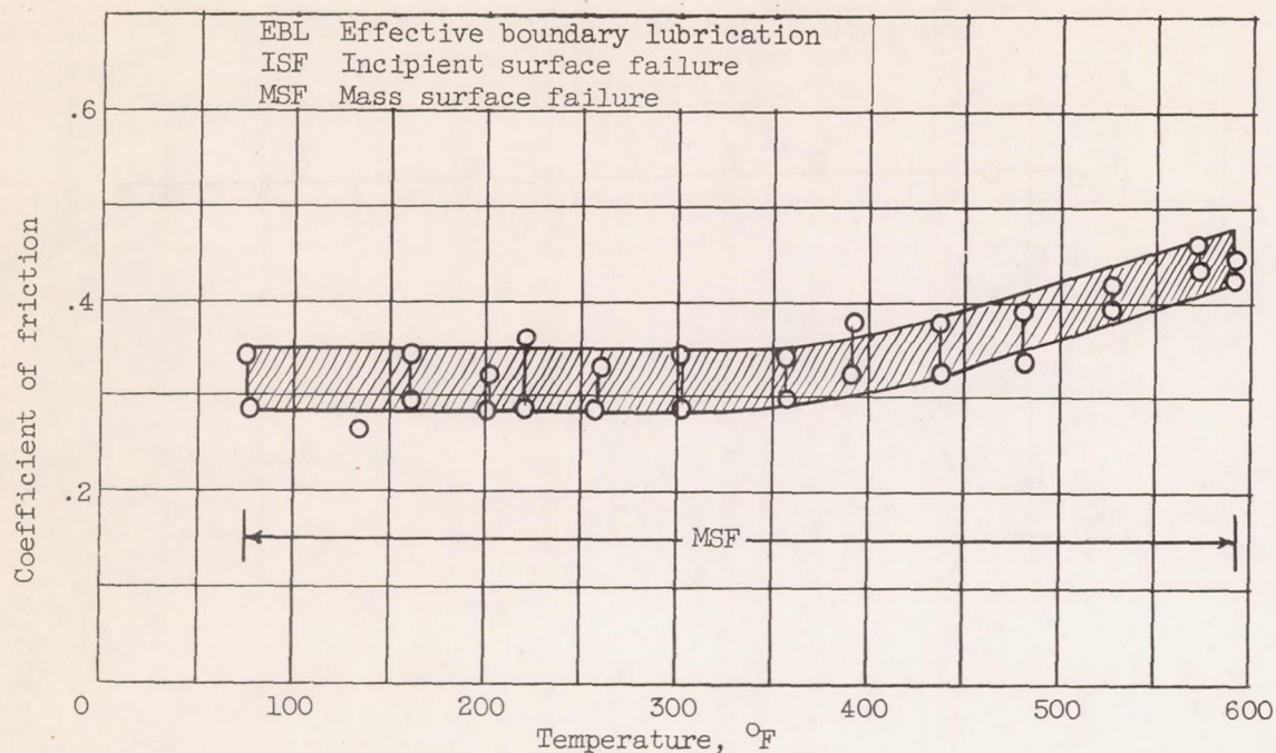
Figure 11. - Effect of temperature on friction of steel specimens boundary-lubricated with 50-centistoke (at 25° C) silicone fluid. Load, 1000 grams; sliding velocity, 120 feet per minute.
