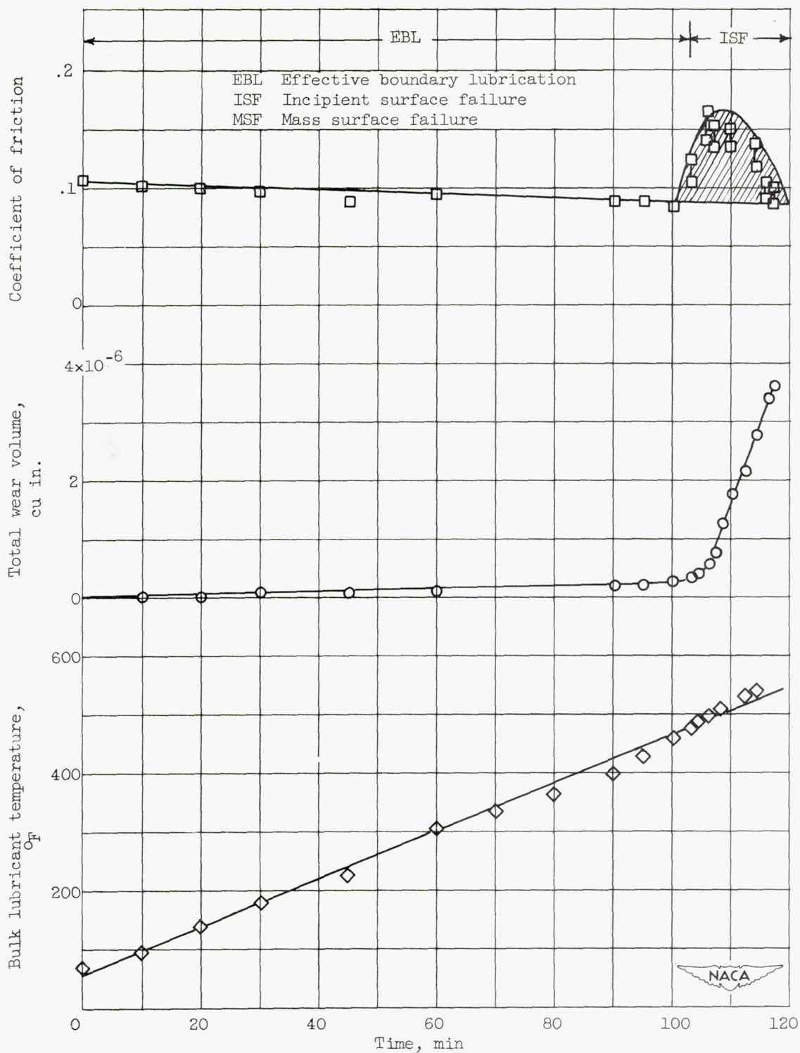
Figure 3. - Relation between unstable friction (cross-hatched area) and wear for typical diester lubricant at increasing bulk temperatures. Load, 1000 grams; sliding velocity, 120 feet per minute.
