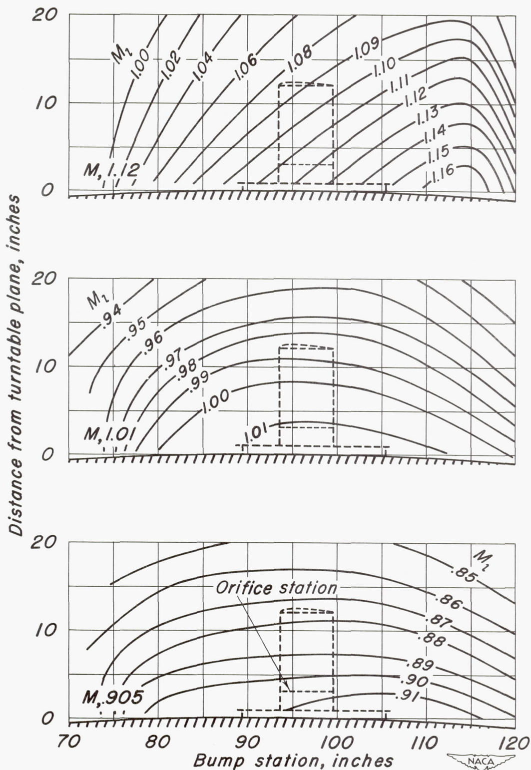
Figure 4.- Typical Mach number contours over the Ames 16-foot tunnel transonic bump.
