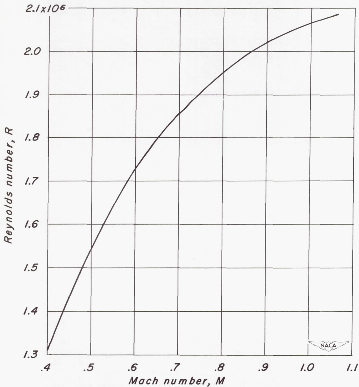
Figure 3.- Variation of Reynolds number with Mach number during the 16-foot wind-tunnel test of the NACA 0015 airfoil model.
