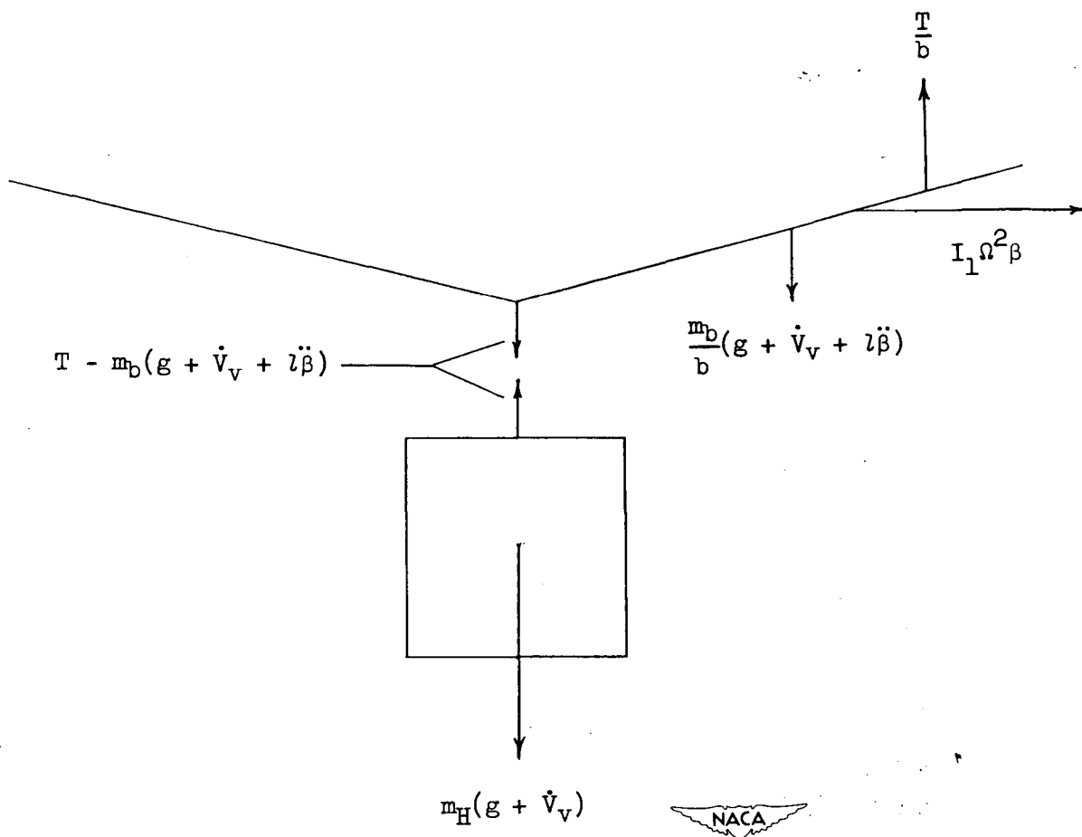
Figure 2.- Schematic diagram showing forces acting on helicopter.
