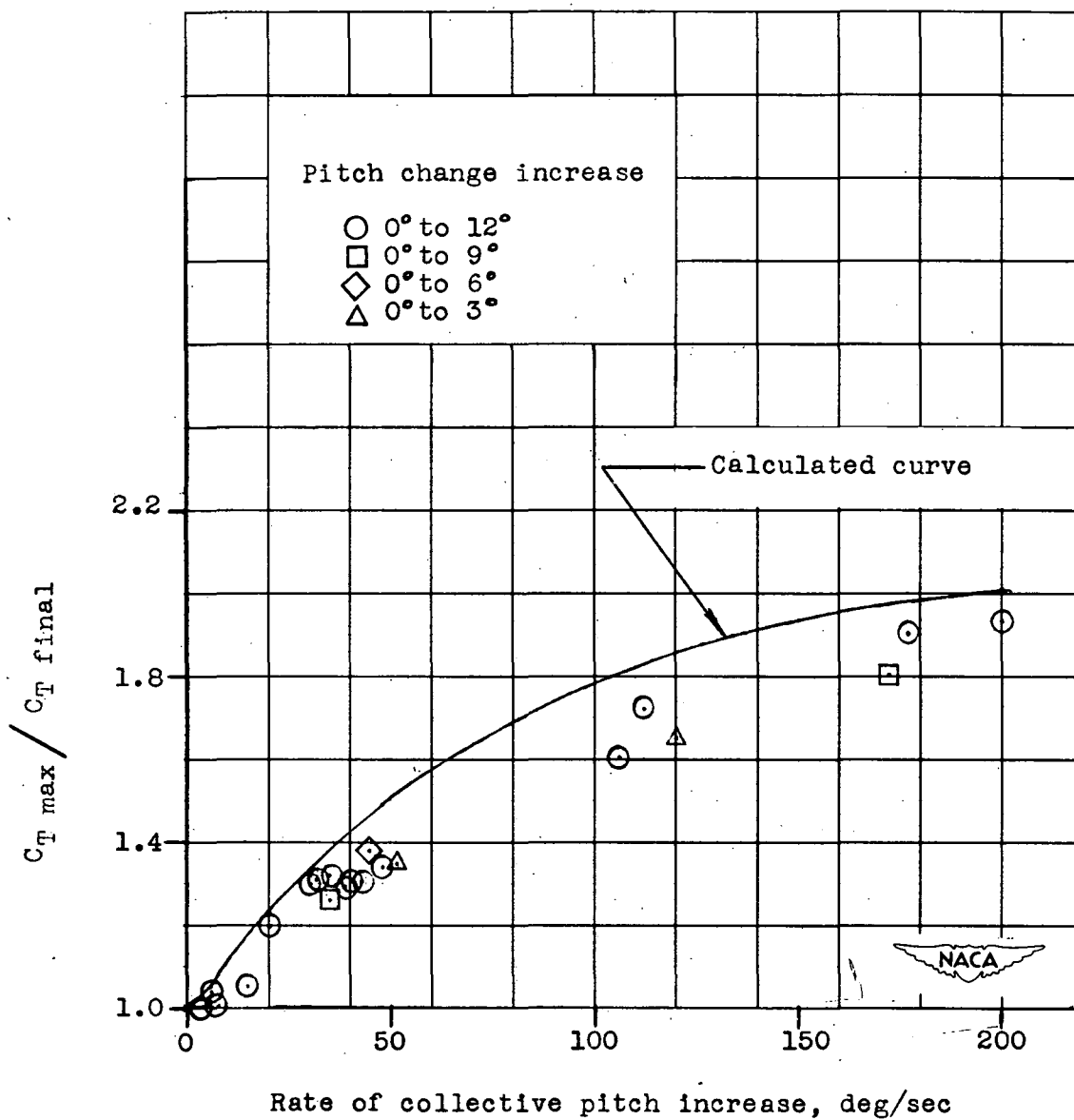
Figure 5.- Comparison of experimental and calculated ratios of C_{T \max} / C_{T \text{ final}} for various rates of collective pitch increase.
