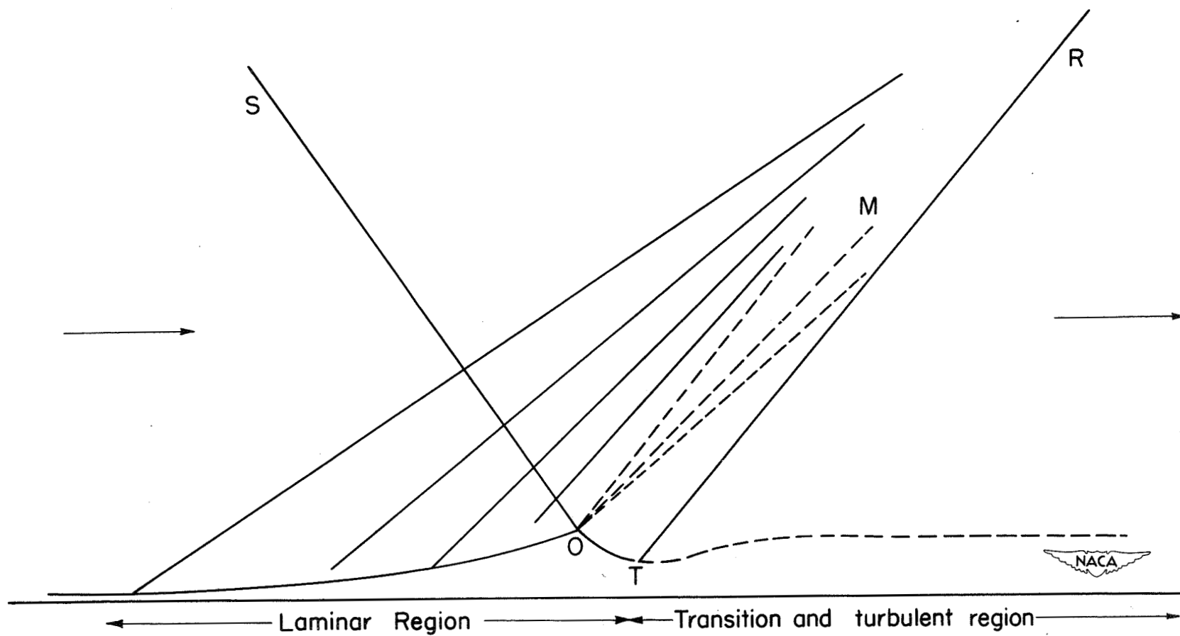
Figure 2.- Sketch of flow field according to first-order theory.
