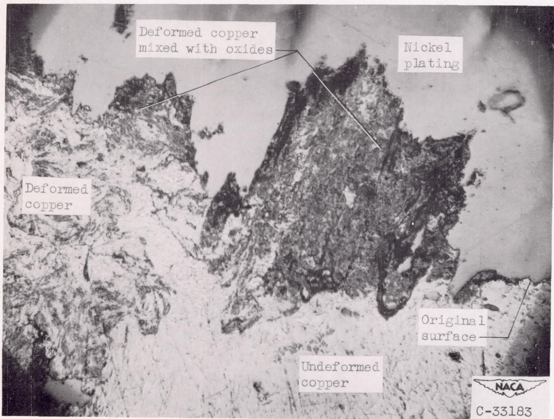
Figure 4. - Photomicrograph of taper section of fretted area of copper specimen fretted against copper for 330 cycles. Horizontal magnification, X500; vertical magnification, approximately X7500.
