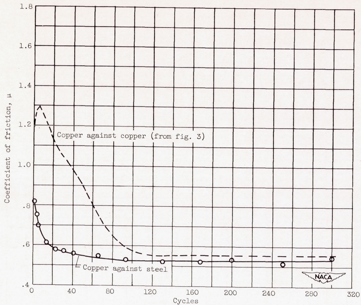
Figure 8. - Friction during fretting of copper against steel.
